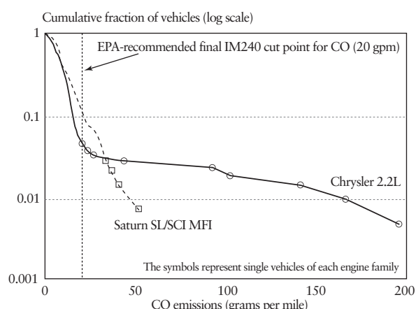
FIGURE 3 CO Emissions Distributions of Two Car Models
