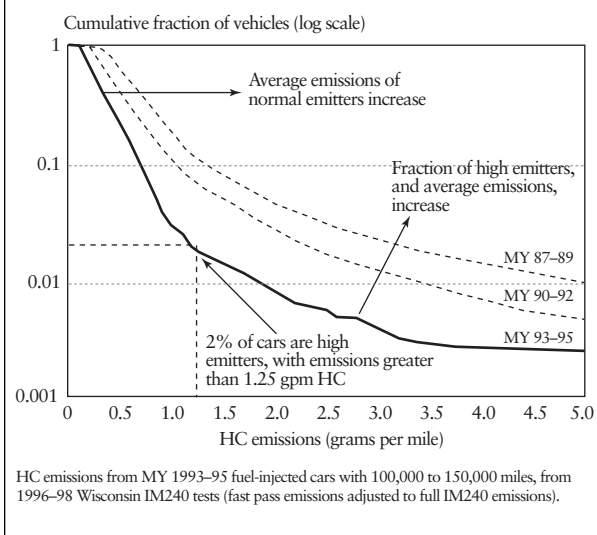
FIGURE 2 Trends in HC Emissions Distributions as Vehicles Age
