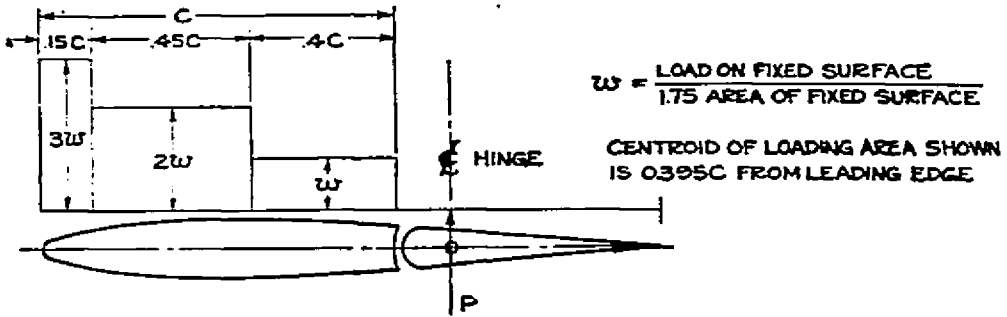
FIG 04-4 "BALANCING" DISTRIBUTION - HORIZONTAL TAIL
