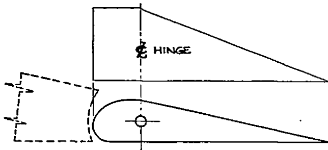
FIG. 04-7 AILERON LOAD DISTRIBUTION
