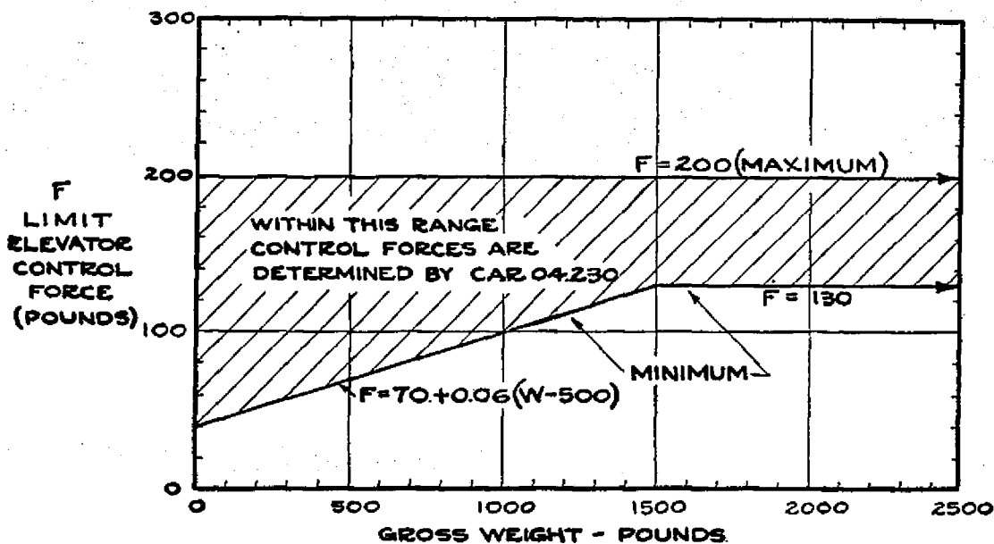
FIG. 04-8 ELEVATOR CONTROL FORCE LIMITS
