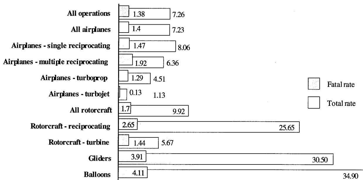
Chart 4. Number of accidents and fatal accidents (top), accident rates and fatal rates per 100,000 aircraft hours flown (bottom), 1997. (See Charts 28 through 37 in appendix.)
