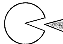
Accidents
