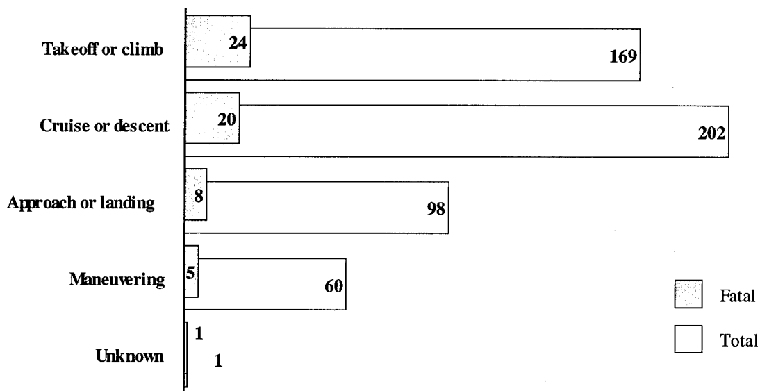
Chart 15. First phase of operation for the 530 aircraft that experienced loss of engine power, 1997.
