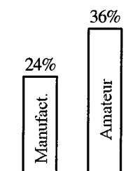
Destroyed aircraft
