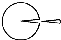
Hours flown
