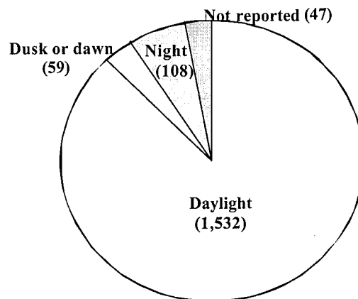
VMC
