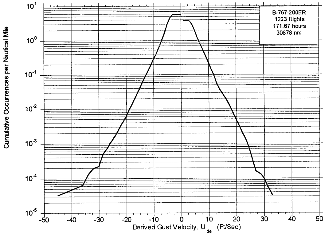
FIGURE A-41. CUMULATIVE OCCURRENCES OF DERIVED GUST VELOCITY PER NAUTICAL MILE, FLAPS EXTENDED
