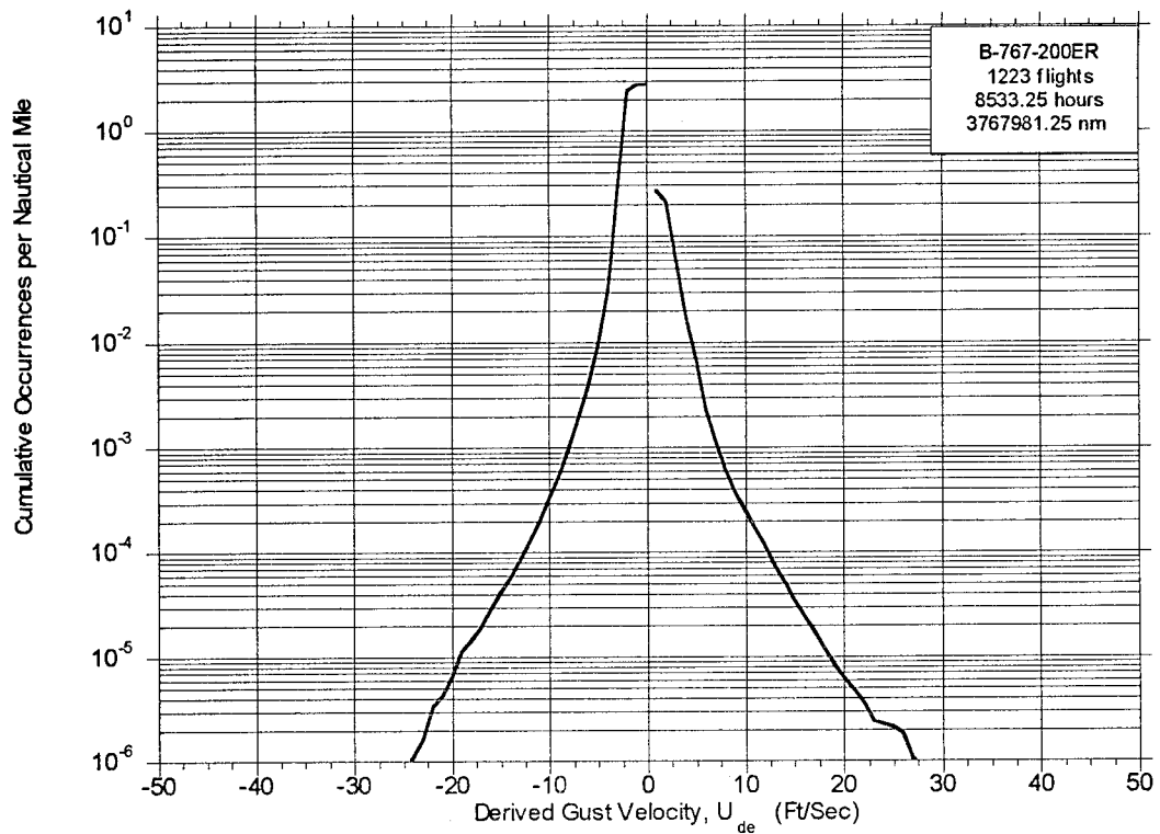
FIGURE A-42. CUMULATIVE OCCURRENCES OF DERIVED GUST VELOCITY PER NAUTICAL MILE, FLAPS RETRACTED
