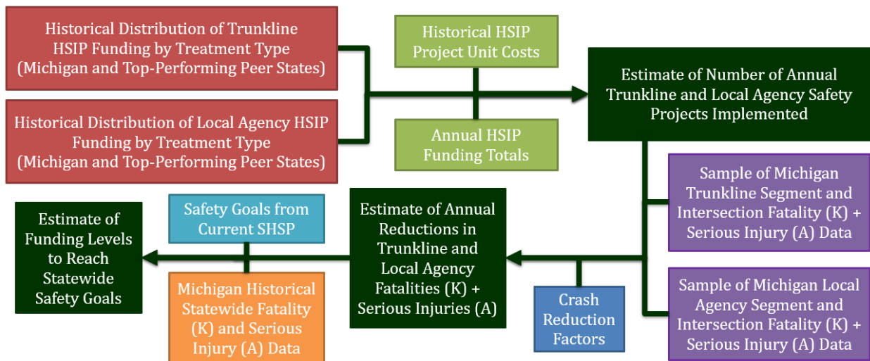
Figure 28. Flowchart of Estimation Process
