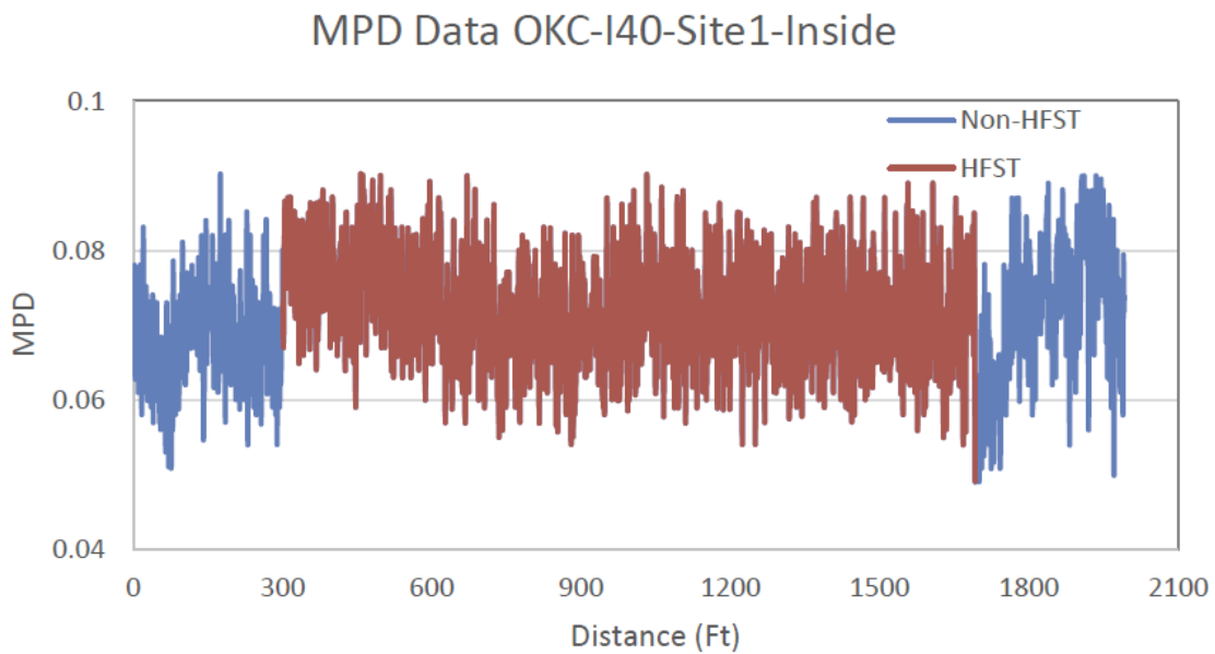
Figure C13: Mean Profile Depth, Site 1, Inside Lane
