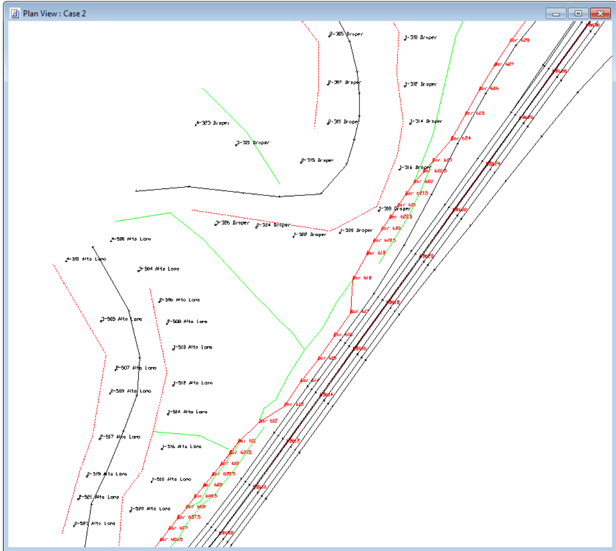
Figure 21. FHWA TNM Plan View of a portion of a model of a study area.
