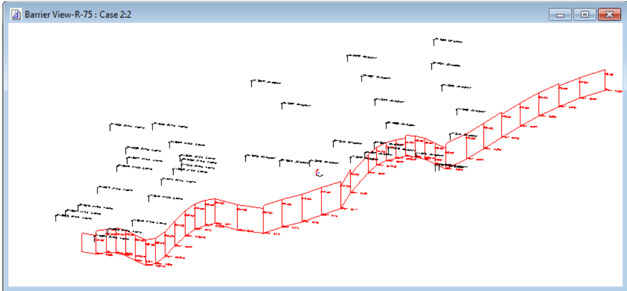
Figure 22. FHWA TNM Barrier View of a noise barrier design.
