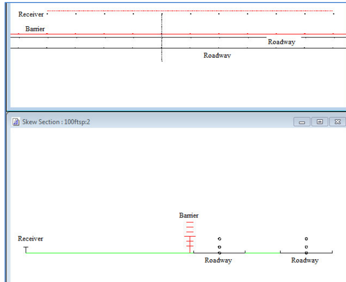
Figure 28. Plan view (top) and cross-sectional view (bottom) of roadways and noise barrier portion of FHWA TNM model for sensitivity test cases.
