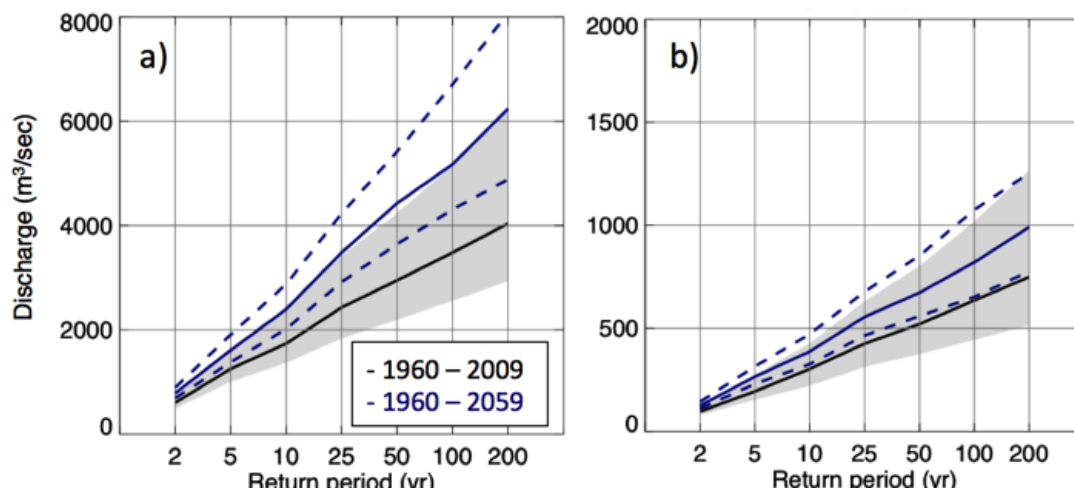
Figure 6. Iowa DOT, current and future ranges for quantiles of peak flow for Cedar River Basin (left) and South Skunk River Basin (right). Shaded region and solid black line demark the 95 th confidence interval and median for 1960-2009. Blue dashed and solid lines demark the 95 th confidence interval and median for 1960-2059. (Source: Iowa DOT)
