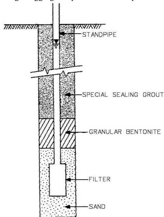
Figure 15-30 Schematic of Open Standpipe Piezometer Installed in Borehole (After Dunnycliff, 1988, 1993)
