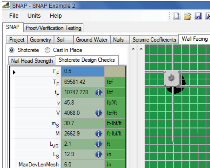
Figure 77. Screen Shot. Example 2, the Shotcrete Design Checks tab.
