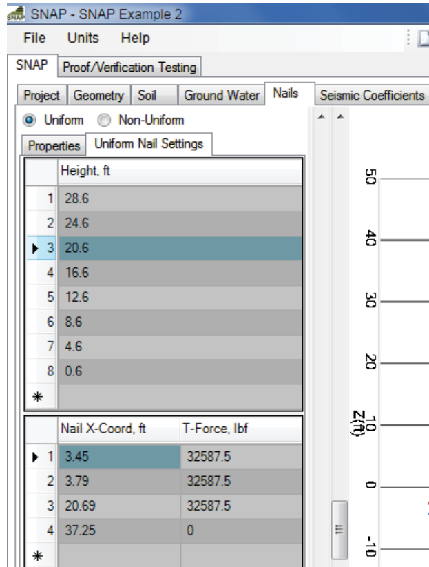
Figure 74. Screen Shot. Example 2, the Uniform Nail Settings tab.
