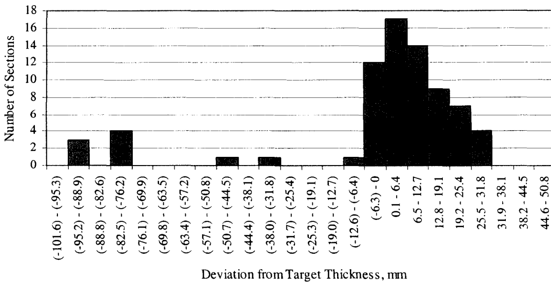
Figure 4: Chart. Example of a skewed distribution for layer thickness deviation (core data, PCC, target thickness 279 mm [11 in]).
