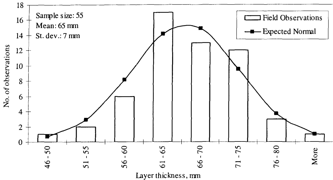
Figure 1: Chart. Example distribution of layer thickness measurements along the section for AC surface and binder layer for the SPS-1 Section 55-0118.
