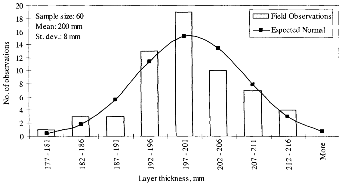
Figure 2: Chart. Example distribution of layer thickness measurements along the section for PCC surface layer for the SPS-8 Section 39-0809.
