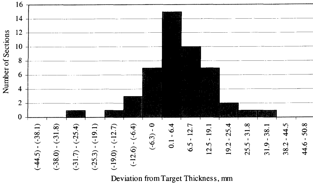
Figure 3: Chart. Example of normally distributed thickness deviations (elevation data, LC, target thickness 152 mm [6 in]).
