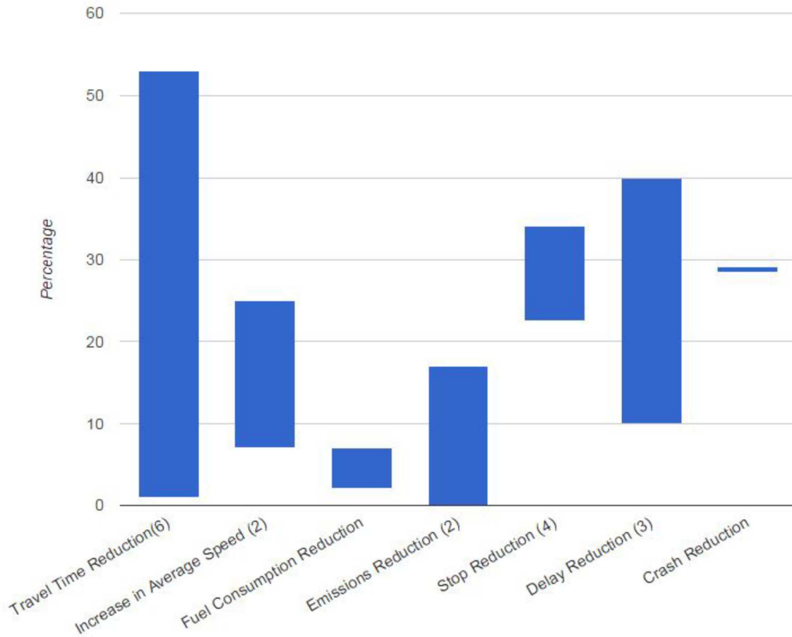
Figure 3-2 Adaptive Signal Control Benefits Found in the Knowledge Resource Database from 2003 to 2016 (ITS Knowledge Resources)
