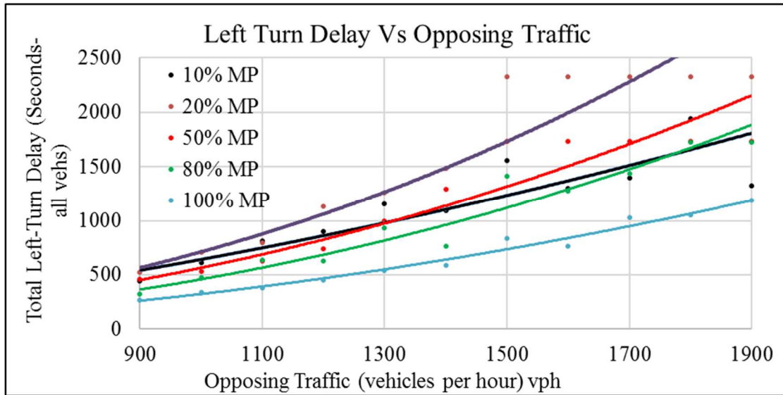
Figure E-9 Relationship between Left-Turn Delay and Opposing Traffic with Different CV Market Penetration (MP)
