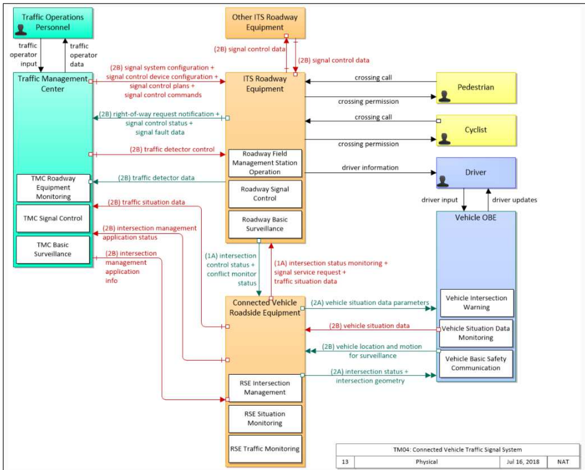
Figure 4-4 TM04 Connected Vehicle Traffic Signal System (ARC-IT 8.2, 2019)
