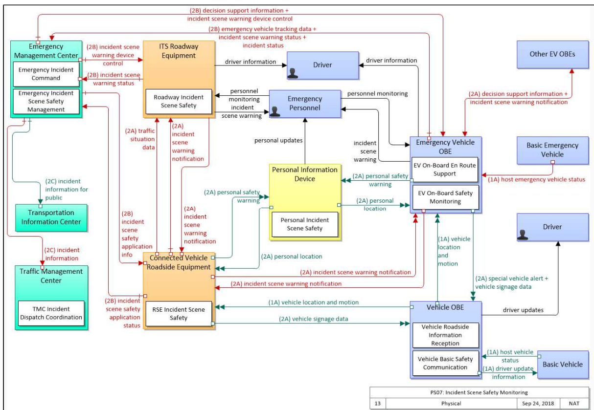
Figure 4-8 PS07 Incident Scene Safety Monitoring (ARC-IT 8.2, 2019)
