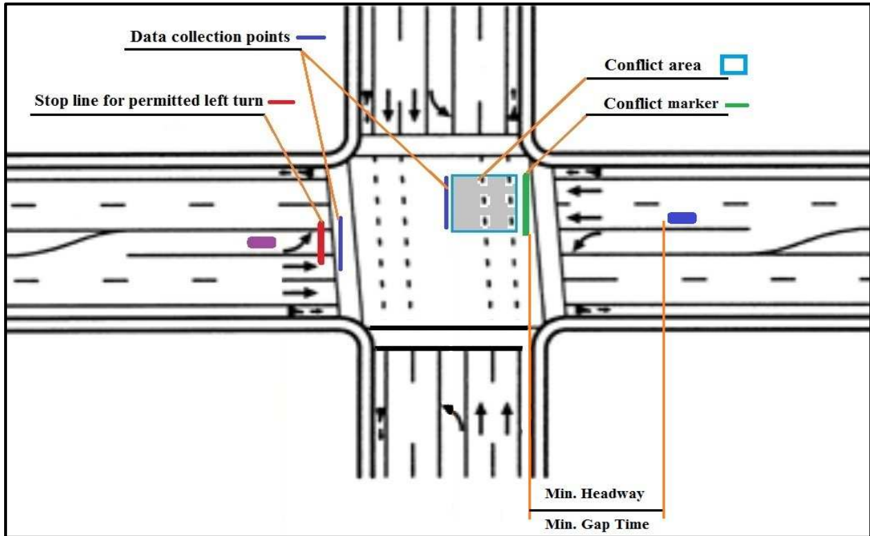
Figure 5-16 Priority Rule Application in VISSIM
