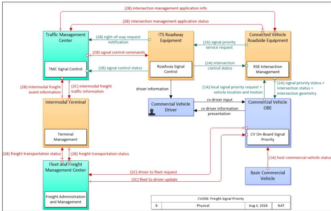
Figure 4-5 CVO06 Freight Signal Priority (ARC-IT 8.2, 2019).
