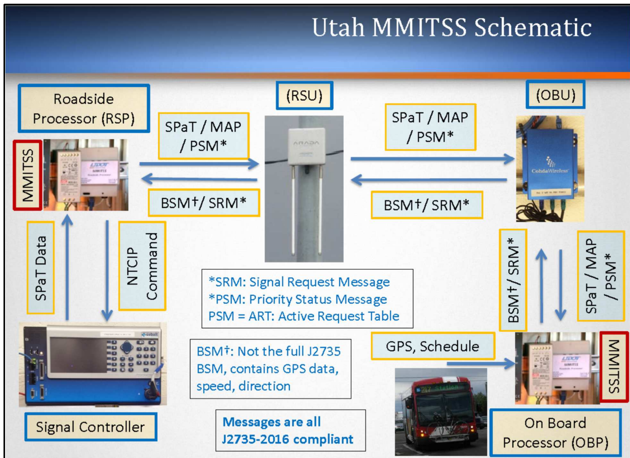
Figure 4-11 The CV-Based Transit Signal Priority Implementation in Utah (Leonard, 2002)
