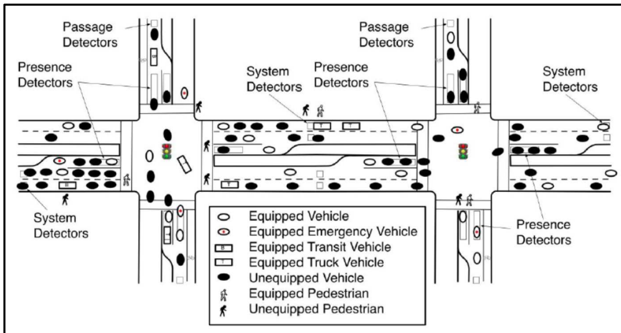
Figure 2-6 Illustration of the MMITSS Concept (University of Arizona et al., 2012)
