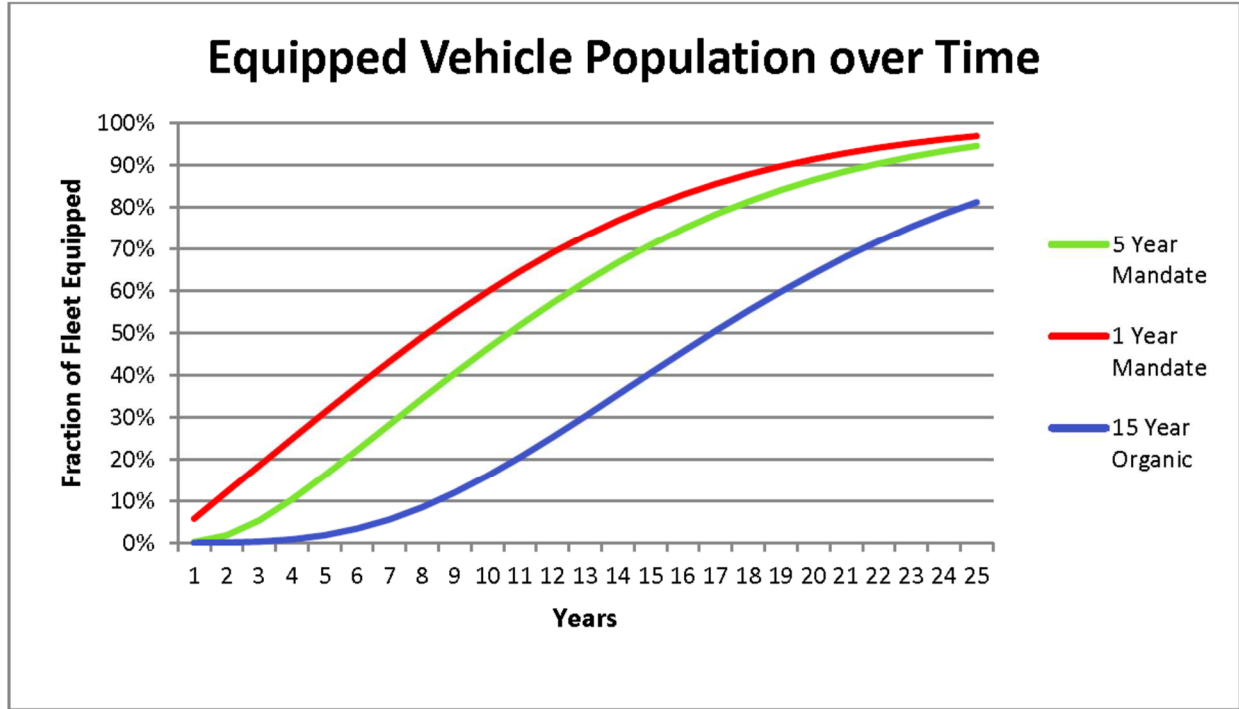
Figure 4-2 Equipped Vehicle Population Over Time (Wright et al., 2014)
