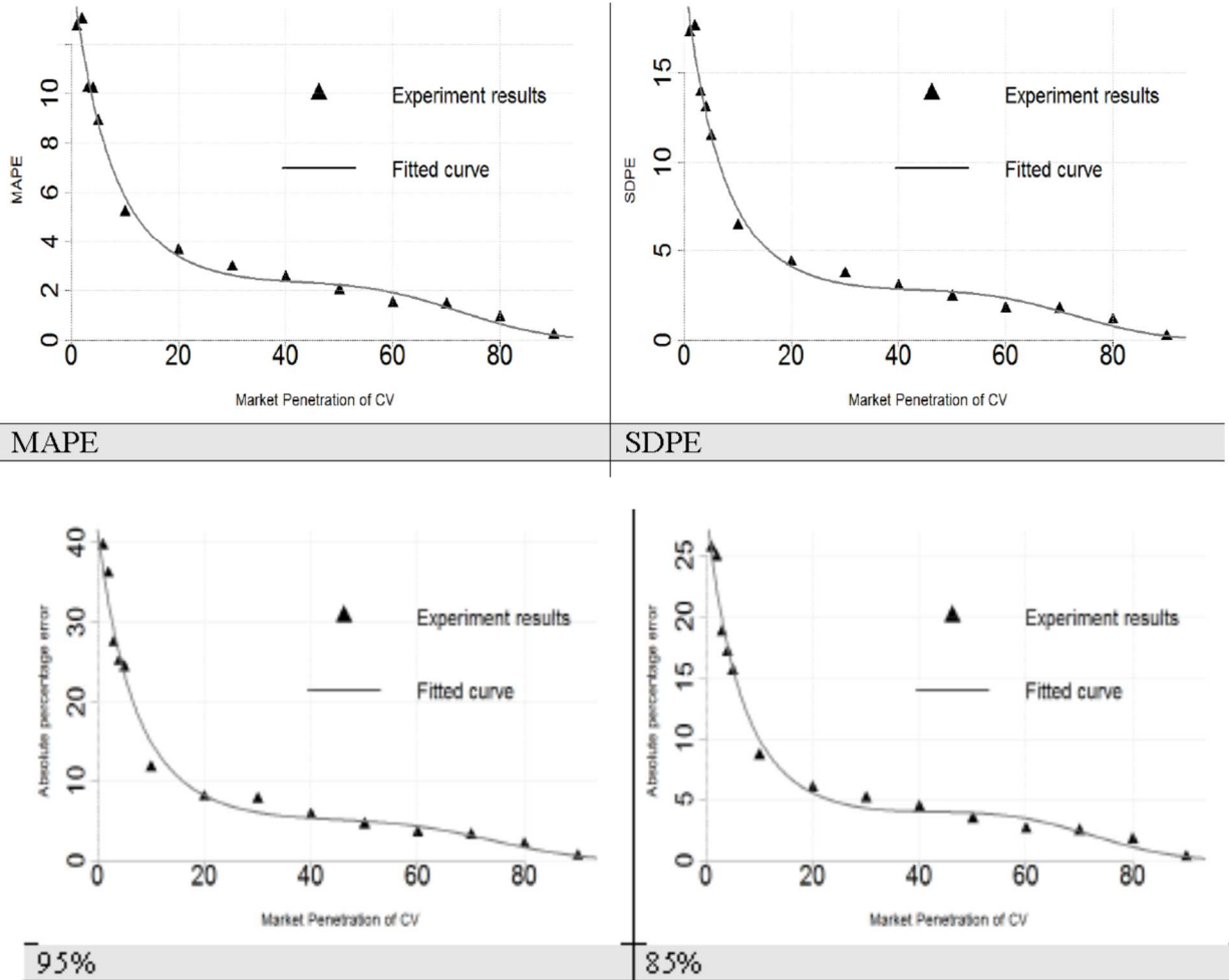
Figure 3-1 Travel Time Accuracy as a Function of CV Market Penetration for an Arterial Segment (Iqbal et al., 2017)
