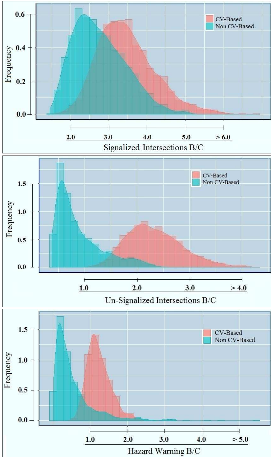
Figure 5-10 Distribution of the benefits of the existing and CV-Based solutions
