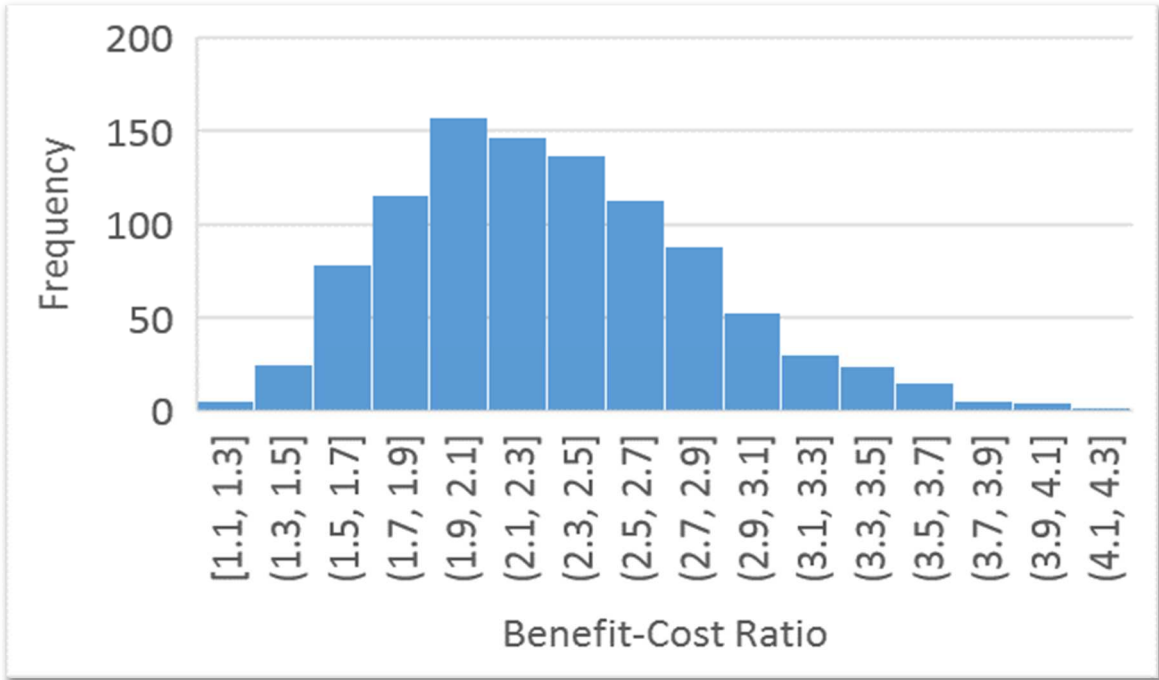
Figure E-2 Distribution of Benefit-Cost Ratios for CV-Based Unsignalized Intersection
