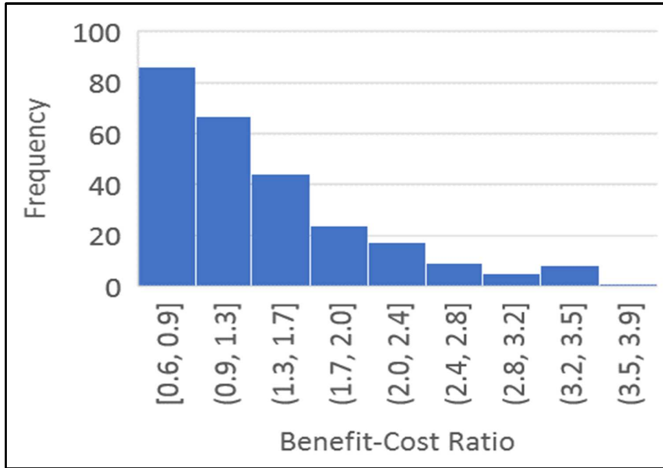
Figure 5-8 Distribution of Benefit-Cost Ratios for GLOSA
