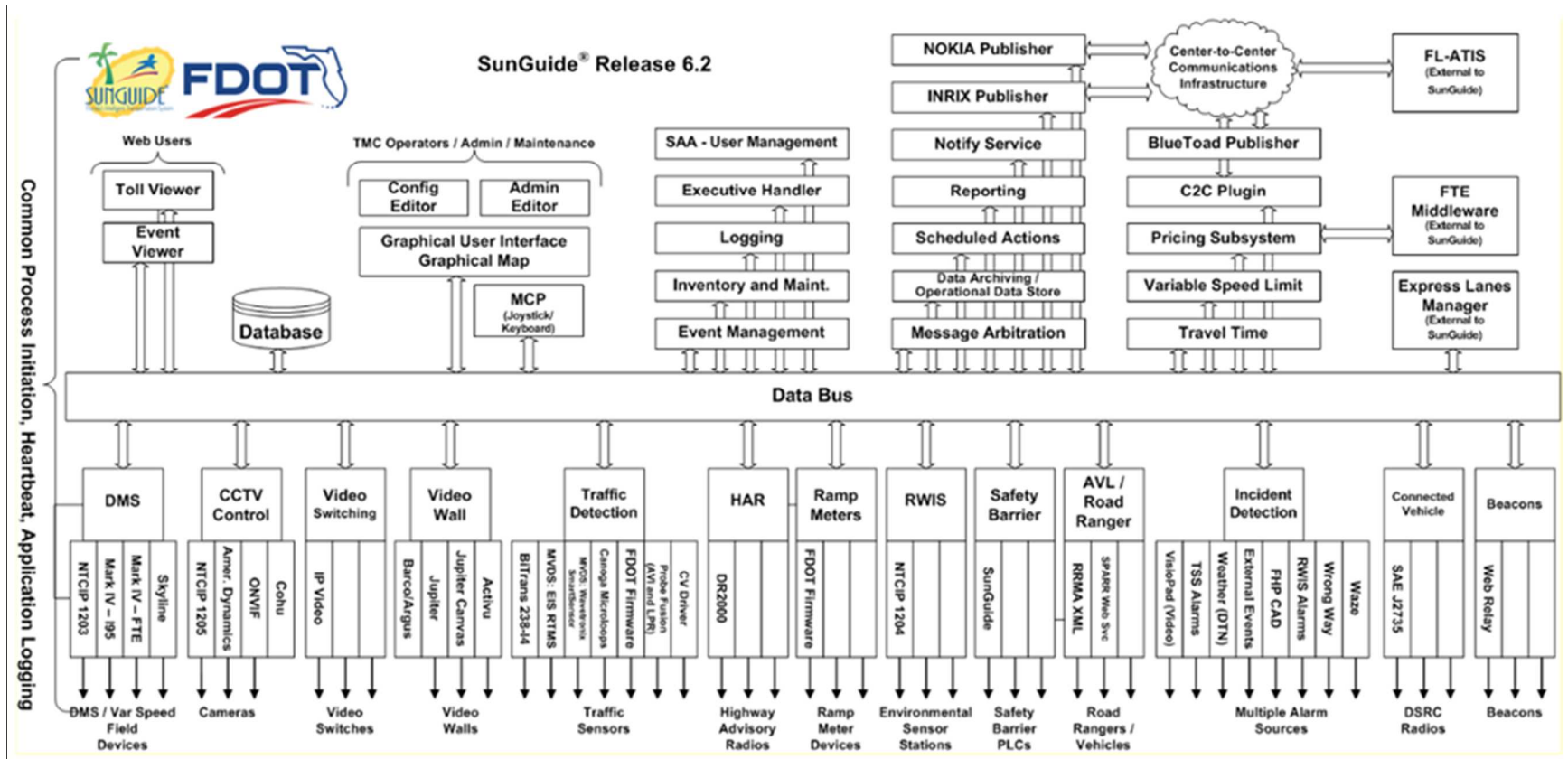
Figure 4-9 SunGuide® Software Architecture
