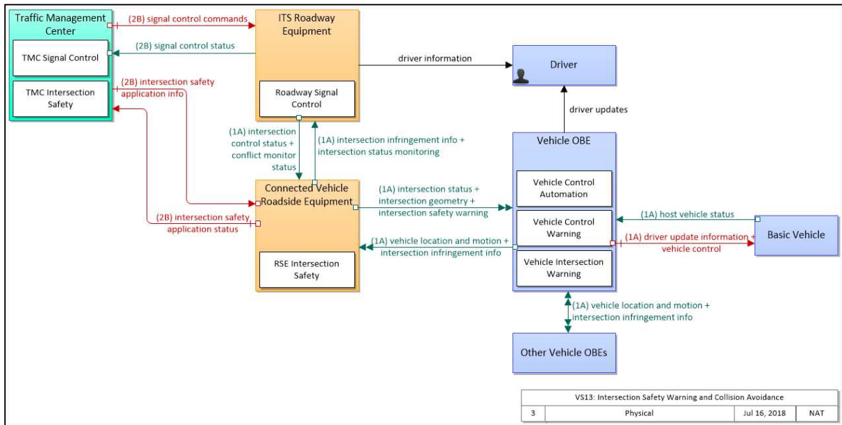
Figure 4-7 VS13 Intersection Safety Warning and Collision Avoidance (ARC-IT 8.2, 2019).
