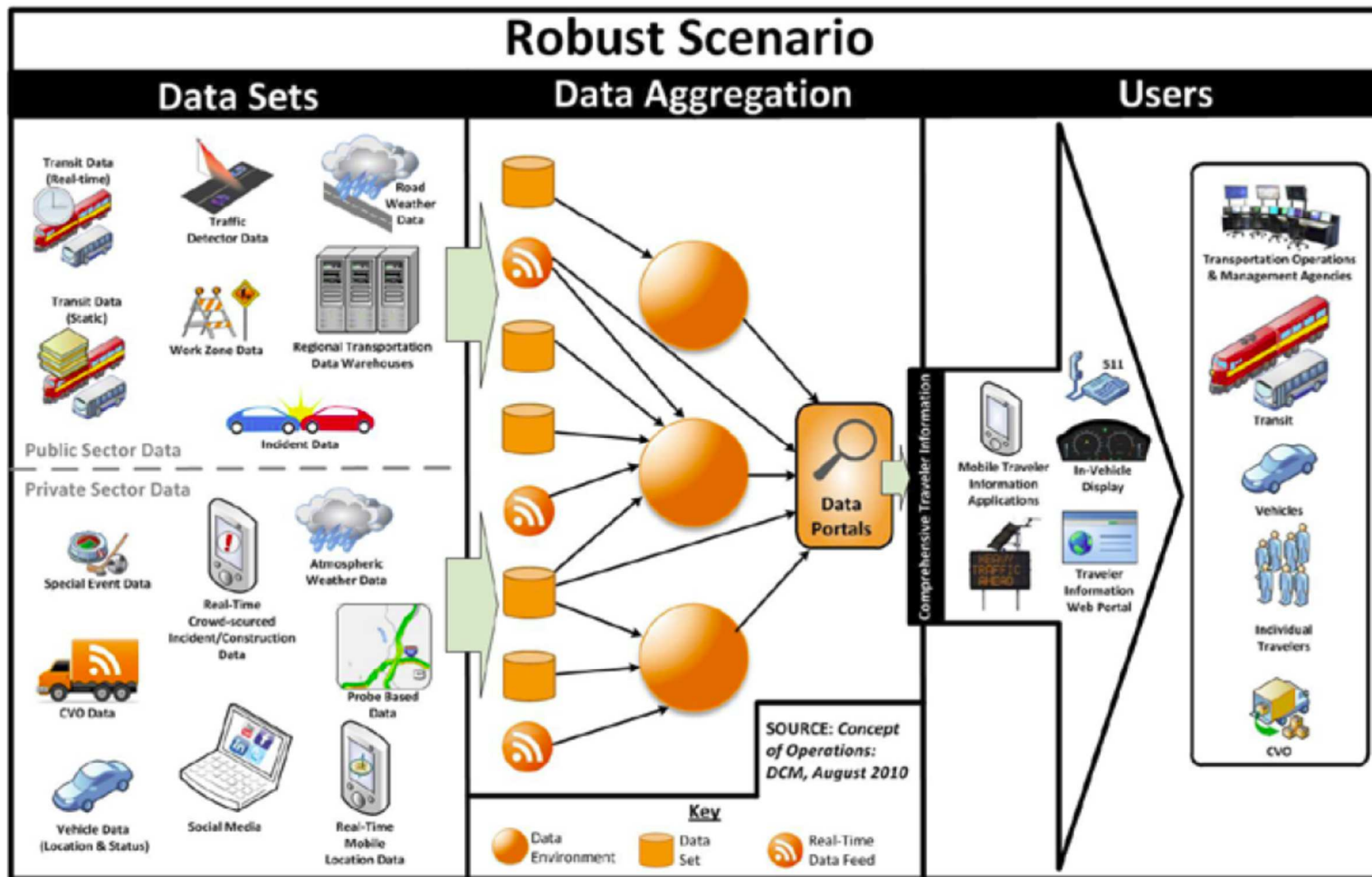
Figure 3-6 Robust EnableATIS Operational Scenario (Burgess et al., 2012)
