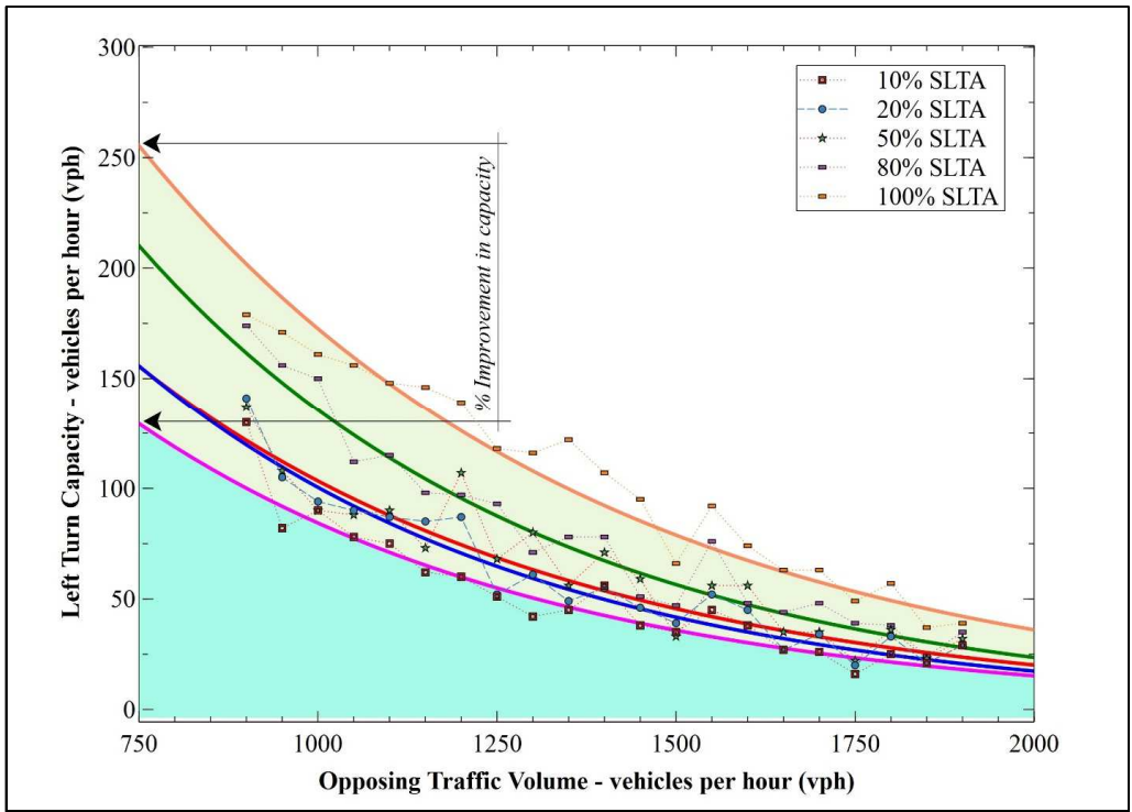
Figure 5-19 Impact of SLTA on Left-Turn Capacity
