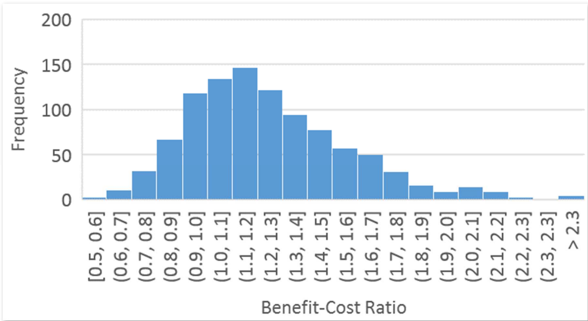
Figure 5-5 Distribution of Benefit-Cost Ratios for CV-Based Unsignalized Intersection
