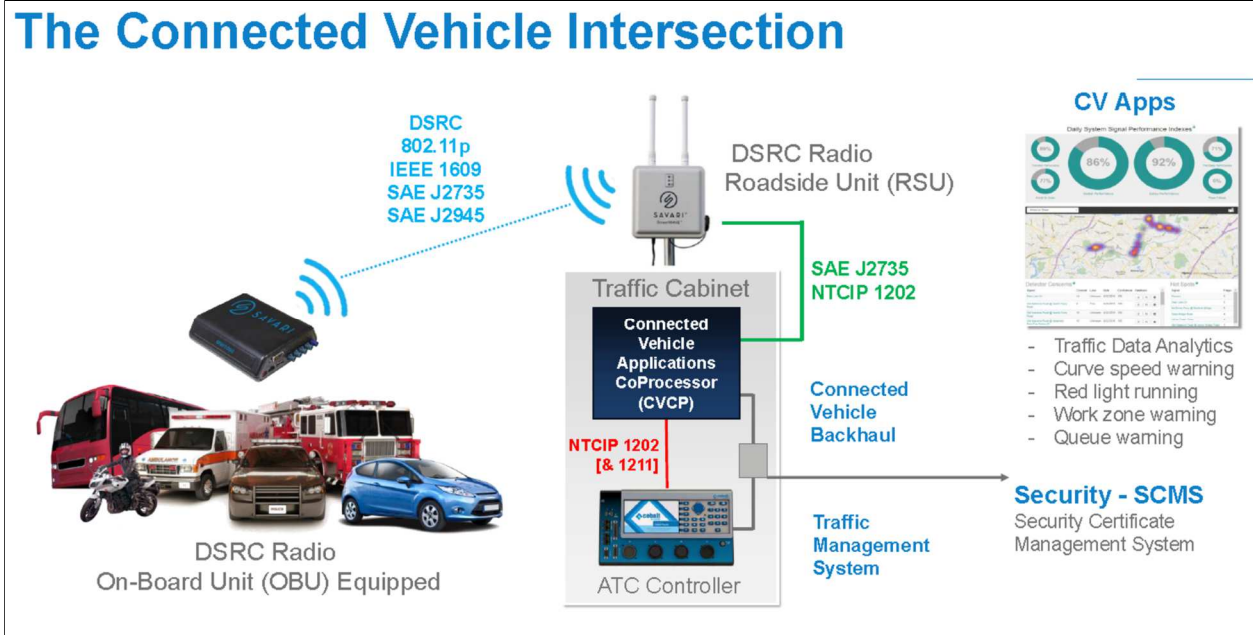
Figure 4-10 The Signal Controller and Econolite CV Co-Processor as Part of the Connected Vehicle Intersection (Provenzano, 2016; Mohaddes, 2017)
