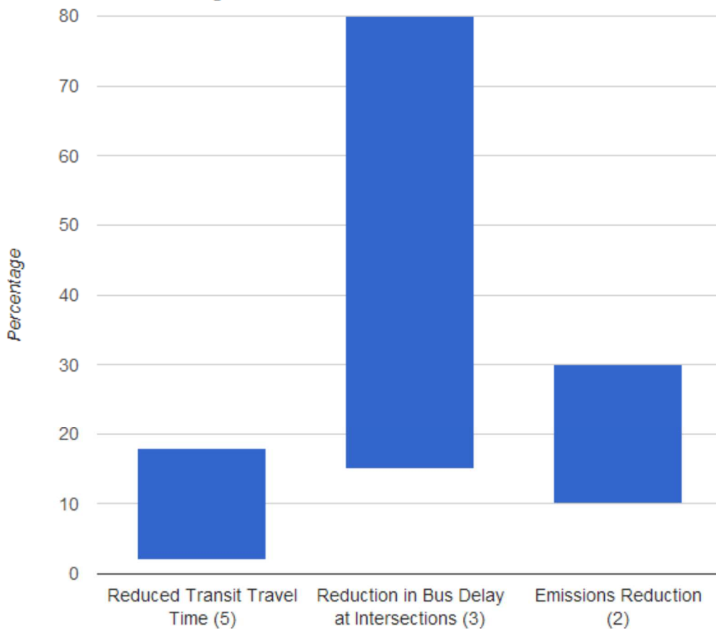
Figure 3-3 Benefits of Transit Signal Priority Systems (ITS Knowledge Resources)
