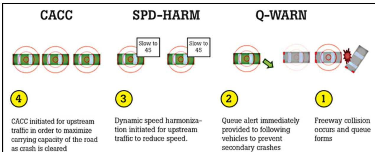
Figure 2-5 Combined Q-WARN/SPD-HARM/CACC Illustration (Mahmassani et al., 2012)
