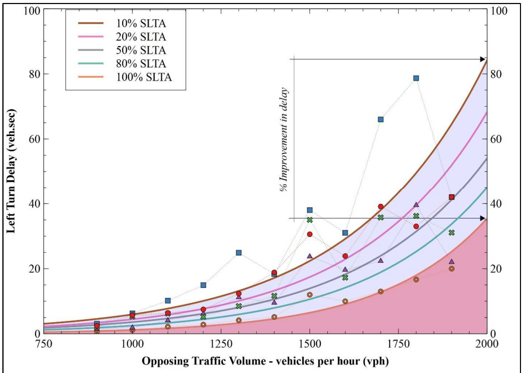
Figure 5-20 Relationship Between Left-Turn Delay and Opposing Traffic
