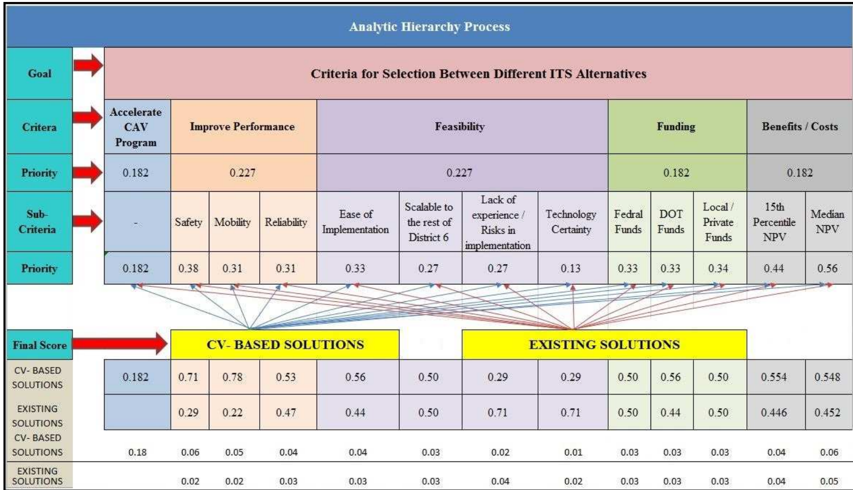
Figure A-2: Global Scores
