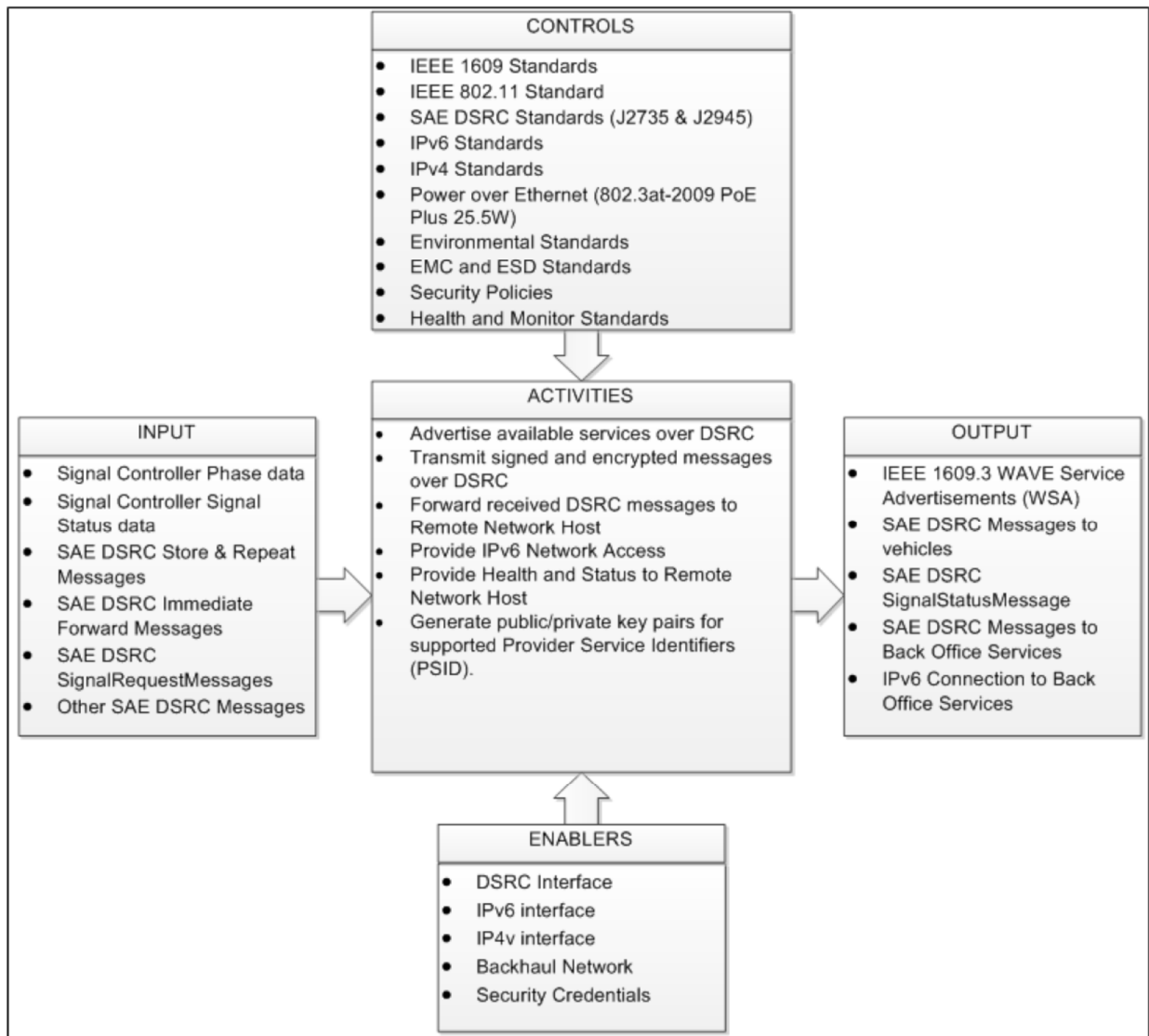
Figure 4-12 Context Diagram of an RSU (Chang, 2017)
