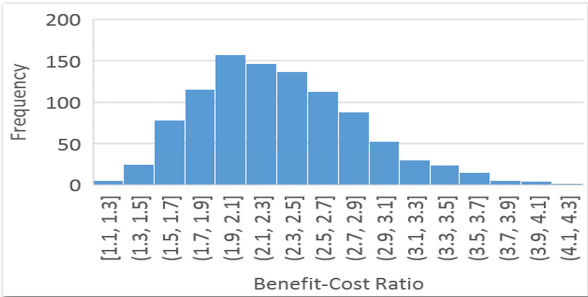
Figure 5-4 Distribution of Benefit-Cost Ratios for CV-Based Hazard Warning
