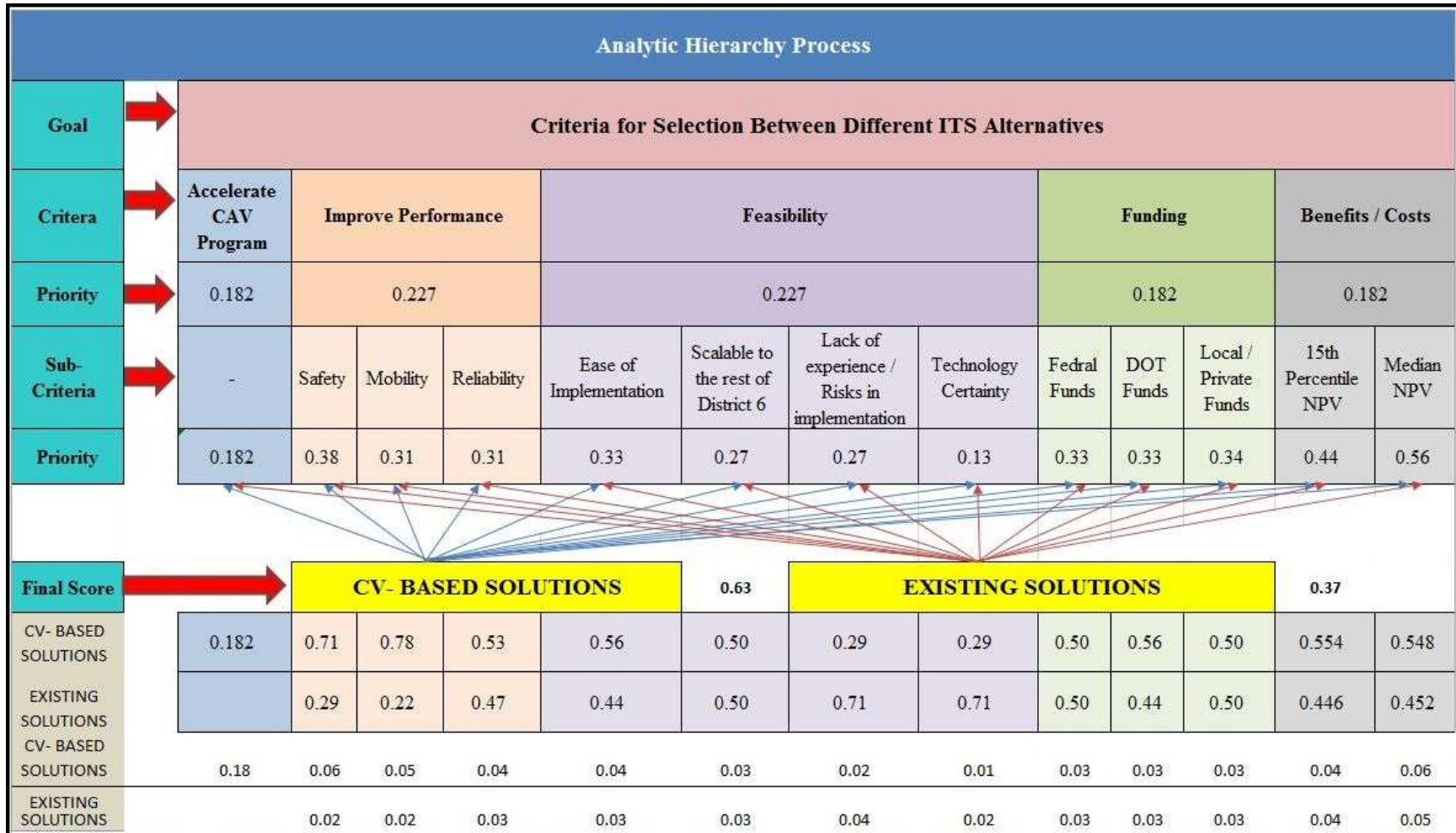
Figure A-3: AHP Results and Final Score
