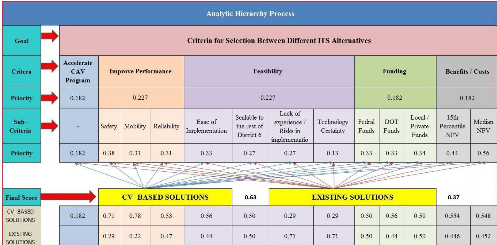
Figure E-7 AHP decision-making levels
