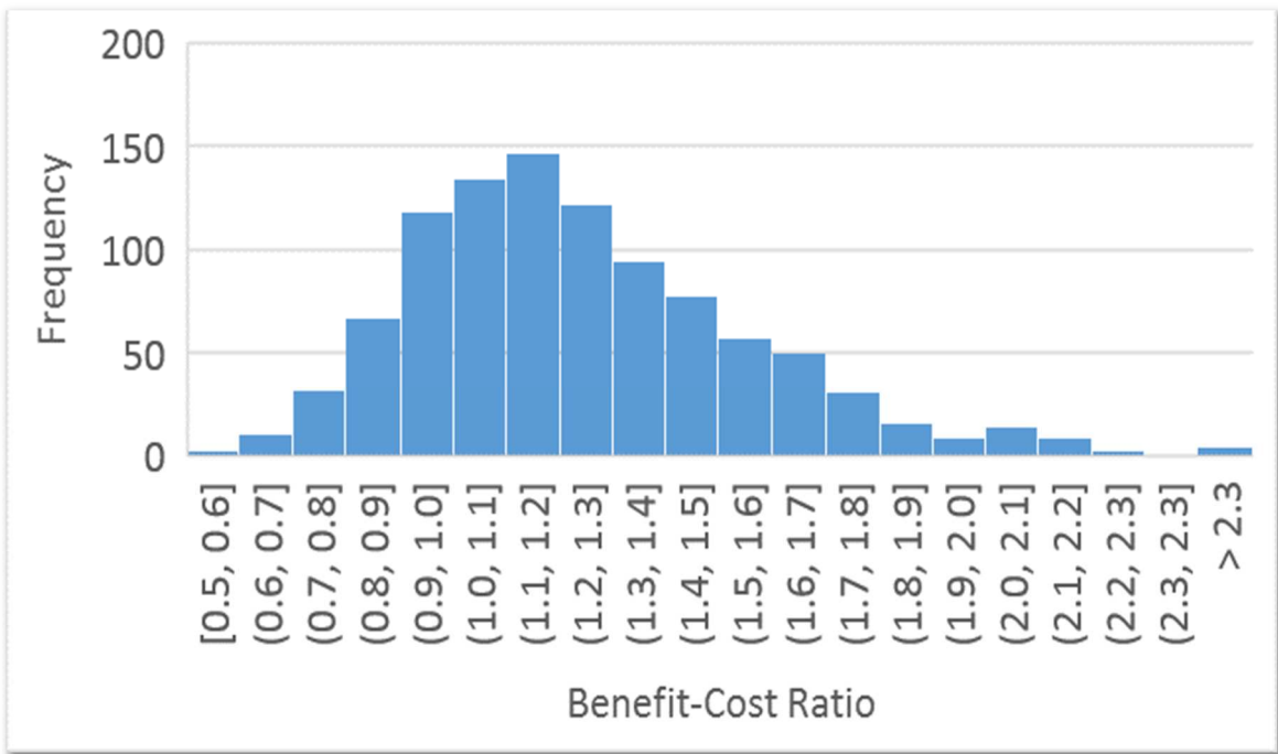
Figure E-3 Distribution of Benefit-Cost Ratios for CV-Based Unsignalized Intersection
