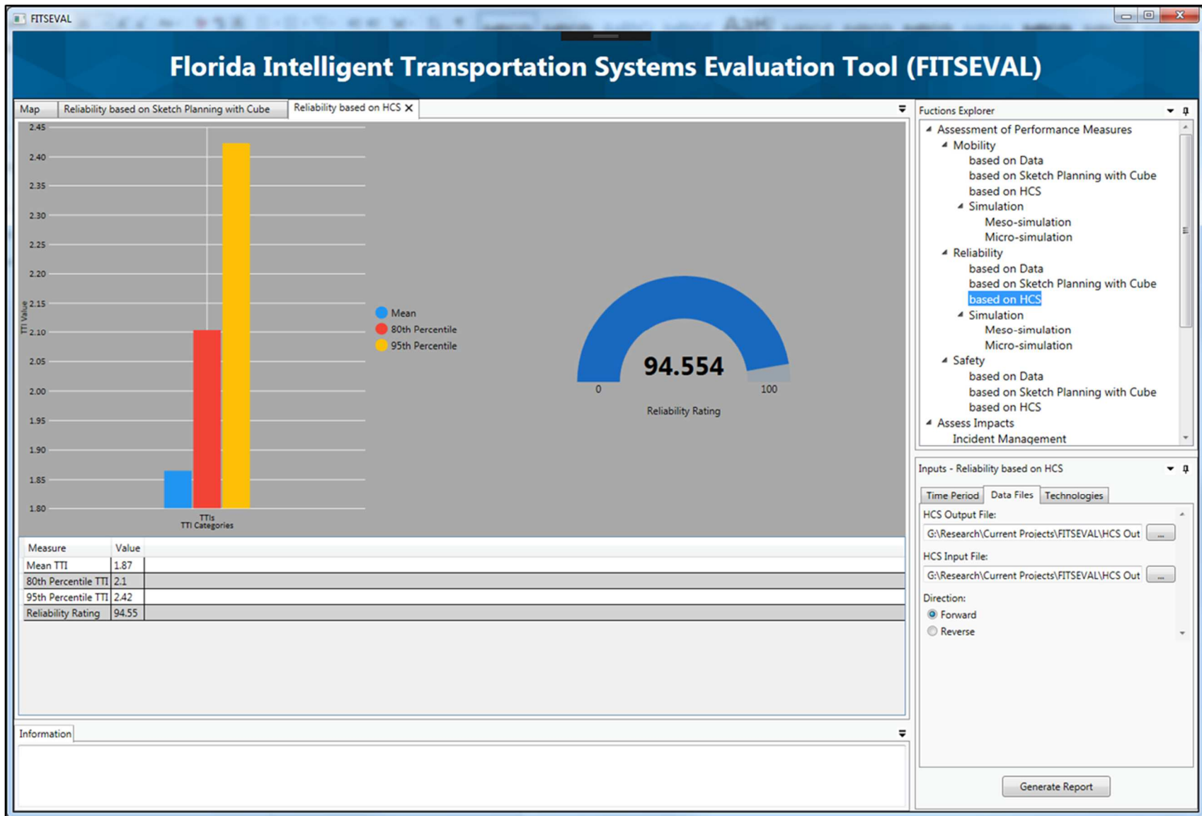
Figure 5-13 Reliability Dashboard Estimated Based on HCS Output
