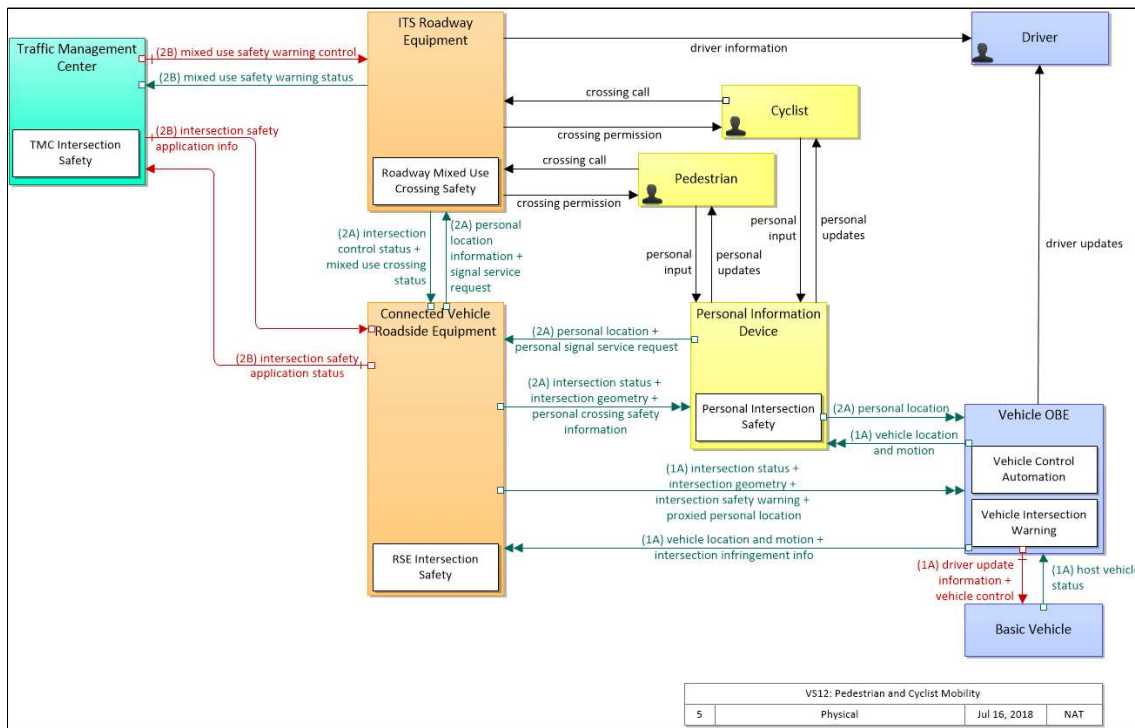
Figure 4-6 VS12 Pedestrian and Cyclist Safety (ARC-IT 8.2, 2019)
