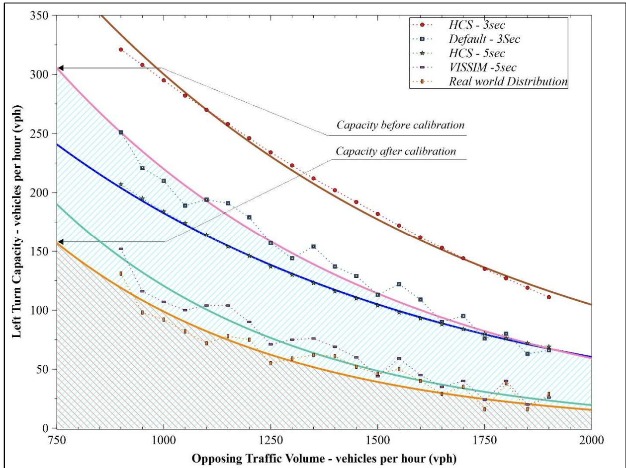
Figure 5-18 Relationship between Left-Turn Capacity and Opposing Traffic
