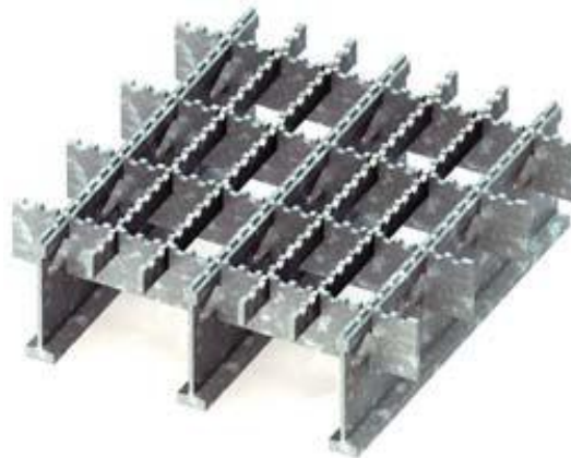
Figure 10 Open Steel Grid Deck (courtesy of BGFMA (11))
