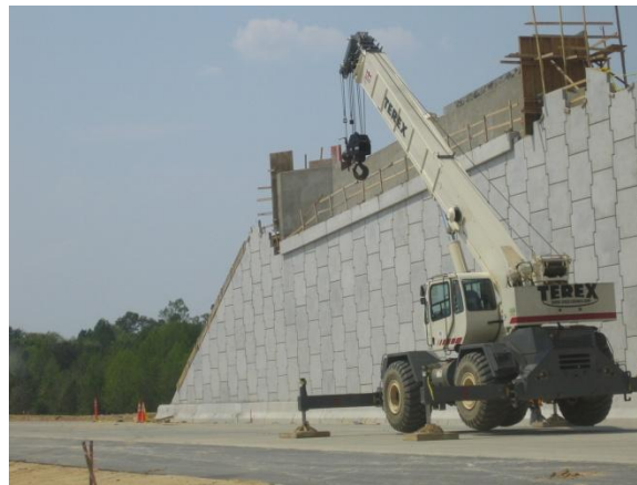
Figure 12 Conventional stub abutment with MSE retaining wall and wingwalls parallel to the abutment cap.
