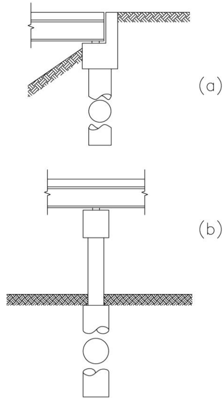
Figure 7 Drilled shaft applications: a) drilled shafts for a conventional stub abutment: b) drilled shafts used for a pier.
