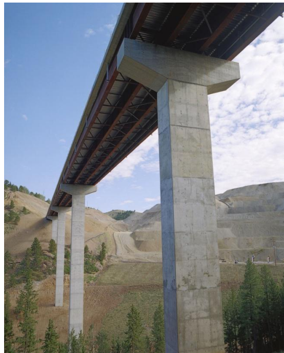
Figure 20 Single column hammerhead pier with very tall columns over a deep valley.
