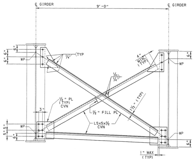
Figure 3 Detail sketch of a typical X-frame cross-frame type
