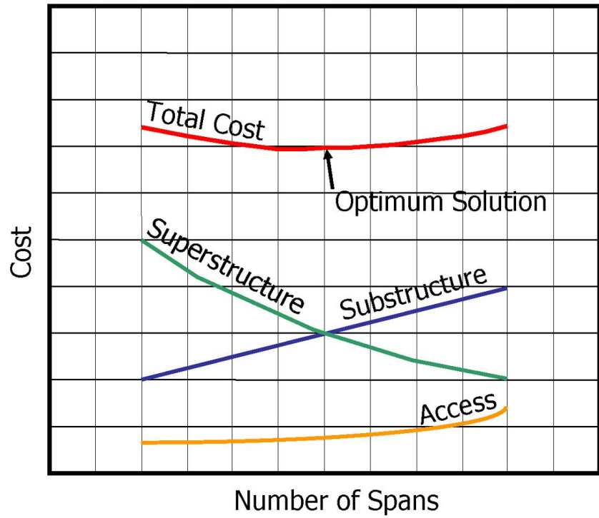
Figure 1 Graph showing typical bridge cost curves
