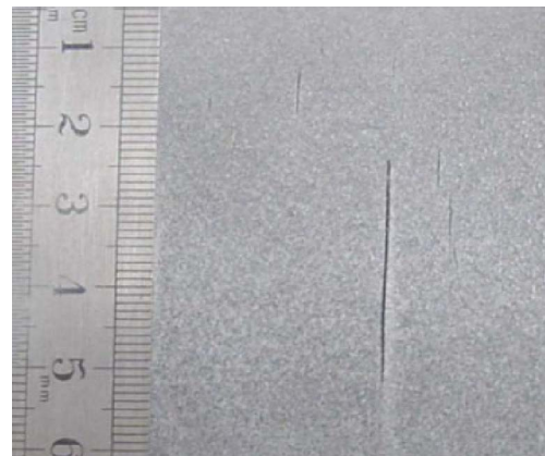
Figure 1. Typical crack group resulting from WIDEM fatigue testing at Lucchini
