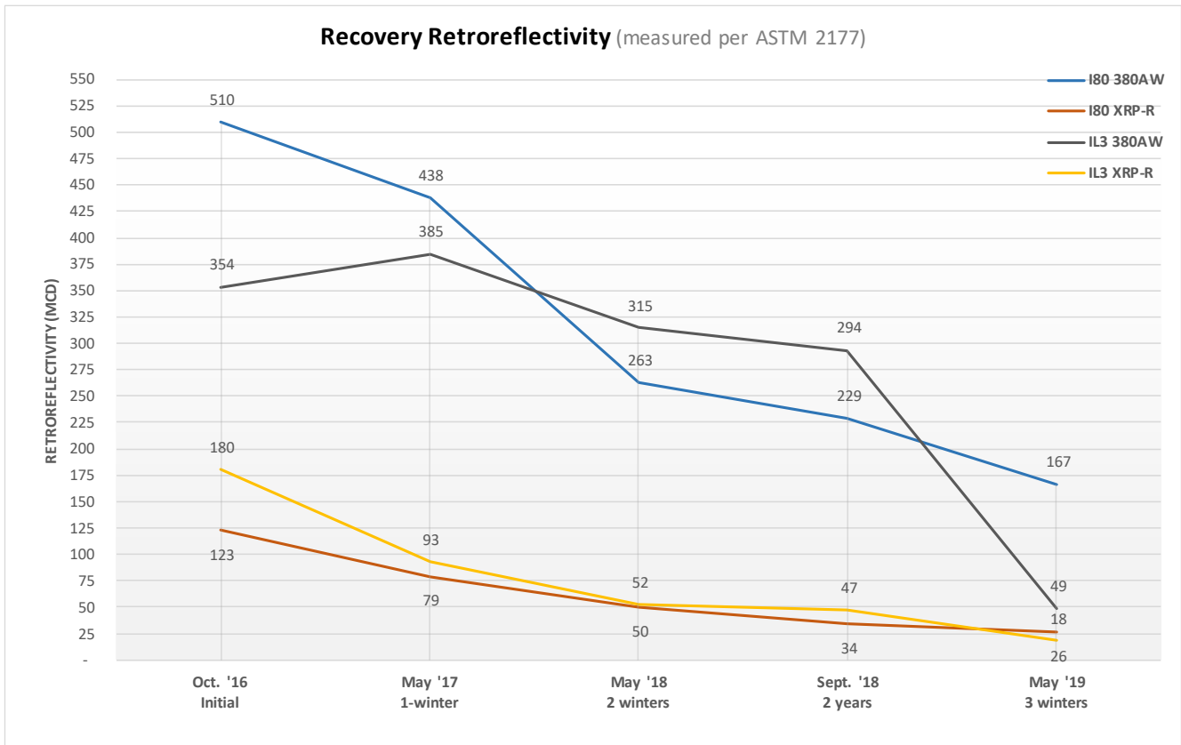
Figure 26. Recovery retroreflectivity over time.
