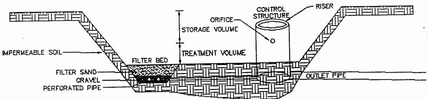
Figure 6-6: DRY DETENTION POND
