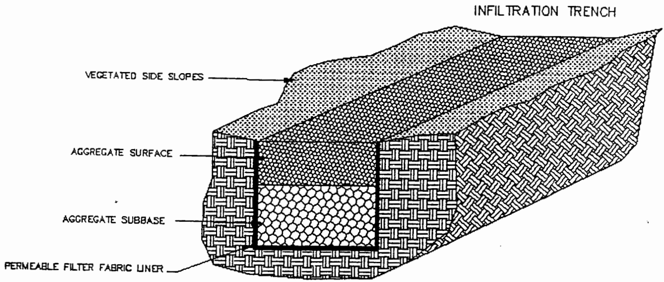
Figure 6-8: INFILTRATION STRIP
