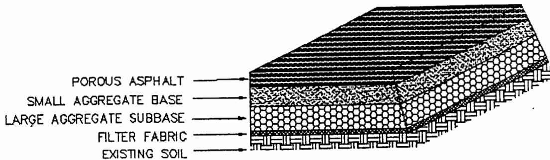
Figure 6-2: POROUS PAVEMENT - A) POROUS MODULAR CONCRETE, B) POROUS ASPHALT
