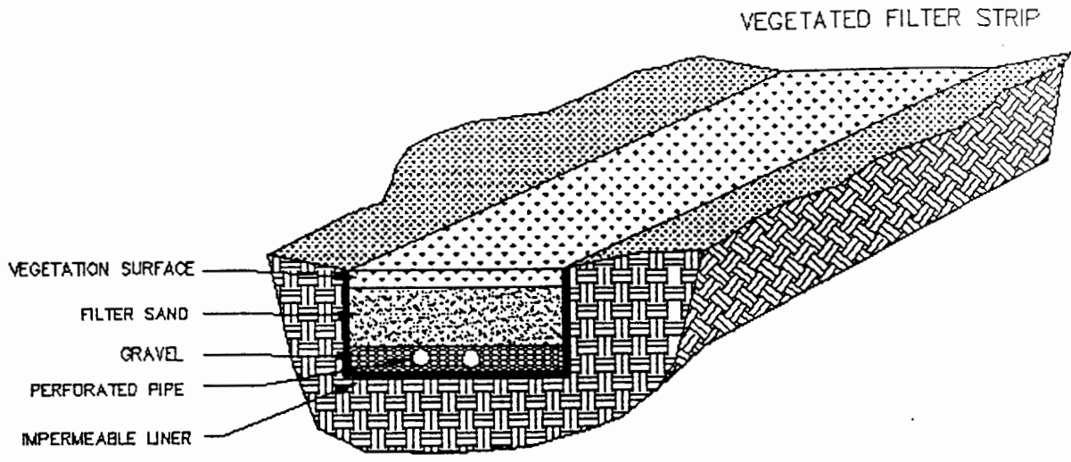
Figure 6-7: VEGETATED FILTER STRIP
