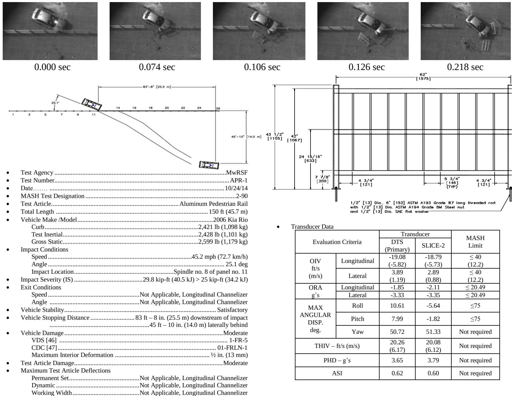
Figure 175. Summary of Test Results and Sequential Photographs, Test No. APR-1
