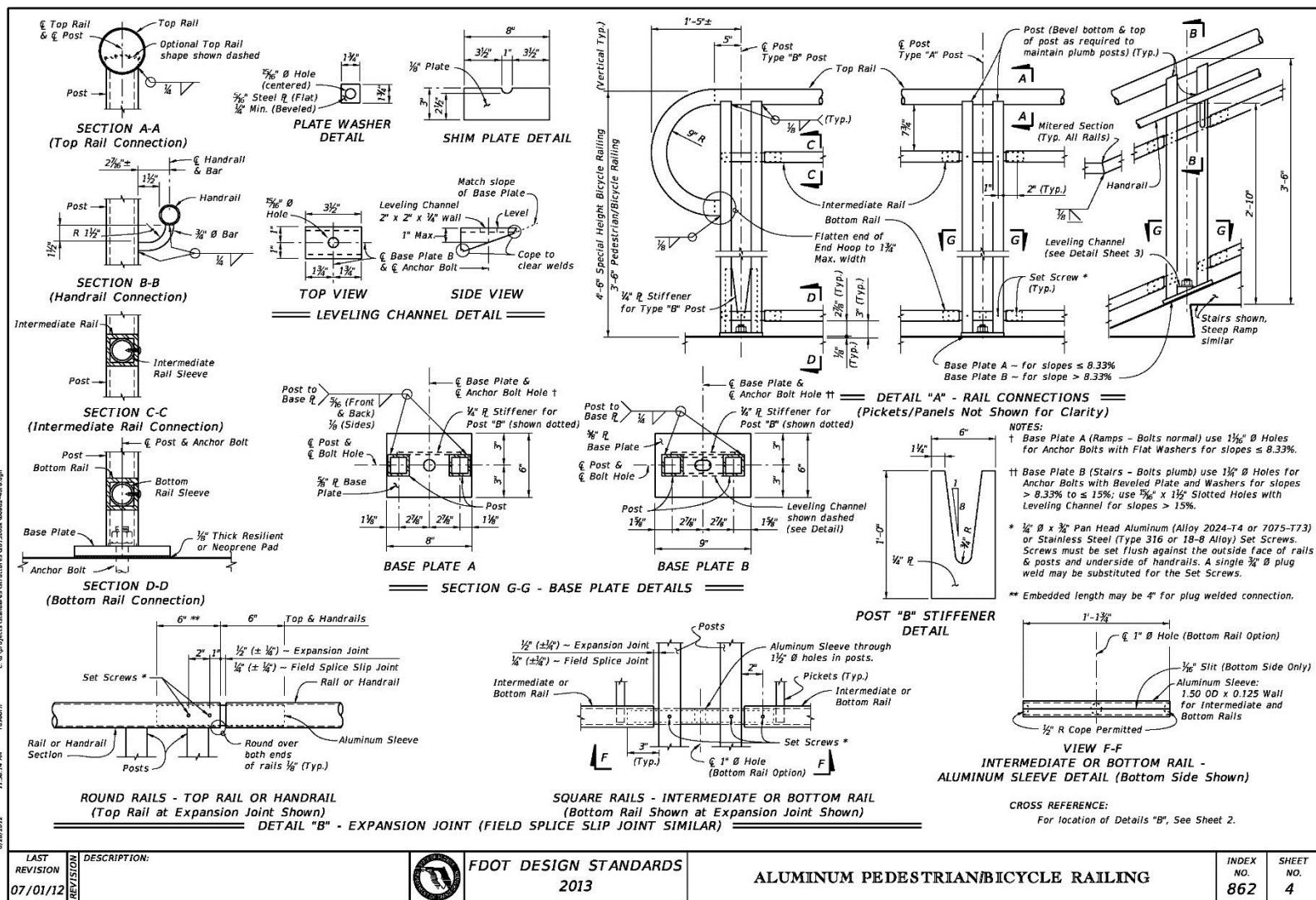
Figure 23. FDOT Aluminum, Pedestrian-Only Rail (Sheet 4 of 8) [32-33]
