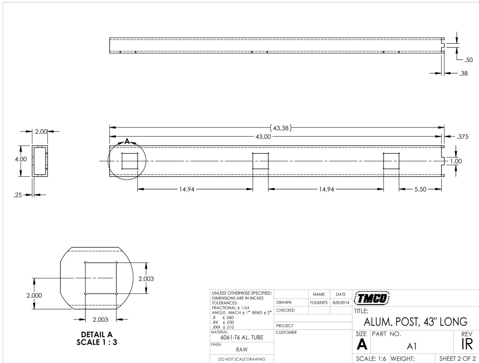
Figure F-3. Fabrication Drawings, Test Nos. APR-1 and APR-2
