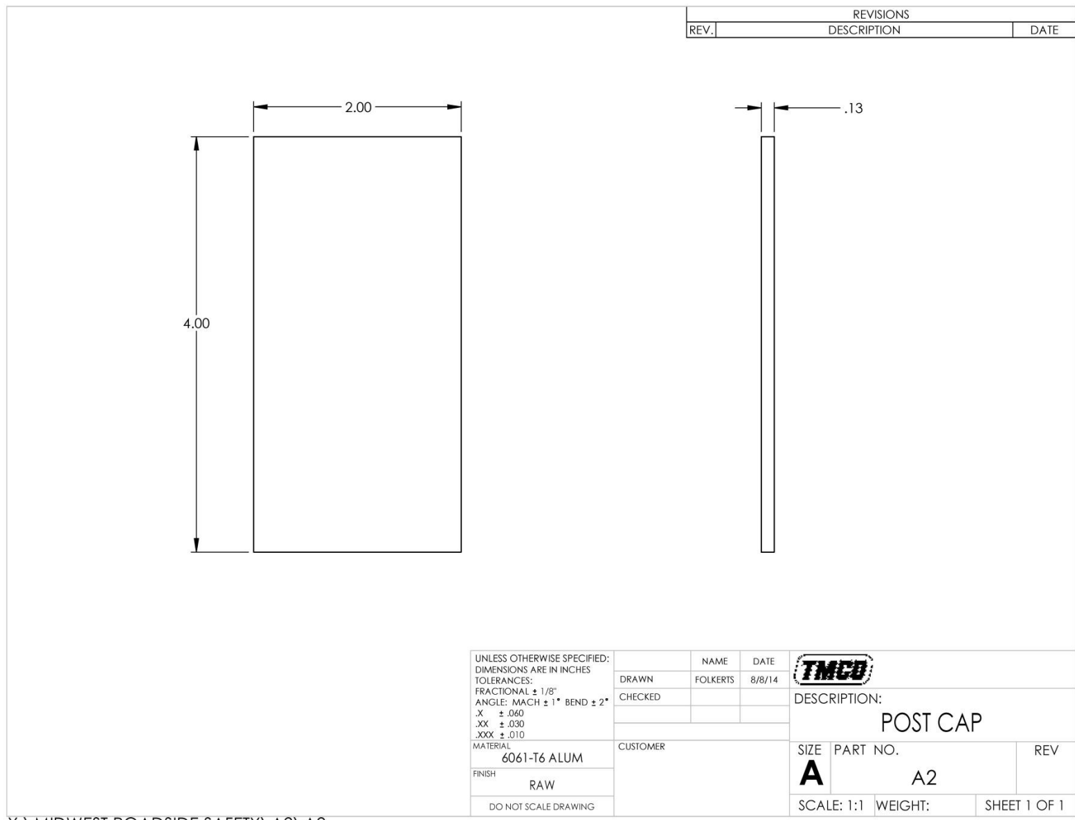
X:\MIDWEST ROADSIDE SAFETY\A2\A2 Figure F-4. Fabrication Drawings, Test Nos. APR-1 and APR-2
