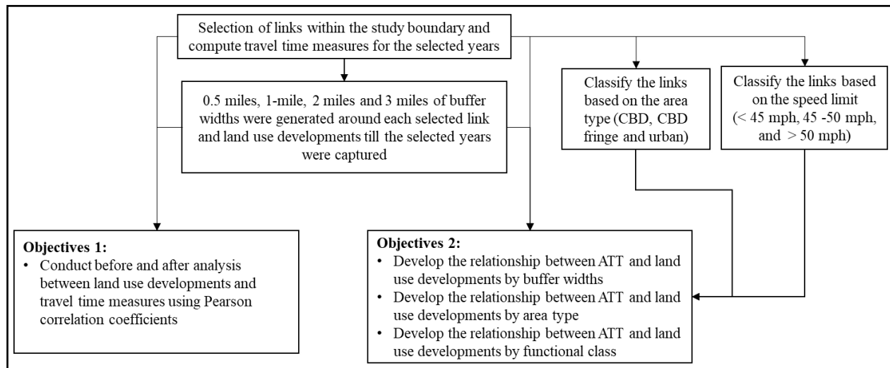
Figure 4. Methodology – Flowchart
