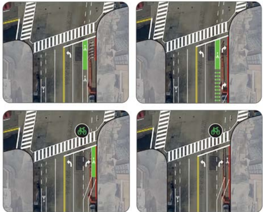
Figure 8: Images show several intersections with different treatments to separate right turning vehicles from bicycle traffic. Treatments include through bicycle and vehicle travel lanes, through intersection guidelines, phase separation, and concrete median separation. (Image courtesy of Madison Area Transportation Planning Board and the Volpe Center)
