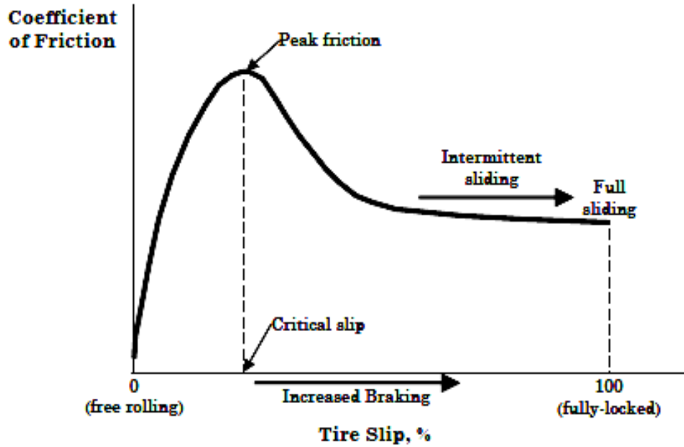
Figure 2-1. Coefficient of Friction V. Tire Slip (Henry 2000).
