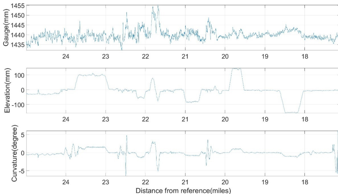
Figure 40 – Track Geometry for Test Section
