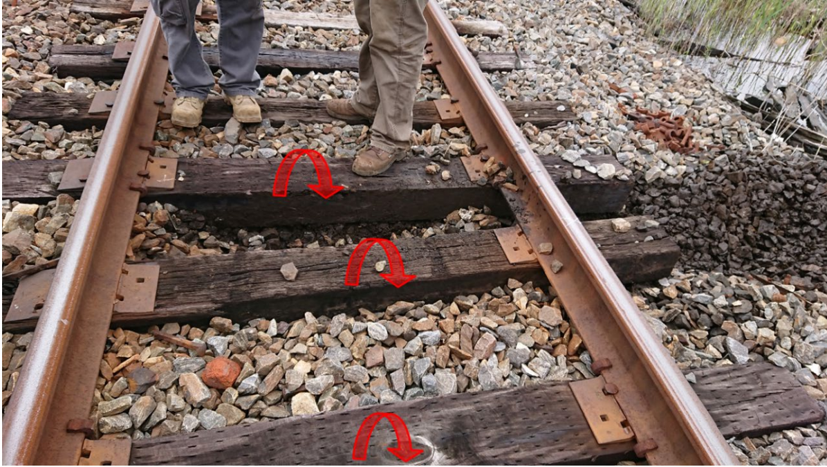
Figure 37 – Tie Skew Change Detection
