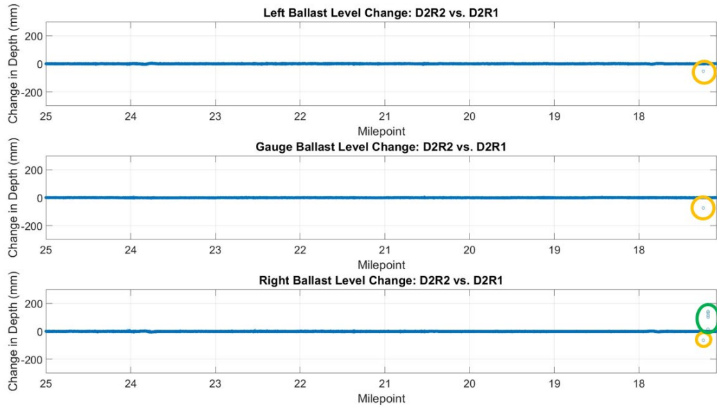
Figure 27 – Modeling Ballast Height at Gauge and End-of-Tie Noise Floor (D2R2 vs. D2R1)
