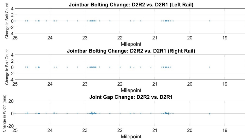
Figure 51 – Modeling Joint Bar Bolting Noise Floor (D2R2 vs. D2R1)
