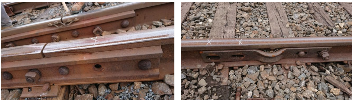
Figure 52 – Deliberate Changes to Joint Bar Bolting
