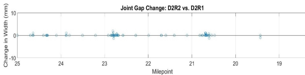
Figure 63 – Modeling Joint Gap Noise Floor (D2R2 vs. D2R1)
