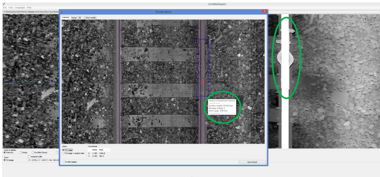
Figure 54 – Right Rail at MP 22+3076 with Two Bolts (D1R1)
