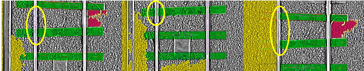
Figure 61 – Ends of Joint Bar Bolts Buried by Ballast (from left to right: May, June, and September)
