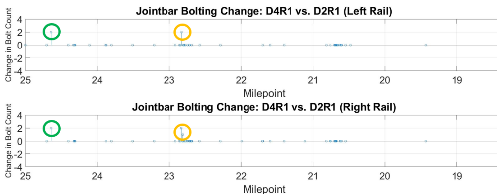
Figure 56 – Joint Bar Bolting Changes between May and June (D4R1 vs. D2R1)
