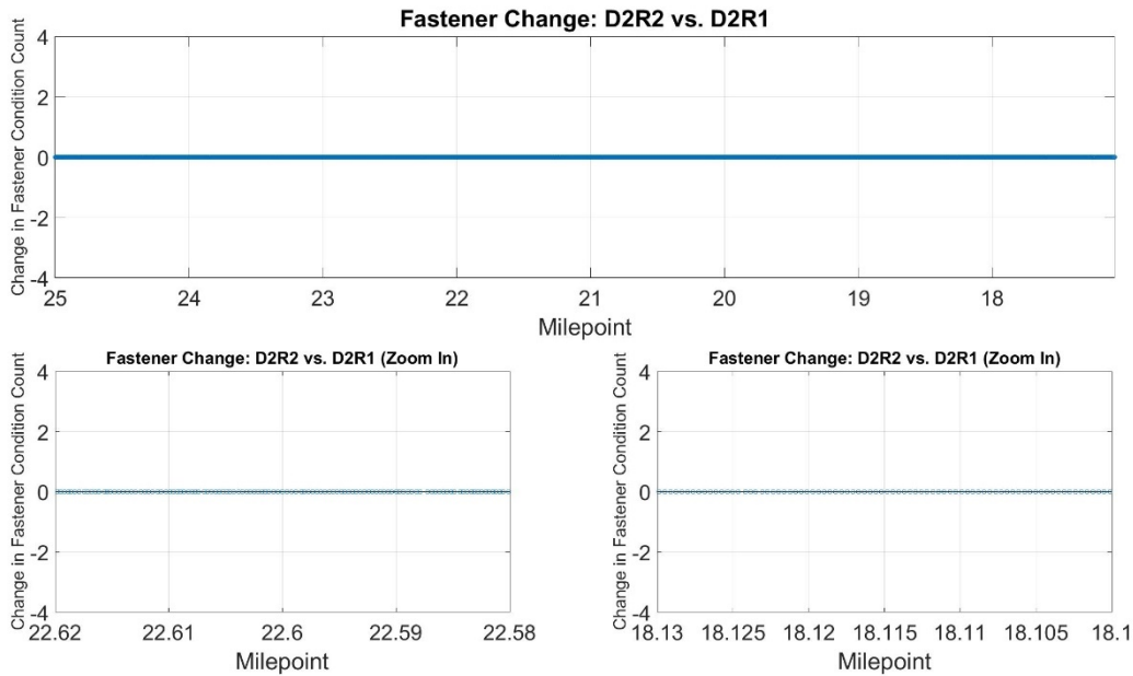
Figure 66 – Modeling Fastener Status Noise Floor (D2R2 vs. D2R1)
