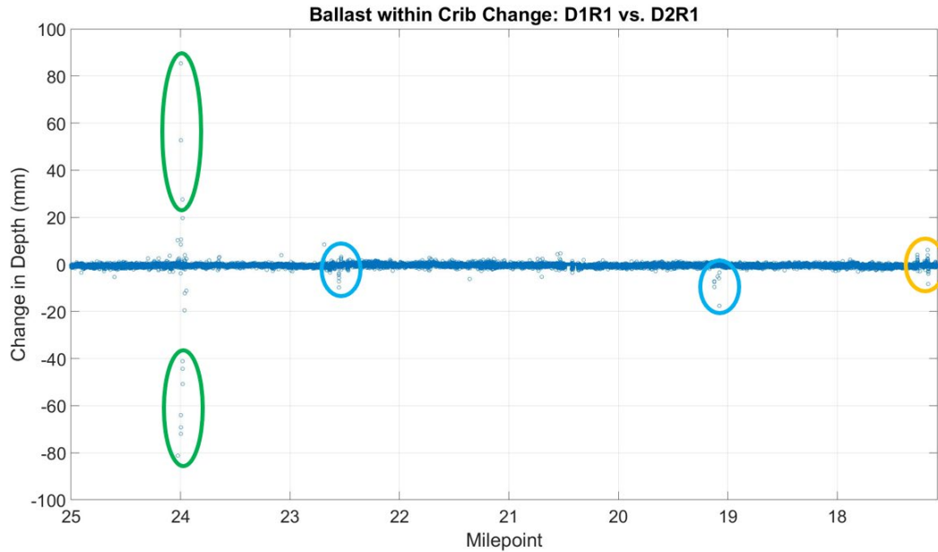
Figure 22 – Detecting Deliberate Ballast-in-Crib Change (D1R1 and D2R1)
