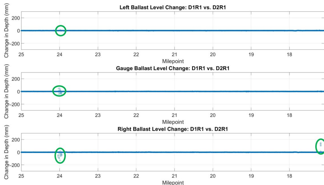
Figure 31 – Detecting Deliberate Ballast in Gauge and End-of-Tie Change (D1R1 and D2R1)
