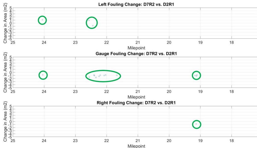
Figure 36 – Organic Changes in Ballast Fouling over the Test Period (D7R2 vs. D2R1)
