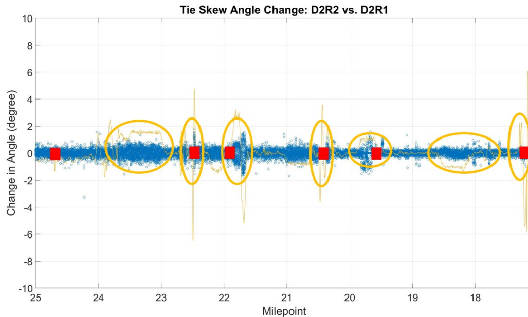
Figure 41 – Track Alignment (yellow line) Overlaid on Plot of Tie Skew Angle Change
