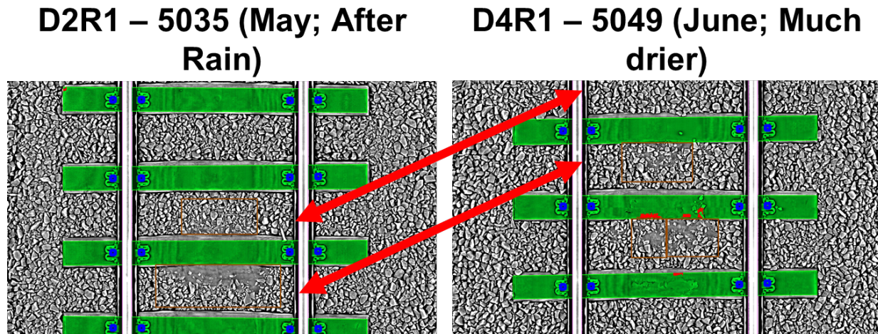
Figure 35 – Reduction in Surface Fouling between May and June
