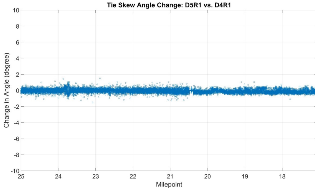
Figure 39 – Same Direction Runs Produce More Consistent Skew Angle Measurements
