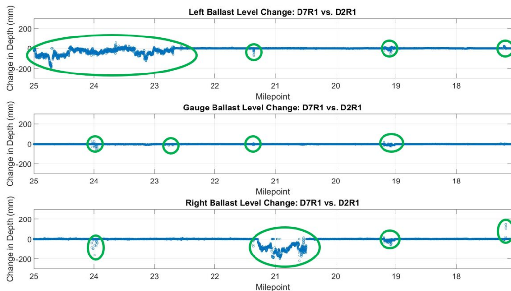
Figure 32 – Height of Changes in Ballast per Meter of Travel between May and September
