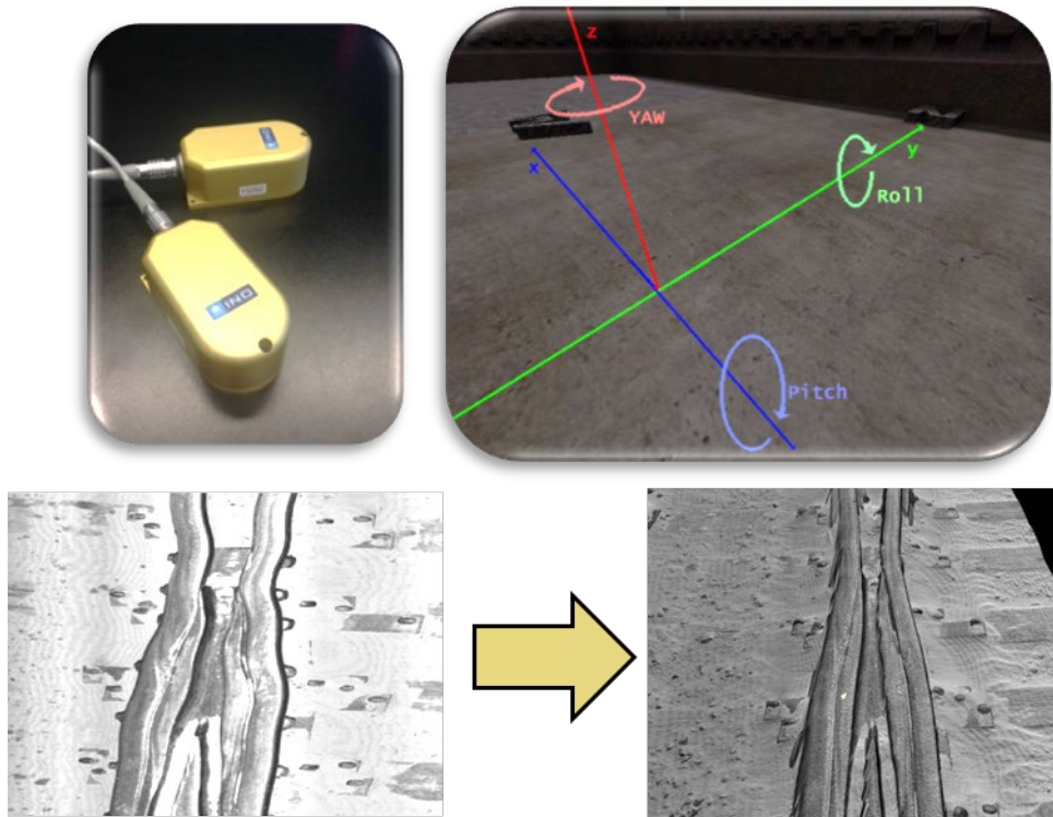
Figure 8 – Correction for Vehicle Motion
