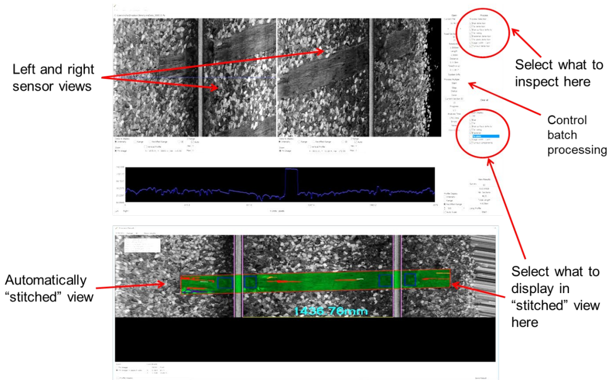
Figure 13 – LRAIL Inspection Software Interface
