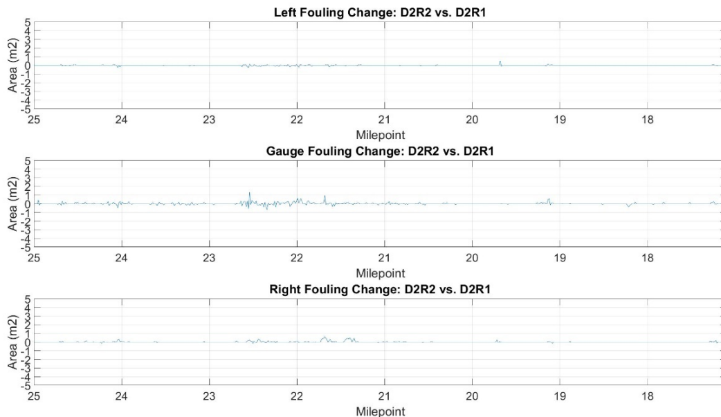
Figure 34 – Difference in Area of Fouling between Runs (D2R2 vs. D2R1)
