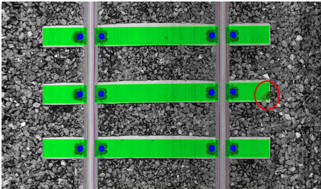
Figure 48 – Intensity Image Showing Automatically Detected Chipping on Concrete Tie
