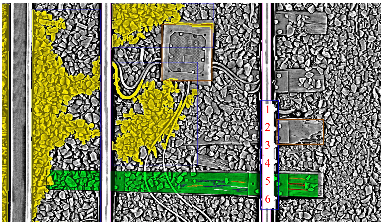
Figure 58 – Right Rail Joint Bar in May Showing Six Bolts with 100 percent of Heads on the Gauge Side of the Rail
