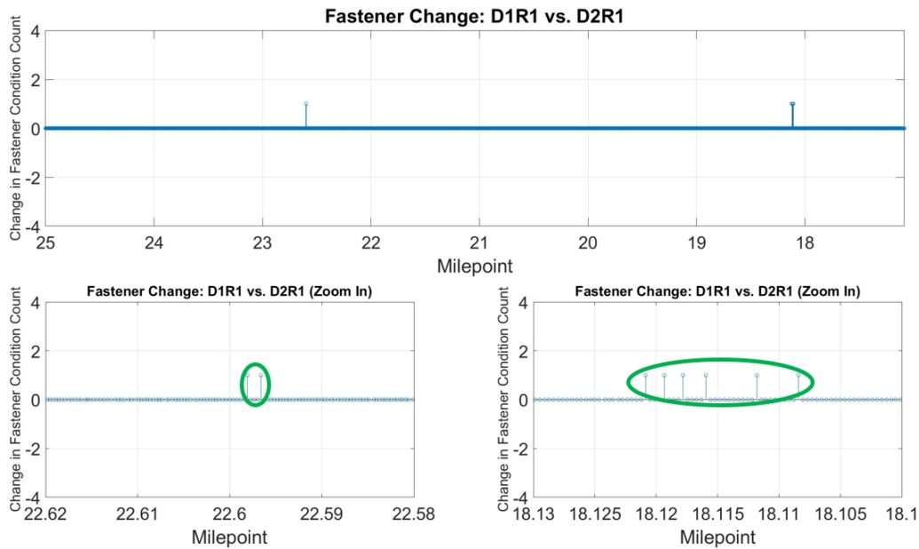
Figure 70 – Detecting Deliberate Fastener Change (D1R1 and D2R1)
