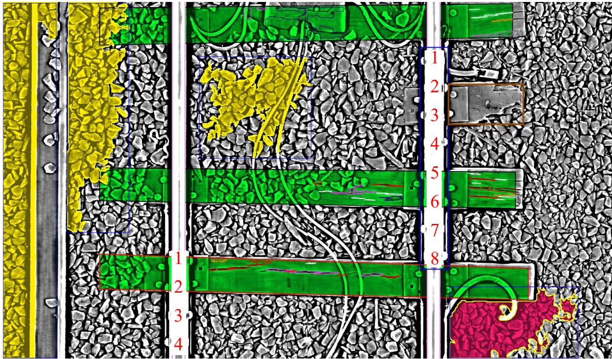
Figure 59 – Part 1 of Left and Right Rail Joints in June Showing Eight Bolts (four on either side of the joint) with Staggered Heads
