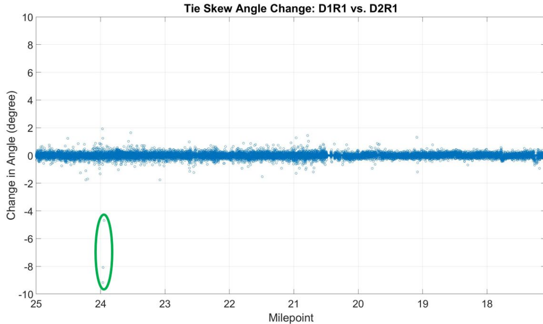
Figure 43 – Detecting Deliberate Tie Skew Change (D1R1 and D2R1)
