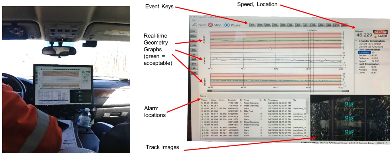
Figure 4 – Real-time User Interface
