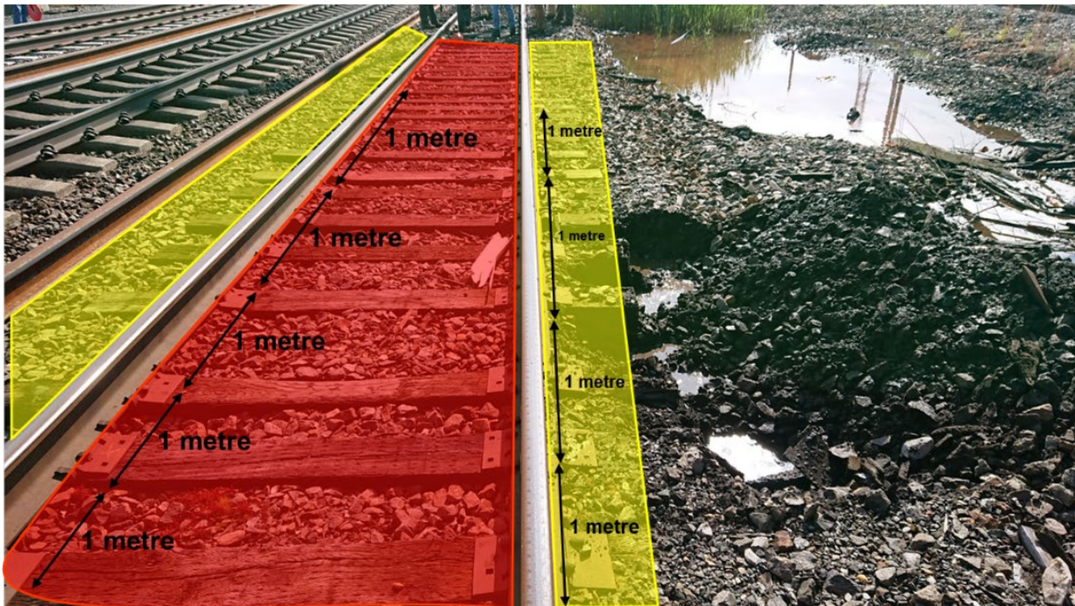
Figure 26 – Running Meter Ballast Height Measurements
