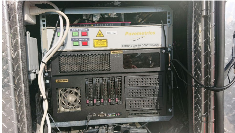
Figure 2 – Onboard Computing and Power Supply
