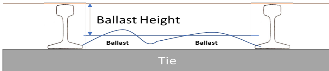
Figure 18 – Ballast Height Measurement
