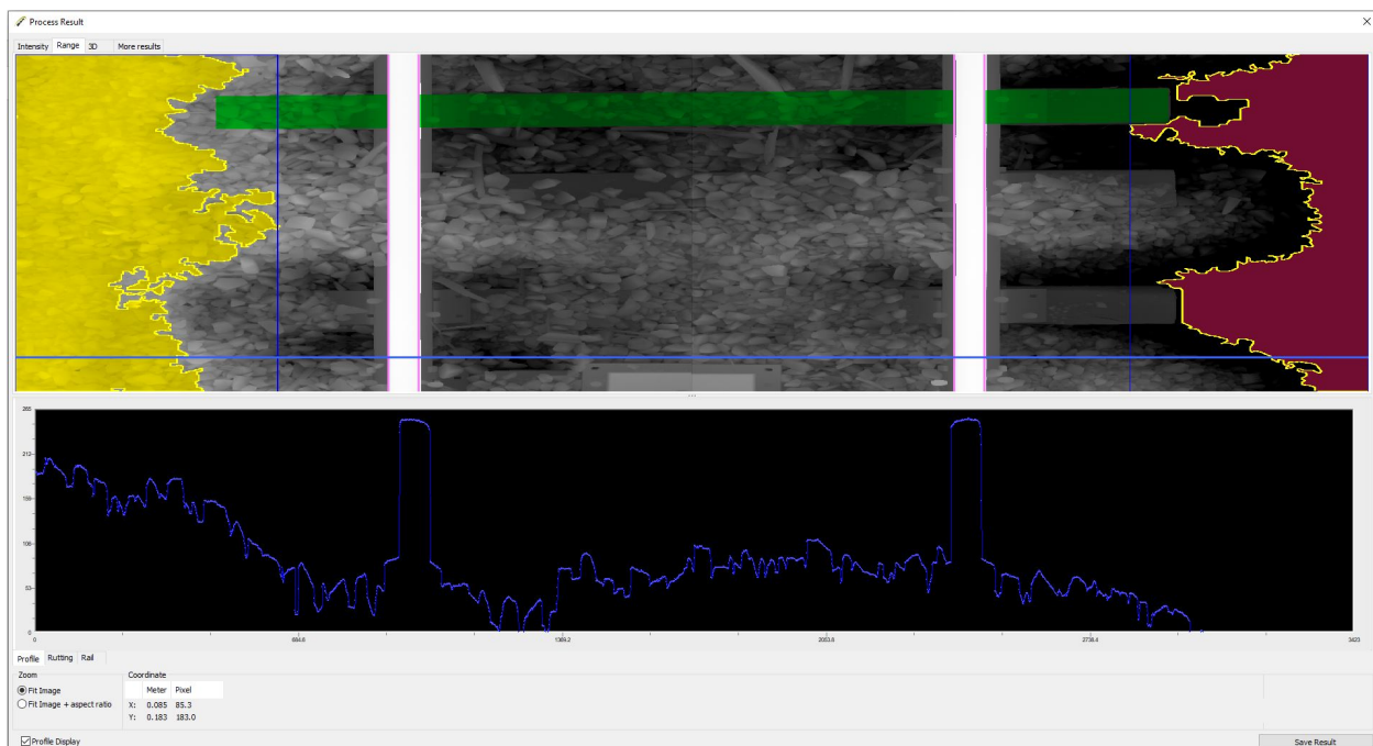
Figure 62 – 3-Dimensional Range Data Showing Height Profile of Ballast
