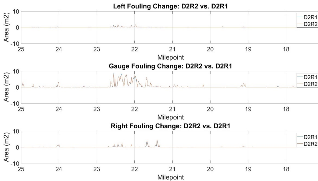
Figure 33 – Modeling Ballast Fouling Noise Floor (D2R2 vs. D2R1)
