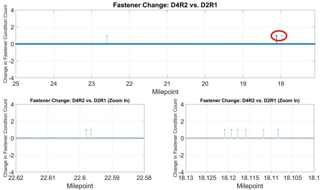
Figure 68 – Modeling Fastener Status Noise Floor (D4R2 vs. D2R1)
