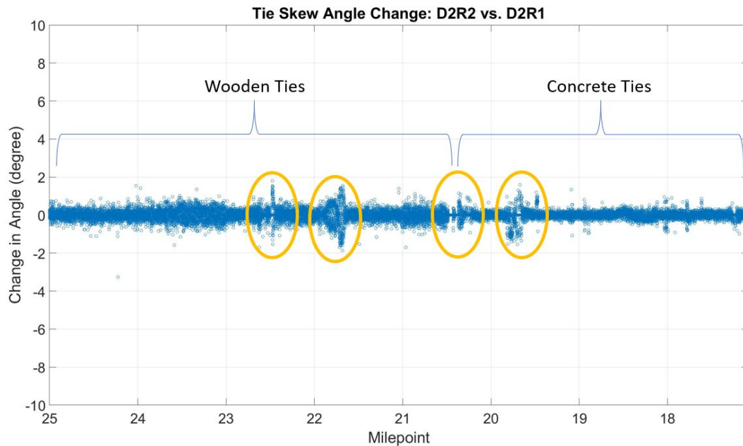
Figure 38 – Modeling Tie Skew Noise Floor (D2R2 vs. D2R1)
