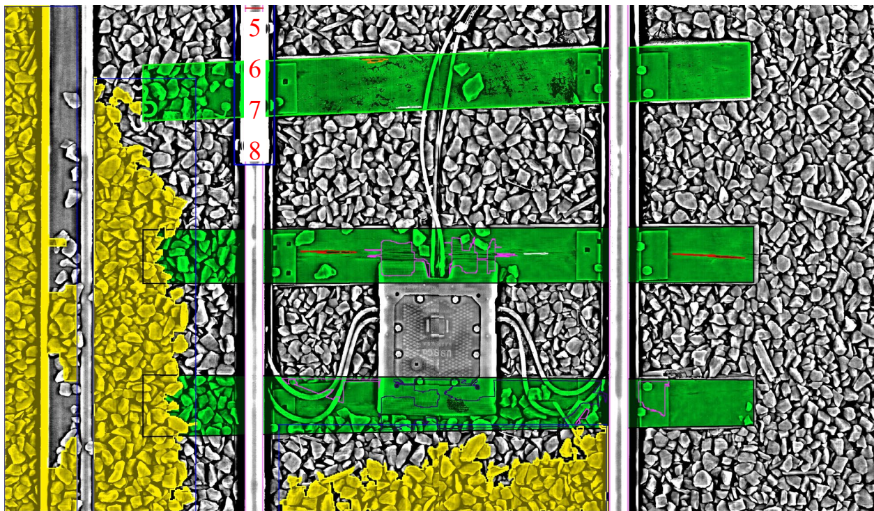
Figure 60 – Part 2 of Left and Right Rail Joints in June Showing Eight Bolts (four on either side of the joint) with Heads Alternating between Gauge and Field Sides
