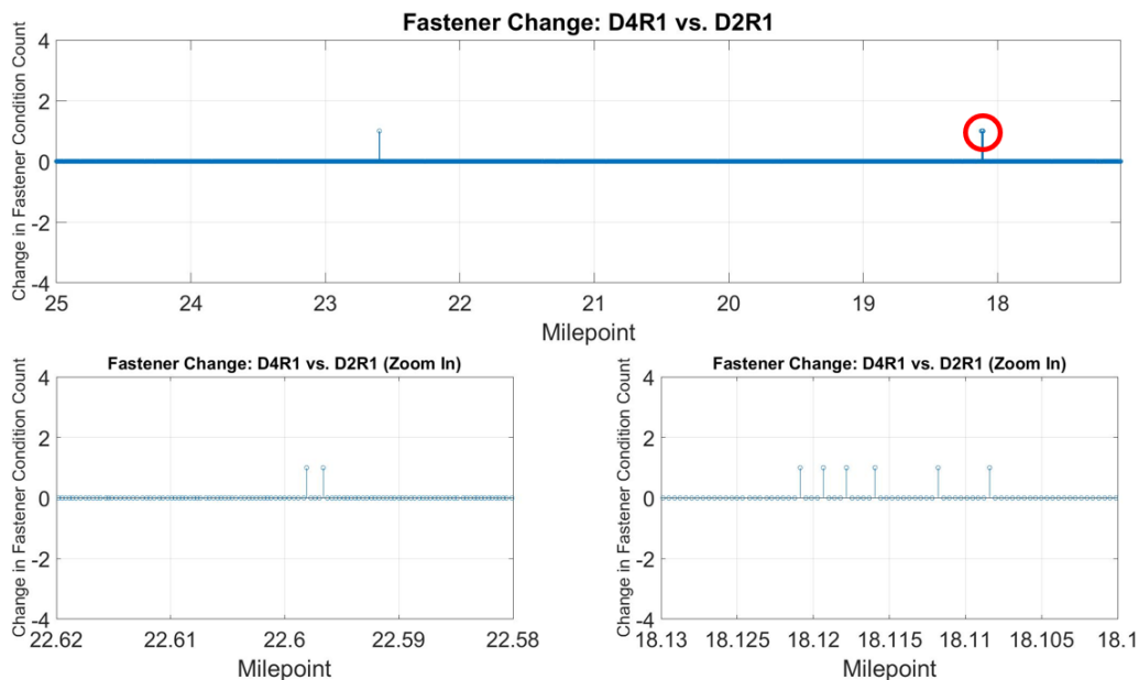
Figure 67 – Modeling Fastener Status Noise Floor (D4R1 vs. D2R1)
