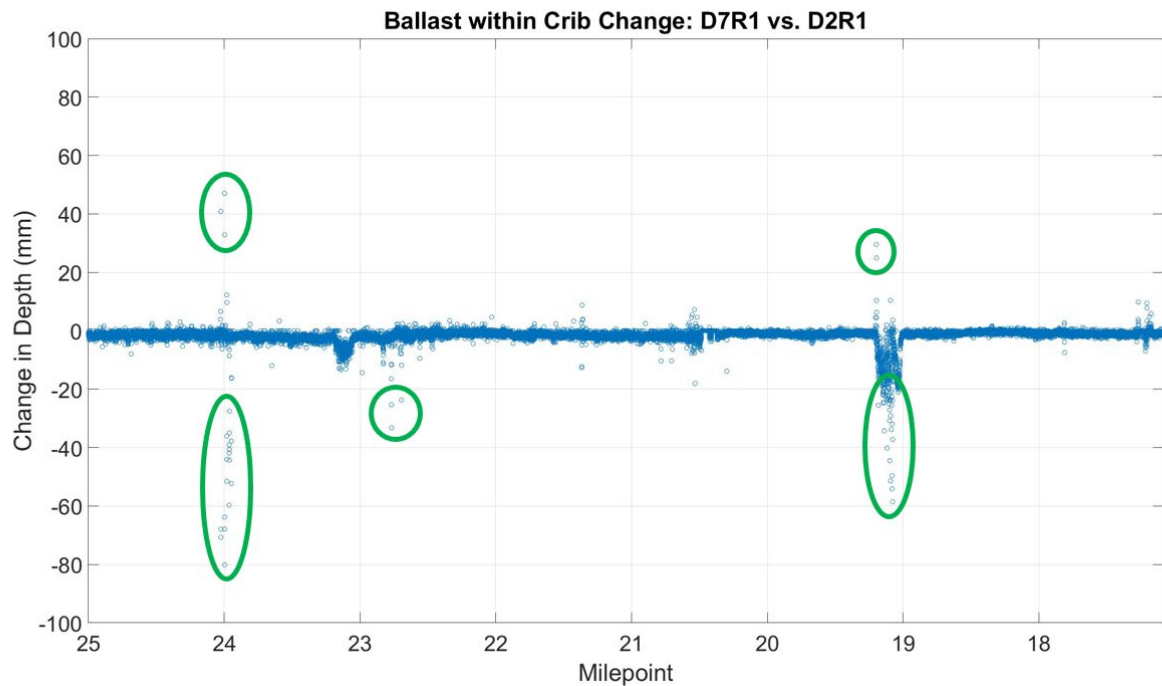
Figure 25 – Ballast-in-Crib Changes between May and September
