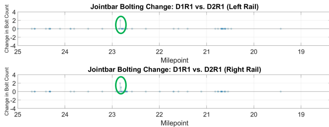
Figure 53 – Detecting Deliberate Joint Bar Bolting Change (D1R1 and D2R1)
