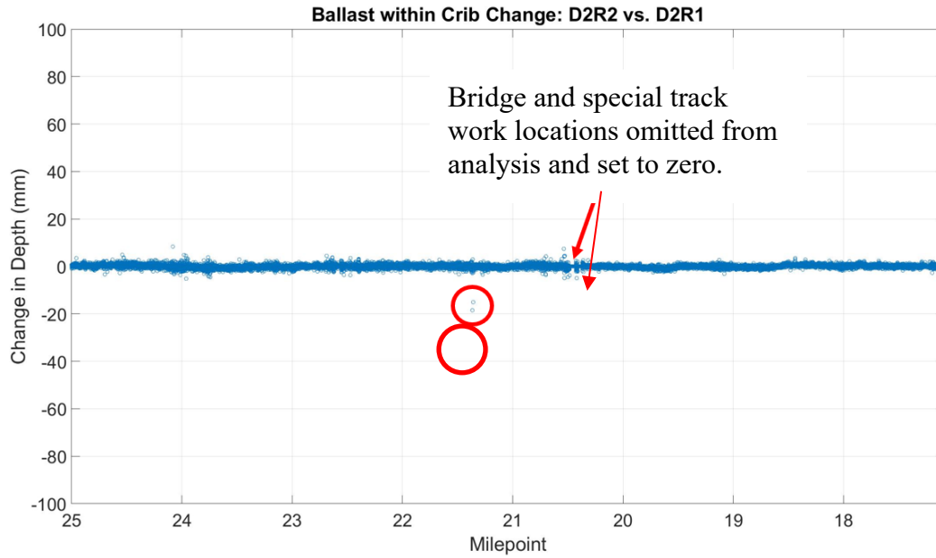
Figure 19 – Modeling Ballast-in-Crib Height Noise Floor (D2R2 vs. D2R1)
