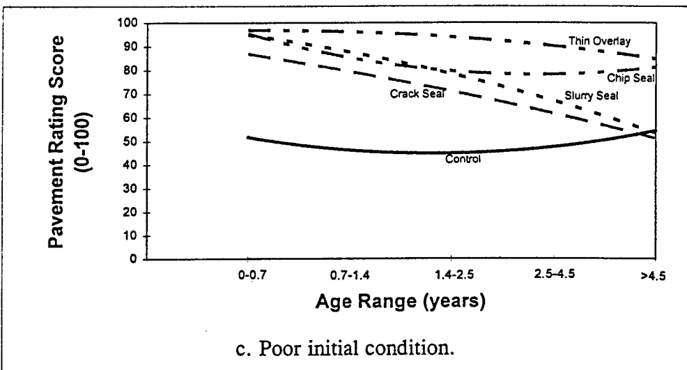
Figure 14. Pavement rating score (PRS) vs. age range by treatment type and initial condition for the wet-no freeze environmental zone, post-construction data only.
