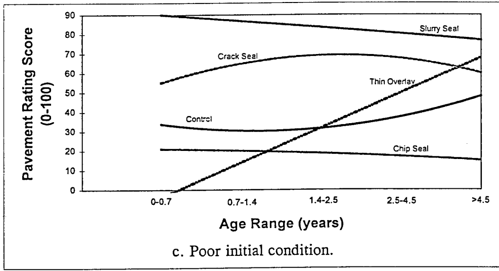
Figure 12. Pavement rating score (PRS) vs. age range by treatment type and initial condition for the dry-no freeze environmental zone, post-construction data only.
