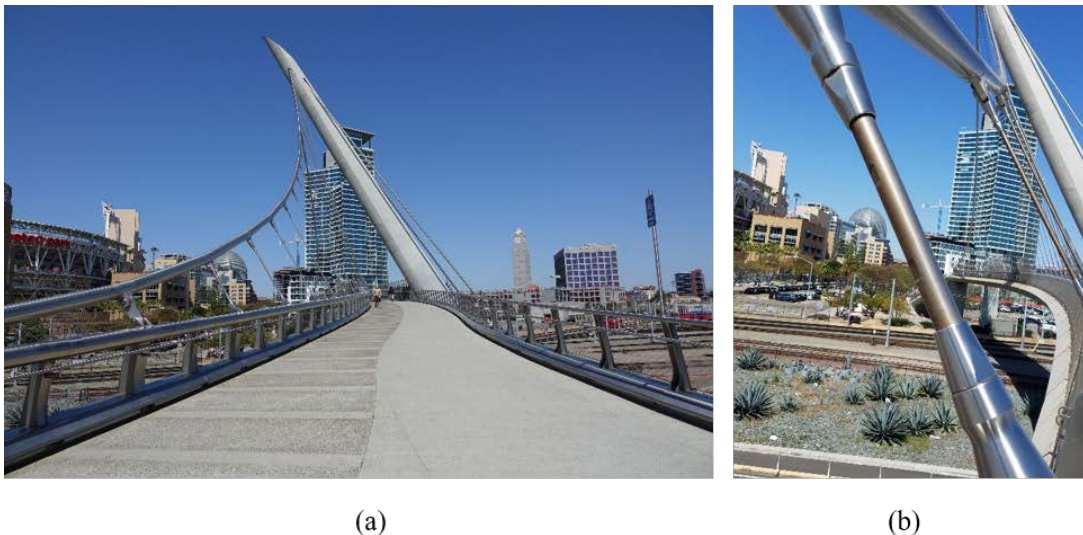
Figure 27. Harbor Drive Pedestrian Bridge: (a) overall view; (b) close-up of Grade 2205 duplex stainless steel suspender. Photograph courtesy of Catherine Houska.
