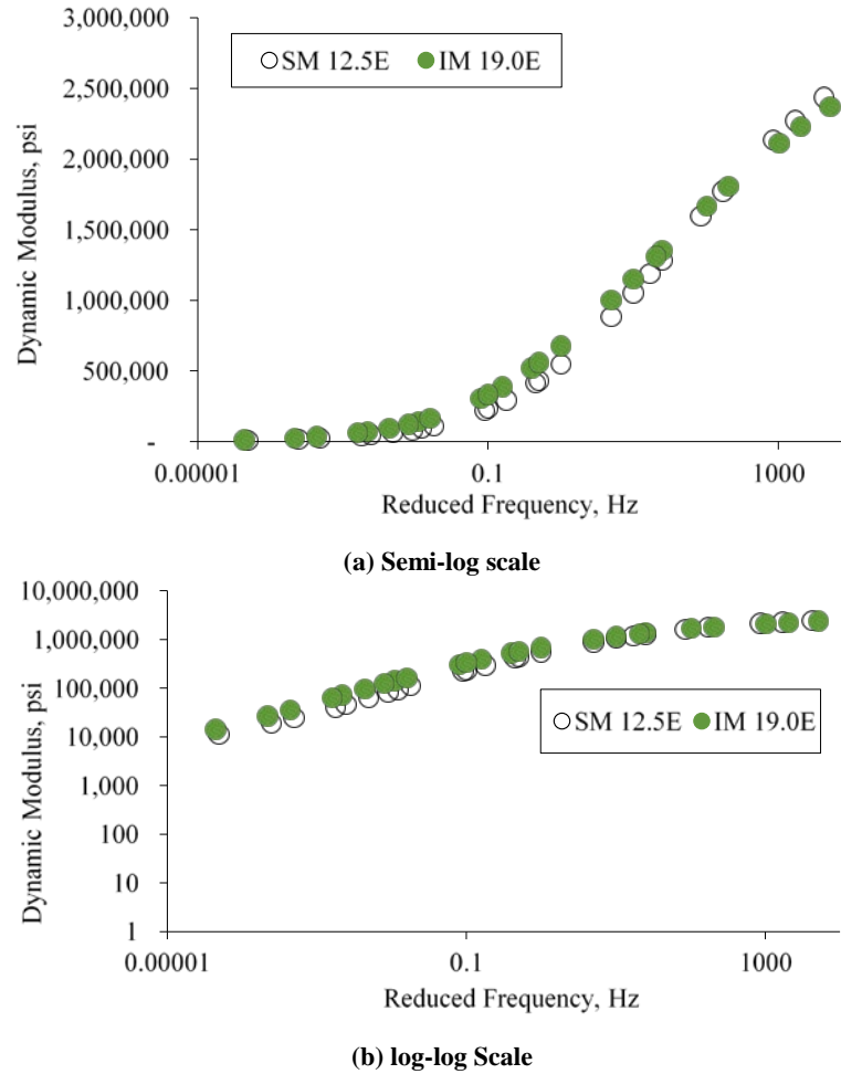
Figure 17. Dynamic Modulus Test Results for SM 12.5E and IM 19.0E Mixtures
