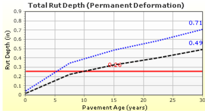
Figure A1. Total Rut Depth
