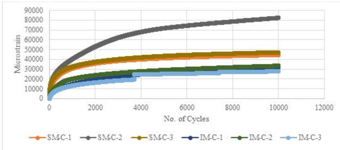
Figure 18. RLPD Results (No. of Cycles vs. Microstrain). RLPD = Repeated load permanent deformation.
