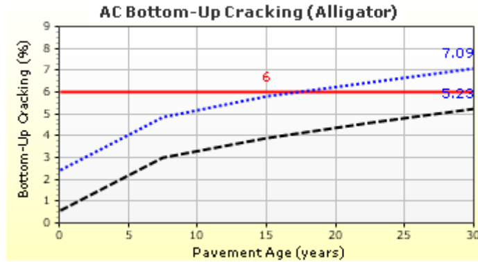
Figure A2. AC Bottom-Up Cracking. AC =asphalt concrete.
