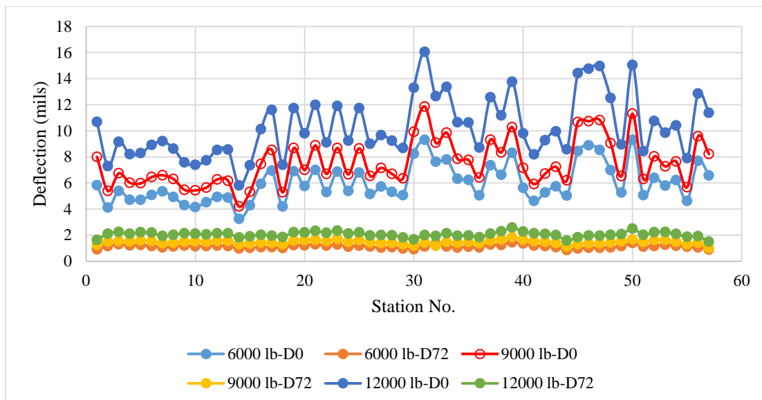
Figure 19. Deflection Results From FWD Testing at Eastbound Lane 1. FWD =falling weight deflectometer; D0 = deflection at loading plate; D72 = deflection at 72 in from loading plate.
