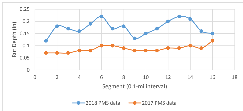
Figure A6. Rut Data for SR 406 (Westbound). PMS = Pavement Management System.
