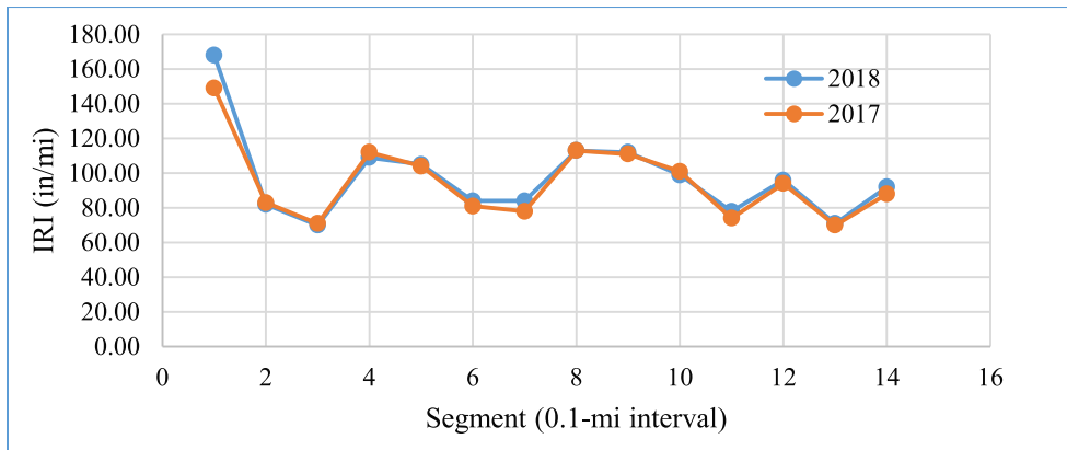
Figure A3. IRI Data for SR 406 (Eastbound). IRI = International Roughness Index.
