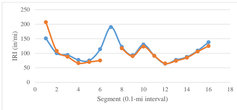
Figure A4. IRI Data for SR 406 (Westbound). IRI = International Roughness Index.
