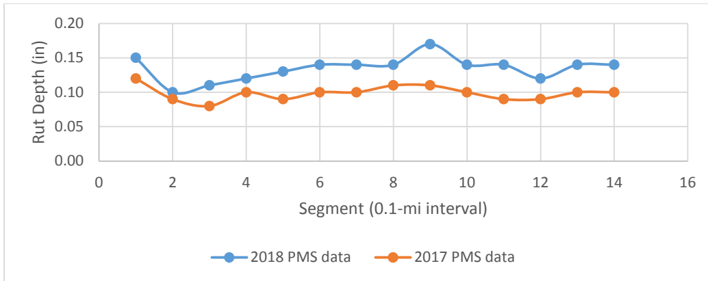
Figure A5. Rut Data for SR 406 (Eastbound). PMS = Pavement Management System.
