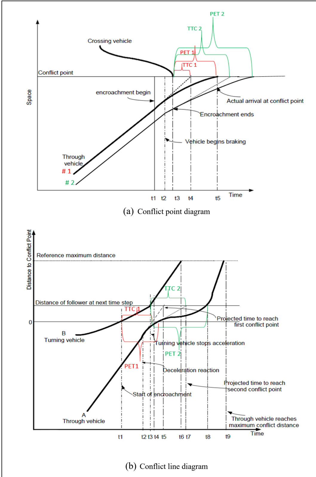
Figure 19- Conflict diagrams in SSAM (a) conflict point, (b) conflict line
