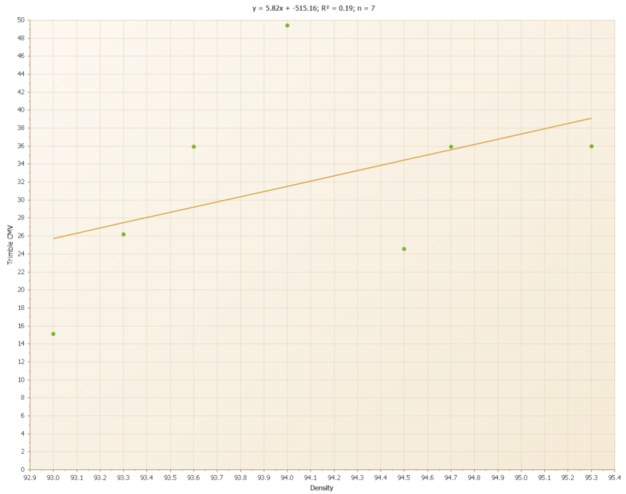
Figure 21 Linear Regression
