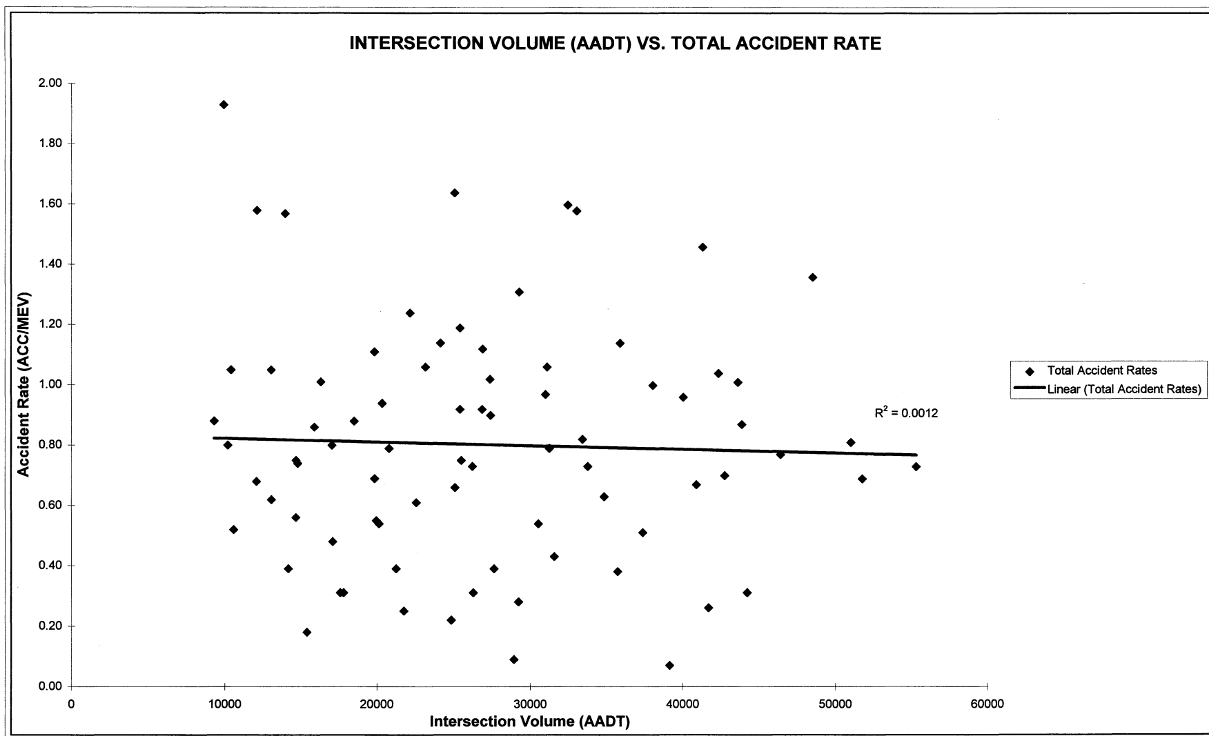
Figure 13. Intersection Volume (AADT) vs. Total Accident Rate
