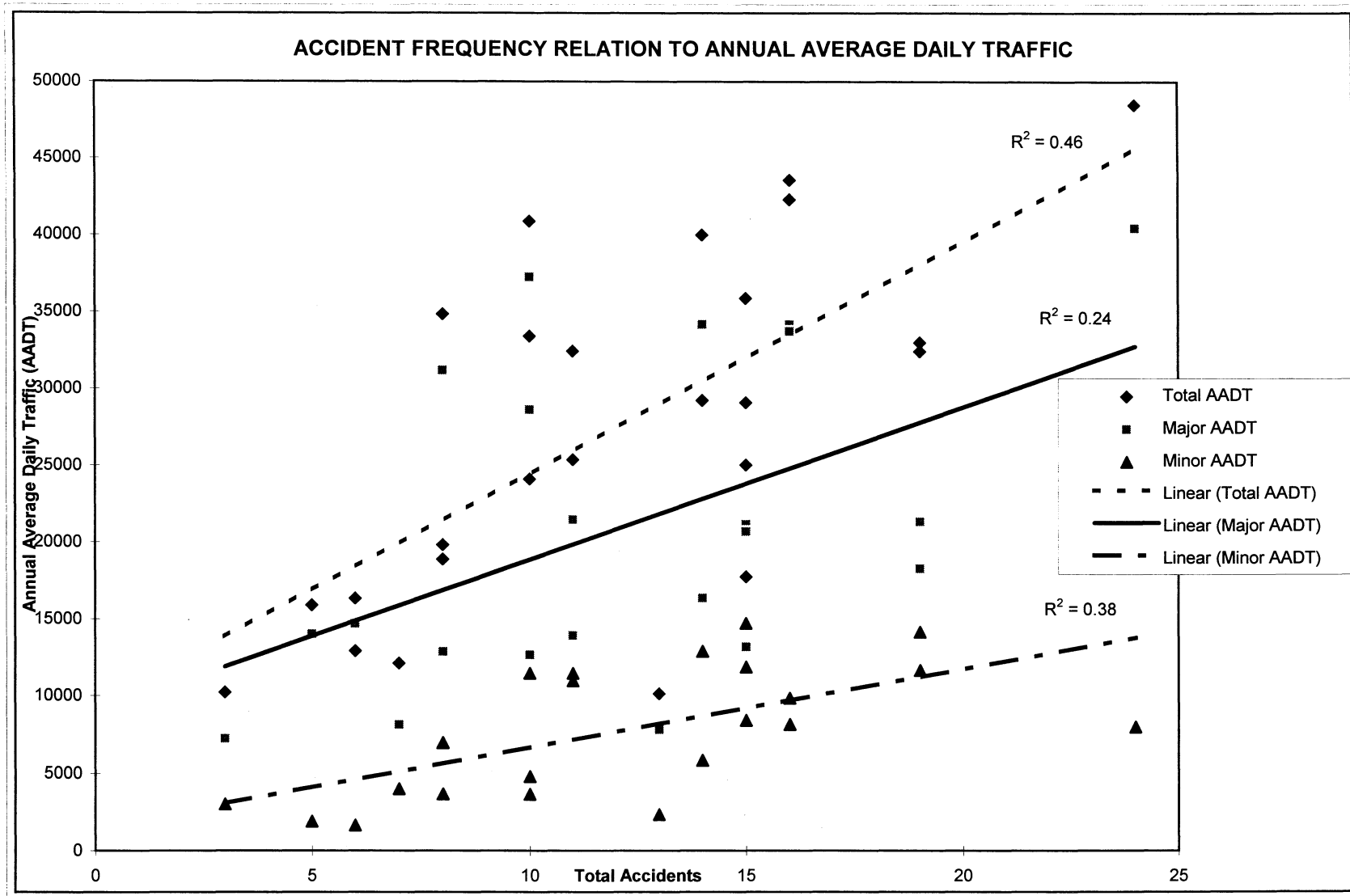
Figure 12. Accident Frequency Relation to Annual Average Daily Traffic
