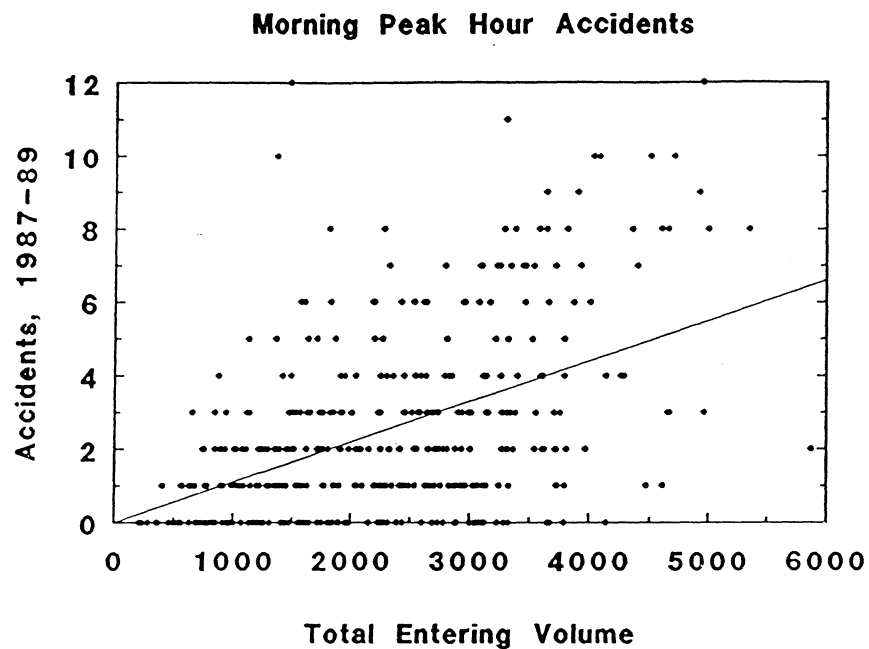
Figure 1. Morning Peak Hour Accidents
