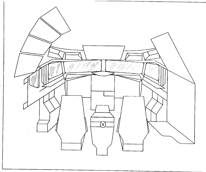
FIGURE B-8. DATA LINK DEVICE LOCATION 8 CENTER PEDESTAL AFT MIDDLE
