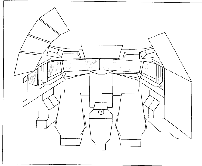
FIGURE B-7. DATA LINK DEVICE LOCATION 7 CENTER PEDESTAL MIDDLE
