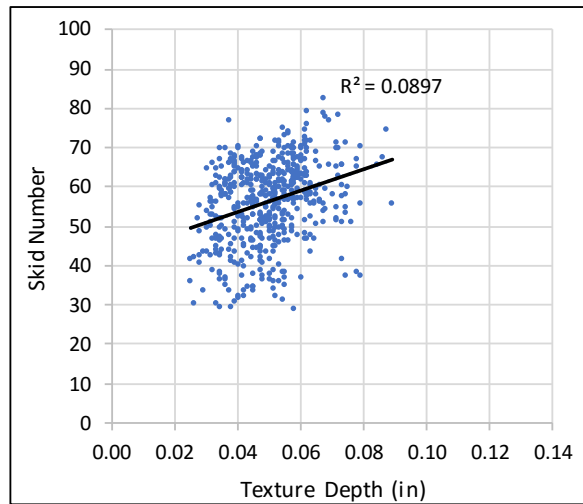
Figure 5.8 SN and Texture Depth for Chip Seal Pavements by Last Seal Year (2017-2012)
