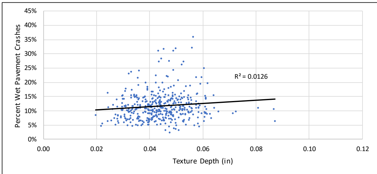
Figure 5.26 2013-2017 Percent Wet Pavement Crashes and Texture Depth - Asphalts
