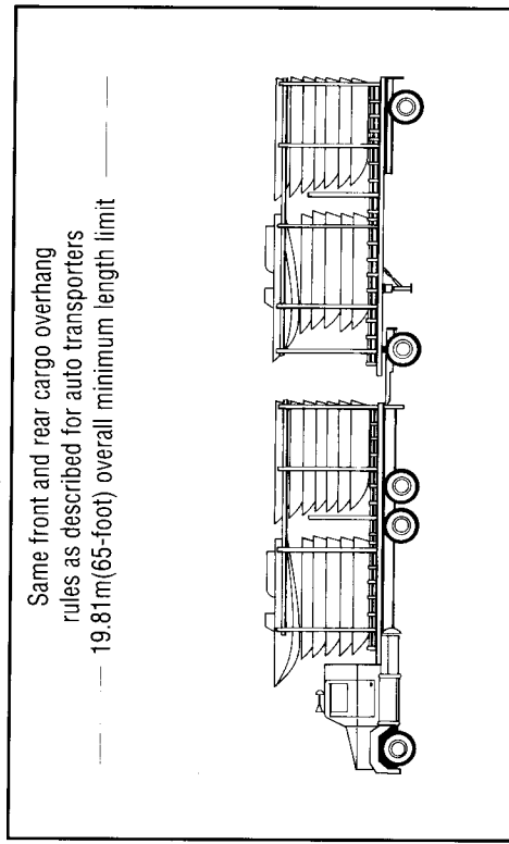
FIGURE 8. STRAIGHT TRUCK TOWING A TRAILER TRANSPORTING BOATS
