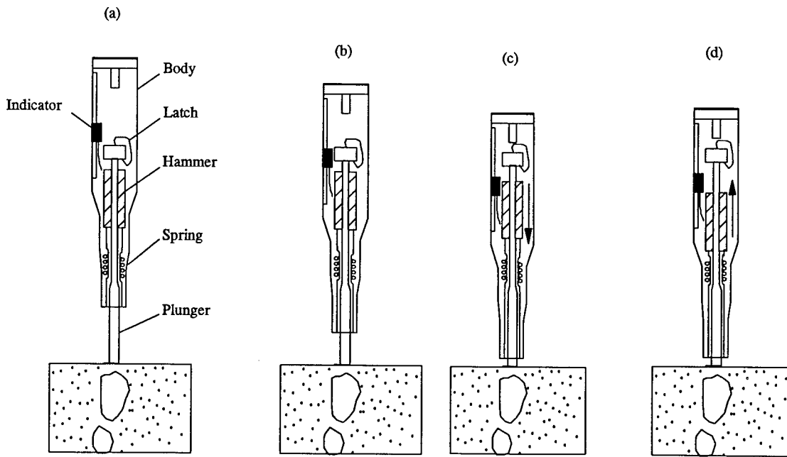
Figure 1. Rebound hammer.
