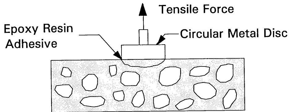
a) Method for testing uncored concrete
