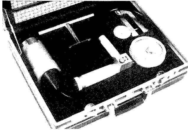
Figure 15. Break-off tester calibrator.
