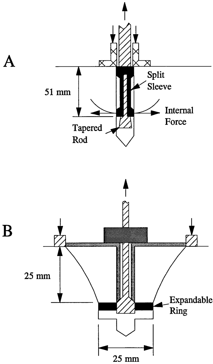
Figure 10. A) Drilled-in test using split-sleeve and tapered bolt. B) CAPO test using rounded shoulder and expandable washer.
