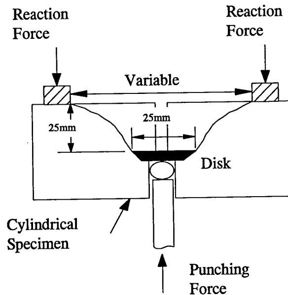
Figure 7. Test configuration for early tests by Kierkegaard-Hansen.
