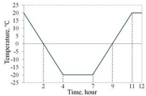
(c) F-T test temperature curve
