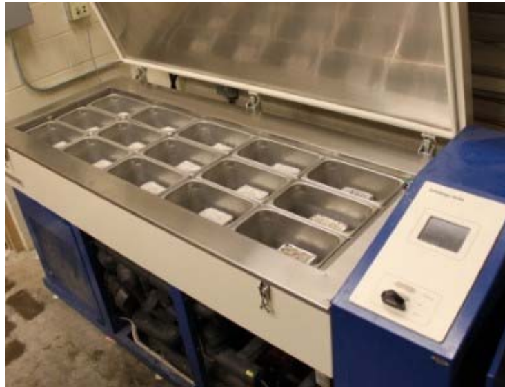
(a) Salt frost test machine
