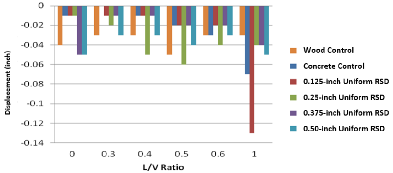
Figure 30. Vertical Field Displacement for Uniform RSD Conditions
