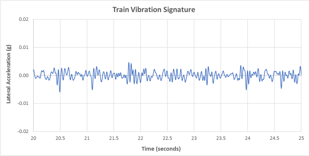
Figure 9 – Example Response Signature from Train Loading
