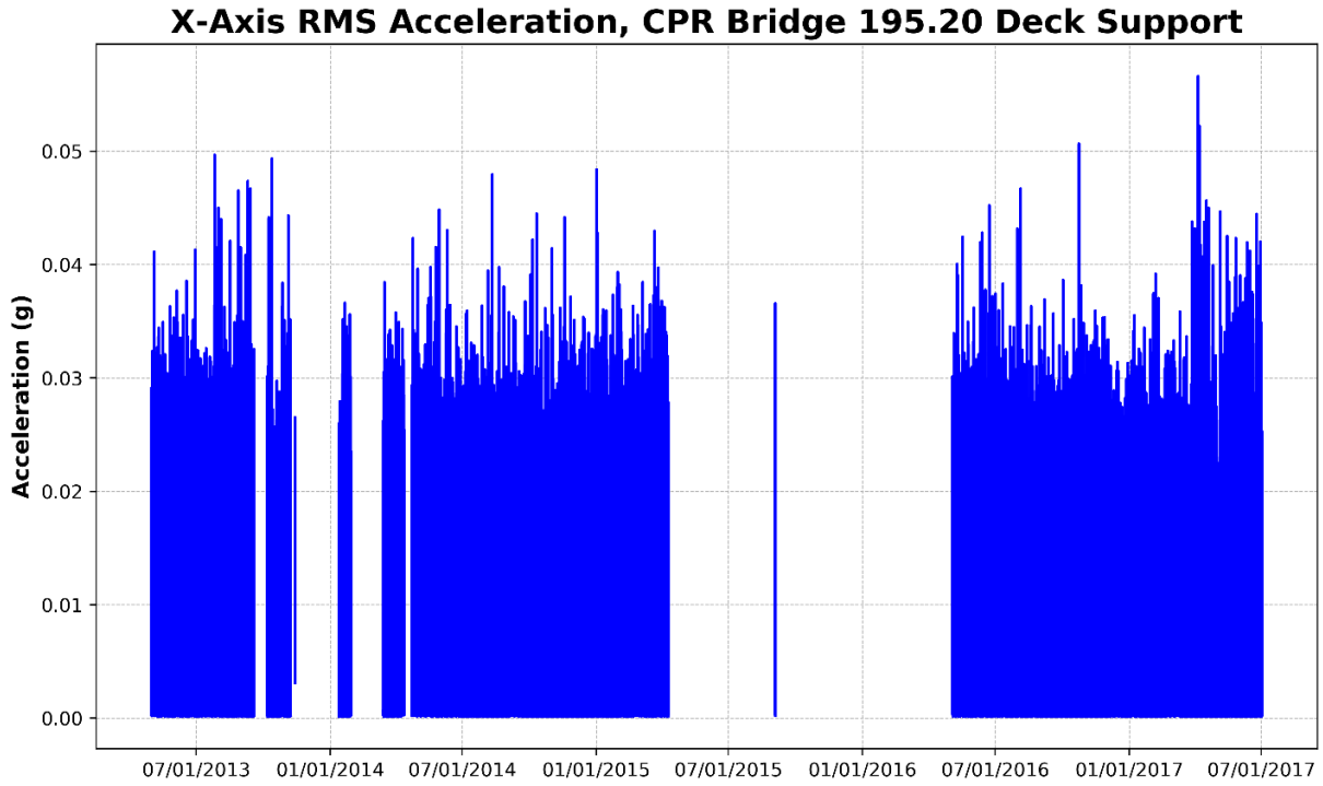
Figure 67 – Deck Support, X-Axis RMS Acceleration (Parallel to Track)
