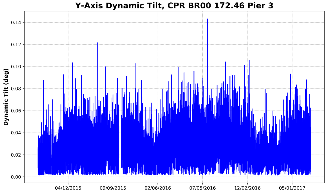
Figure 106 – Pier 3, Y-Axis Dynamic Tilt (Parallel to Track)
