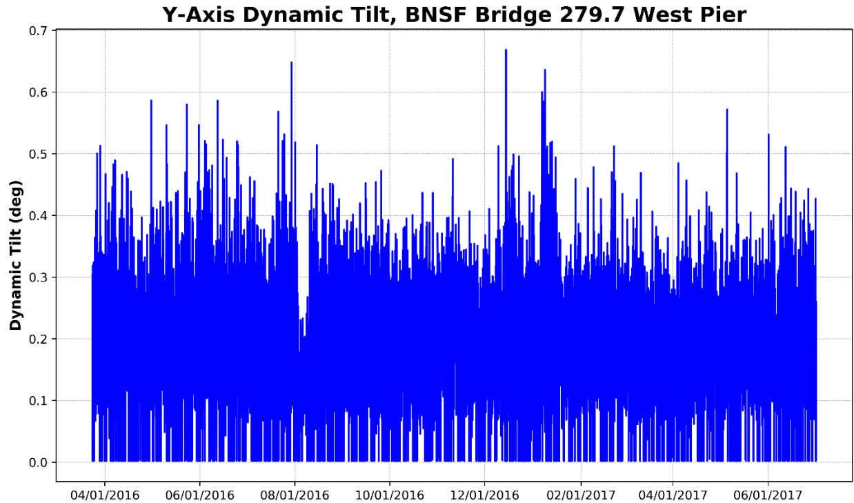
Figure 45 – West Pier, Y-Axis Dynamic Tilt (Parallel to Track)
