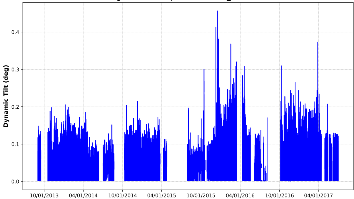
Y-Axis Dynamic Tilt, BNSF Bridge 77.54 Pier 5
