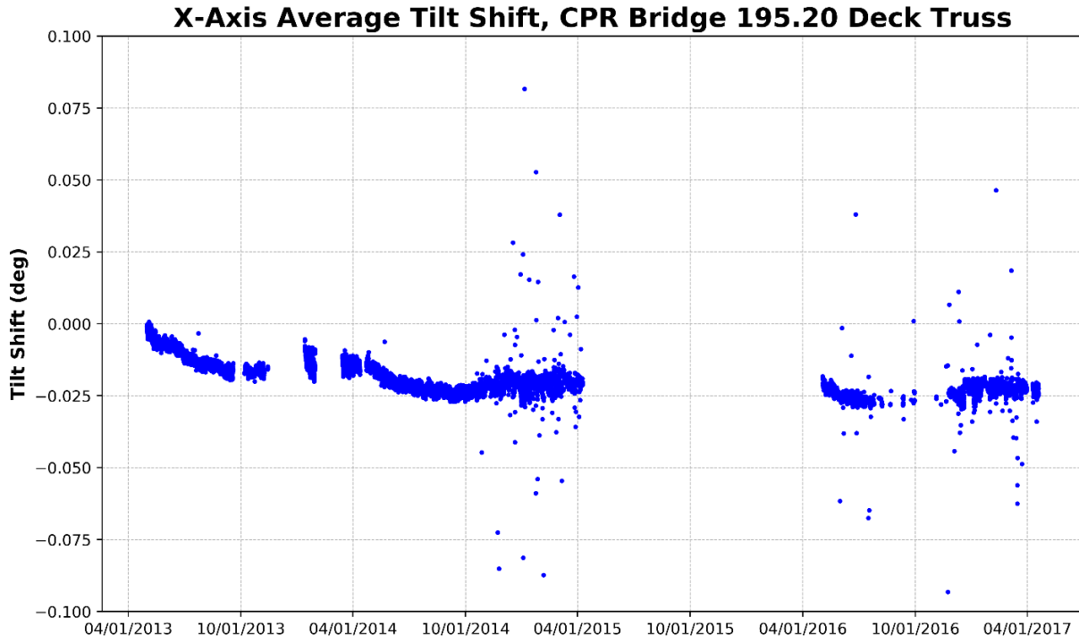
Figure 55 – Deck Truss, X-Axis Average Tilt (Parallel to Track)
