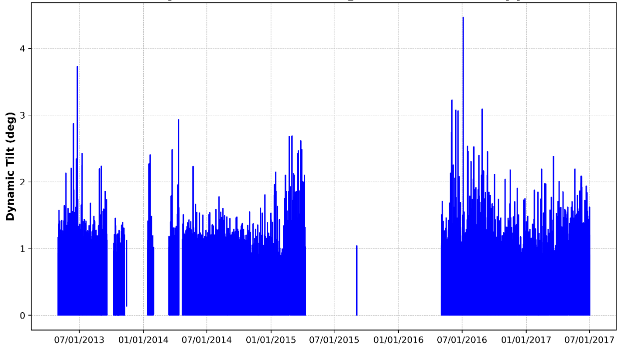
Y-Axis Dynamic Tilt, CPR Bridge 195.20 Deck Support
