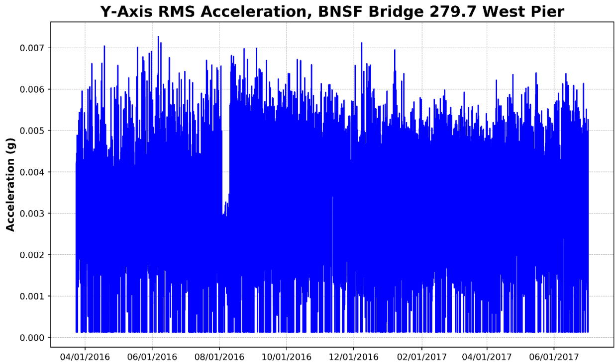
Figure 49 – West Pier, Y-Axis RMS Acceleration (Parallel to Track)
