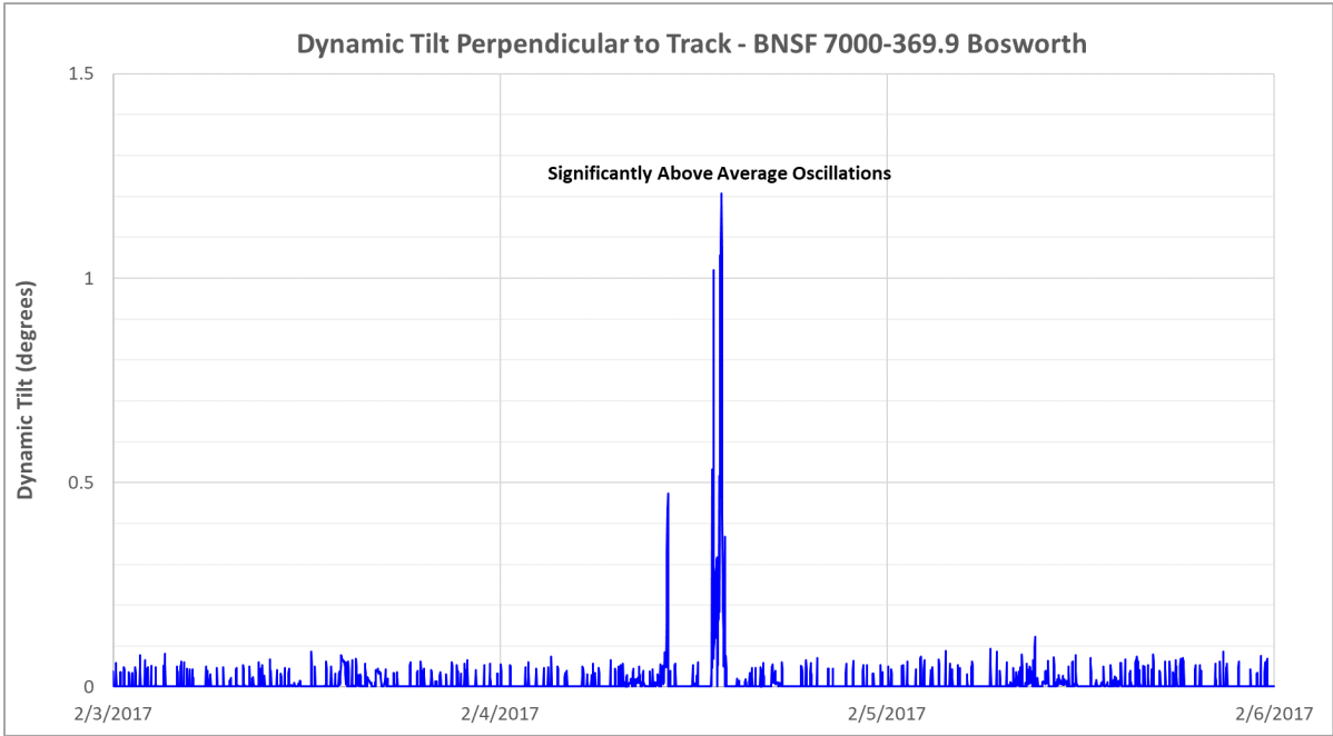
Figure 8 – Example of Above Average Dynamic Oscillations
