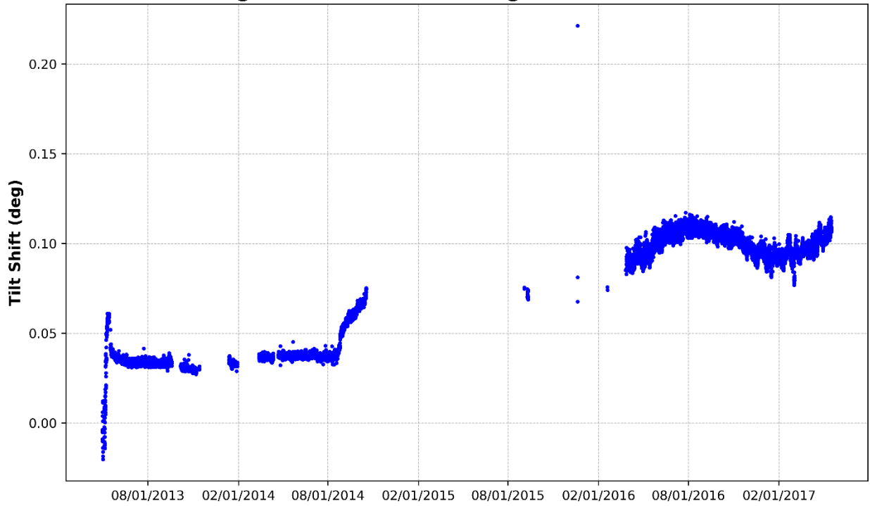
X-Axis Average Tilt Shift, CPR Bridge 195.20 Deck Plate Girder
