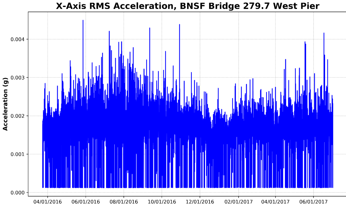
Figure 48 – West Pier, X-Axis RMS Acceleration (Perpendicular to Track)
