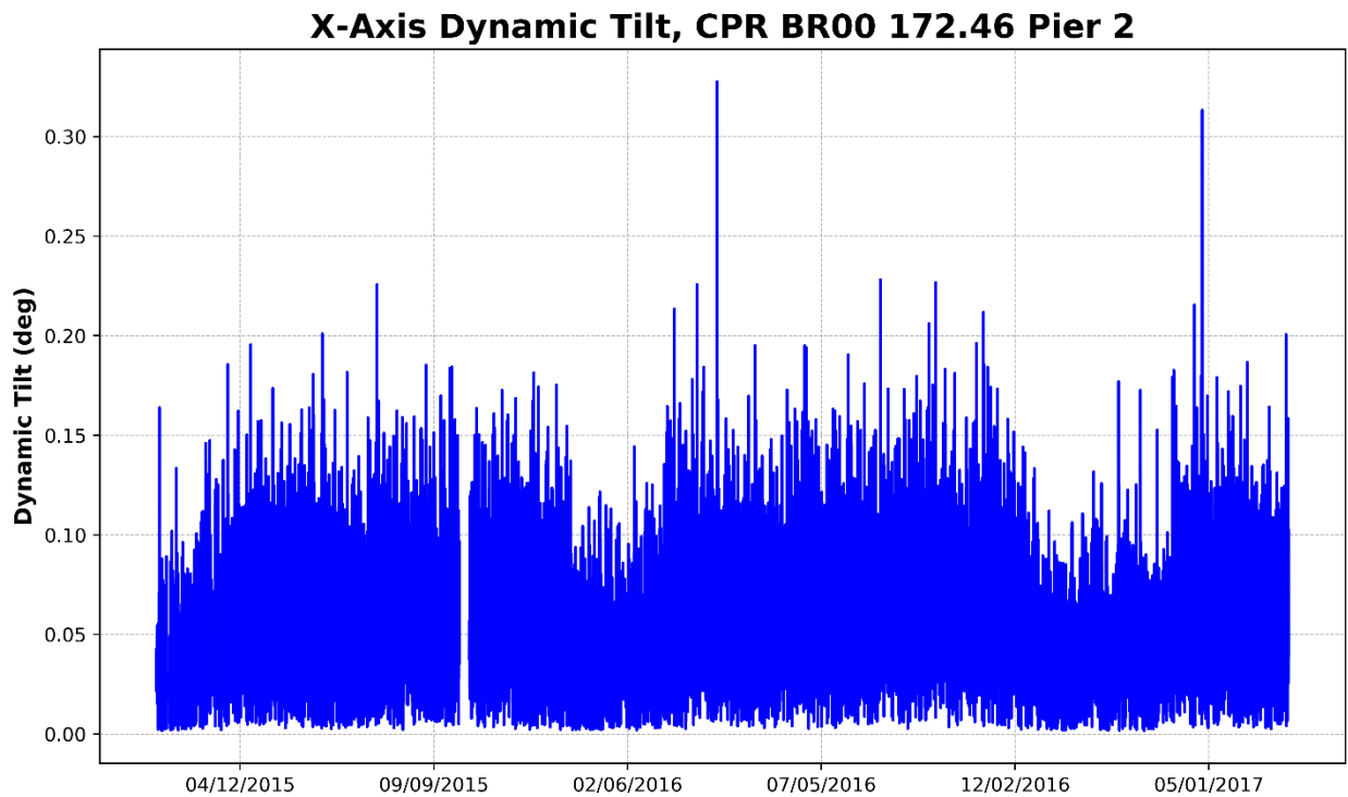
Figure 103 – Pier 2, X-Axis Dynamic Tilt (Perpendicular to Track)
