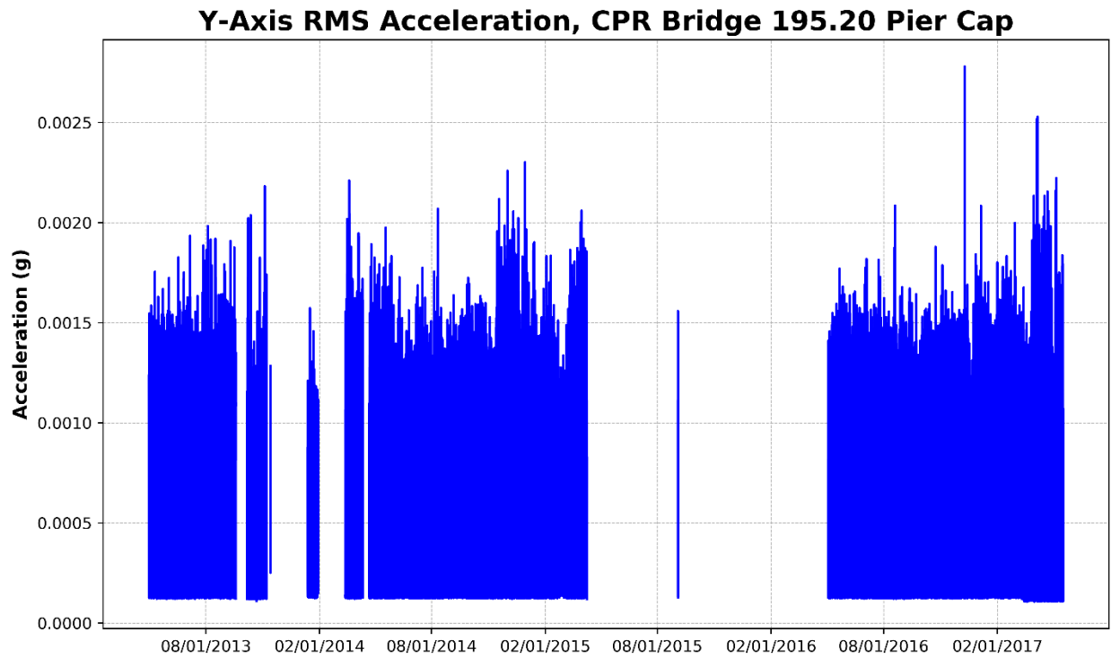
Figure 70 – Pier Cap, Y-Axis RMS Acceleration (Perpendicular to Track)
