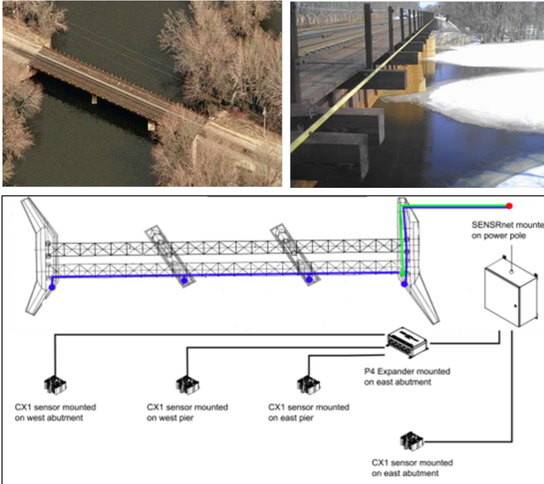
Figure 113 – CPR 121.95 Watertown Sensor Locations
