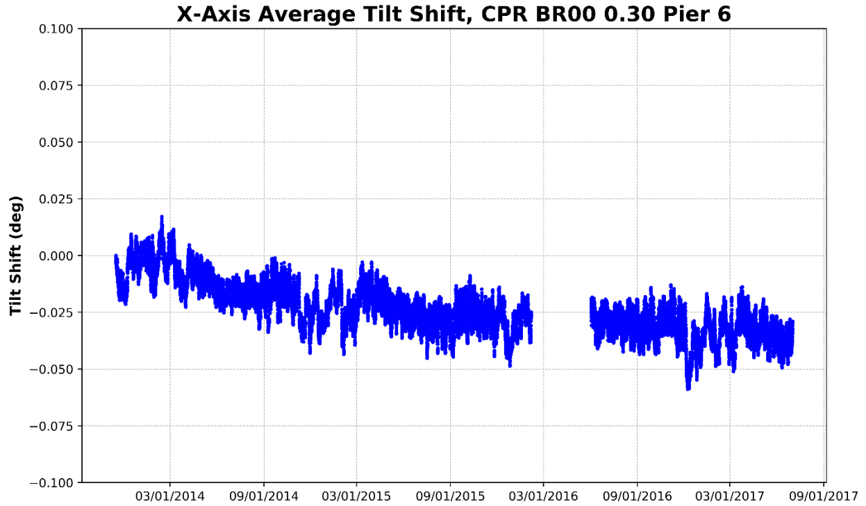
Figure 80 – Pier 6, X-Axis Average Tilt (Parallel to Track)
