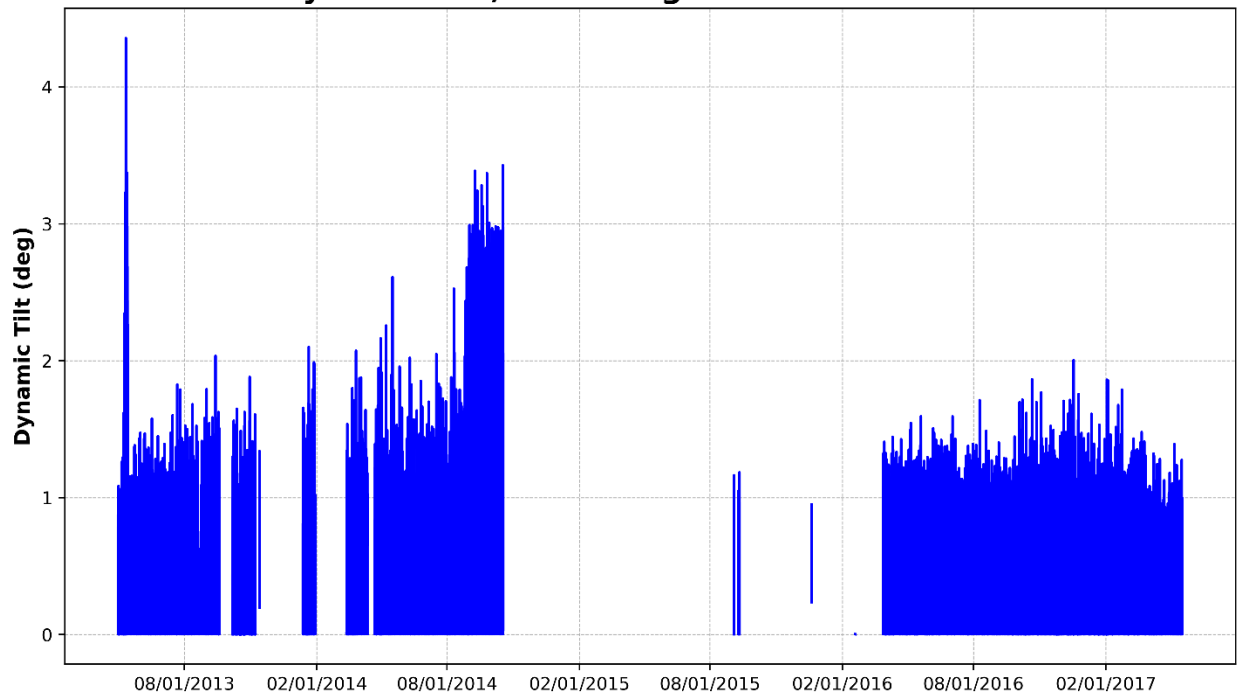
Figure 65 – Deck Plate Girder, X-Axis Dynamic Tilt (Parallel to Track)
