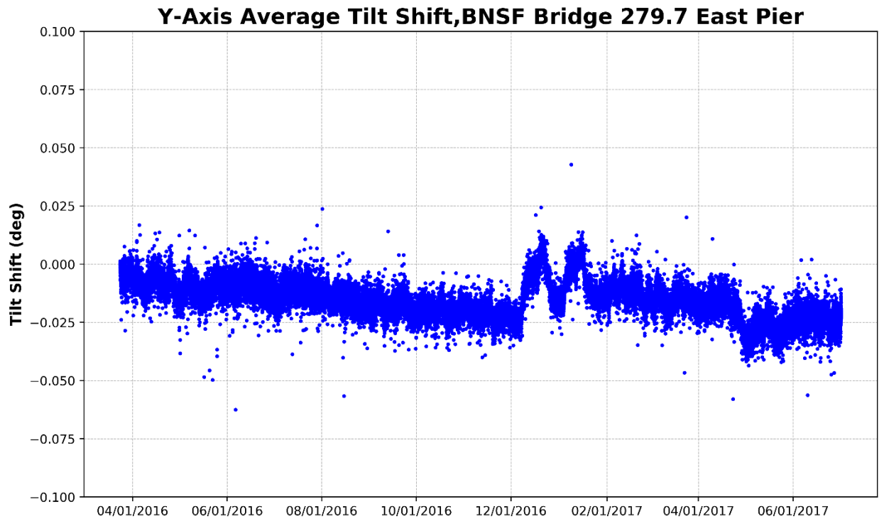
Figure 39 – East Pier, Y-Axis Average Tilt (Parallel to Track)
