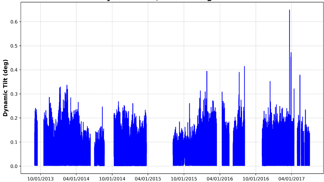
Y-Axis Dynamic Tilt, BNSF Bridge 77.54 Pier 3
