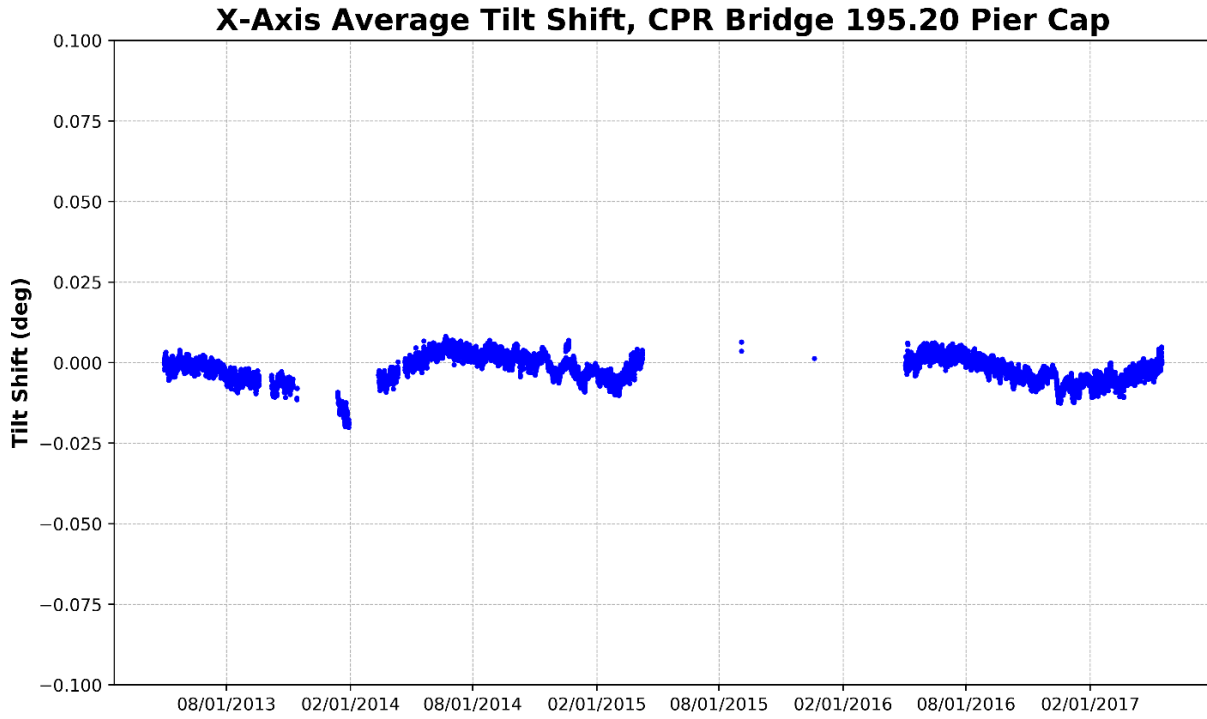
Figure 53 – Pier Cap, X-Axis Average Tilt (Parallel to Track)
