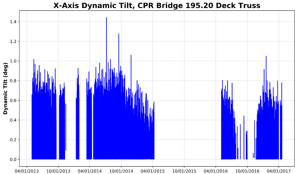
Figure 63 – Deck Truss, X-Axis Dynamic Tilt (Parallel to Track)
