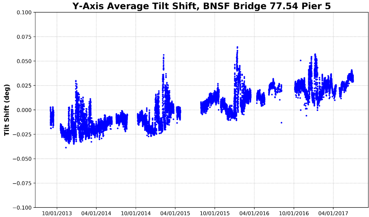
Figure 20 – Pier 5, Y-Axis Average Tilt (Perpendicular to Track)
