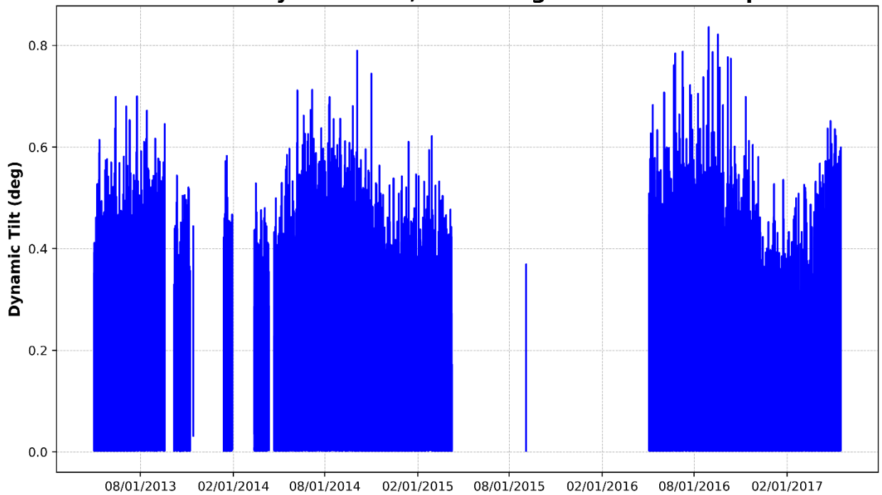
X-Axis Dynamic Tilt, CPR Bridge 195.20 Pier Cap
