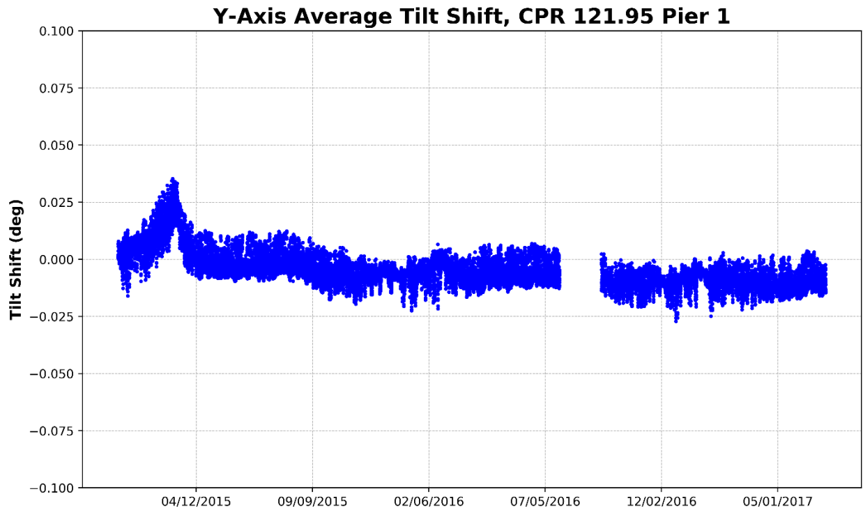
Figure 115 – Pier 1, Y-Axis Average Tilt
