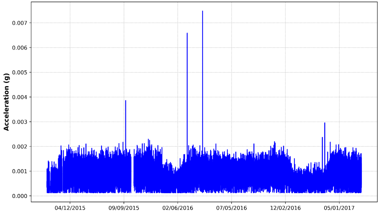
Figure 109 – Pier 2, X-Axis RMS Acceleration (Perpendicular to Track)
