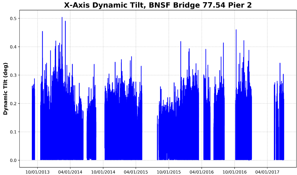
Figure 21 – Pier 2, X-Axis Dynamic Tilt (Parallel to Track)
