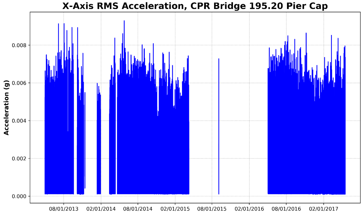
Figure 69 – Pier Cap, X-Axis RMS Acceleration (Parallel to Track)
