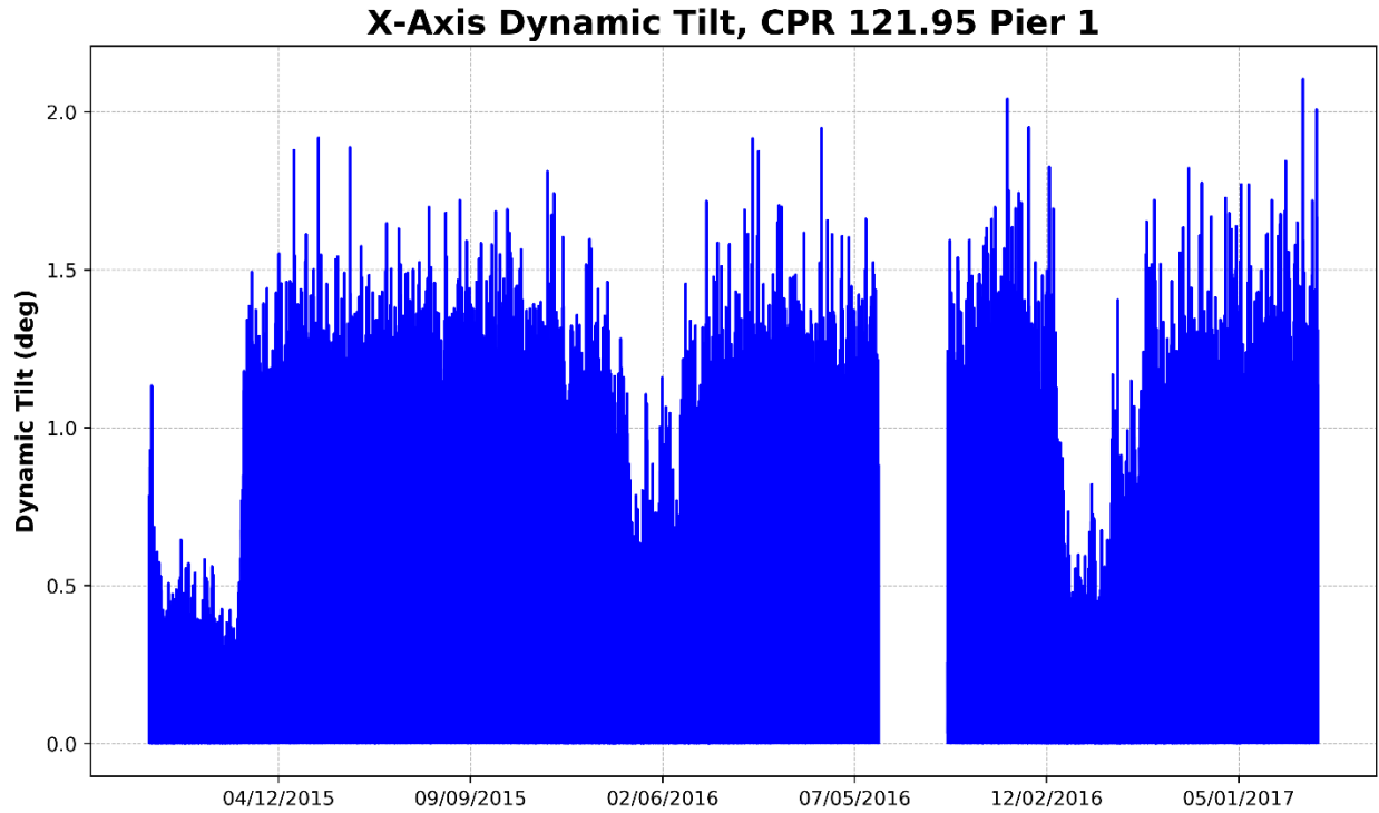
Figure 122 – Pier 1, X-Axis Dynamic Tilt
