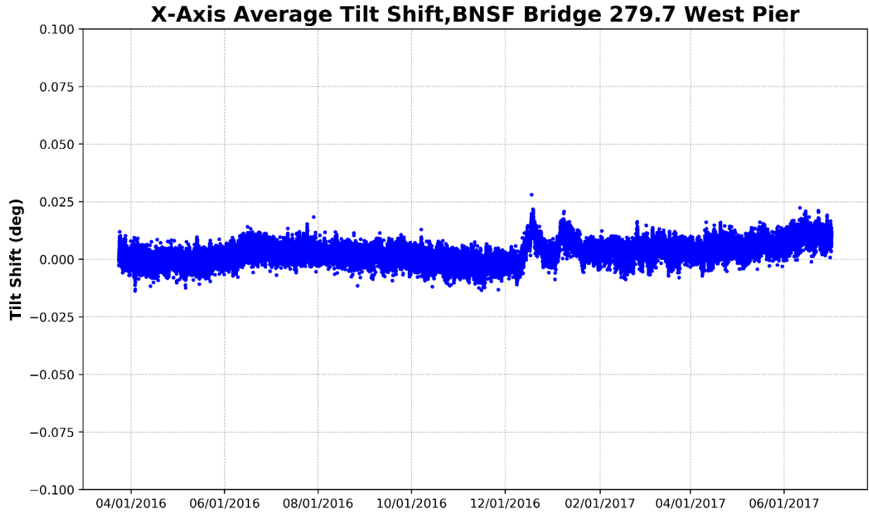
Figure 40 – West Pier, X-Axis Average Tilt (Perpendicular to Track)
