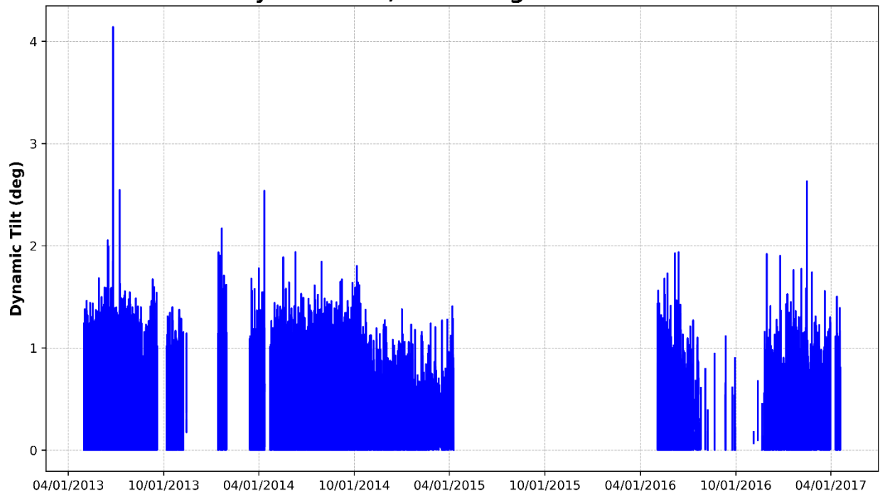
Figure 64 – Deck Truss, Y-Axis Dynamic Tilt (Perpendicular to Track)
