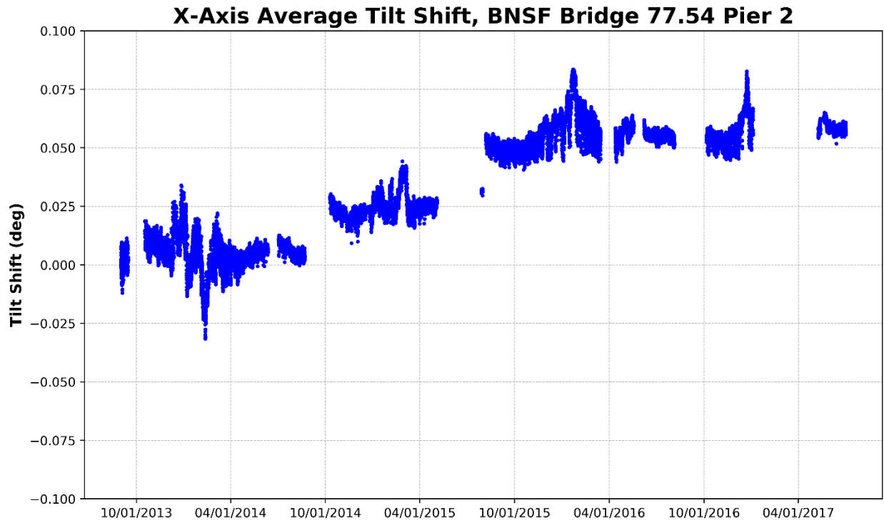
Figure 13 – Pier 2, X-Axis Average Tilt (Parallel to Track)
