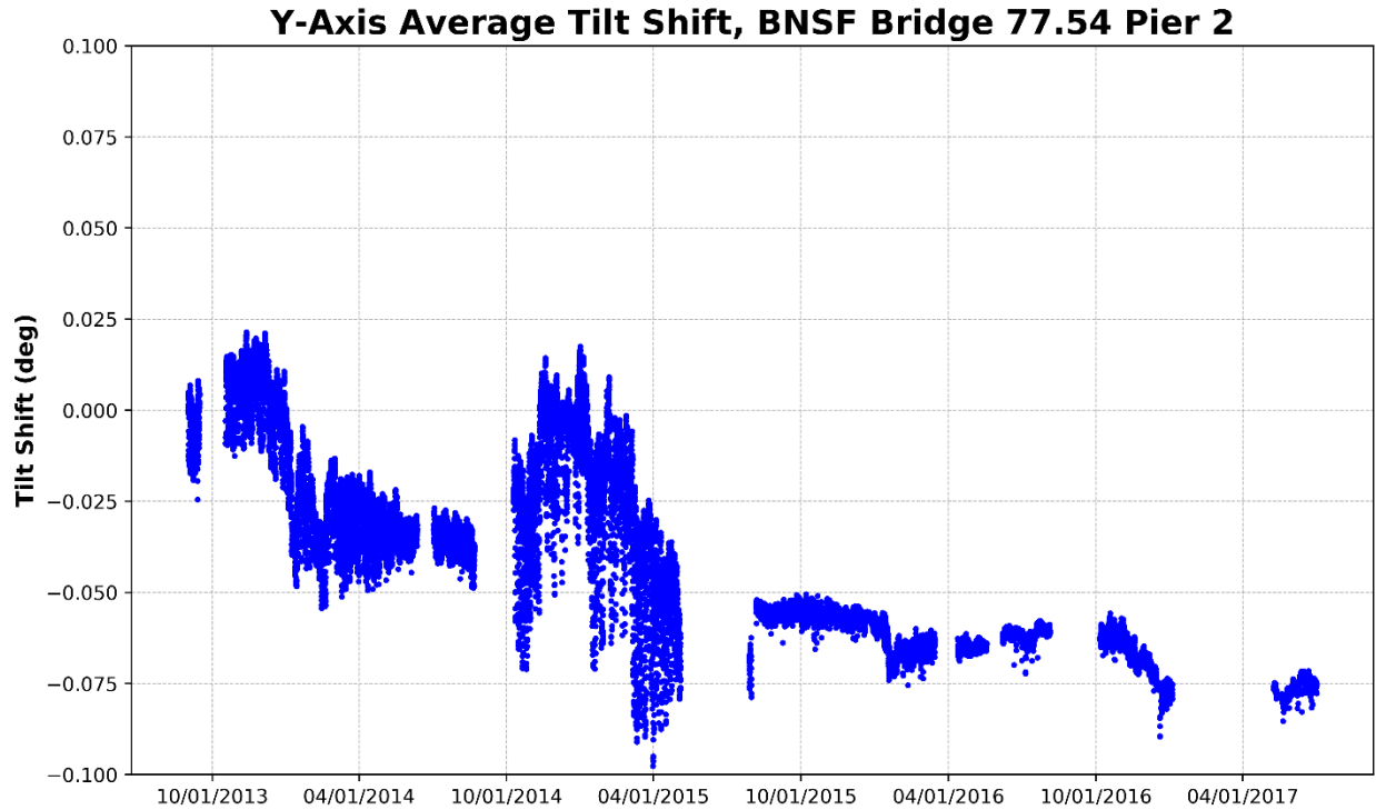
Figure 14 – Pier 2, Y-Axis Average Tilt (Perpendicular to Track)
