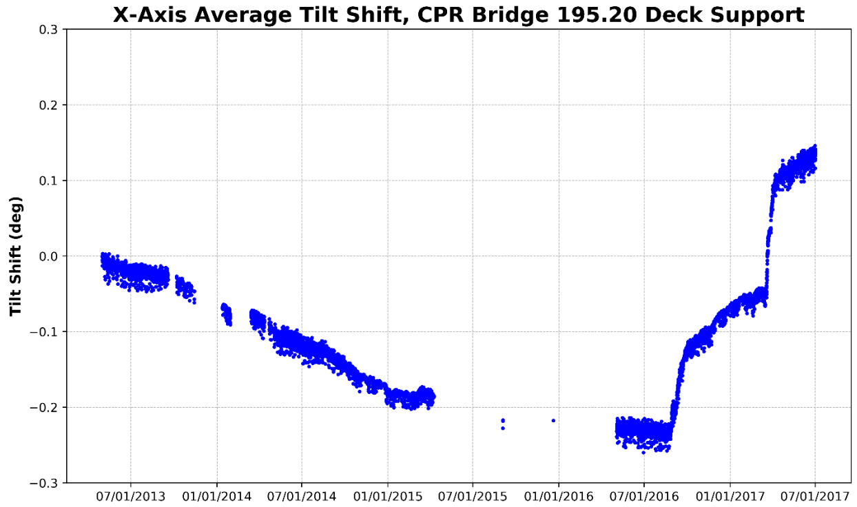
Figure 51 – Deck Support, X-Axis Average Tilt (Parallel to Track)
