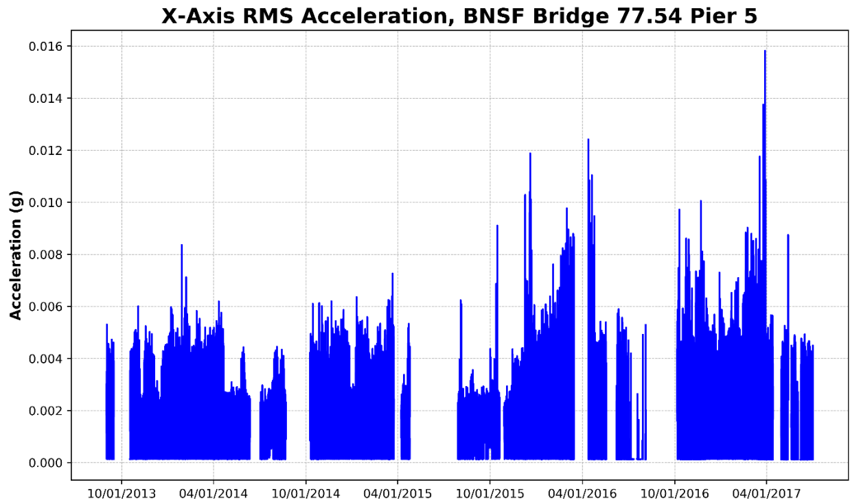
Figure 35 – Pier 5, X-Axis RMS Acceleration (Parallel to Track)
