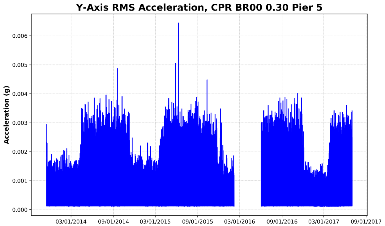
Figure 91 – Pier 5, Y-Axis RMS Acceleration (Perpendicular to Track)
