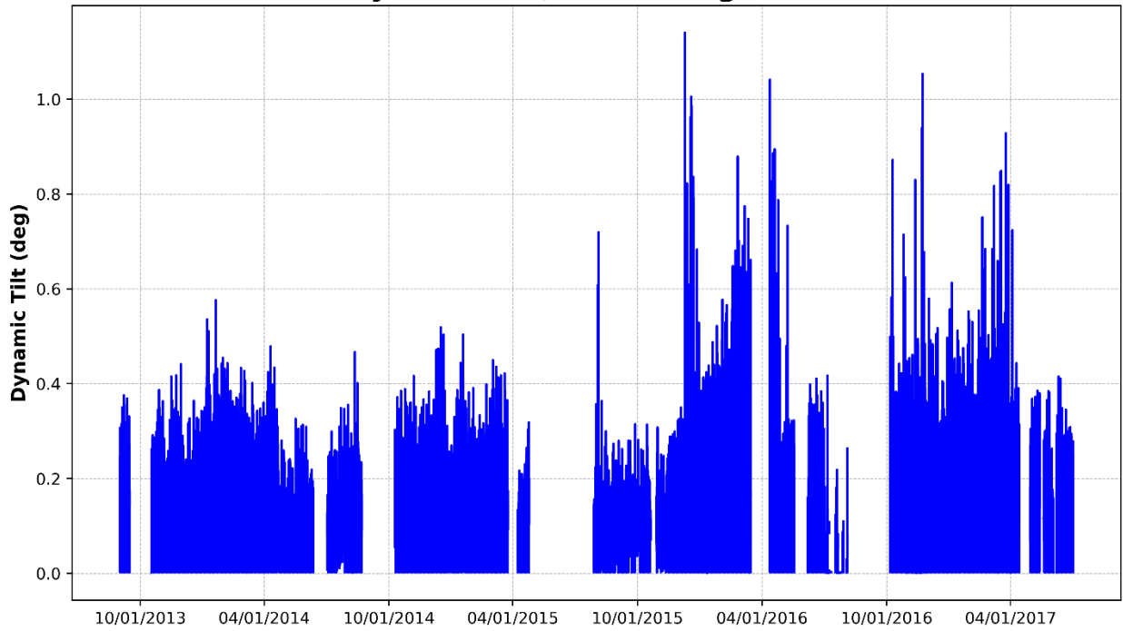
X-Axis Dynamic Tilt, BNSF Bridge 77.54 Pier 5
