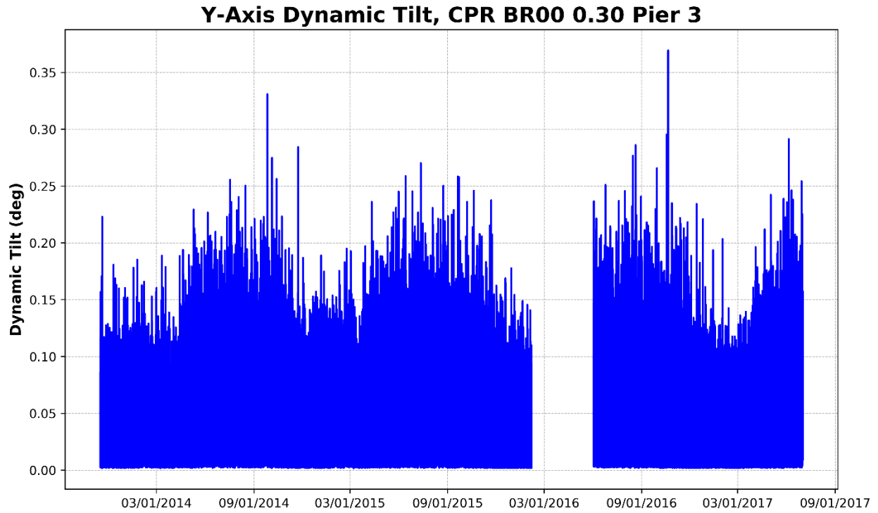
Figure 83 – Pier 3, Y-Axis Dynamic Tilt (Perpendicular to Track)
