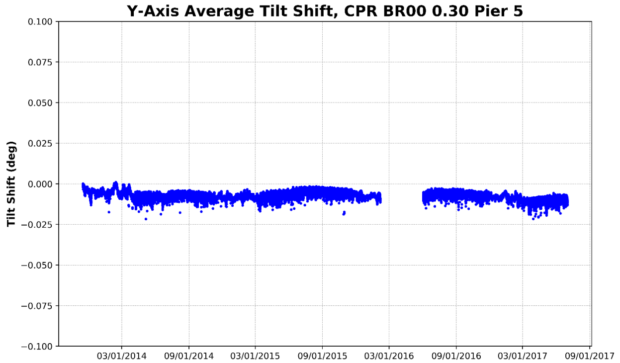
Figure 79 – Pier 5, Y-Axis Average Tilt (Perpendicular to Track)
