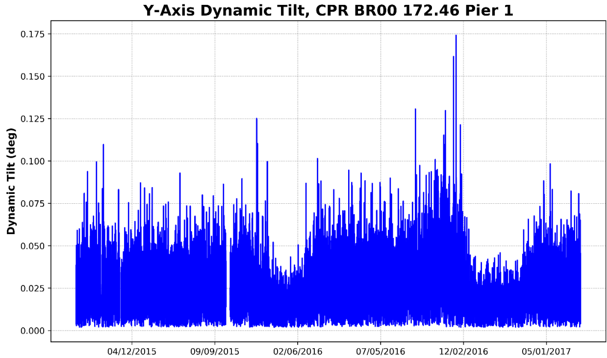
Figure 102 – Pier 1, Y-Axis Dynamic Tilt (Parallel to Track)
