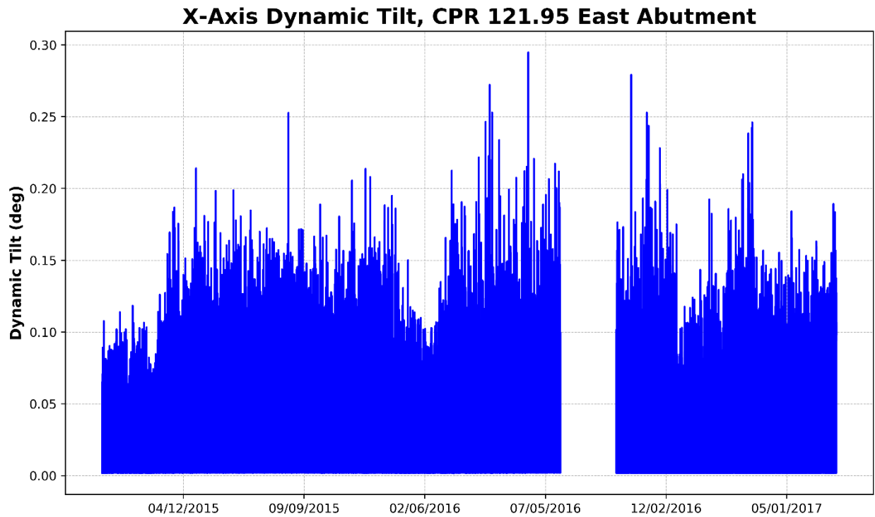
Figure 128 – East Abutment, X-Axis Dynamic Tilt (Perpendicular to Track)
