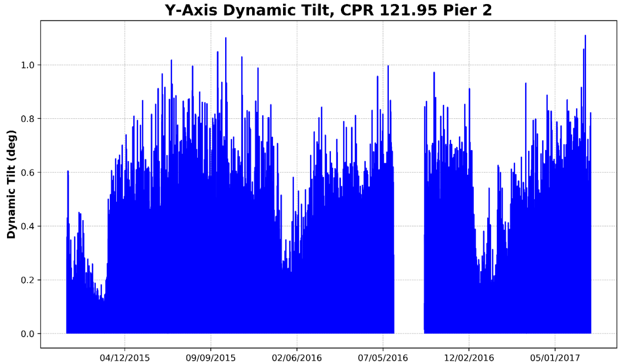
Figure 125 – Pier 2, Y-Axis Dynamic Tilt
