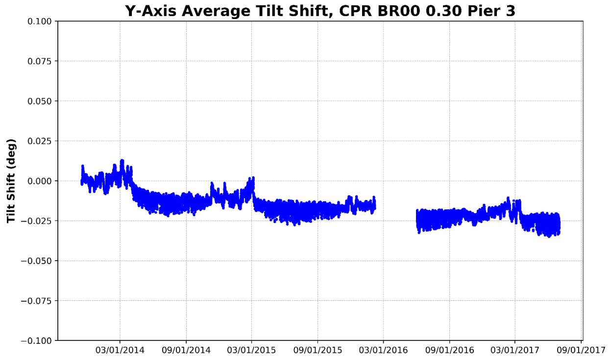
Figure 77 – Pier 3, Y-Axis Average Tilt (Perpendicular to Track)
