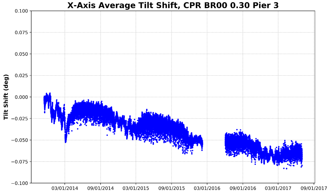
Figure 76 – Pier 3, X-Axis Average Tilt (Parallel to Track)
