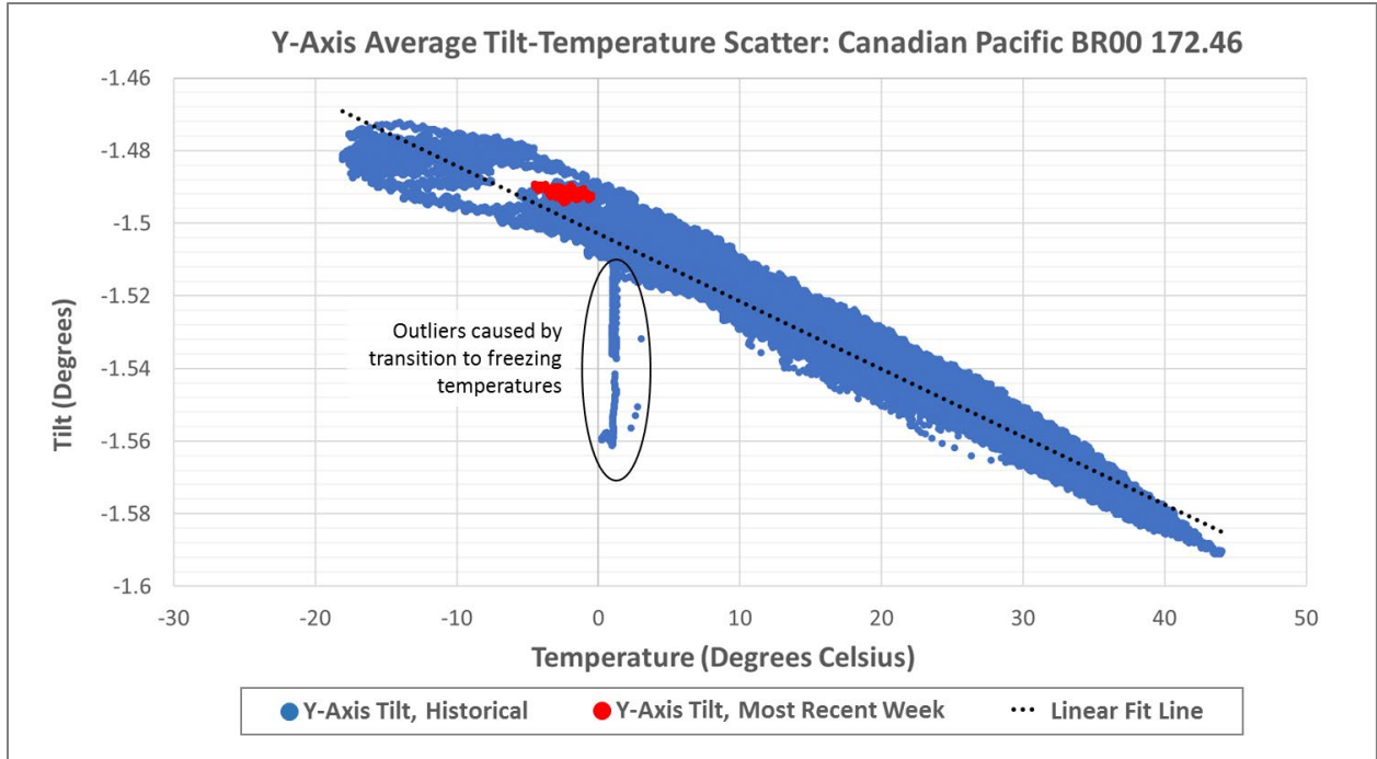
Figure 6 – Visual Analysis of Tilt-Temperature Relationship, Canadian Pacific BR00 172.46 West Pier
