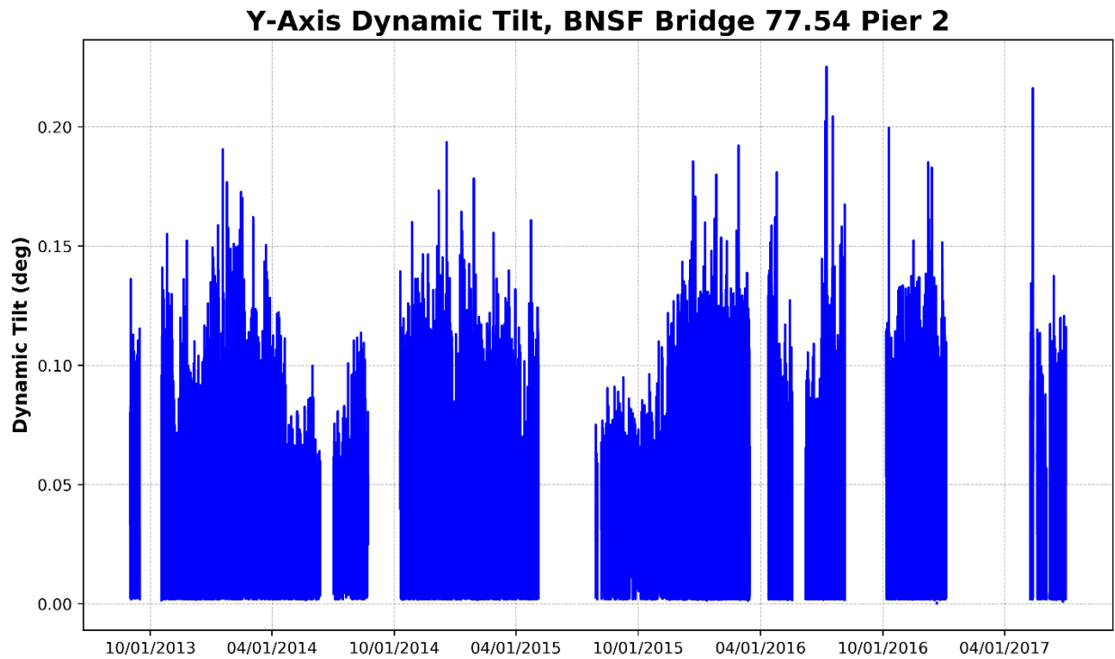
Figure 22 – Pier 2, Y-Axis Dynamic Tilt (Perpendicular to Track)
