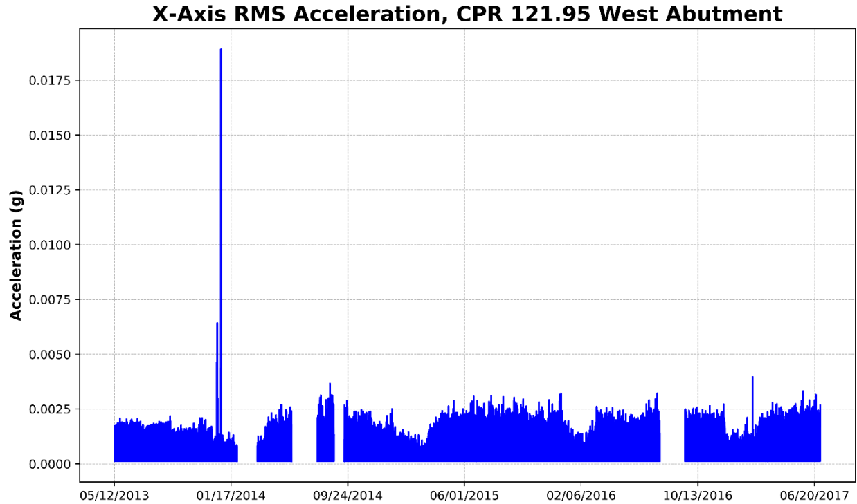
Figure 134 – West Abutment, X-Axis RMS Acceleration (Perpendicular to Track)
