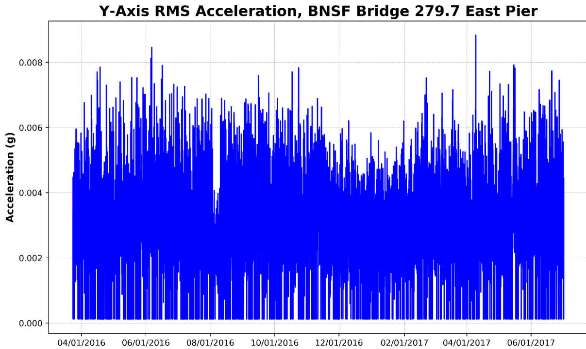
Figure 47 – East Pier, Y-Axis RMS Acceleration (Parallel to Track)
