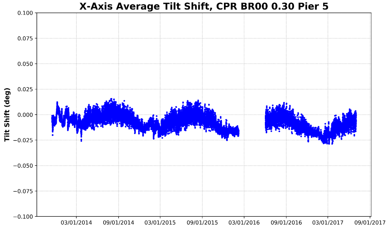
Figure 78 – Pier 5, X-Axis Average Tilt (Parallel to Track)
