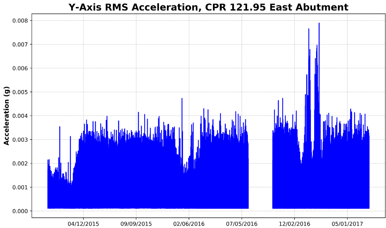
Figure 137 – East Abutment, Y-Axis RMS Acceleration (Parallel to Track)
