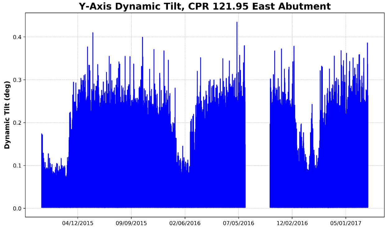
Figure 129 – East Abutment, Y-Axis Dynamic Tilt (Parallel to Track)
