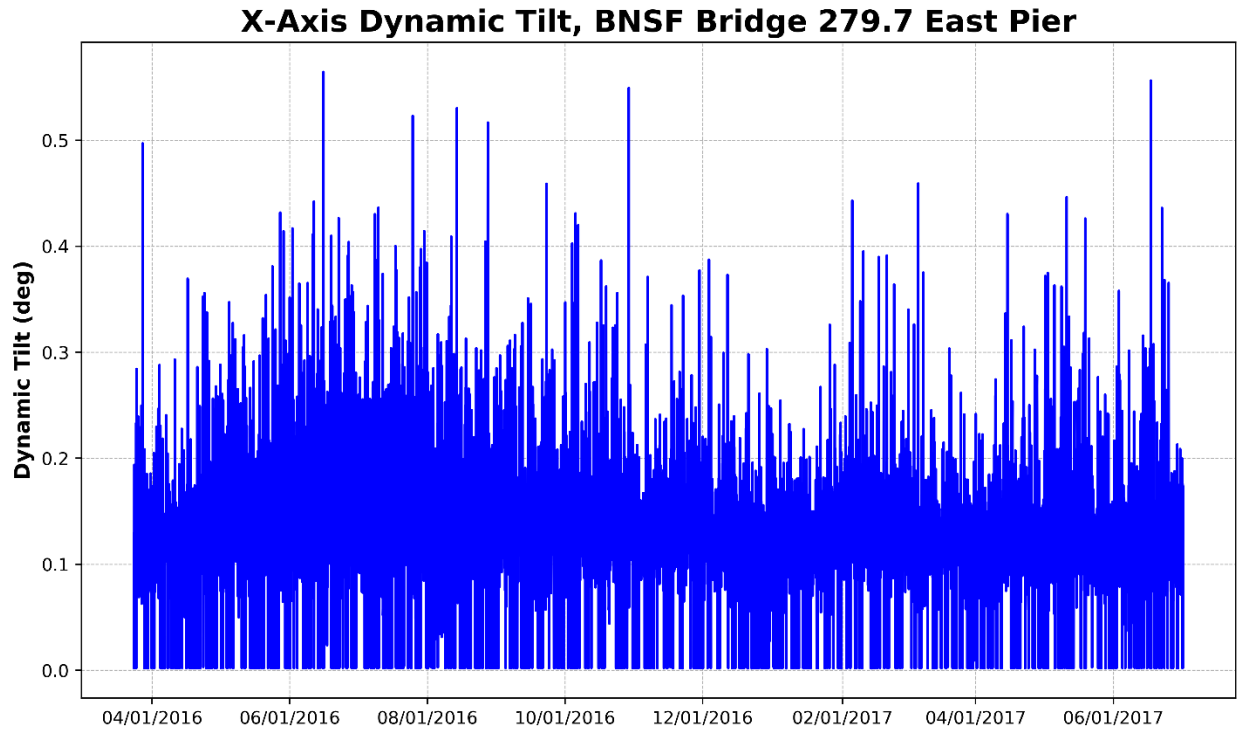
Figure 42 – East Pier, X-Axis Dynamic Tilt (Perpendicular to Track)
