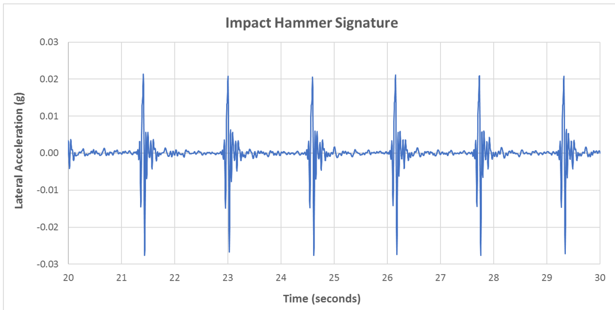
Figure 11 – Example Response Signature from Impact Hammer
