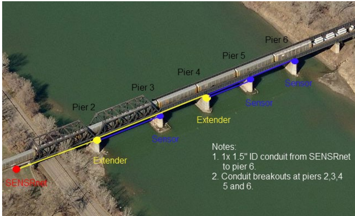
Figure 75 – CPR Medicine Hat Monitoring System Layout
