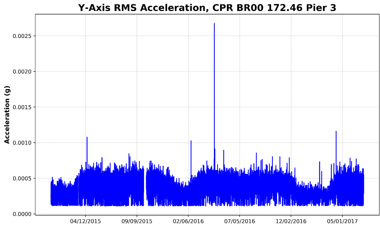
Figure 112 – Pier 3, Y-Axis RMS Acceleration (Parallel to Track)
