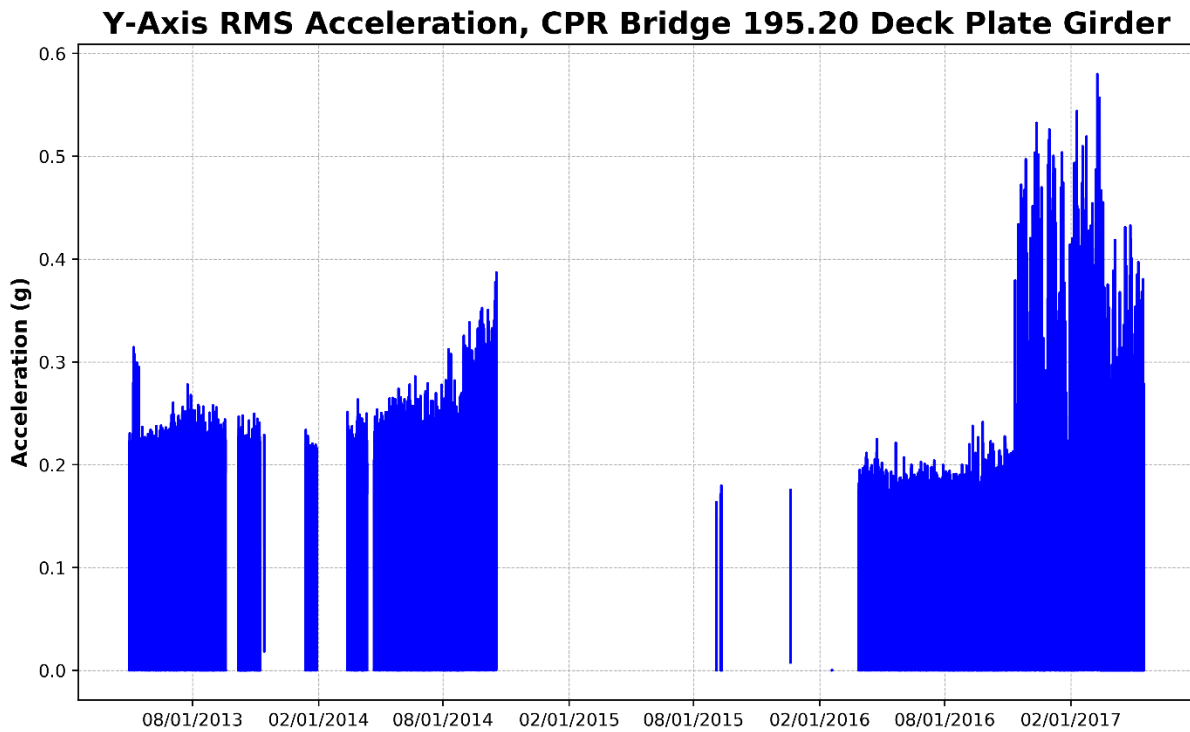
Figure 74 – Deck Plate Girder, Y-Axis RMS Acceleration (Perpendicular to Track)
