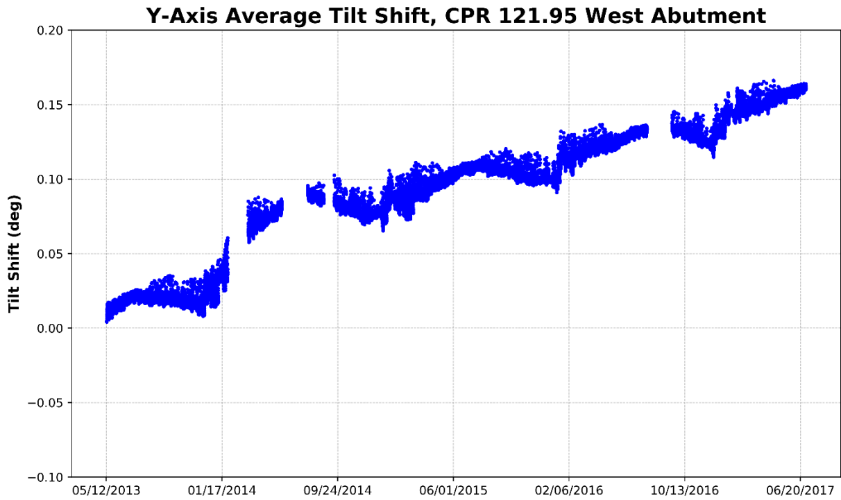
Figure 119 – West Abutment, Y-Axis Average Tilt (Parallel to Track)
