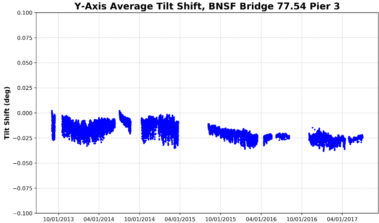
Figure 16 – Pier 3, Y-Axis Average Tilt (Perpendicular to Track)
