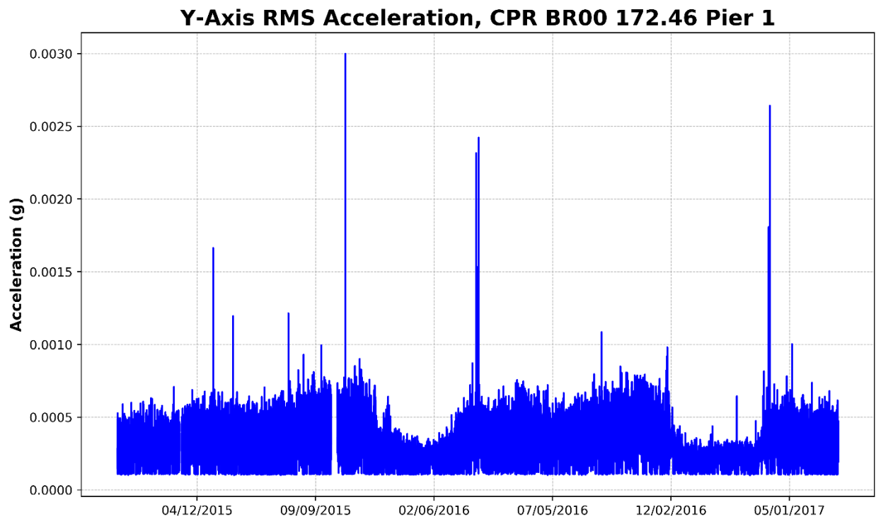
Figure 108 – Pier 1, Y-Axis RMS Acceleration (Parallel to Track)
