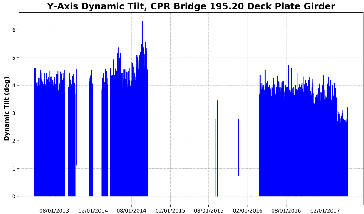
Figure 66 – Deck Plate Girder, Y-Axis Dynamic Tilt (Perpendicular to Track)
