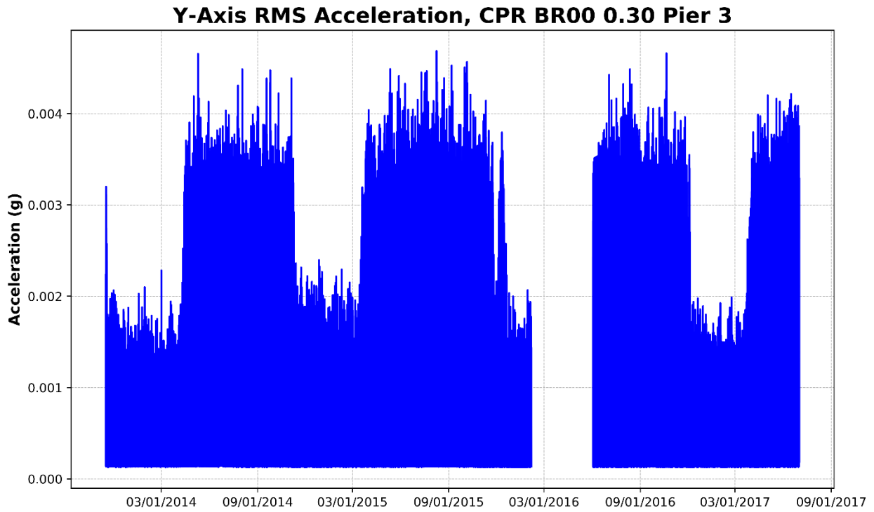
Figure 89 – Pier 3, Y-Axis RMS Acceleration (Perpendicular to Track)
