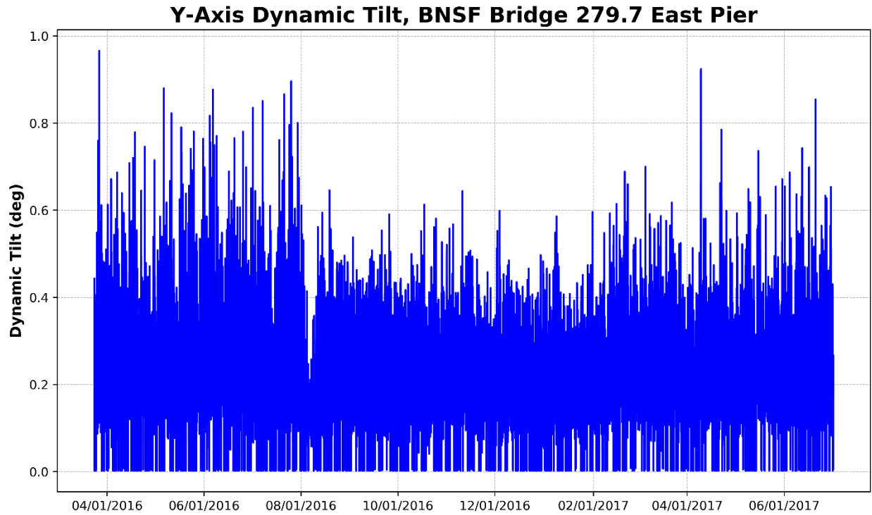
Figure 43 – East Pier, Y-Axis Dynamic Tilt (Parallel to Track)
