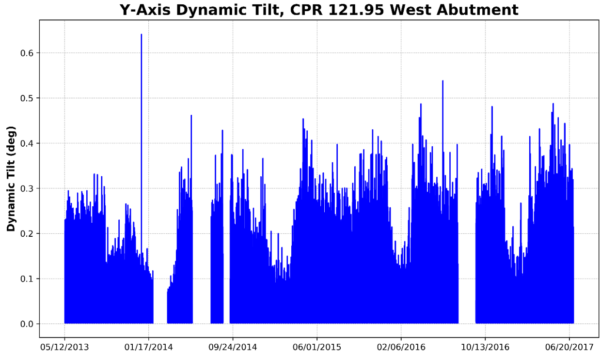
Figure 127 – West Abutment, Y-Axis Dynamic Tilt (Parallel to Track)
