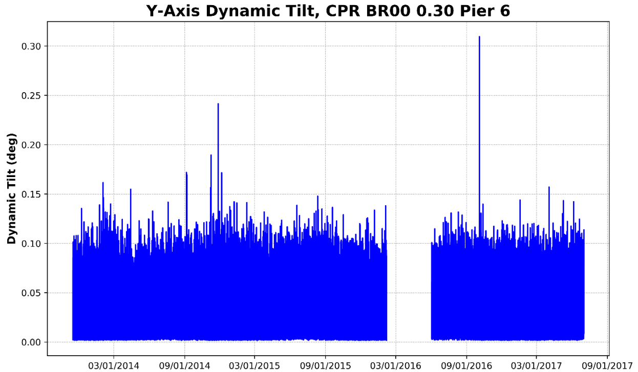
Figure 87 – Pier 6, Y-Axis Dynamic Tilt (Perpendicular to Track)
