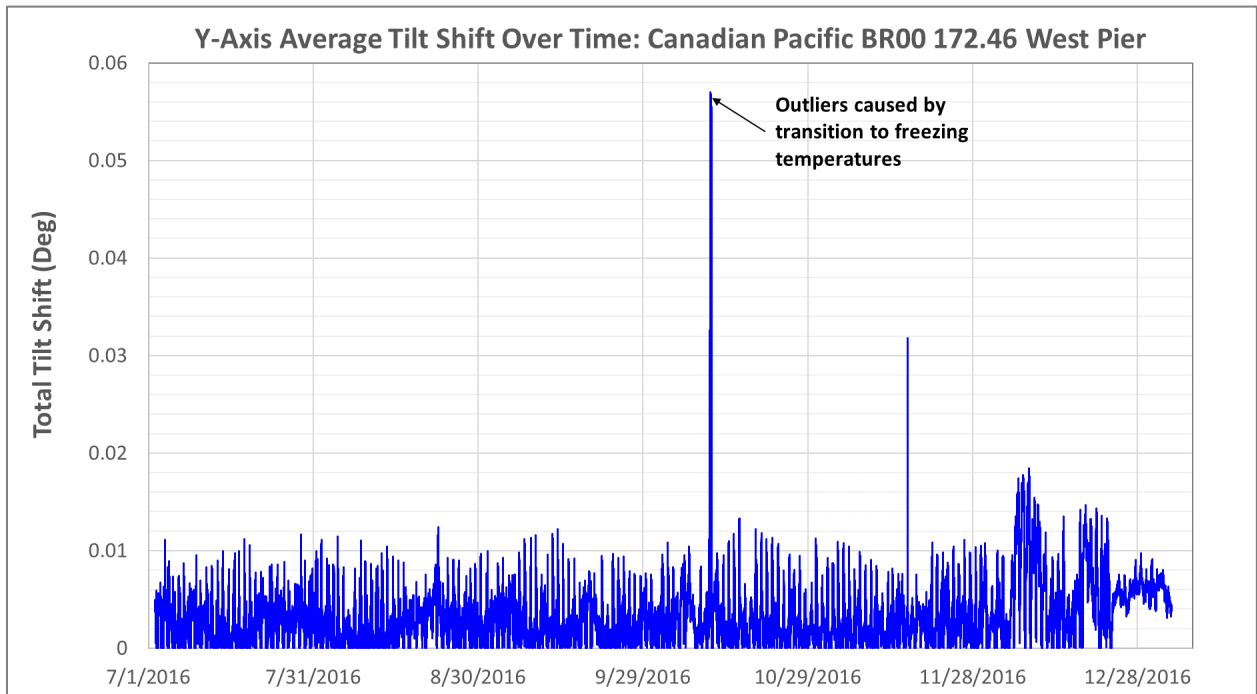
Figure 7 – Tilt Shift of Canadian Pacific BR00 172.46 West Pier Over Time
