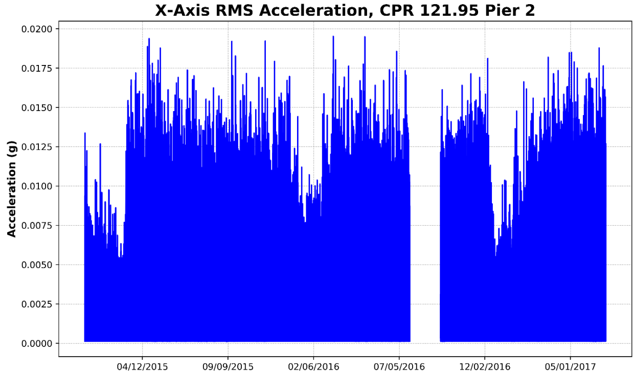
Figure 132 – Pier 2, X-Axis RMS Acceleration
