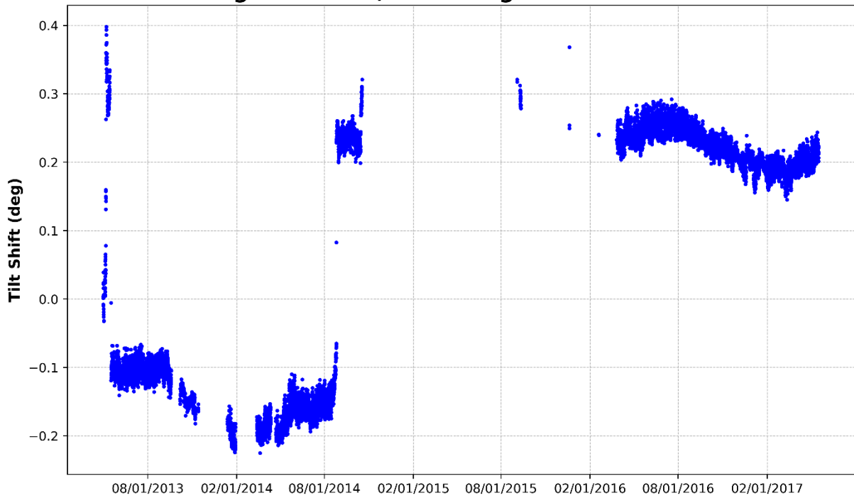
Y-Axis Average Tilt Shift, CPR Bridge 195.20 Deck Plate Girder
