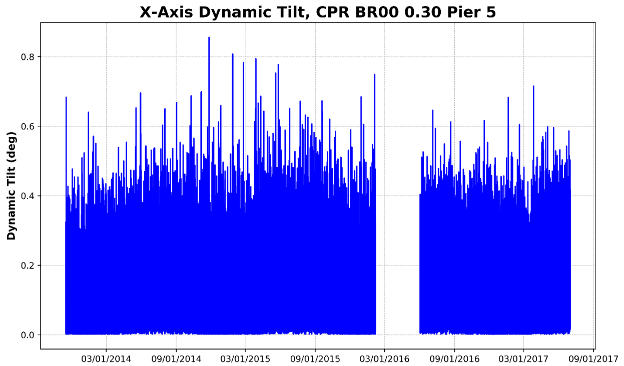
Figure 84 – Pier 5, X-Axis Dynamic Tilt (Parallel to Track)
