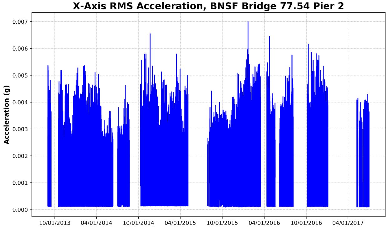
Figure 29 – Pier 2, X-Axis RMS Acceleration (Parallel to Track)
