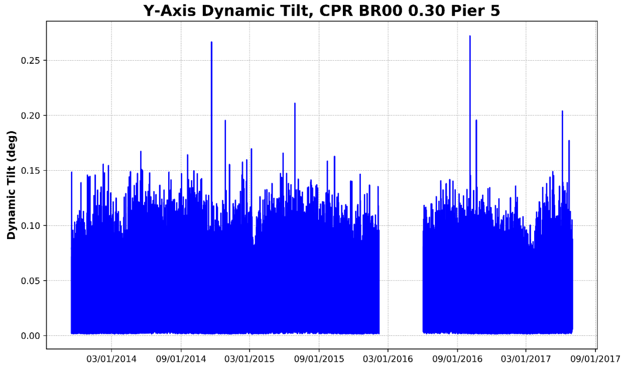
Figure 85 – Pier 5, Y-Axis Dynamic Tilt (Perpendicular to Track)
