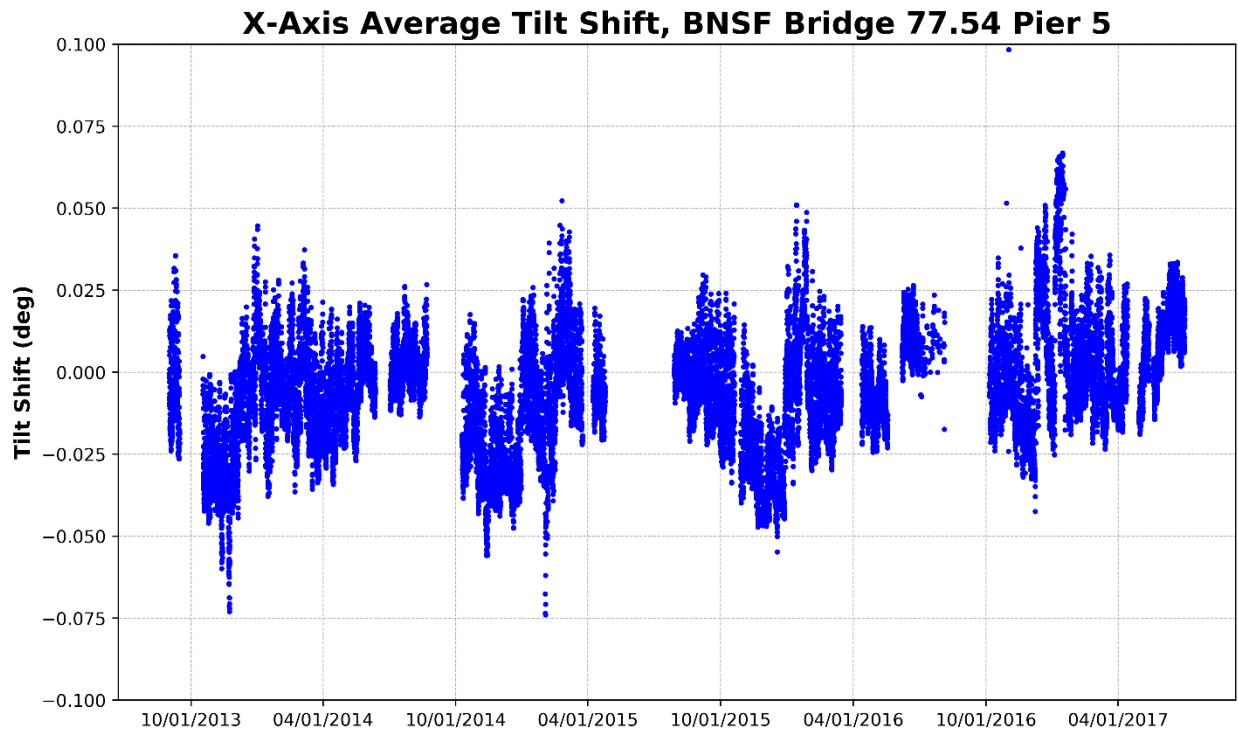
Figure 19 – Pier 5, X-Axis Average Tilt (Parallel to Track)
