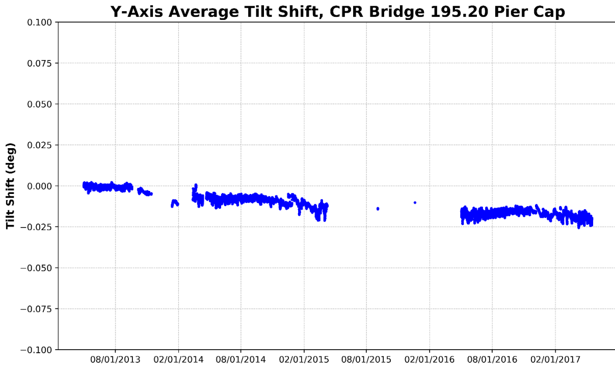
Figure 54 – Pier Cap, Y-Axis Average Tilt (Perpendicular to Track)
