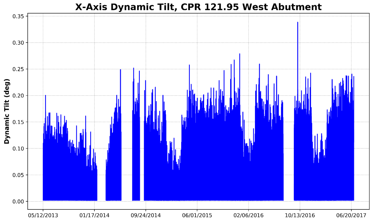
Figure 126 – West Abutment, X-Axis Dynamic Tilt (Perpendicular to Track)
