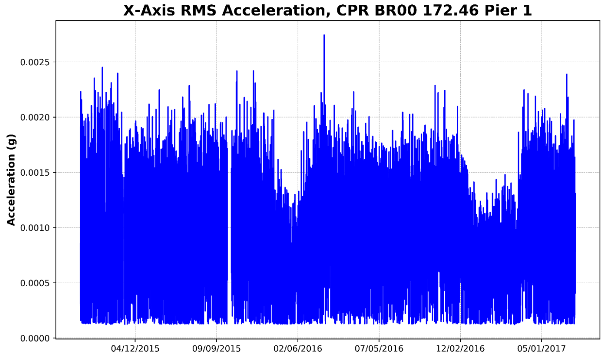
Figure 107 – Pier 1, X-Axis RMS Acceleration (Perpendicular to Track)
