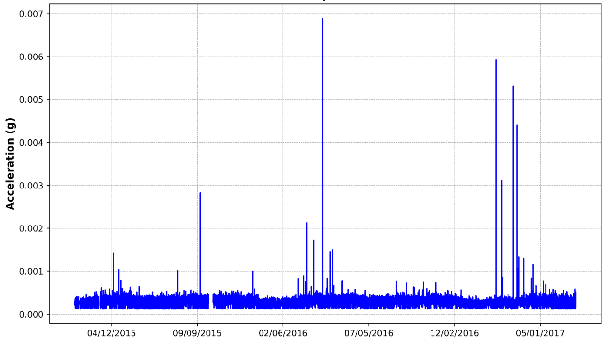
Figure 110 – Pier 2, Y-Axis RMS Acceleration (Parallel to Track)
