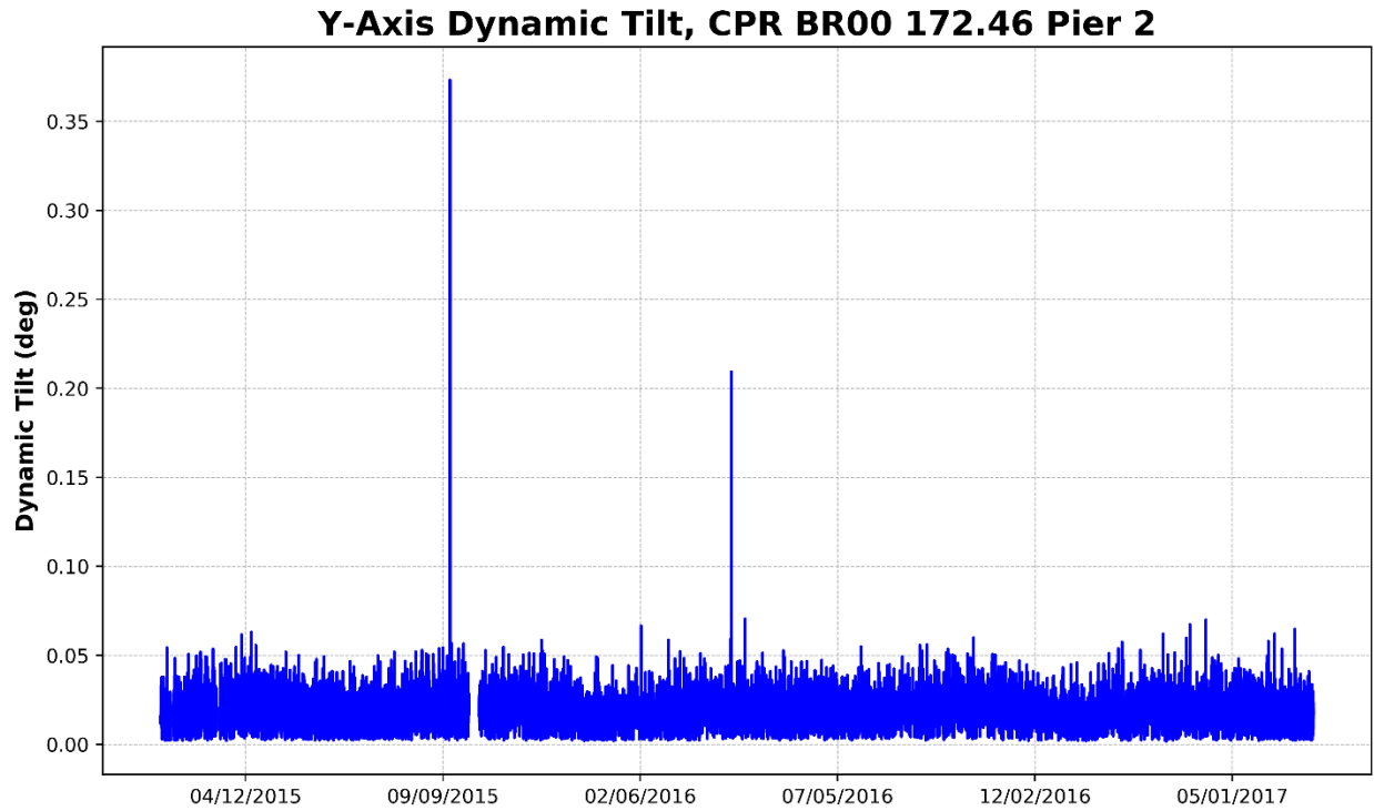
Figure 104 – Pier 2, Y-Axis Dynamic Tilt (Parallel to Track)
