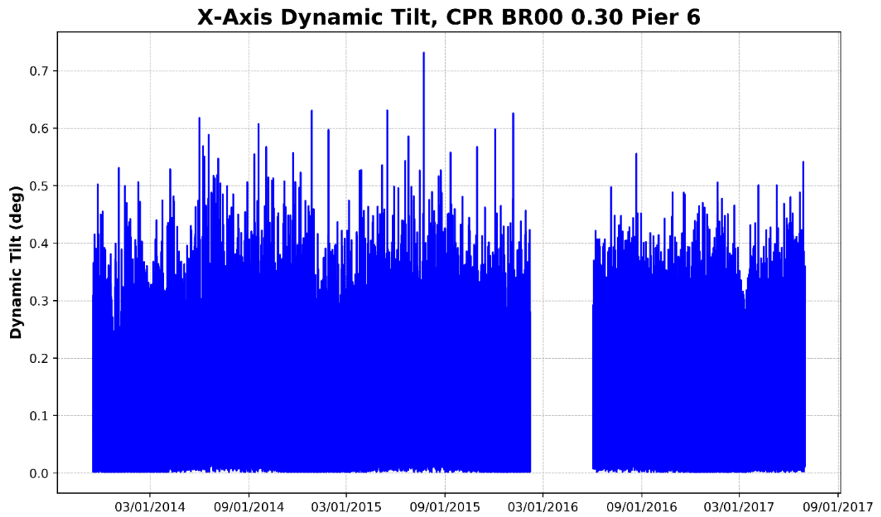
Figure 86 – Pier 6, X-Axis Dynamic Tilt (Parallel to Track)
