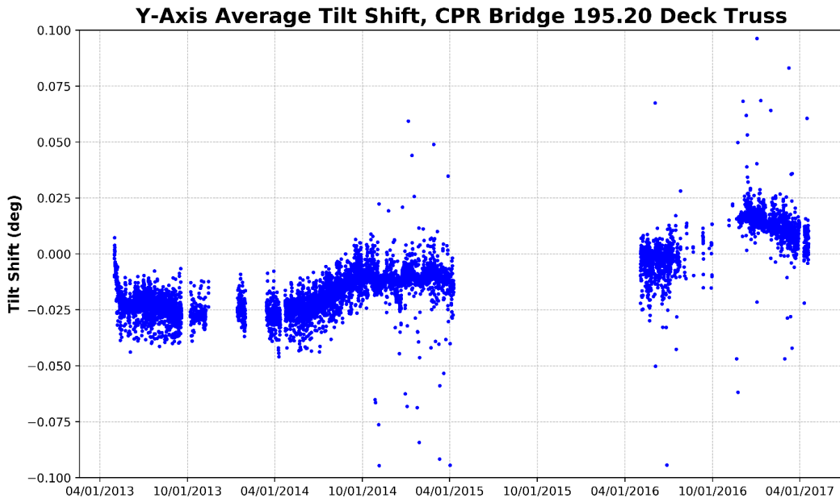
Figure 56 – Deck Truss, Y-Axis Average Tilt (Perpendicular to Track)
