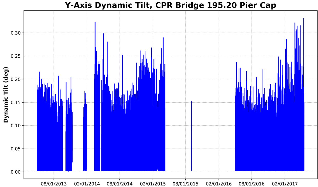
Figure 62 – Pier Cap, Y-Axis Dynamic Tilt (Perpendicular to Track)
