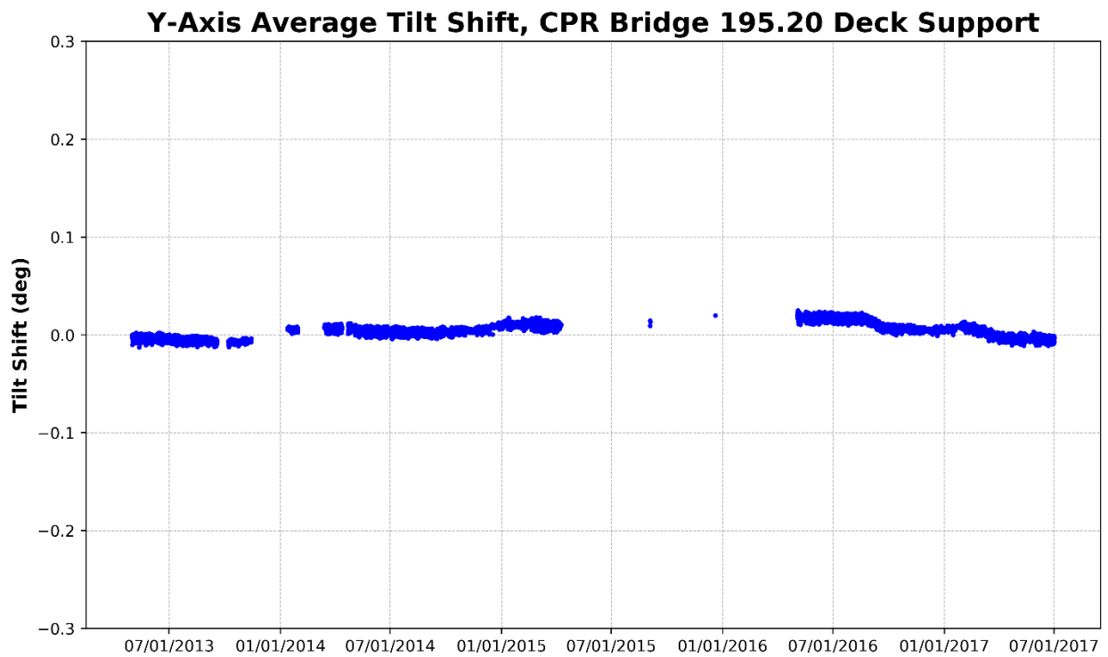
Figure 52 – Deck Support, Y-Axis Average Tilt (Perpendicular to Track)
