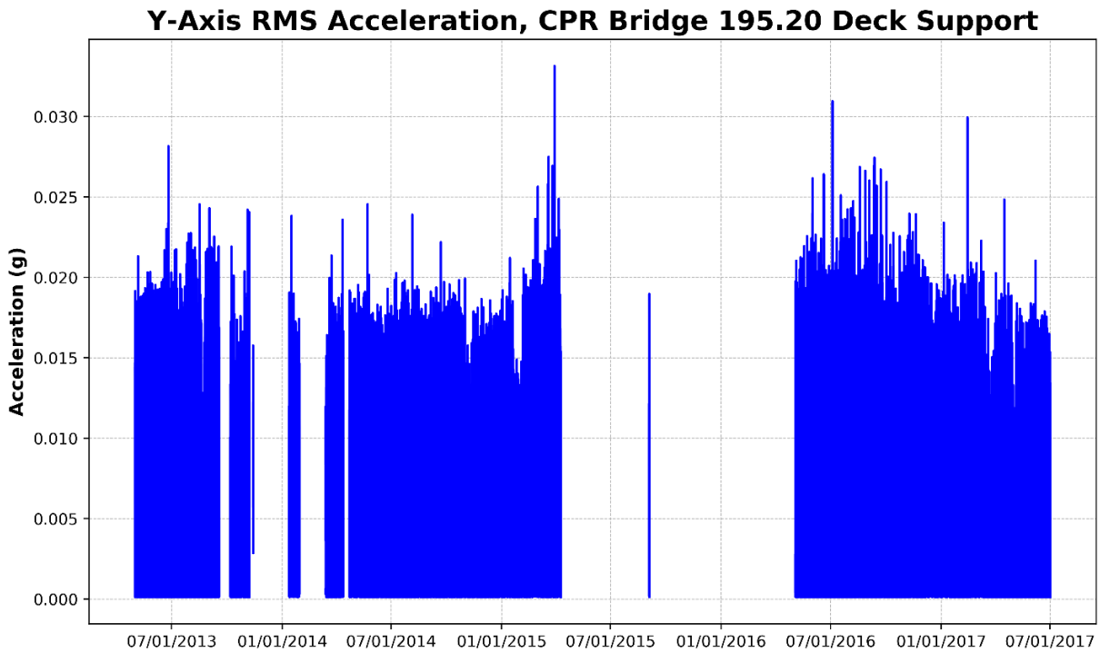
Figure 68 – Deck Support, Y-Axis RMS Acceleration (Perpendicular to Track)
