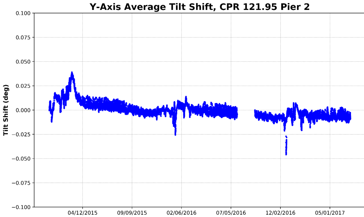
Figure 117 – Pier 2, Y-Axis Average Tilt
