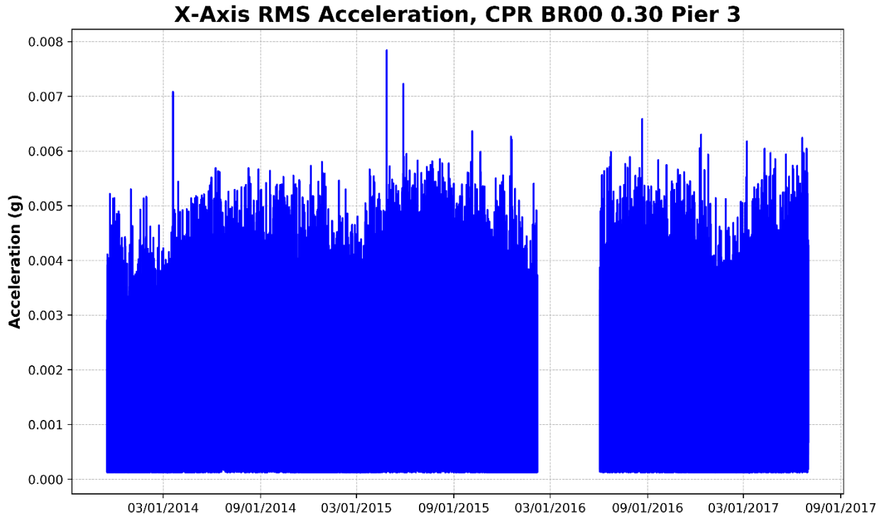
Figure 88 – Pier 3, X-Axis RMS Acceleration (Parallel to Track)
