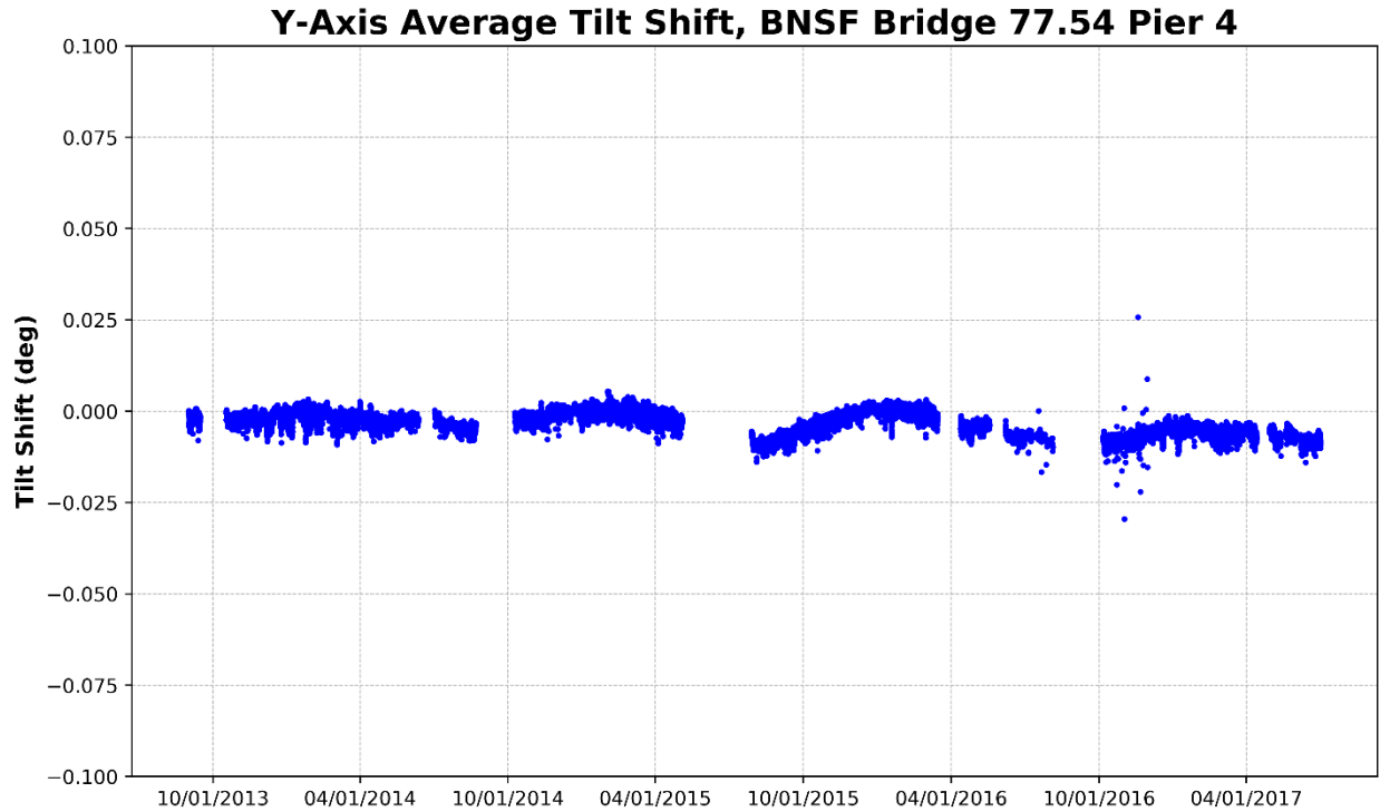
Figure 18 – Pier 4, Y-Axis Average Tilt (Perpendicular to Track)
