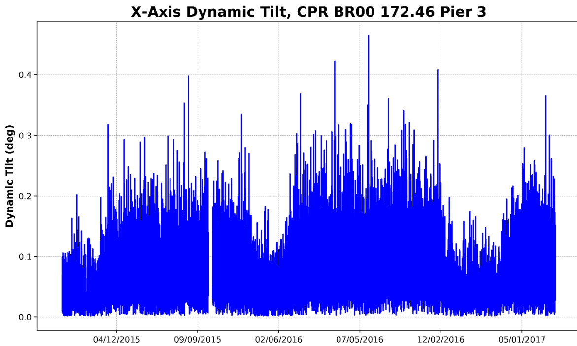
Figure 105 – Pier 3, X-Axis Dynamic Tilt (Perpendicular to Track)
