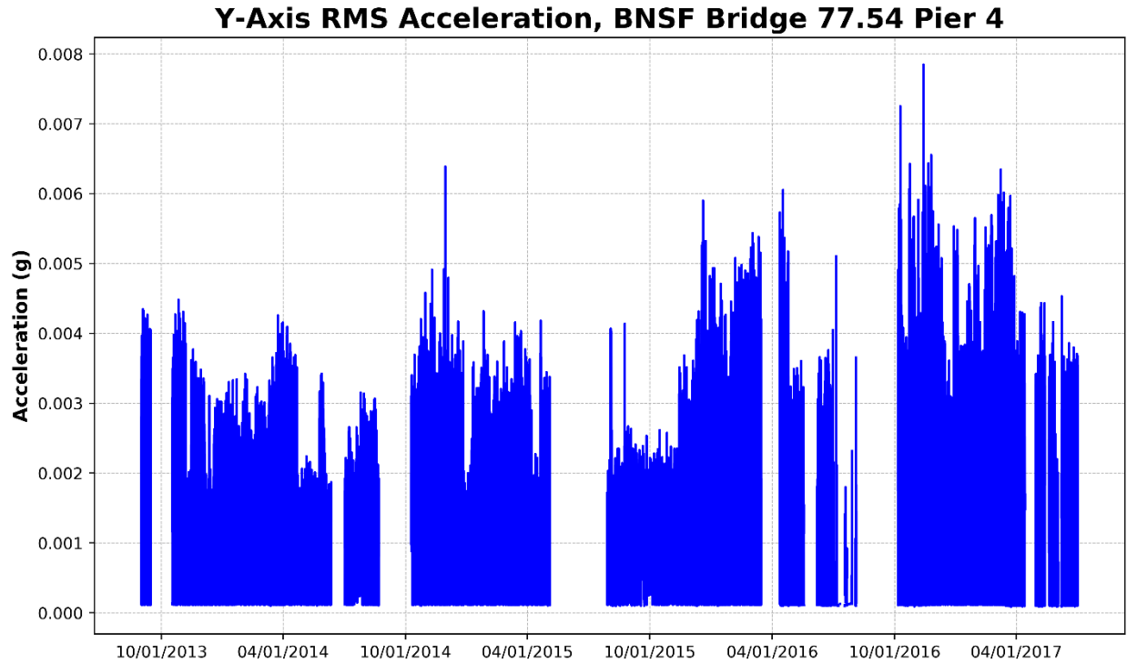
Figure 34 – Pier 4, Y-Axis RMS Acceleration (Perpendicular to Track)
