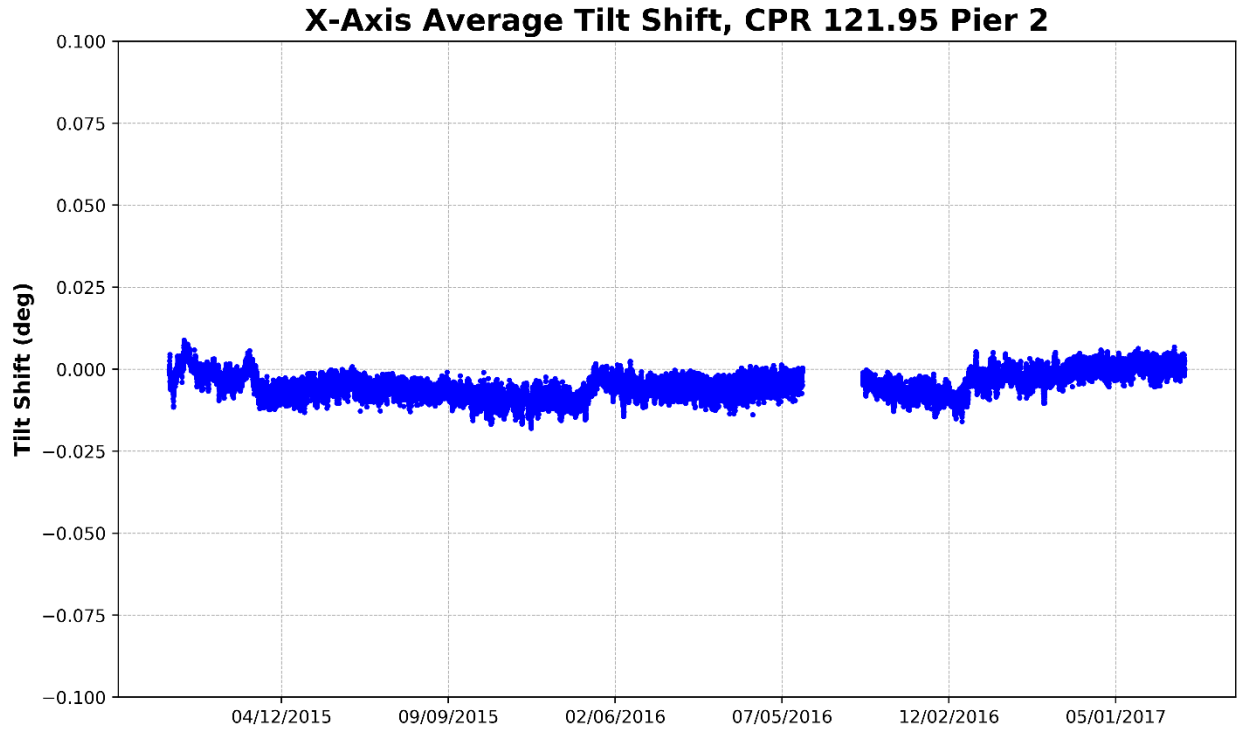
Figure 116 – Pier 2, X-Axis Average Tilt
