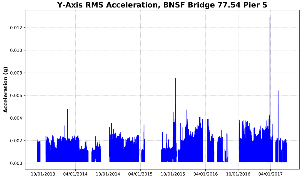
Figure 36 – Pier 5, Y-Axis RMS Acceleration (Perpendicular to Track)
