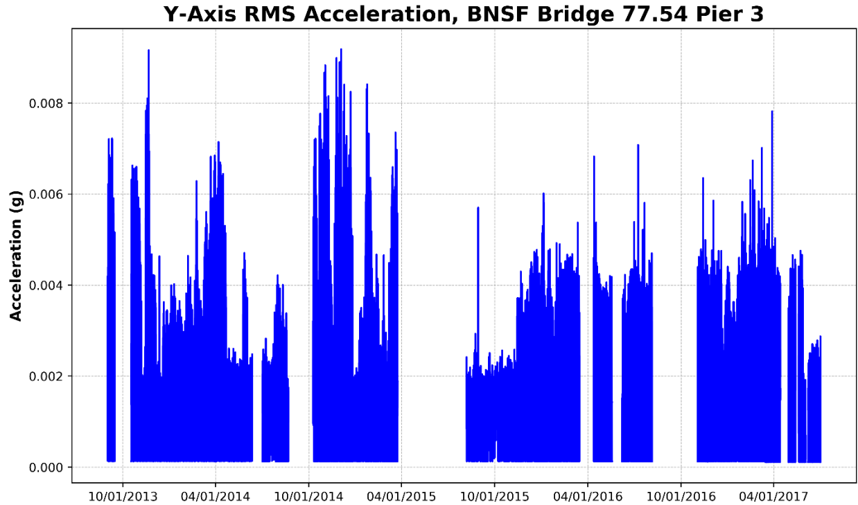
Figure 32 – Pier 3, Y-Axis RMS Acceleration (Perpendicular to Track)
