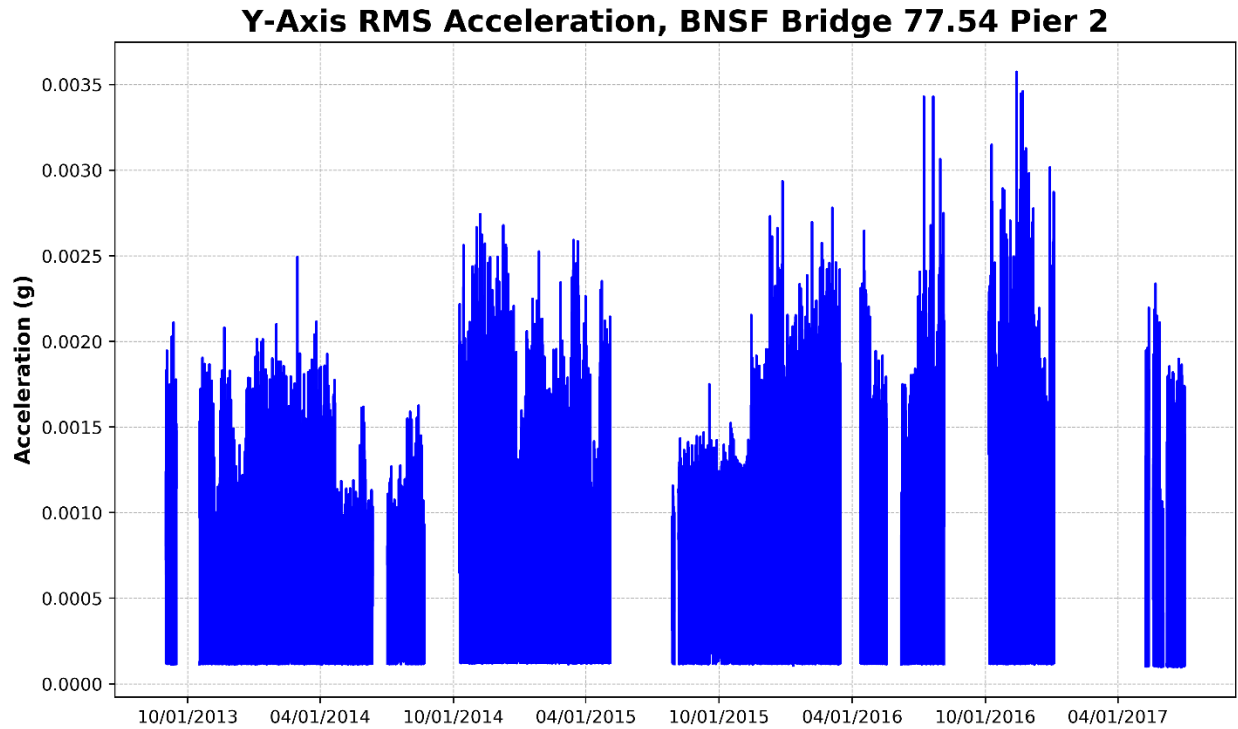
Figure 30 – Pier 2, Y-Axis RMS Acceleration (Perpendicular to Track)
