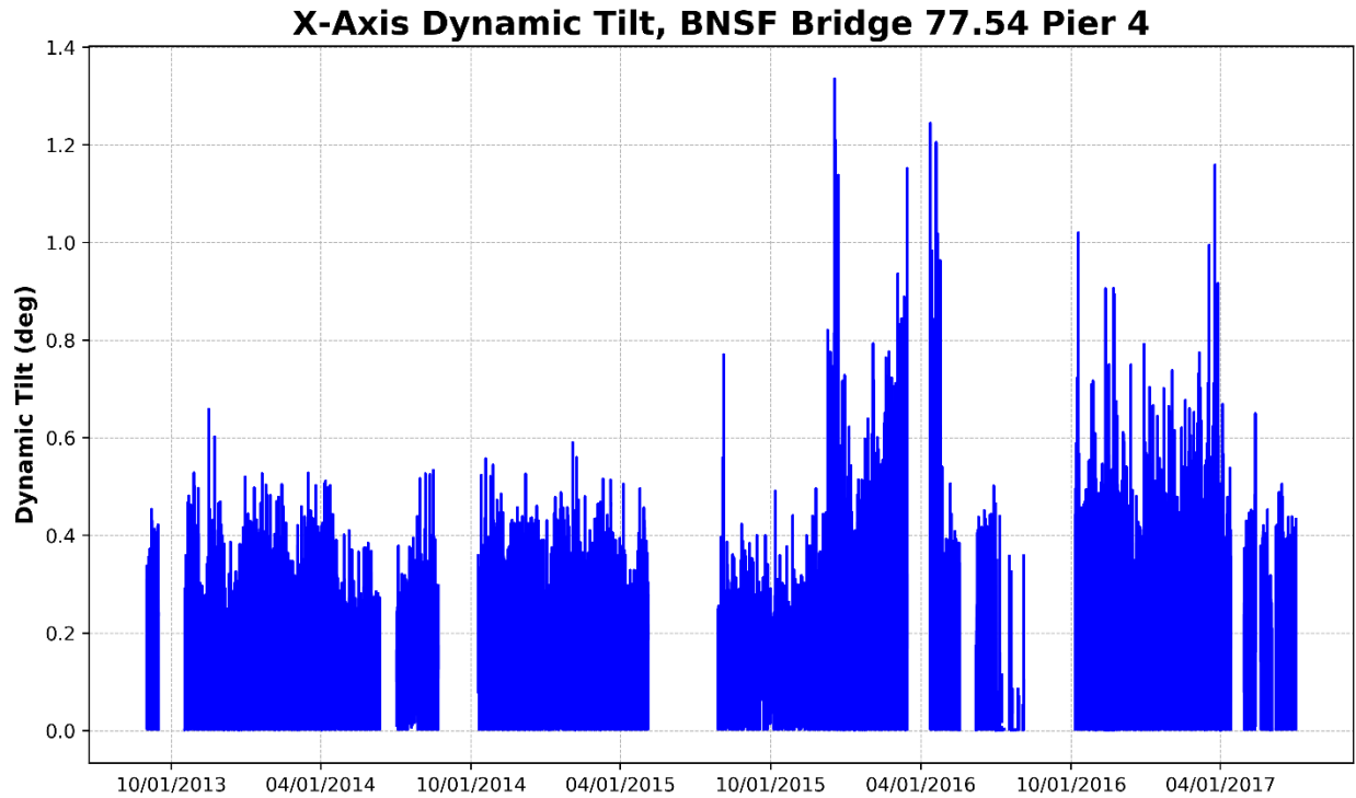
Figure 25 – Pier 4, X-Axis Dynamic Tilt (Parallel to Track)
