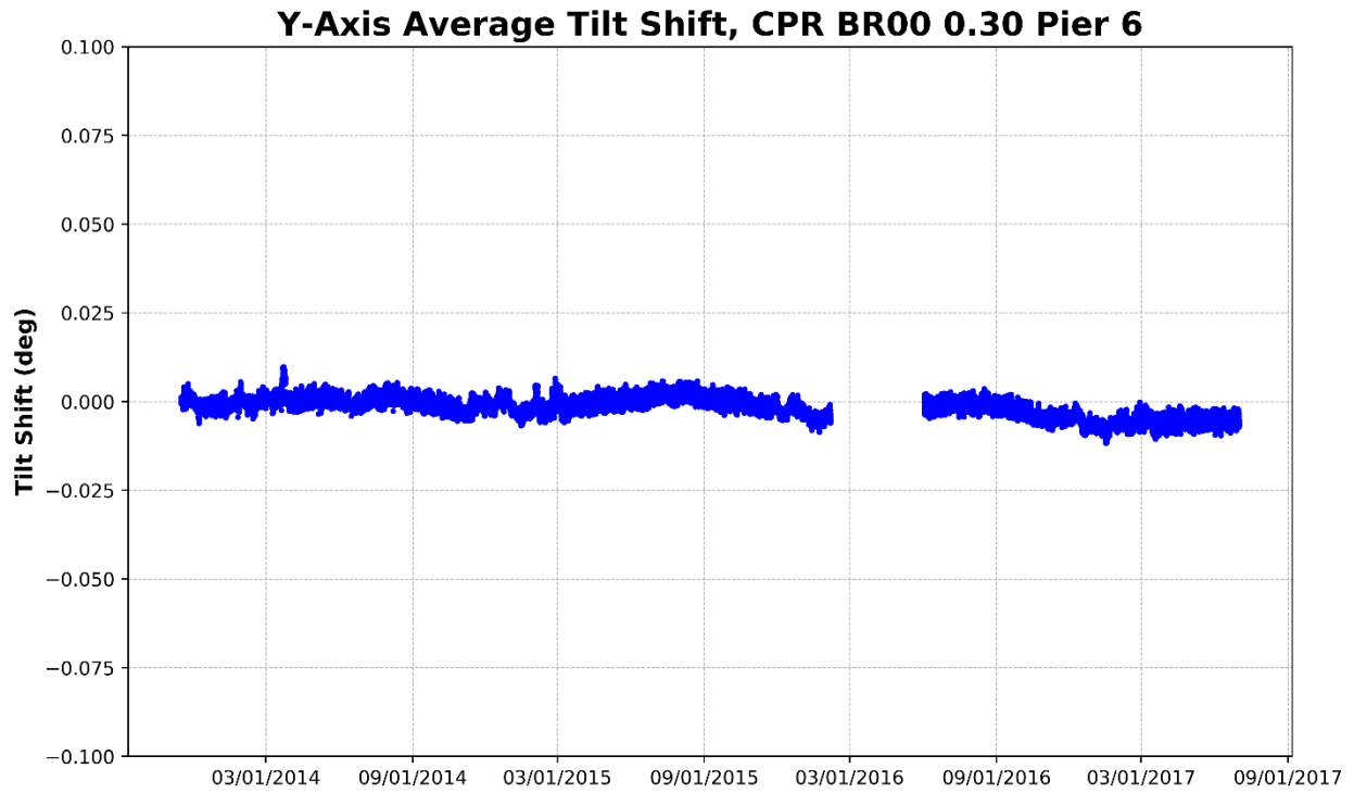
Figure 81 – Pier 6, Y-Axis Average Tilt (Perpendicular to Track)
