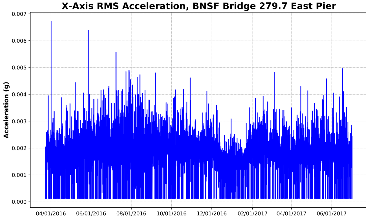
Figure 46 – East Pier, X-Axis RMS Acceleration (Perpendicular to Track)
