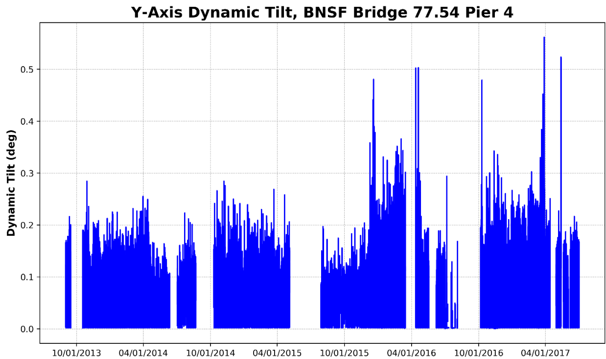
Figure 26 – Pier 4, Y-Axis Dynamic Tilt (Perpendicular to Track)
