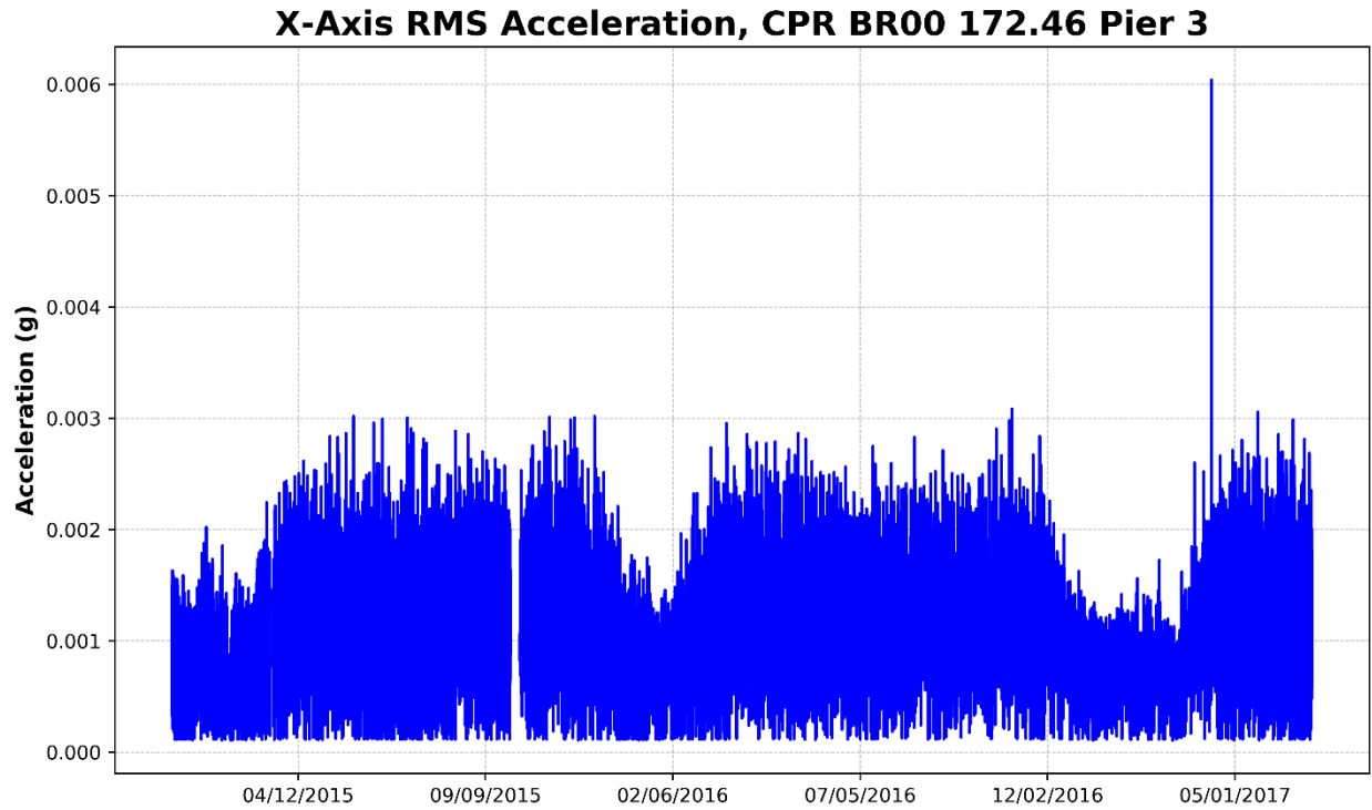
Figure 111 – Pier 3, X-Axis RMS Acceleration (Perpendicular to Track)
