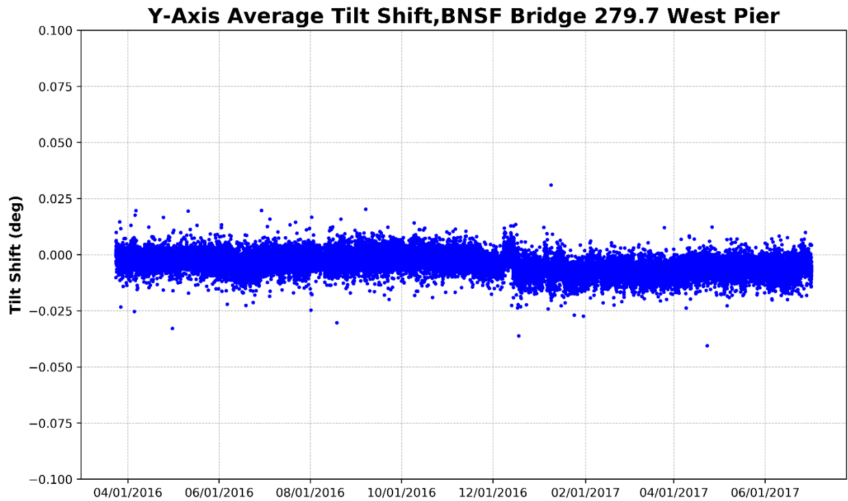
Figure 41 – West Pier, Y-Axis Average Tilt (Parallel to Track)
