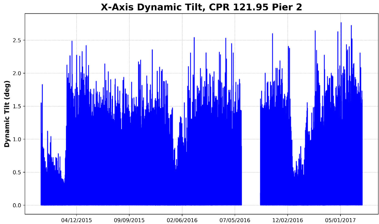
Figure 124 – Pier 2, X-Axis Dynamic Tilt
