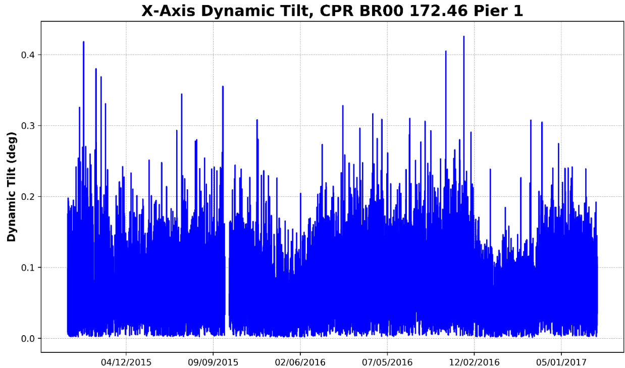
Figure 101 – Pier 1, X-Axis Dynamic Tilt (Perpendicular to Track)
