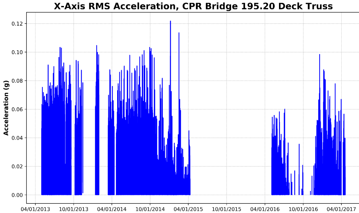
Figure 71 – Deck Truss, X-Axis RMS Acceleration (Parallel to Track)
