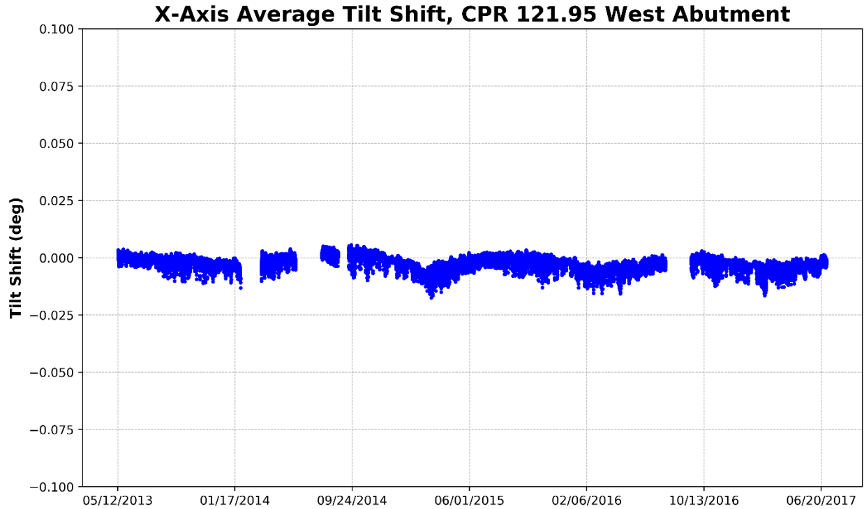
Figure 118 – West Abutment, X-Axis Average Tilt (Perpendicular to Track)
