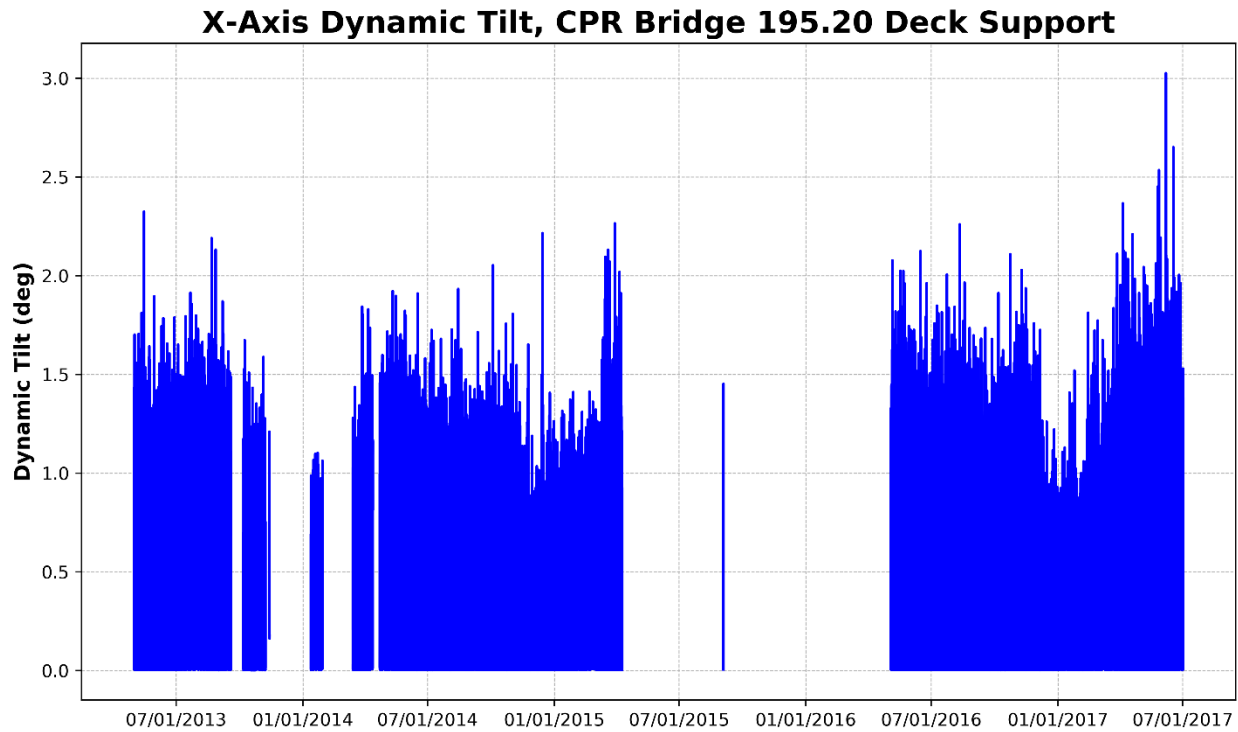
Figure 59 – Deck Support, X-Axis Dynamic Tilt (Parallel to Track)
