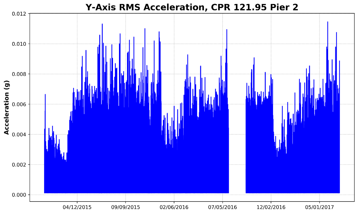
Figure 133 – Pier 2, Y-Axis RMS Acceleration
