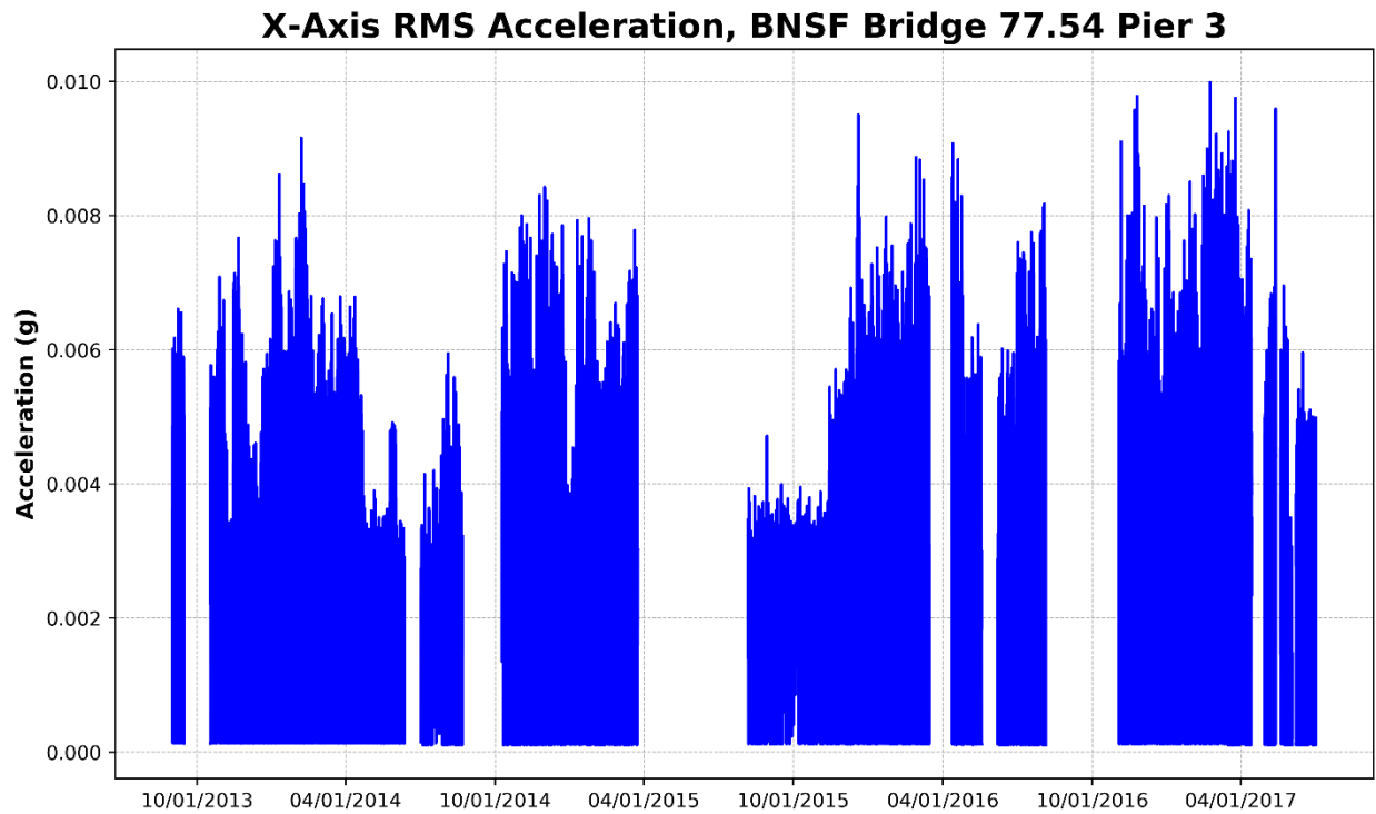
Figure 31 – Pier 3, X-Axis RMS Acceleration (Parallel to Track)
