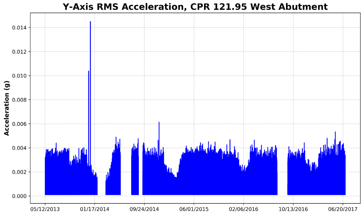
Figure 135 – West Abutment, Y-Axis RMS Acceleration (Parallel to Track)
