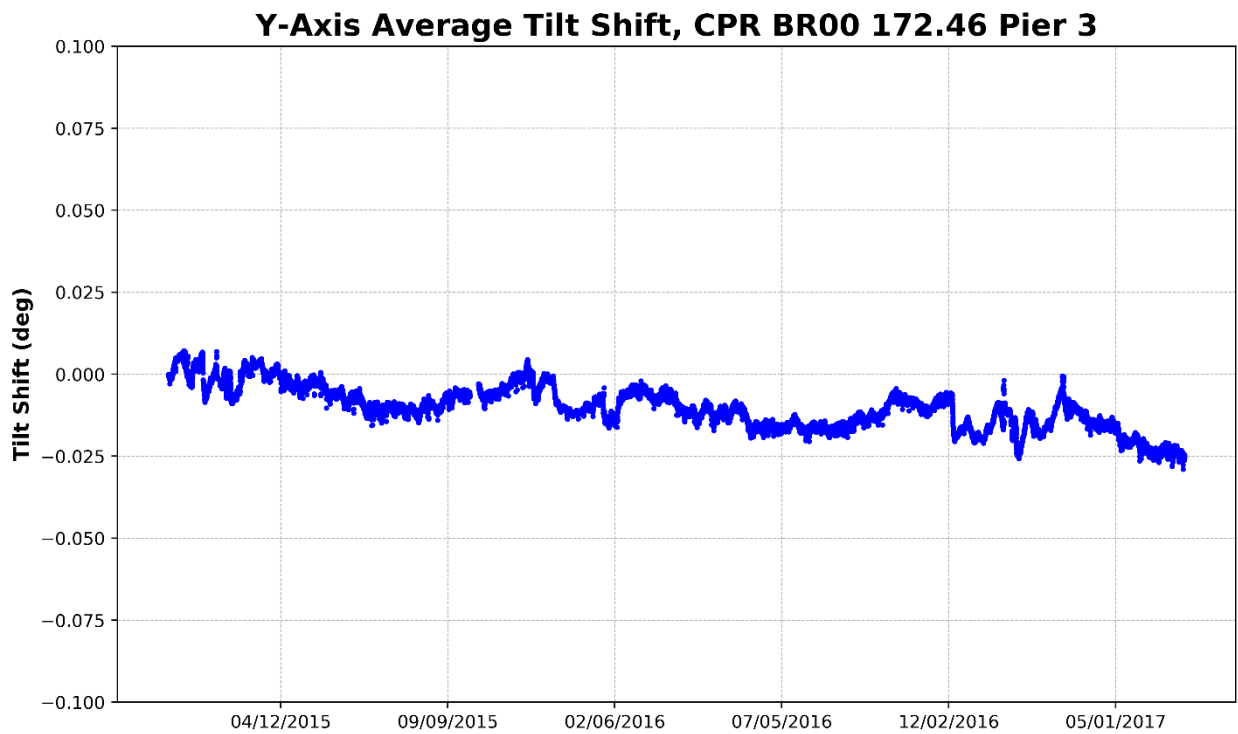
Figure 100 – Pier 3, Y-Axis Average Tilt (Parallel to Track)
