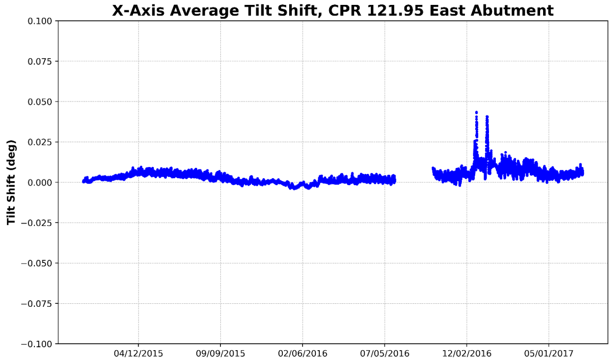
Figure 120 – East Abutment, X-Axis Average Tilt (Perpendicular to Track)
