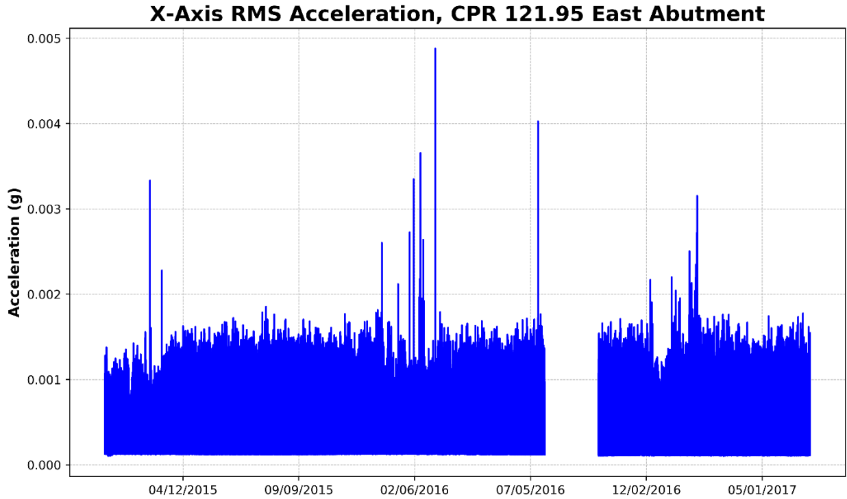
Figure 136 – East Abutment, X-Axis RMS Acceleration (Perpendicular to Track)
