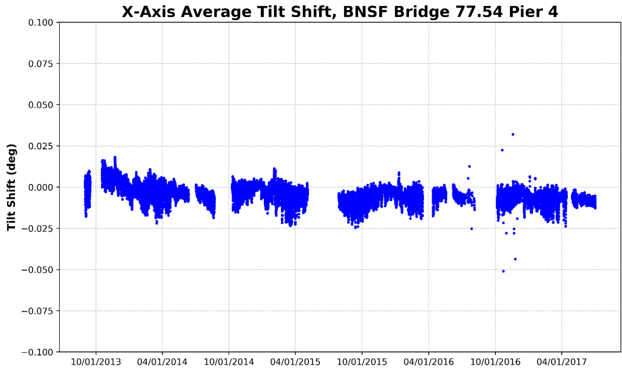
Figure 17 – Pier 4, X-Axis Average Tilt (Parallel to Track)
