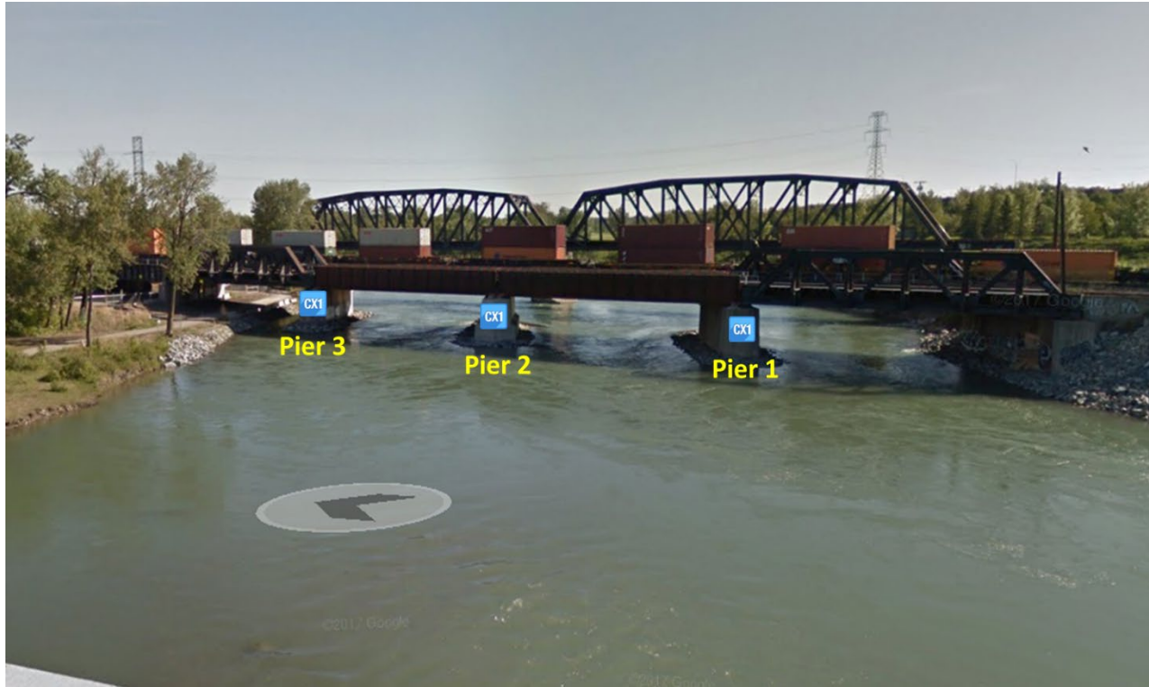
Figure 94 – Sensor Locations on CPR Calgary Bridge 172.46
