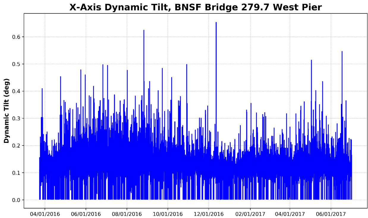
Figure 44 – West Pier, X-Axis Dynamic Tilt (Perpendicular to Track)
