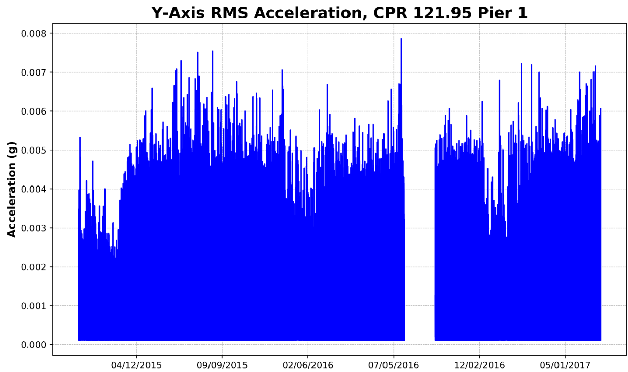
Figure 131 – Pier 1, Y-Axis RMS Acceleration
