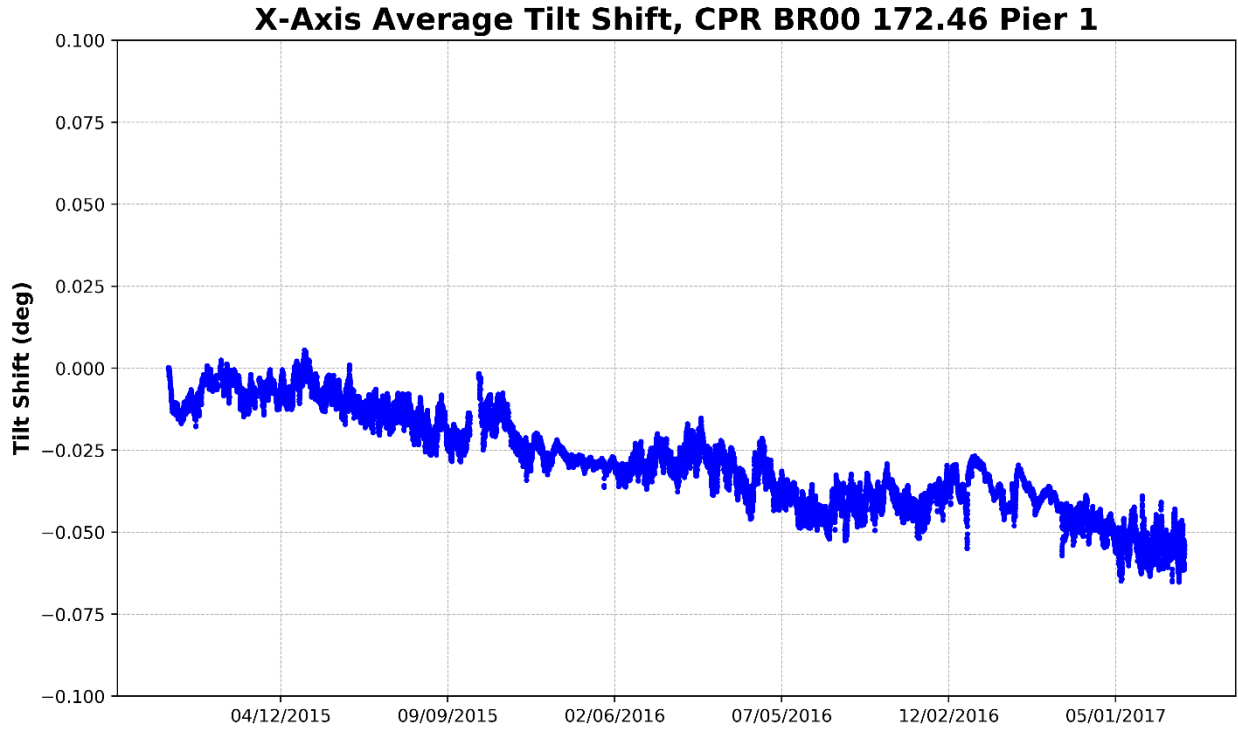
Figure 95 – Pier 1, X-Axis Average Tilt (Perpendicular to Track)
