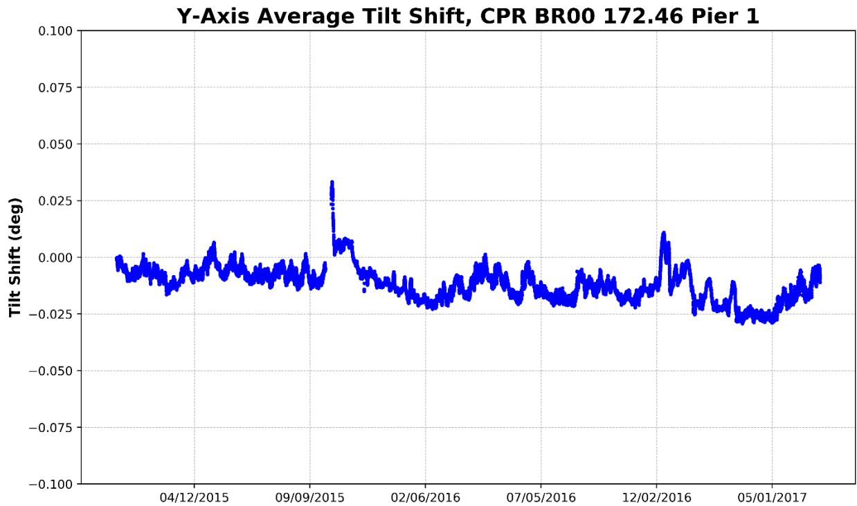
Figure 96 – Pier 1, Y-Axis Average Tilt (Parallel to Track)
