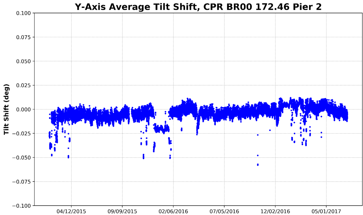
Figure 98 – Pier 2, Y-Axis Average Tilt (Parallel to Track)
