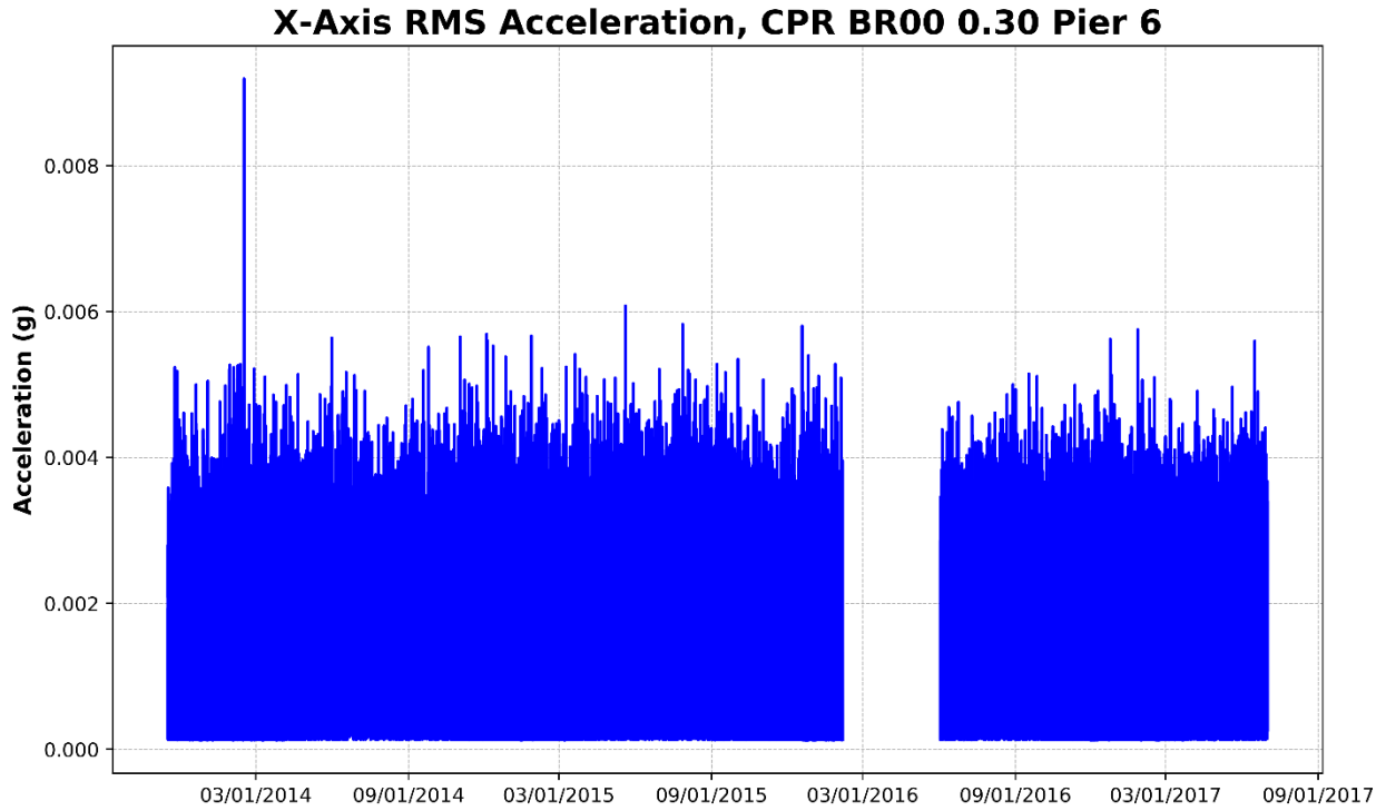
Figure 92 – Pier 6, X-Axis RMS Acceleration (Parallel to Track)
