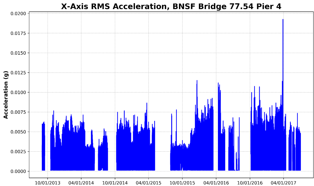
Figure 33 – Pier 4, X-Axis RMS Acceleration (Parallel to Track)
