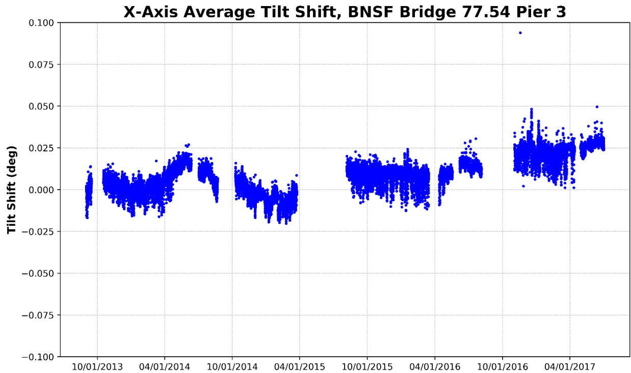
Figure 15 – Pier 3, X-Axis Average Tilt (Parallel to Track)
