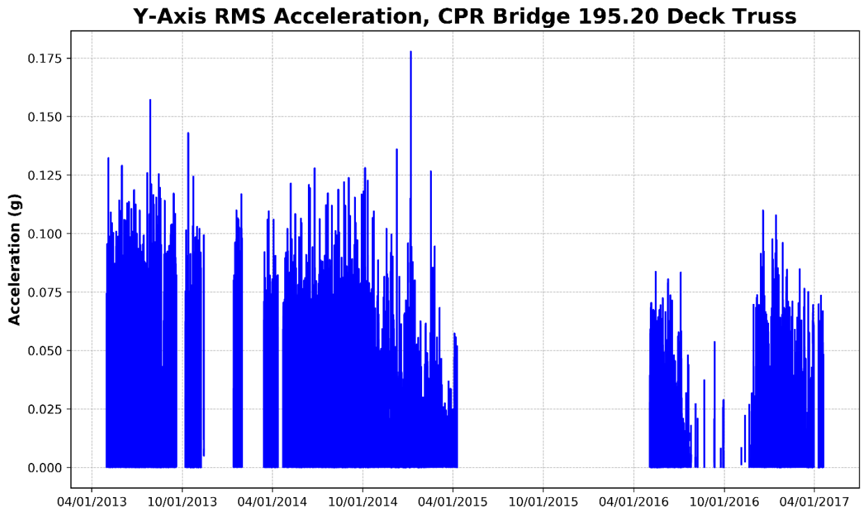
Figure 72 – Deck Truss, Y-Axis RMS Acceleration (Perpendicular to Track)
