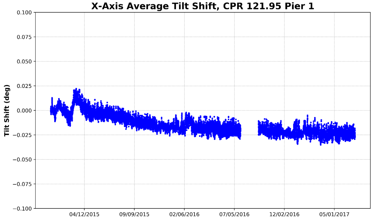
Figure 114 – Pier 1, X-Axis Average Tilt
