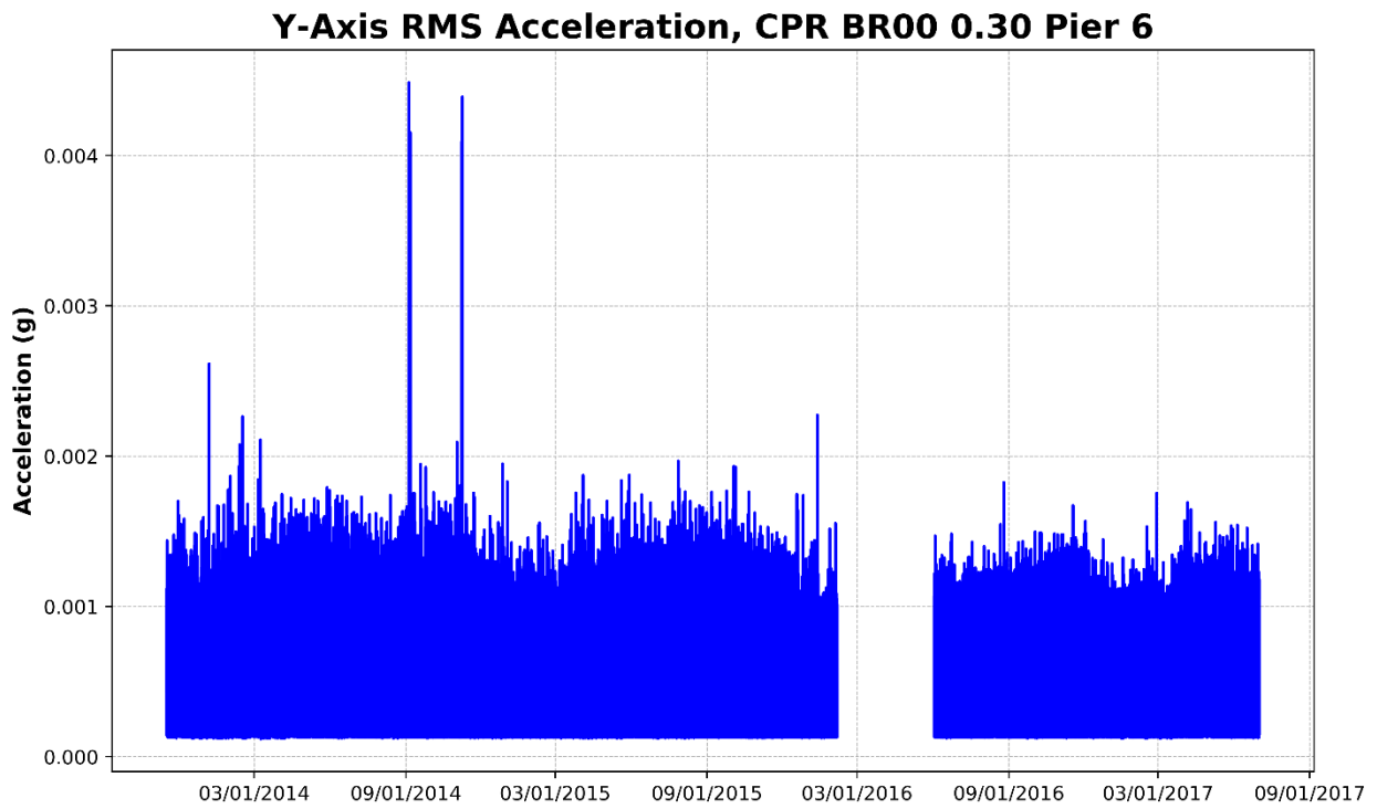
Figure 93 – Pier 6, Y-Axis RMS Acceleration (Perpendicular to Track)
