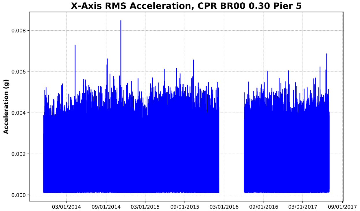
Figure 90 – Pier 5, X-Axis RMS Acceleration (Parallel to Track)
