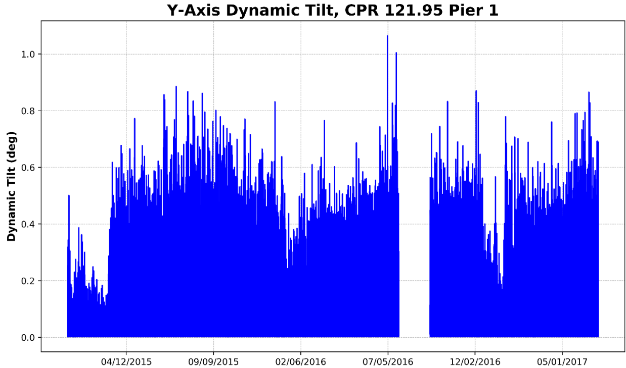
Figure 123 – Pier 1, Y-Axis Dynamic Tilt
