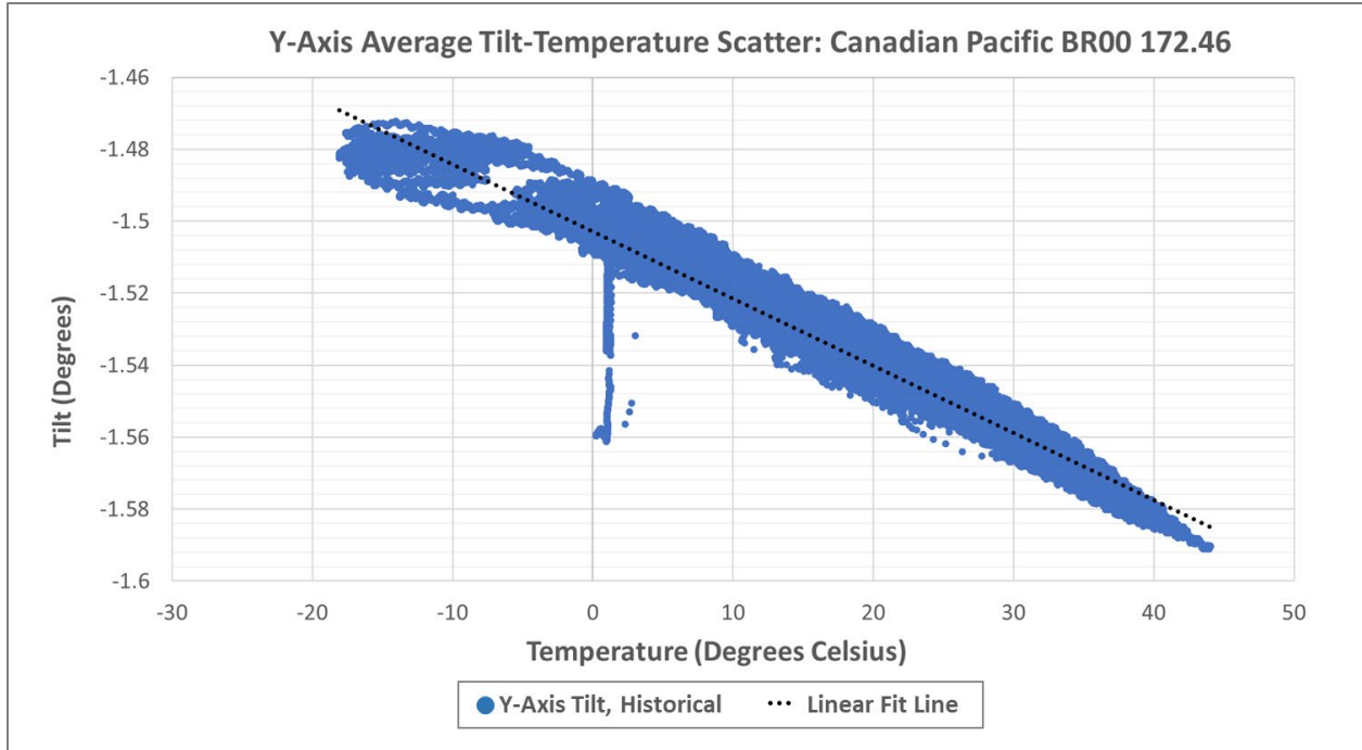
Figure 5 – Example of Tilt-Temperature Relationship, Canadian Pacific BR00 172.46 West Pier
