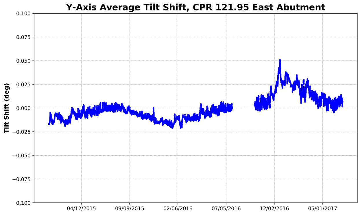
Figure 121 – East Abutment, Y-Axis Average Tilt (Parallel to Track)
