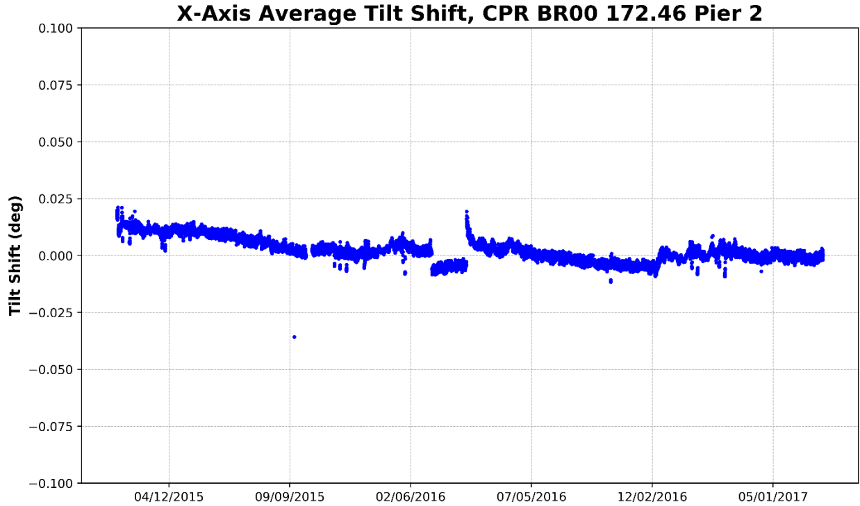
Figure 97 – Pier 2, X-Axis Average Tilt (Perpendicular to Track)
