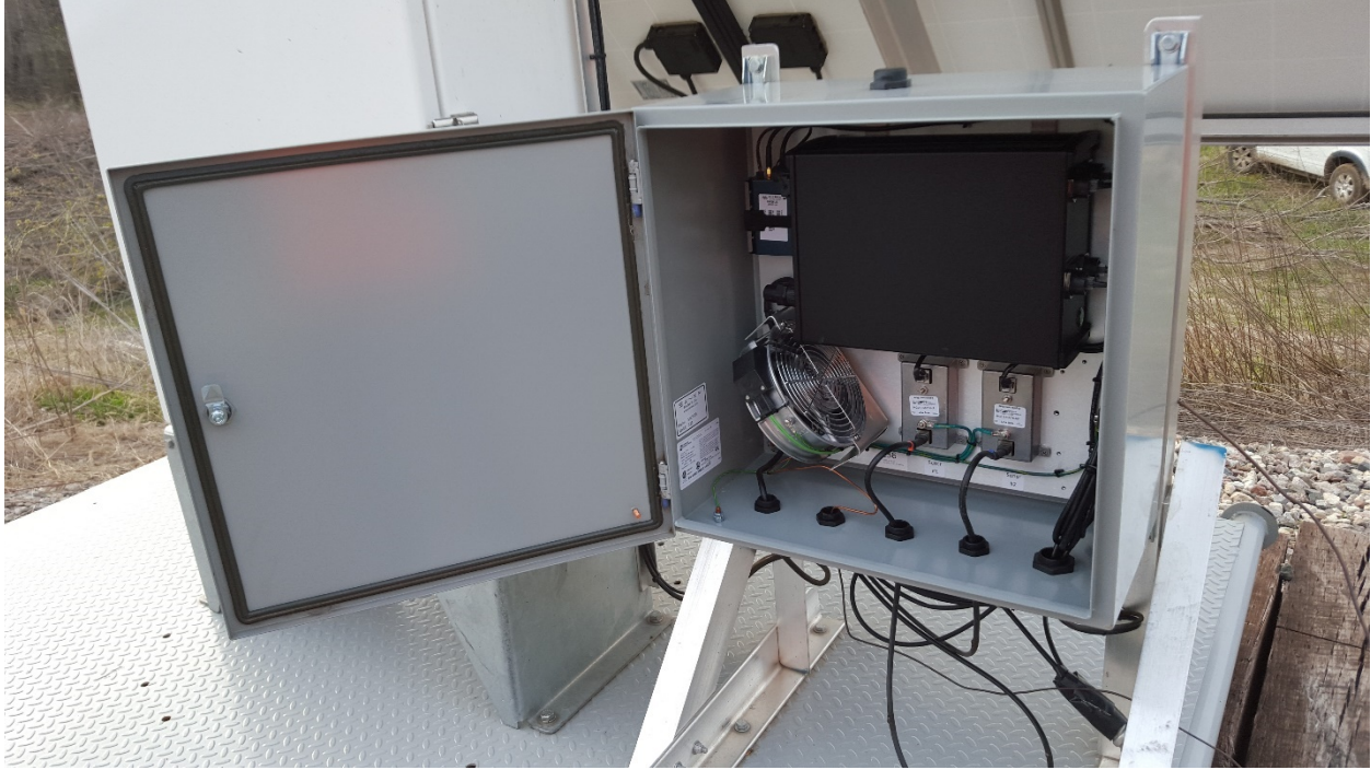
Figure 3 – SENSnet Installed Inside Electrical Enclosure
