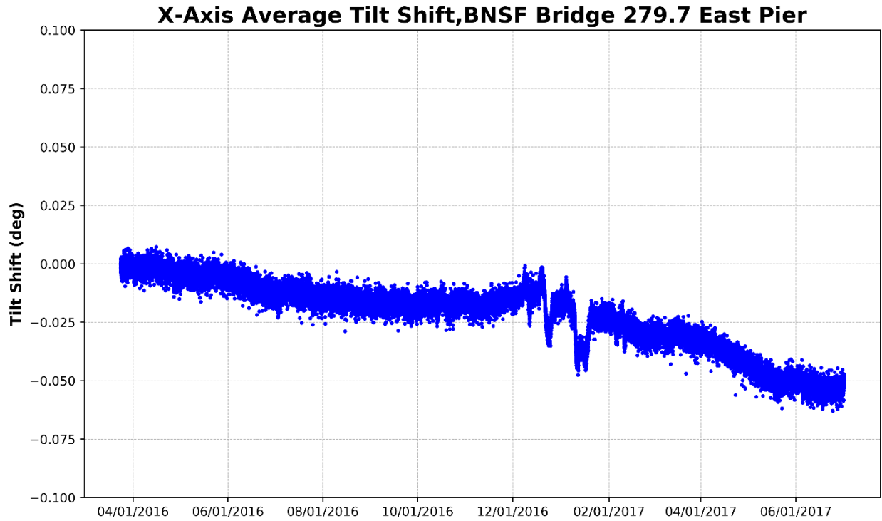
Figure 38 – East Pier, X-Axis Average Tilt (Perpendicular to Track)
