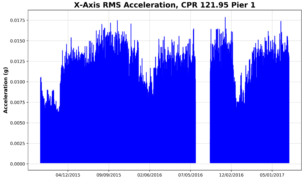
Figure 130 – Pier 1, X-Axis RMS Acceleration
