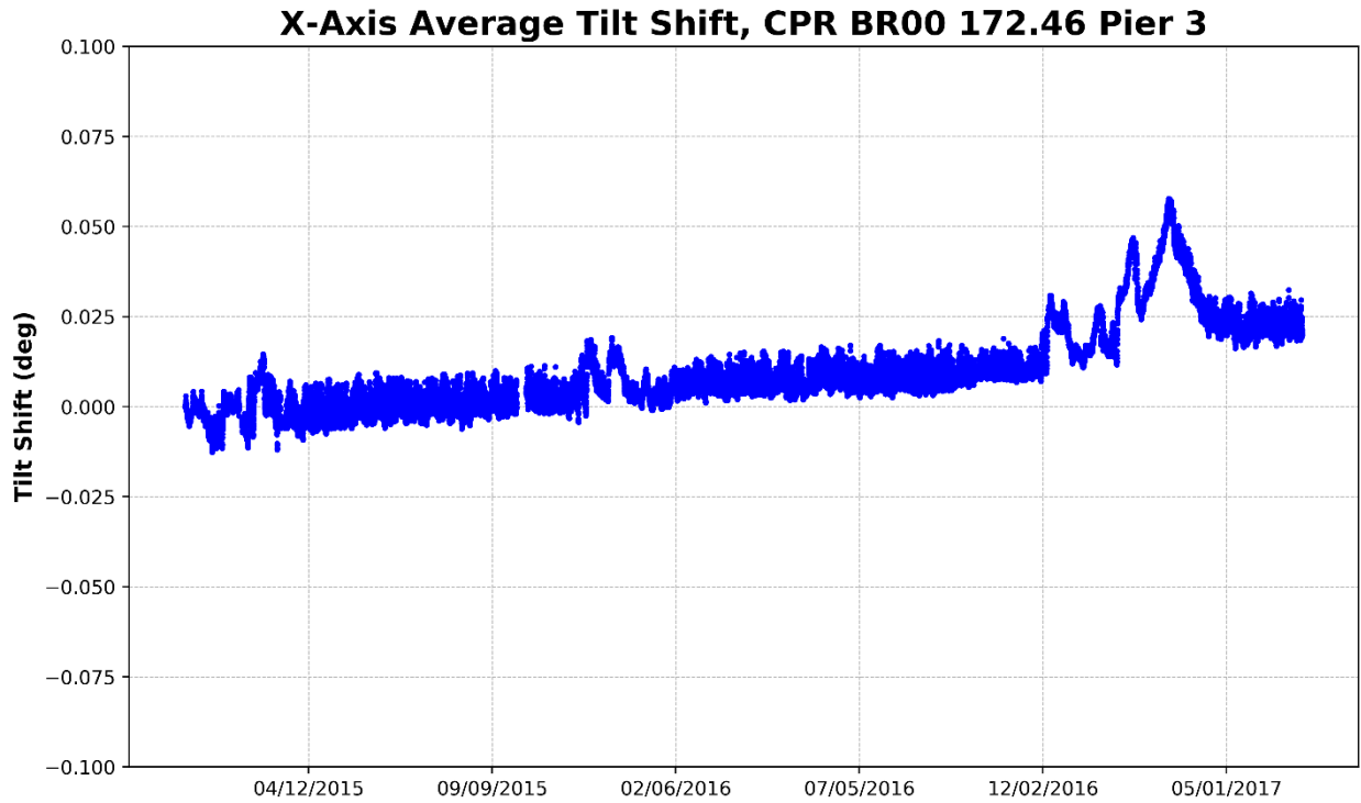
Figure 99 – Pier 3, X-Axis Average Tilt (Perpendicular to Track)
