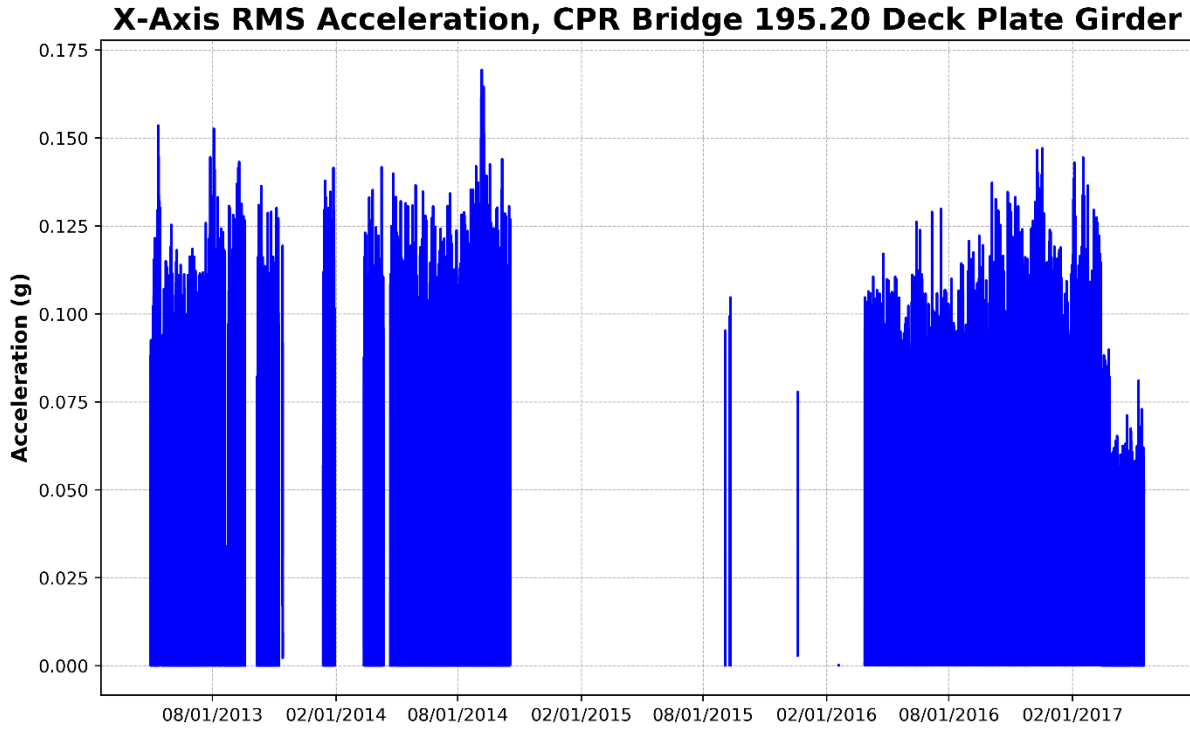
Figure 73 – Deck Plate Girder, X-Axis RMS Acceleration (Parallel to Track)
