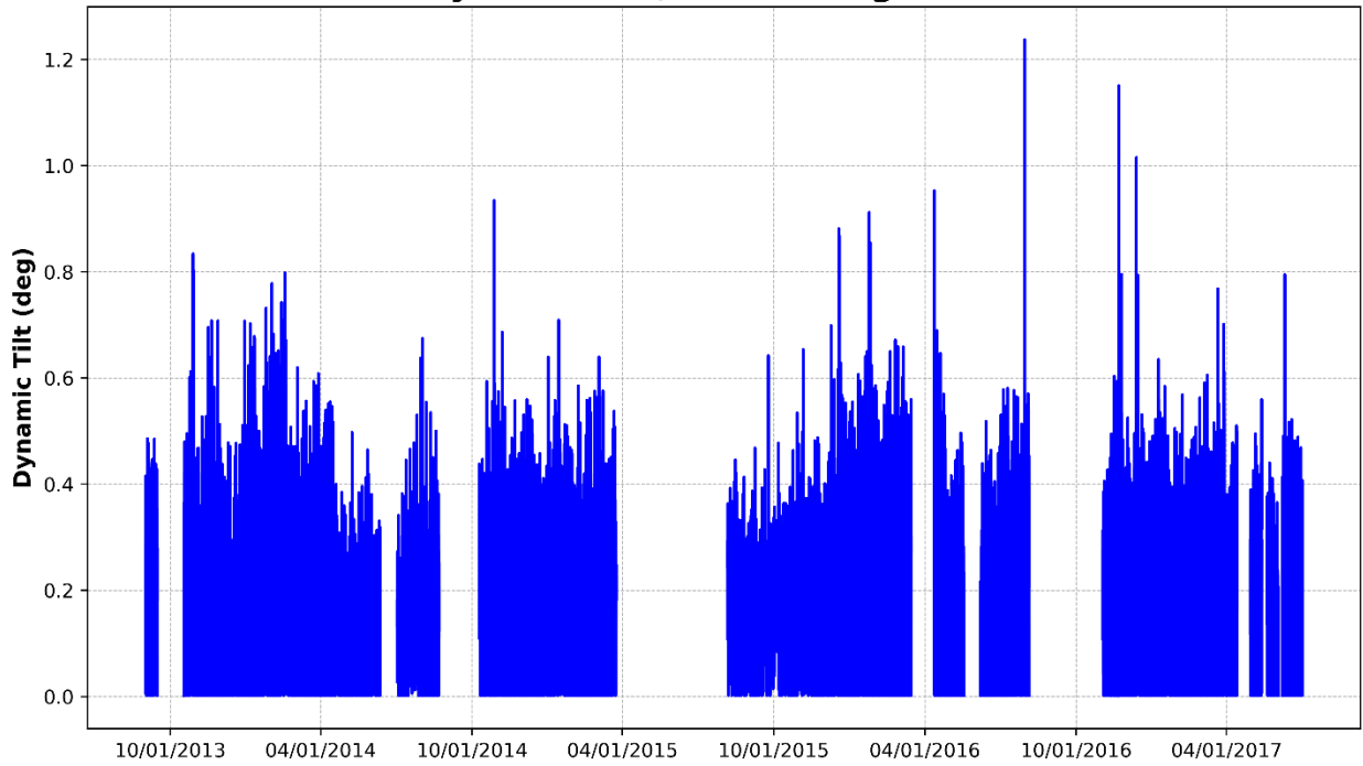
X-Axis Dynamic Tilt, BNSF Bridge 77.54 Pier 3
