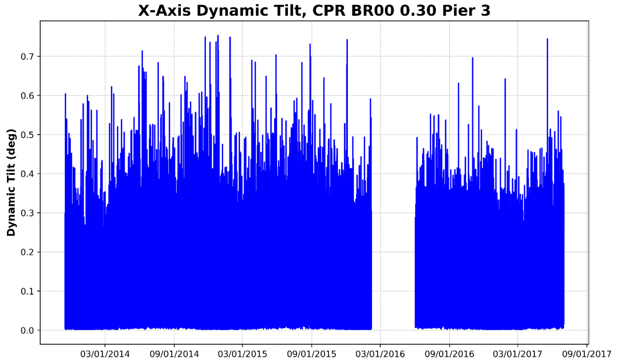
Figure 82 – Pier 3, X-Axis Dynamic Tilt (Parallel to Track)
