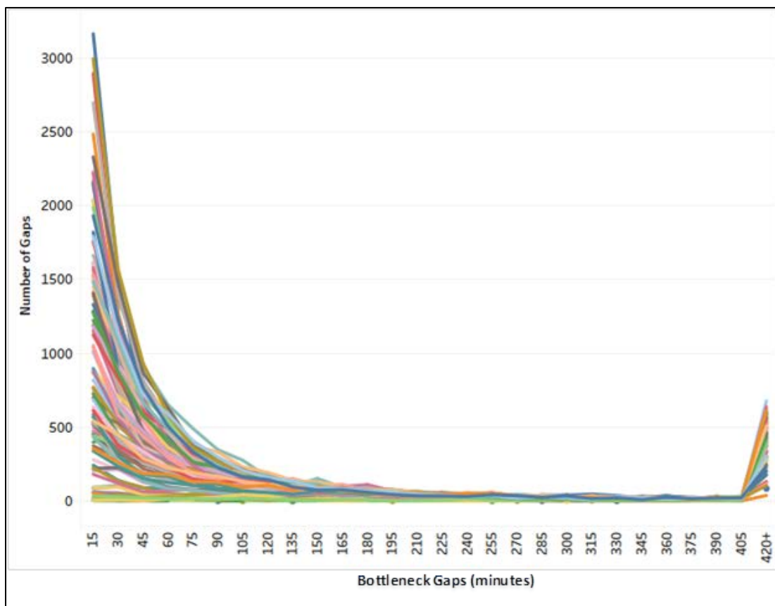
Figure 22. Frequency of Bottleneck Gaps by Intersection. Each color line is one intersection.
