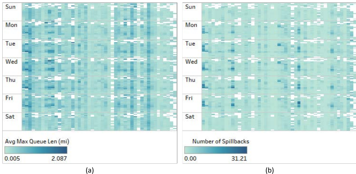
Figure 24. Example of Trends for Day of Week and Time of Day: (a) intersection bottlenecks by average maximum queue length (miles); (b) approach bottlenecks by number of spillbacks. The Y-axis on the heatmaps shows the day of week and time of day (12 A.M. to 11 P.M. top to bottom) within each day of week; the X-axis shows individual intersections in (a) and intersection approaches in (b) sorted by ID number.
