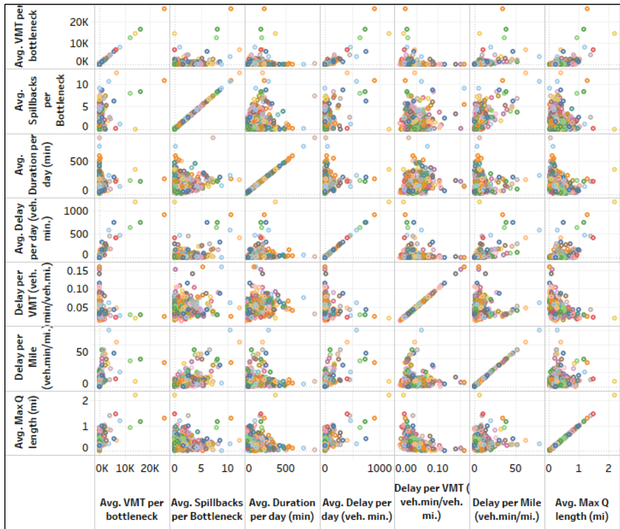
Figure 28. Matrix of Scatter Plots Across Select Performance Measures. Each color represents a different intersection. VMT = vehicle miles traveled; min = minutes, mi = miles; veh.min = vehicle-minutes; veh.mi = vehicle-miles; Max Q = average maximum queue length.
