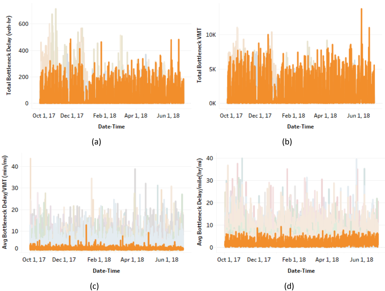
Figure 23. Example of Trends of Performance Measures by Date and Hour of Day for One Intersection in Fairfax County (Intersection 263952): (a) total intersection bottleneck delay (vehicle-hours); (b) total intersection bottleneck vehicle miles traveled (VMT); (c) average bottleneck delay per VMT (minutes/mile-traveled); (d) average bottleneck delay per mile of approach (hours/mile)
