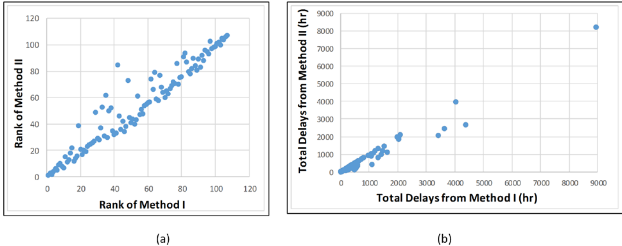
Figure 20. Comparison of Results From Methods I and II for Signalized Intersections: (a) ranks by delays; (b) total delays
