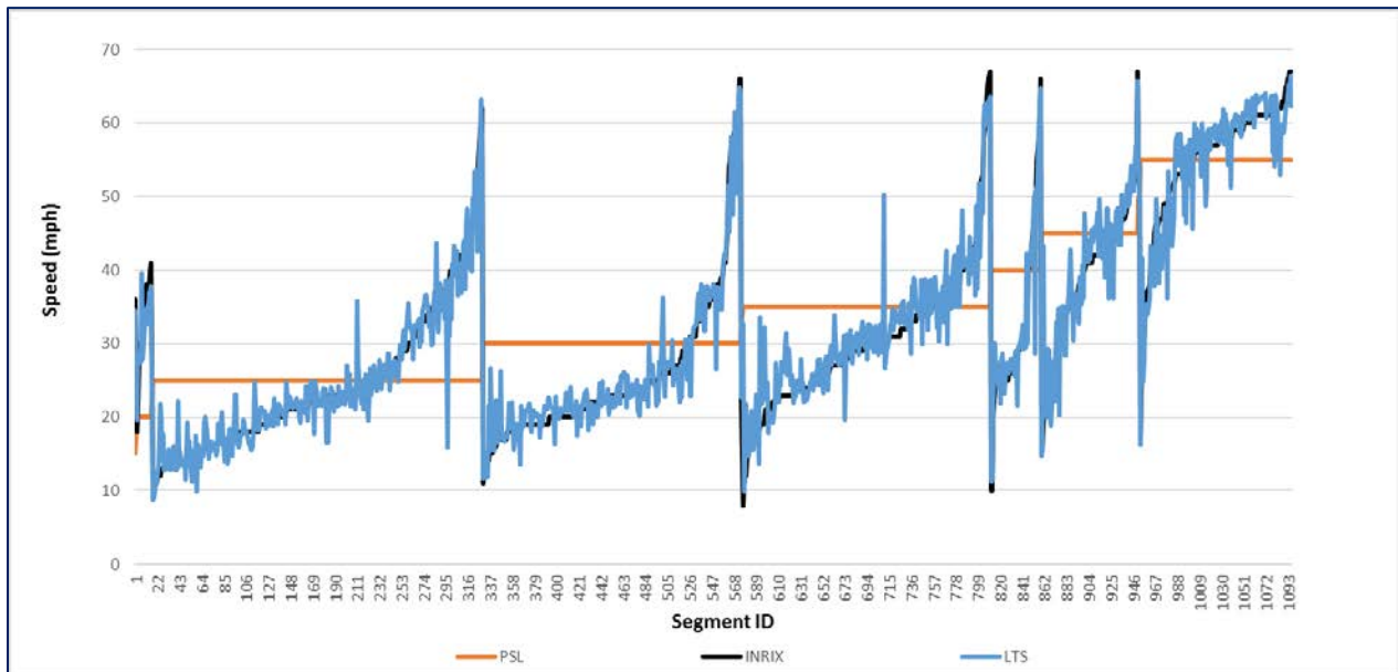
Figure 18. Posted Speed Limit (PSL), INRIX Reference Speed (INRIX), and Light Traffic Speed (LTS) for Studied Segments
