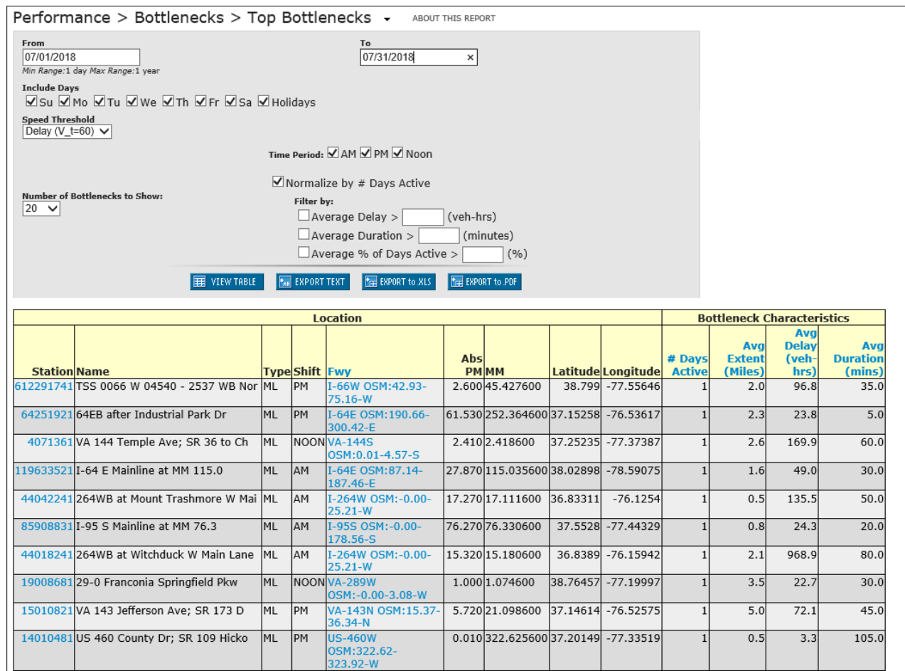
Figure 5. iPeMS Bottleneck Ranking Table. The analysis period and other options are shown at the top. The results list at the bottom provides the locations and characteristics of the top-ranked bottlenecks.
