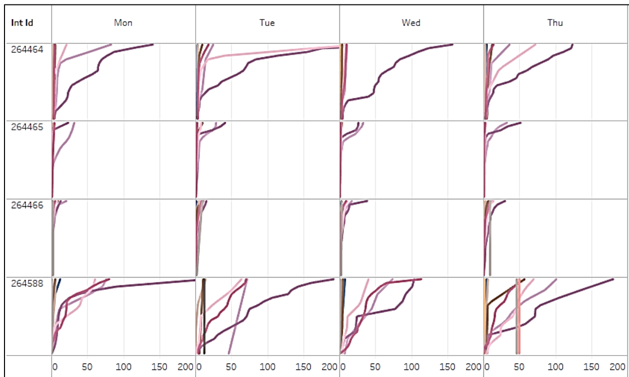
Figure 12. Snippet of Vehicle-Hours of Delay Cumulative Distribution Function (CDF). The CDFs illustrate the variability of bottleneck intensity across days, time of day, and intersections; the line color indicates the hour of day.
