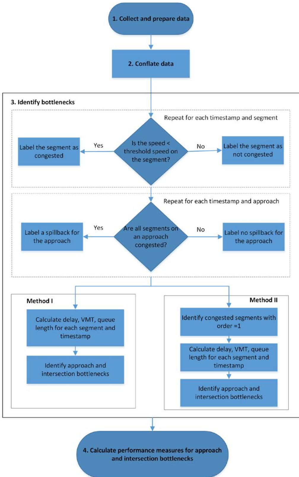
Figure 8. Overview of Bottleneck Identification Methodology
