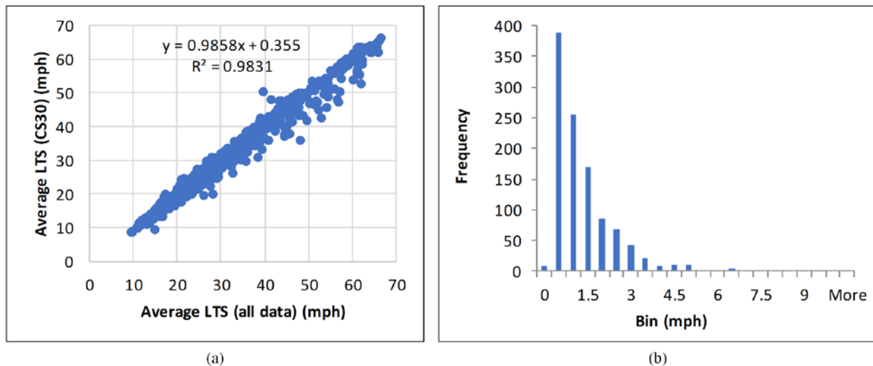
Figure 19. Comparison of Light Traffic Speed (LTS) Calculated From Score 30 (CS30) Data and All Data Using (a) Scatter Plots and (b) Histogram of Absolute Differences
