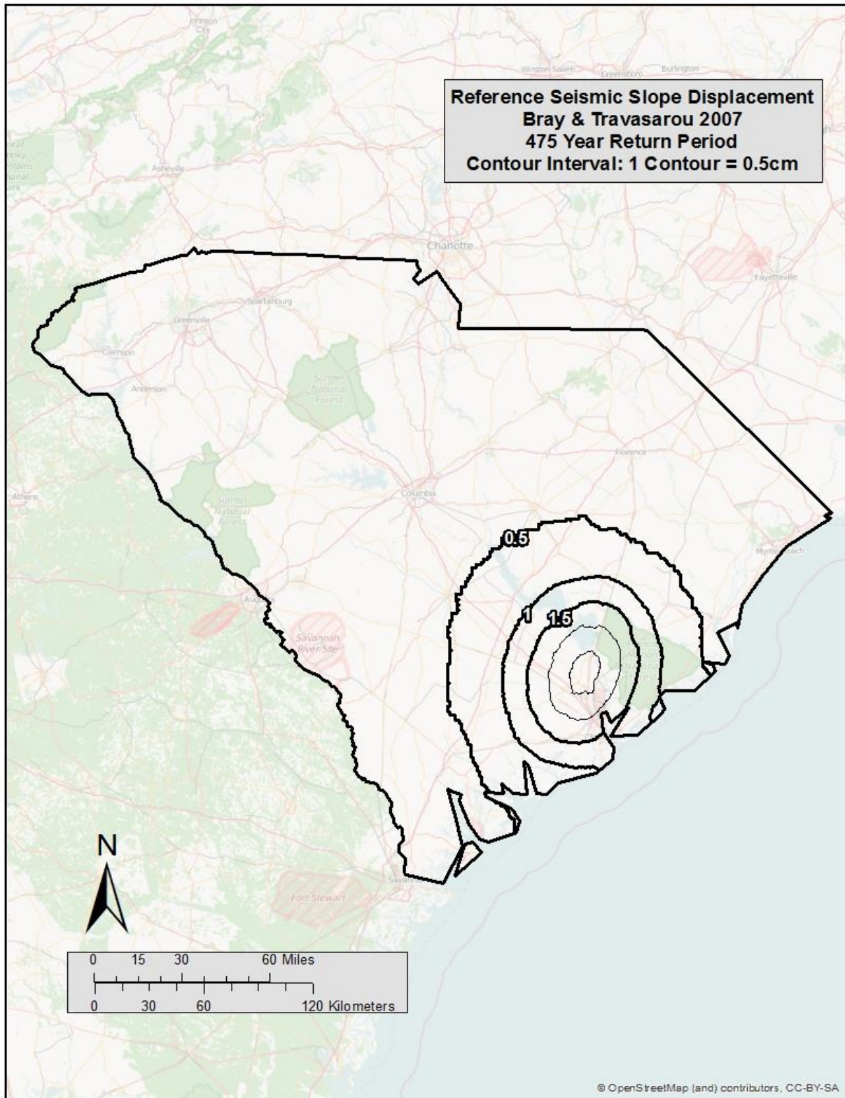
Figure E- 22 Bray and Travarasrou (2007) Seismic Slope Displacement ( D^{ref} ) Map for South Carolina (Tr = 475)
