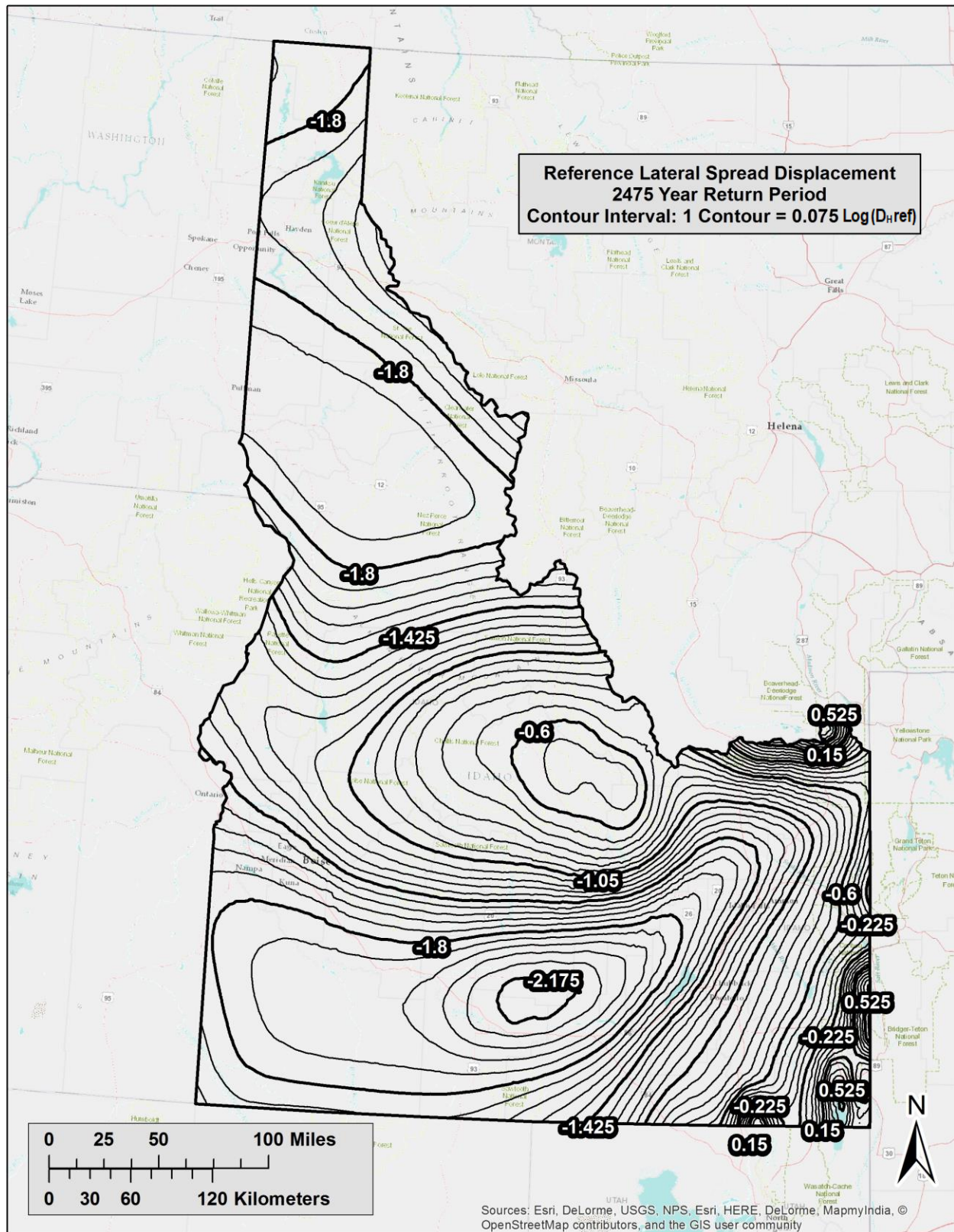
Figure C- 9 Log D_H^{ref} for Idaho ( T_R = 2475 years)
