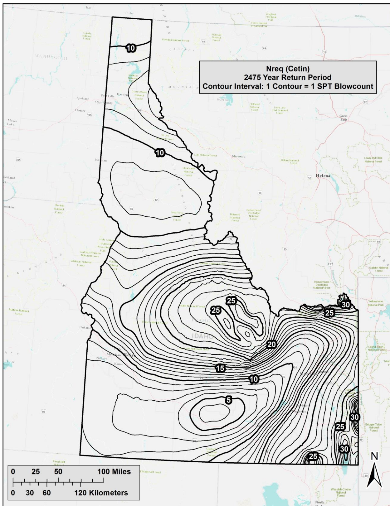
Figure B- 15 N_{req} for Idaho ( T_R = 2475 years)
