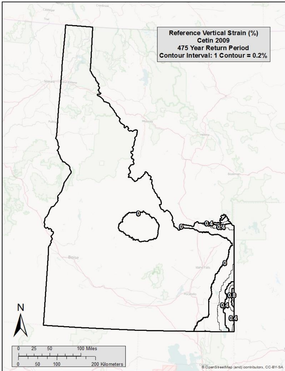
Figure D- 7 Cetin et al. (2009) Post-Liquefaction Settlement ( \varepsilon^{ref} ) Map for Idaho (Tr = 475)
