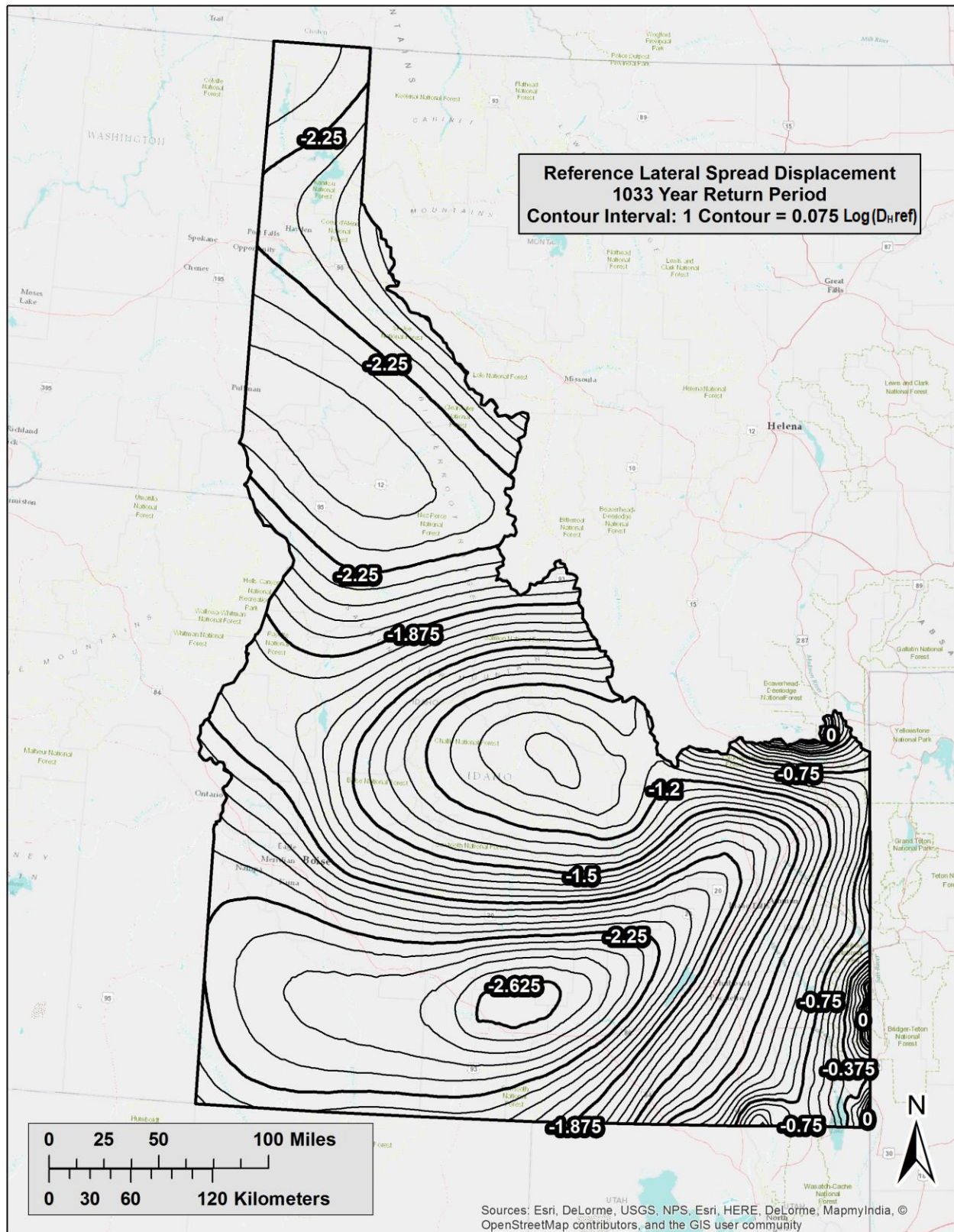
Figure C- 8 Log D_{H}^{ref} for Idaho ( T_R = 1033 years)
