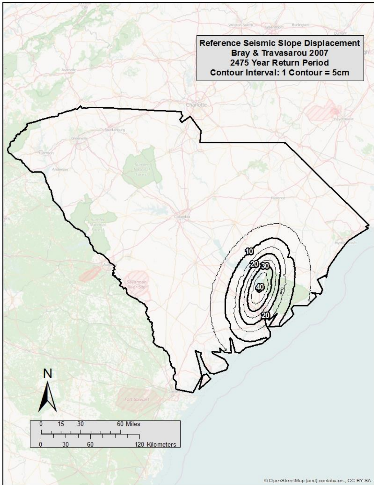
Figure E- 23 Bray and Travarasrou (2007) Seismic Slope Displacement ( D^{ref} ) Map for South Carolina (Tr = 1,033)
