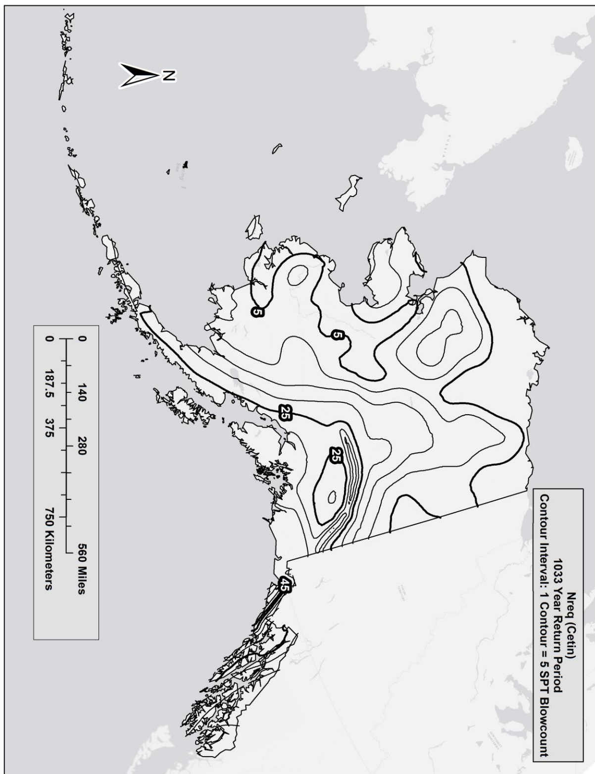
Figure B- 5 N_{req} for Alaska ( T_R = 1033 years)
