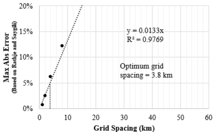
Figure 4-18 Variation of maximum percent error (based on Rathje & Saygili 2009) with increasing distance between grid points for Eureka, CA. (Pink zone, PGA = 1.4004)
