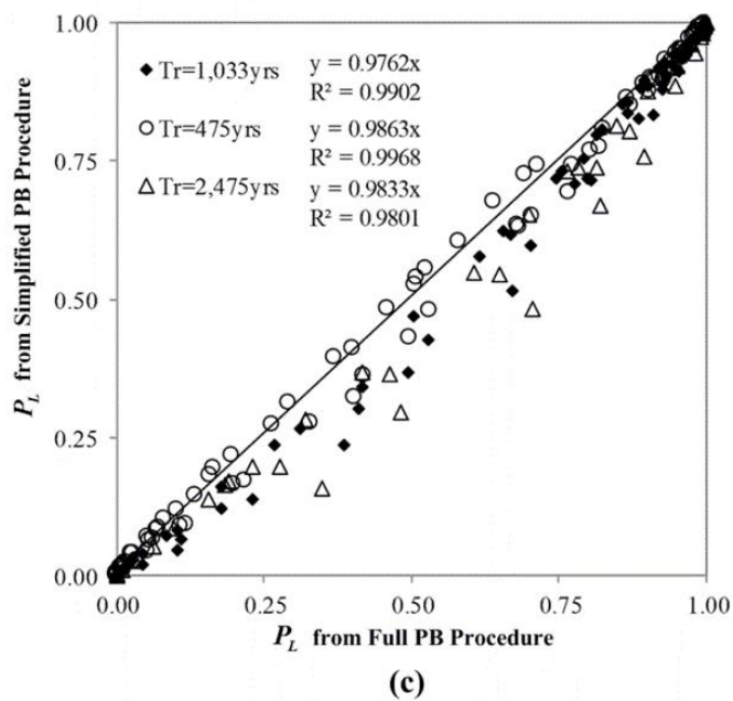
Figure 3-3 Comparative scatter plots for simplified and full performance-based procedures for (a) \widehat{CSR}_{M=7.5, \sigma_v'=1atm} (\%) , (b) FS_L , (c) P_L , and (d) \Delta N_L
