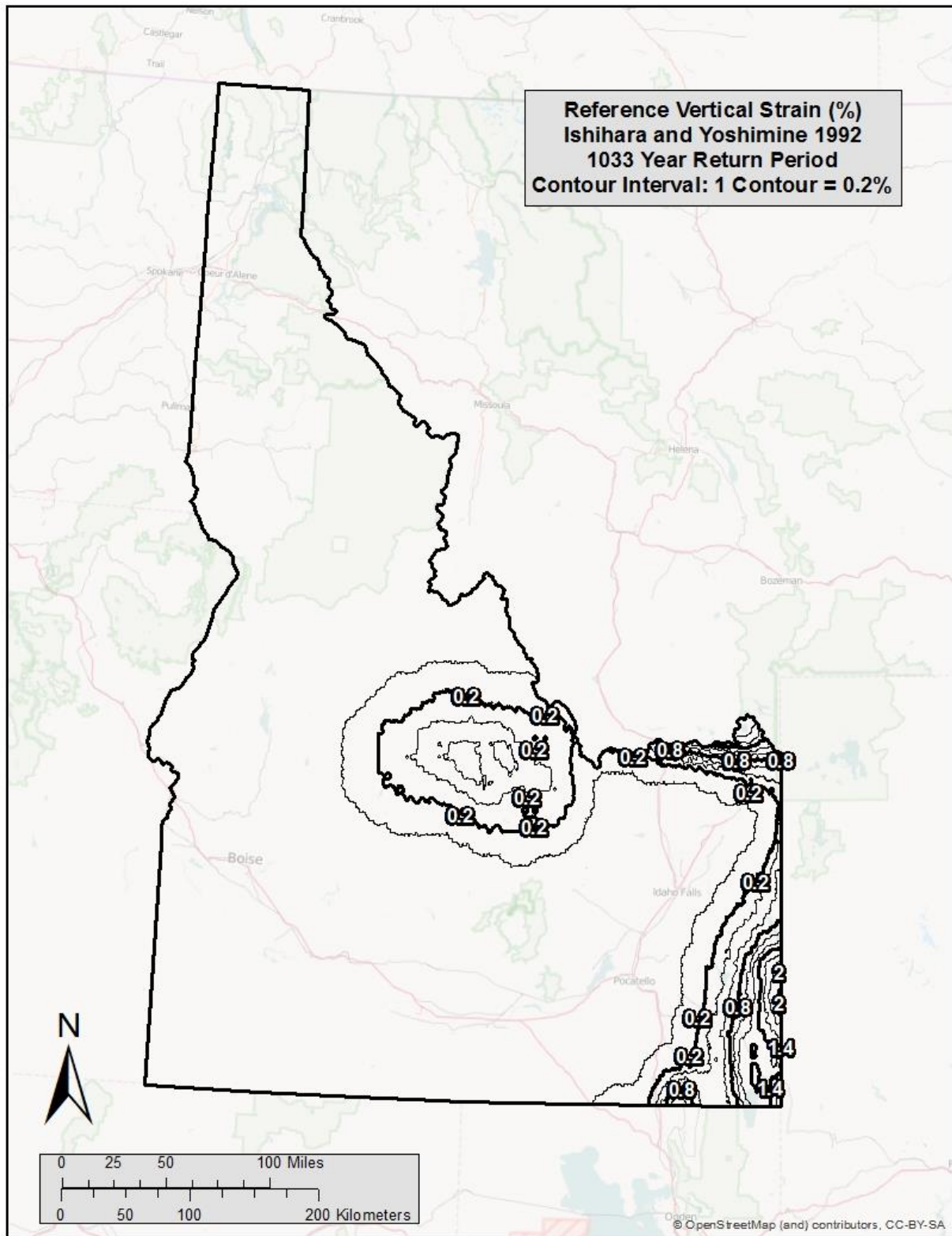
Figure D- 11 Ishihara and Yoshimine (1992) Post-Liquefaction Settlement ( \varepsilon^{ref} ) Map for Idaho (Tr = 1,033)
