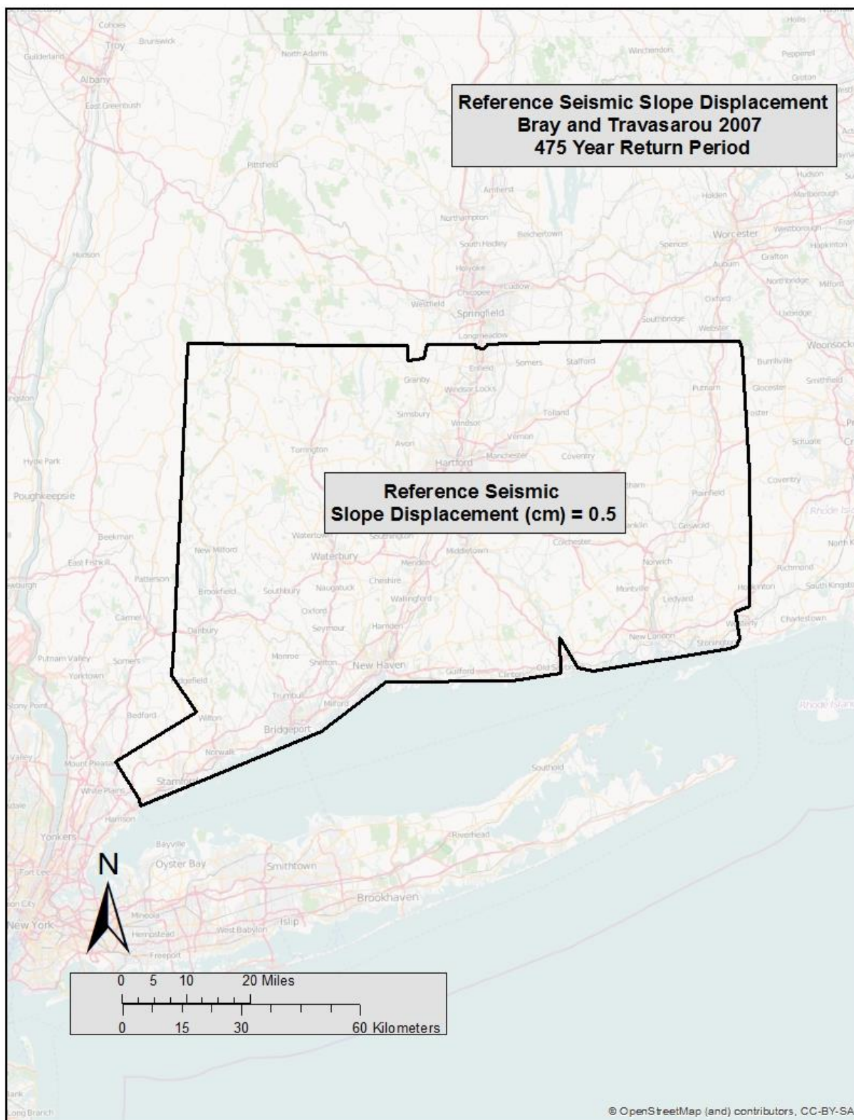
Figure E- 4 Bray and Travarasrou (2007) Seismic Slope Displacement ( D^{ref} ) Map for Connecticut ( Tr = 475 )
