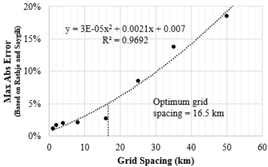
Figure 4-19 Variation of maximum percent error (based on Rathje & Saygili 2009) with increasing distance between grid points for Portland, OR. (Orange zone, PGA = 0.4366 )
