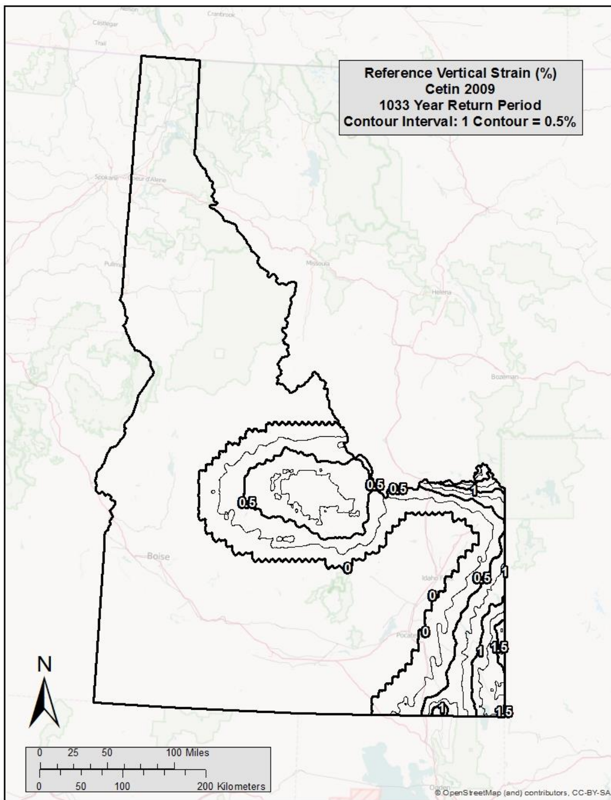
Figure D- 8 Cetin et al. (2009) Post-Liquefaction Settlement ( \varepsilon^{ref} ) Map for Idaho (Tr=1,033)
