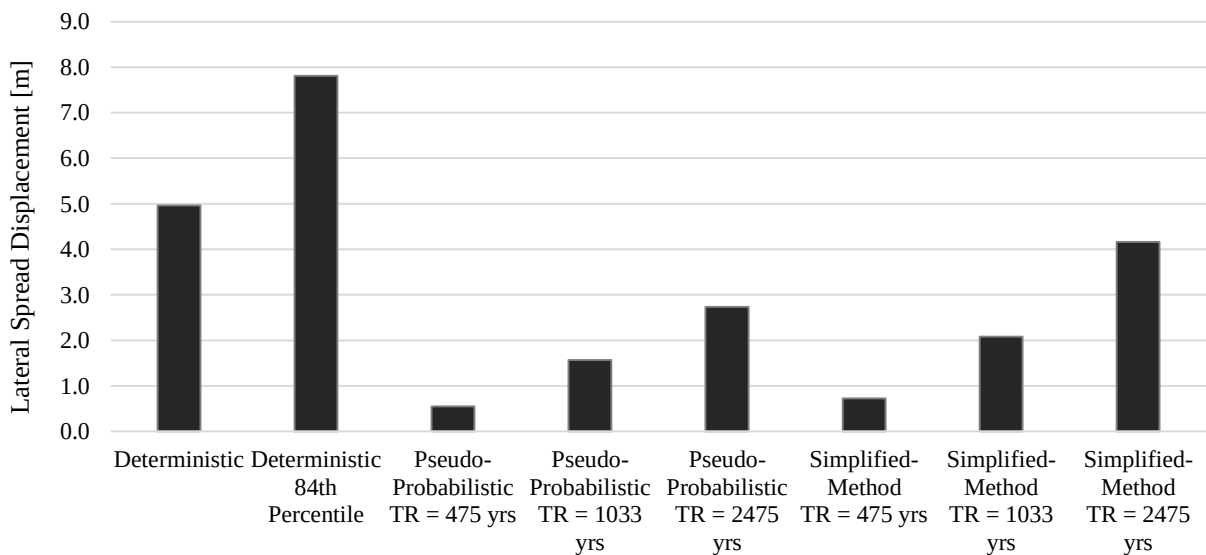
Figure 6-8 Comparison of Deterministic, Pseudo-probabilistic, and Simplified methods for Salt Lake City, UT (Latitude 40.755, Longitude -111.898).
