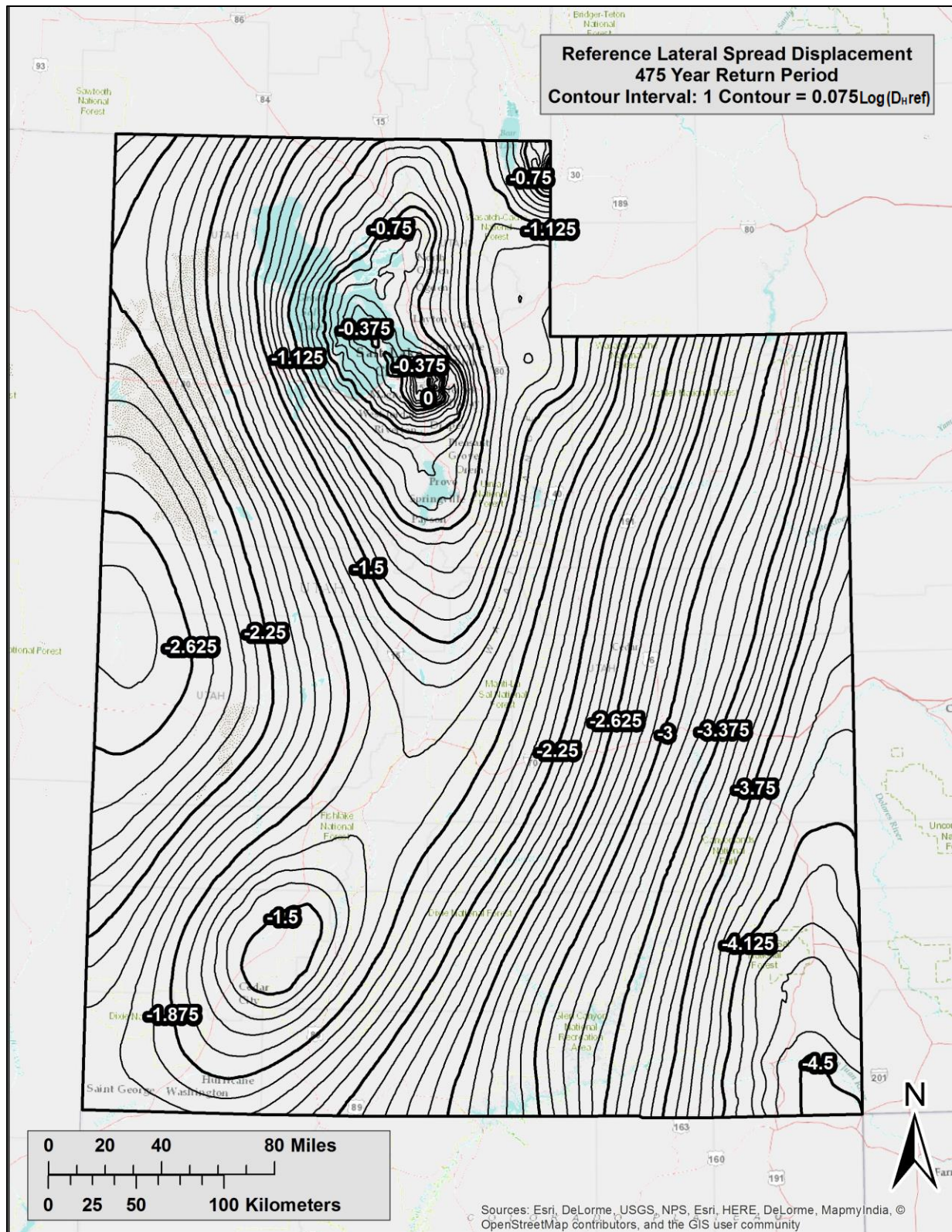
Figure C- 16 \log D_H^{\text{ref}} for Utah ( T_R = 475 years)
