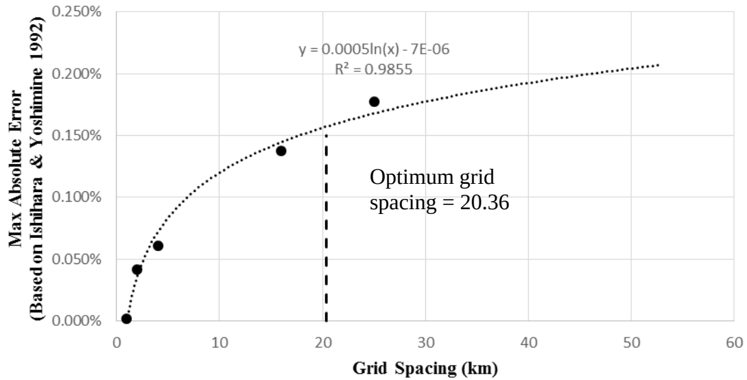
Figure 4-15 Variation of maximum percent error (based on Ishihara & Yoshimine 1992) with increasing distance between grid points for Portland, OR. (Orange zone, PGA = 0.4366 )
