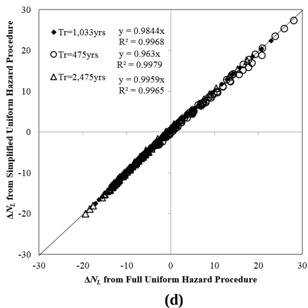
Figure 3-3 Comparative scatter plots for simplified and full performance-based procedures for (a) \widehat{CSR}_{M=7.5, \sigma_v'=1atm} (\%) , (b) FS_L , (c) P_L , and (d) \Delta N_L
