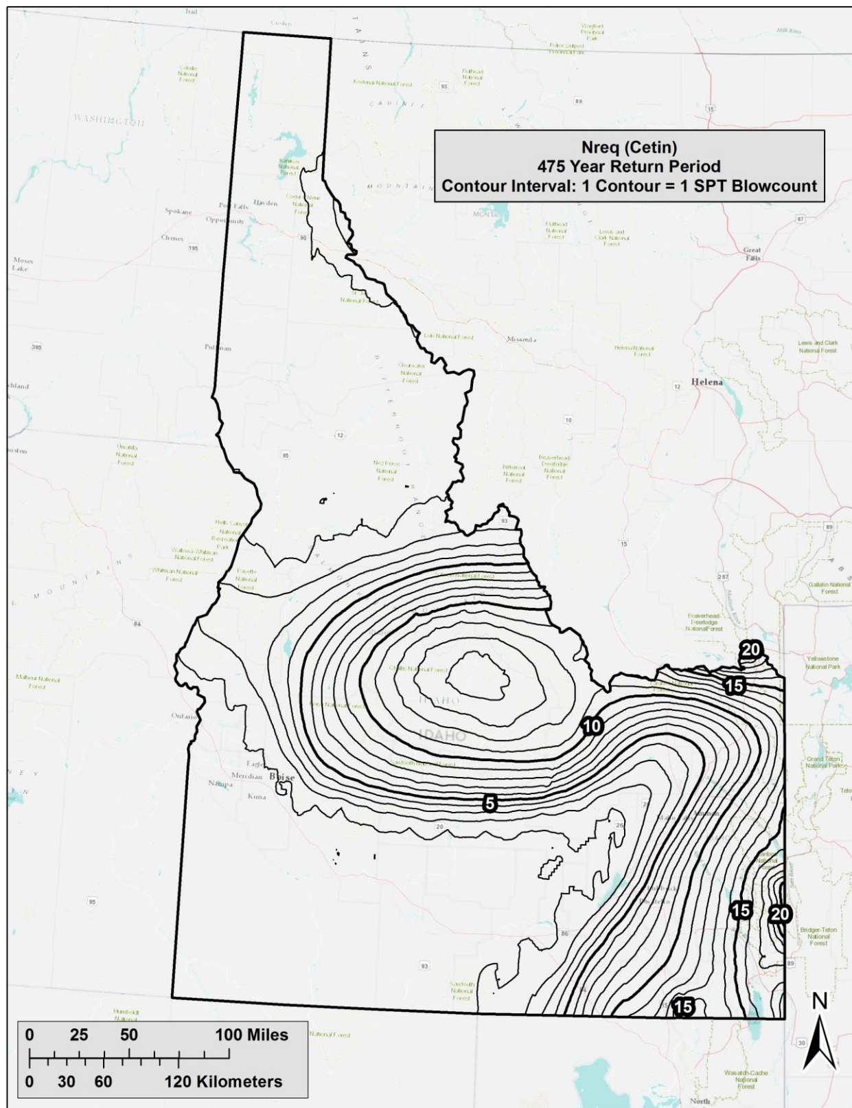
Figure B- 13 N_{req} for Idaho ( T_R = 475 years)
