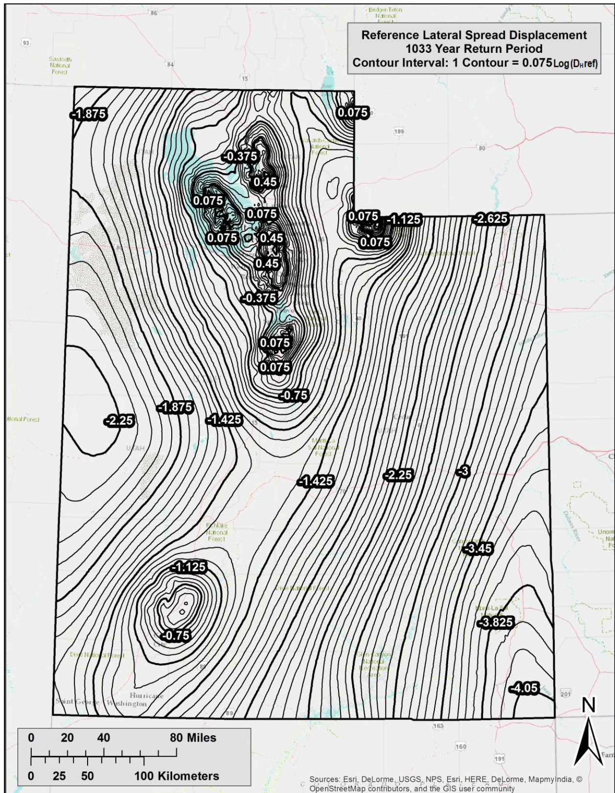
Figure C- 17 Log D_H^{ref} for Utah ( T_R = 1033 years)
