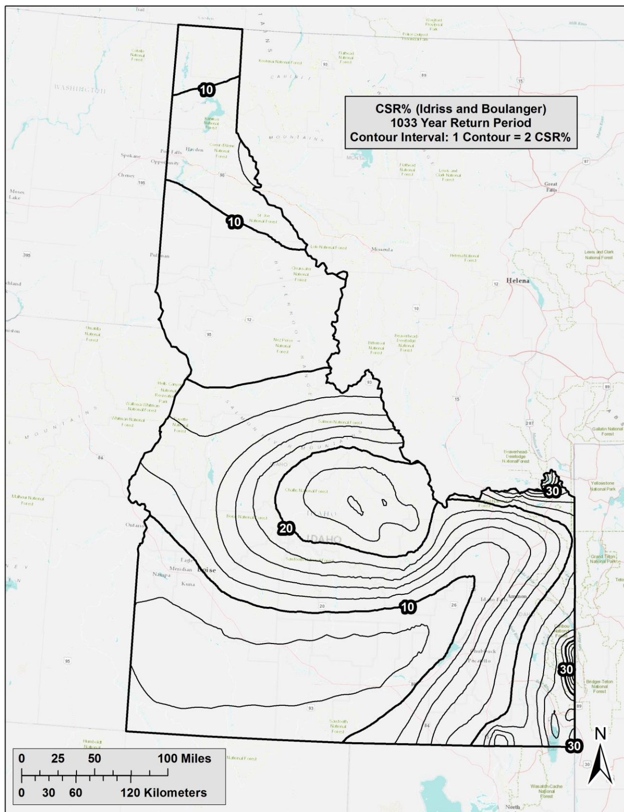
Figure B- 11 CSR% for Idaho ( T_R = 1033 years)
