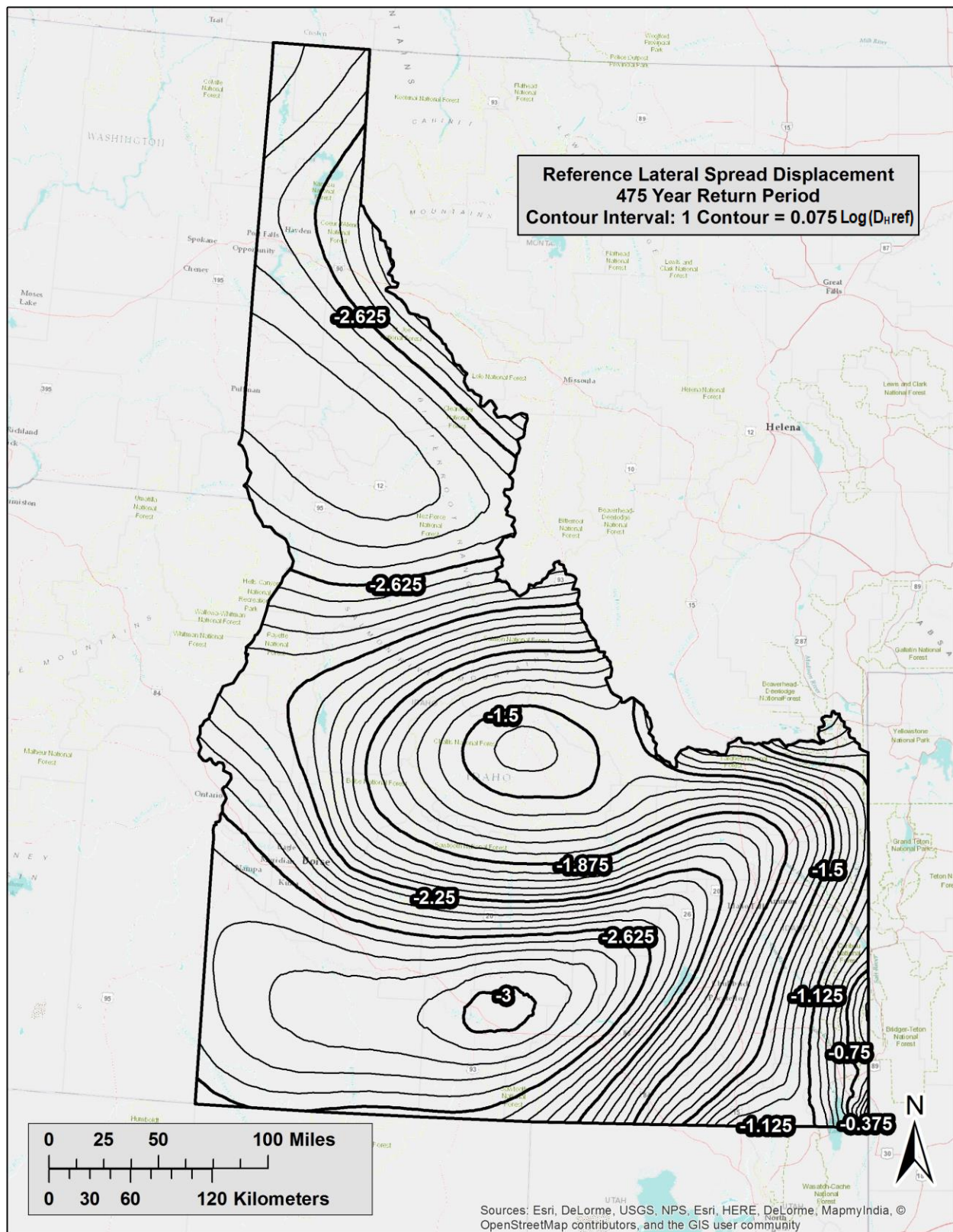
Figure C- 7 Log D_H^{ref} for Idaho ( T_R = 475 years)
