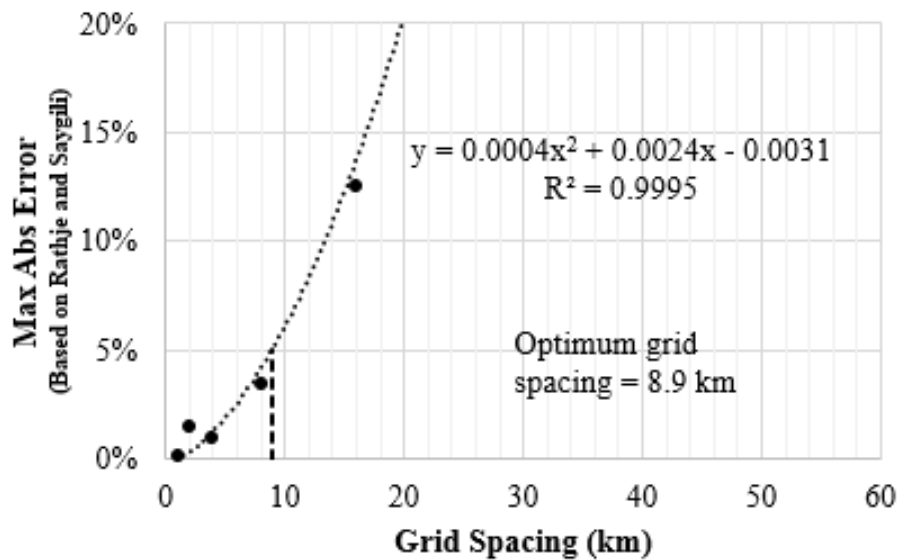
Figure 4-20 Variation of maximum percent error (based on Rathje & Saygili 2009) with increasing distance between grid points for Butte, MT. (Yellow zone, PGA = 0.1785 )
