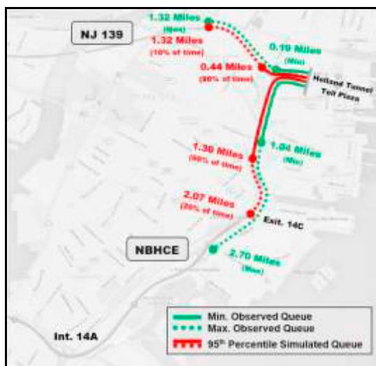
Fig. 3. 95 Percentile Maximum Simulated Queue Lengths in Base Case
