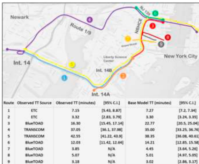
Fig. 2. Comparison of Observed and Simulated Travel Times on Selected Paths
