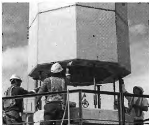
(c) PT bars coupled, placement of subsequent segments with epoxy applied to adjoining segment faces
