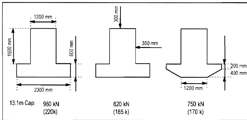
Figure 3.20 Modifying the cap cross-section led to a reduced cap weight
