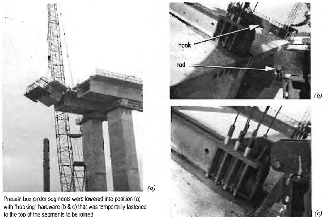
Figure 3.13 Construction of the JFK Causeway
