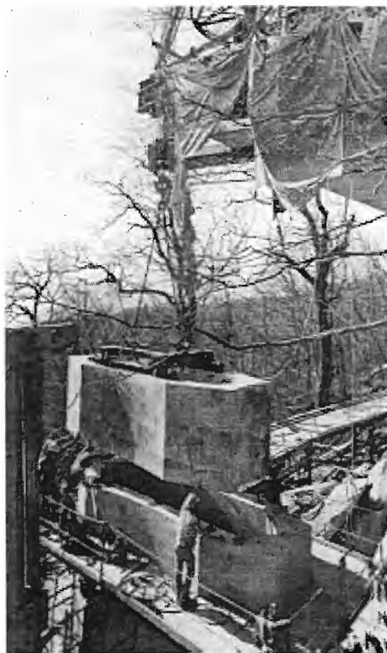
Figure 2.6 Precast hollow concrete pier segments lowered into position from the deck above at the Linn Cove Viaduct in North Carolina [10]
