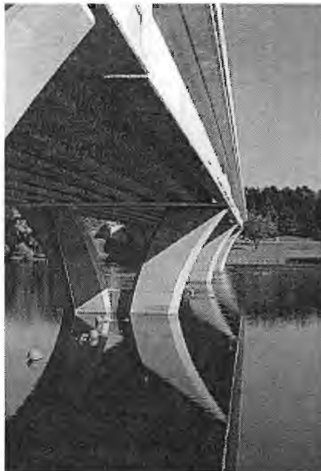
Figure 4.11 Cast-in-place substructures can be curved or tapered
