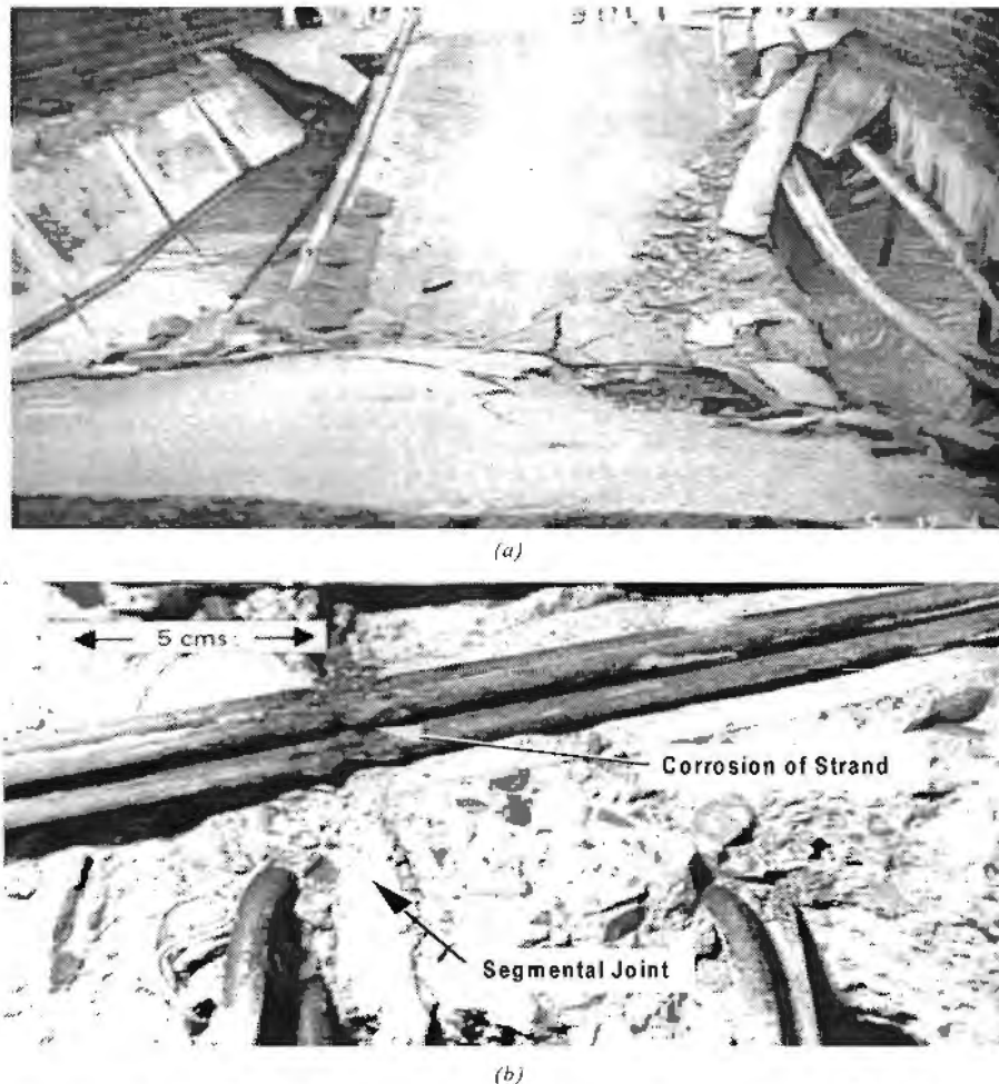
Figure 3.14 (a) The collapse of a bridge at Ynys-y-Gwas in Wales; (b) Collapse was attributed to corrosion of prestressing strand at mortar-filled segmental joints [from Reference 69]
