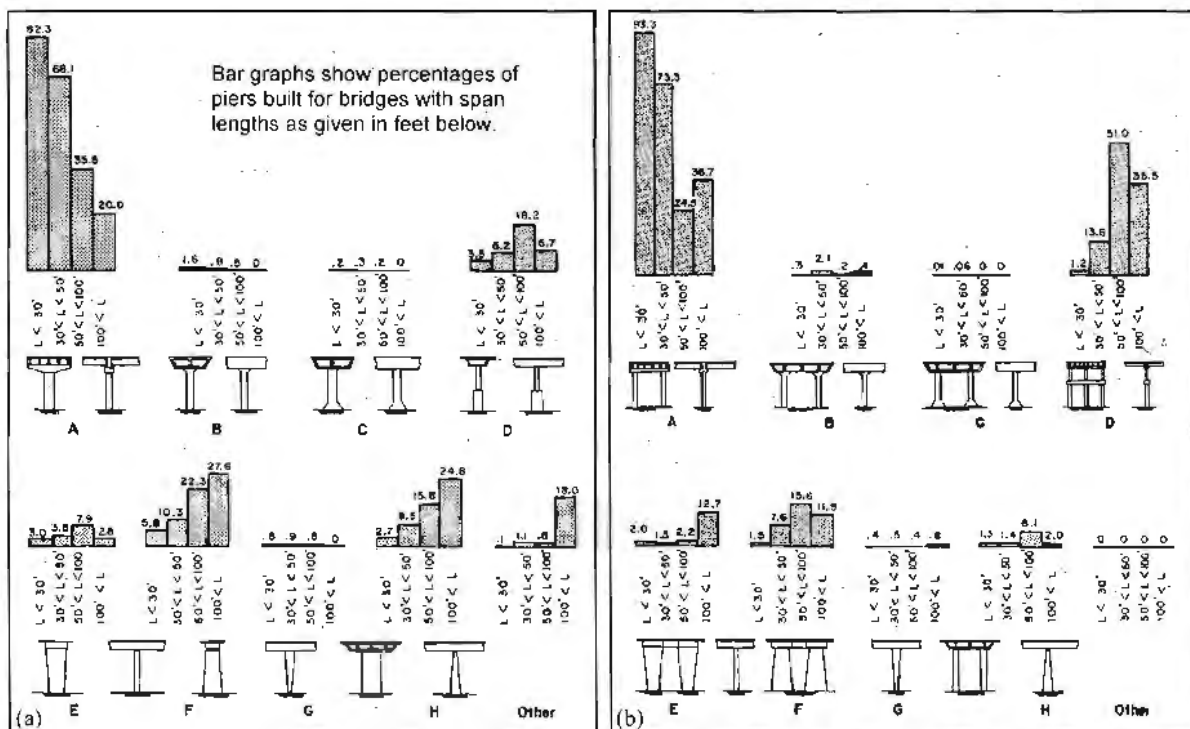
Figure 2.1 Survey results on pier types built from 1960-1980 [9]
