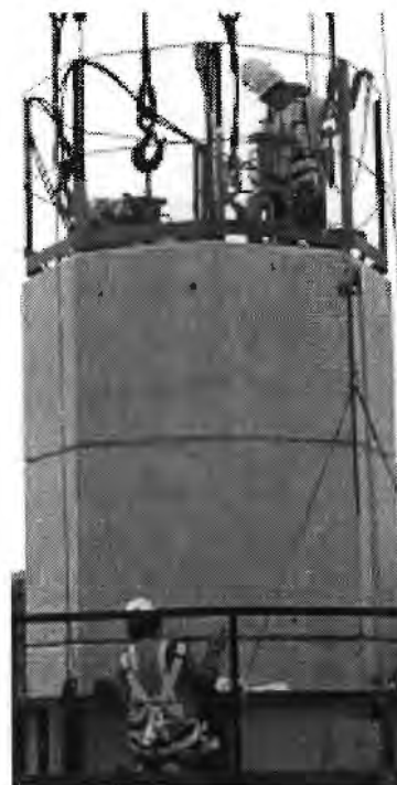
(d) New segment post-tensioned down to previously erected segments
