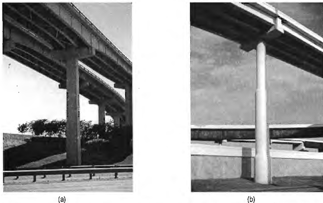
Figure 4.30 A subtle column taper (a) is more attractive than abrupt changes in cross section (b) for tall columns
