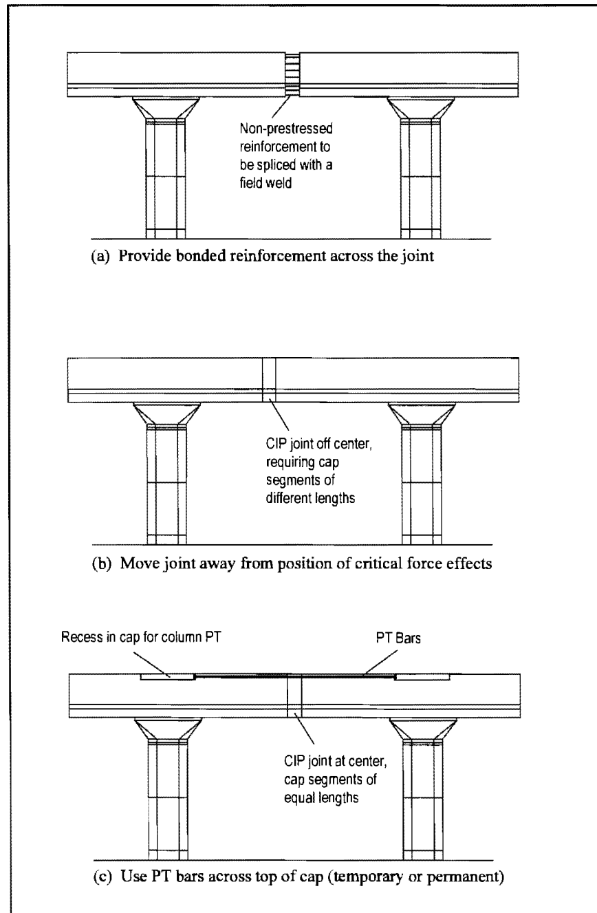
Figure 3.33 Alternate connection options for frame bents
