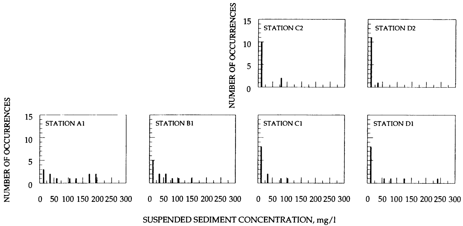
XXVI-2. Histograms of maximum increased suspended sediment concentration, Apple River Island
