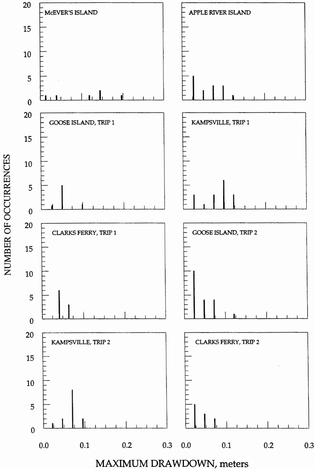
XXIV-1. Histograms of maximum drawdown, upstream barges
