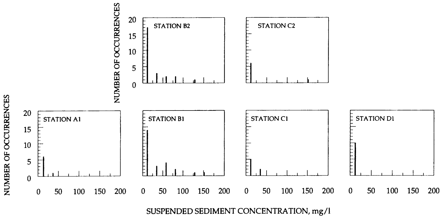
XXVI-6. Histograms of maximum increased suspended sediment concentration, Goose Island, trip 2
