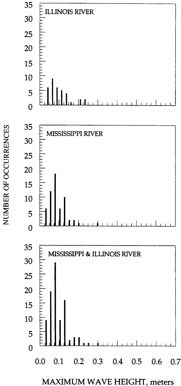
XXIII-4. Histograms of maximum wave height for the river system, upstream barges
