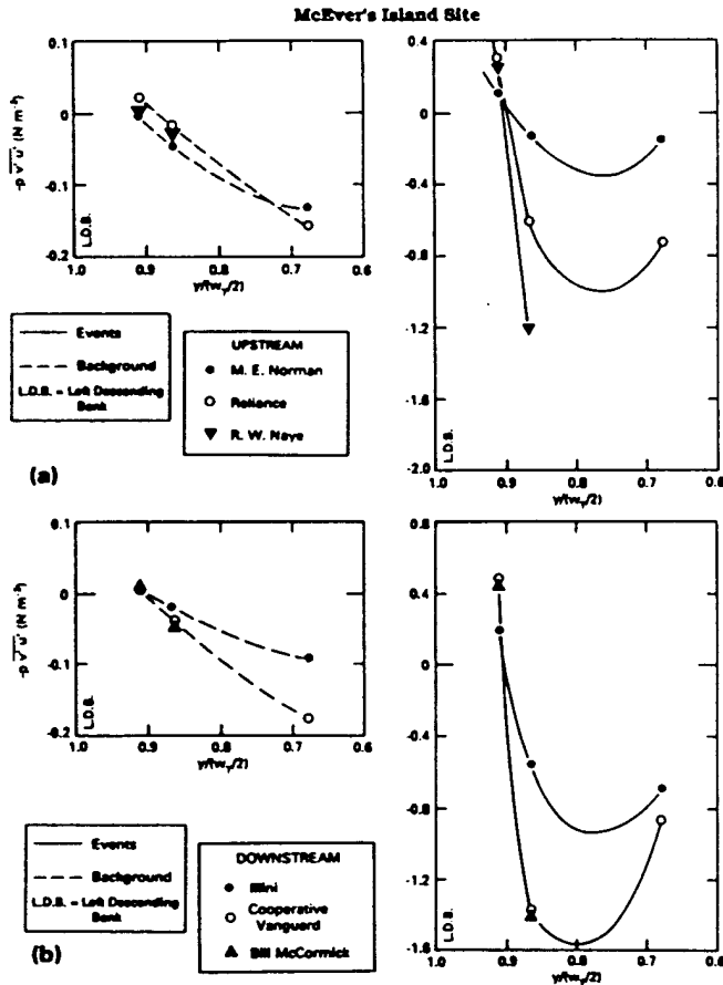
FIG. 7. Lateral Reynolds Stress Distributions before and during Series of Events at McEver's Island Site
