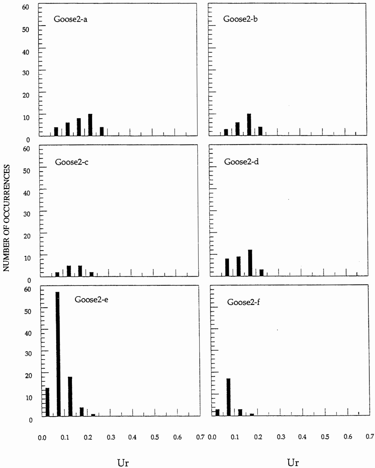
XXI-17. Histograms of absolute U_{r(max)} within various zones, Goose Island, trip 2
