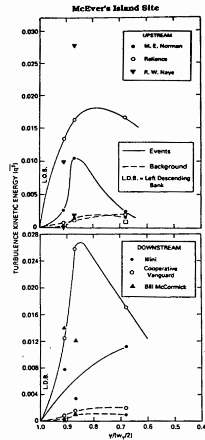
FIG. 10. Lateral Variations of Turbulent Kinetic Energy for Upstream and Downstream Events: Background and Events
