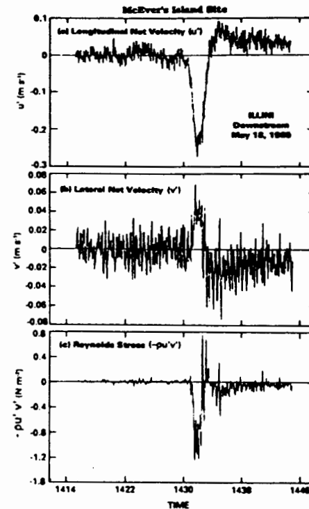
FIG. 4. Temporal Variations of Turbulent Fluctuating Velocities and Reynolds Stress for Downstream Barge
