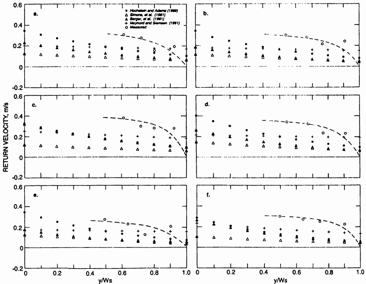
FIG. 5. Comparison between Computed and Measured Lateral Velocity Distribution for Upstream Bound Barges: (a) Sugarland; (b) Conti Karla; (c) Mr. Lawrence; (d) Charles Lehman; (e) Nicholas Duncan; (f) Mr. Paul
