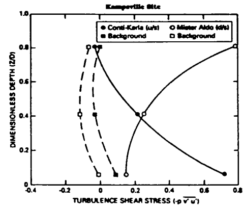
FIG. 8. Vertical Variations of Reynolds Stress for Longitudinal Component of Velocity: Background and Events
