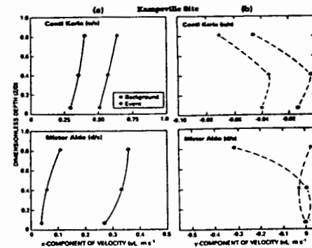
FIG. 6. Variations of Velocity with Depth before and during Upstream and Downstream Barge Movements; (a) Longitudinal Velocity; and (b) Transverse Velocity at the Kampsville Site
