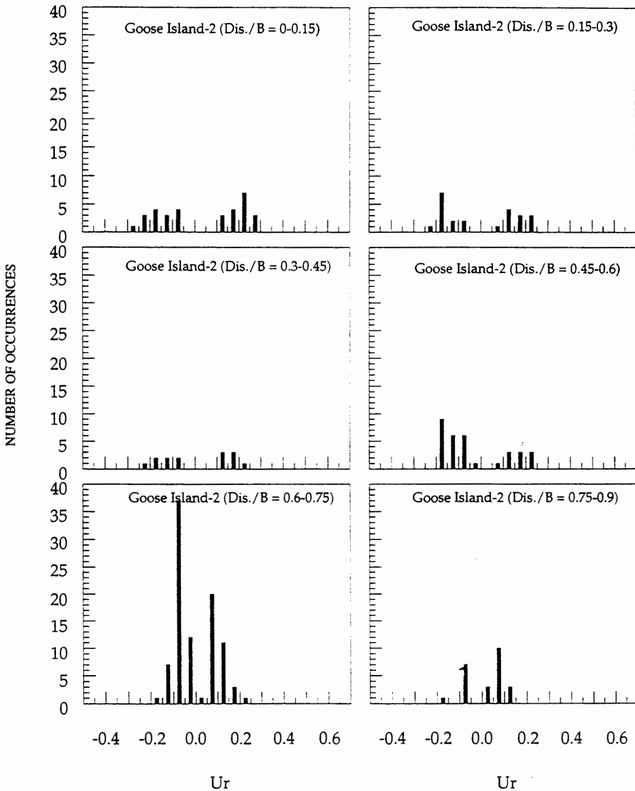
XXI-6. Histograms of U_{r(max)} within various zones, Goose Island, trip 2 ( U_{r(max)} carries signs to indicate an upstream- or downstream-bound barge effect)
