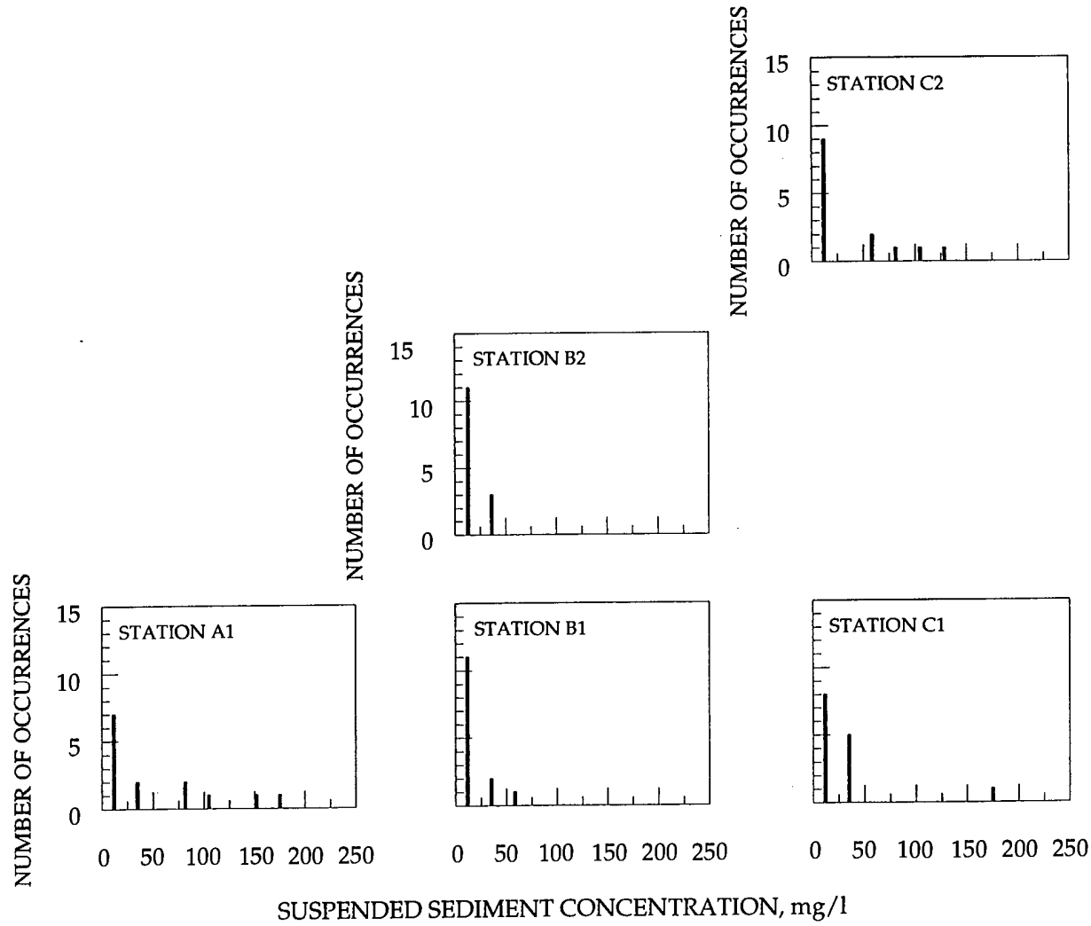
XXVI-3. Histograms of maximum increased suspended sediment concentration, Goose Island, trip 1
