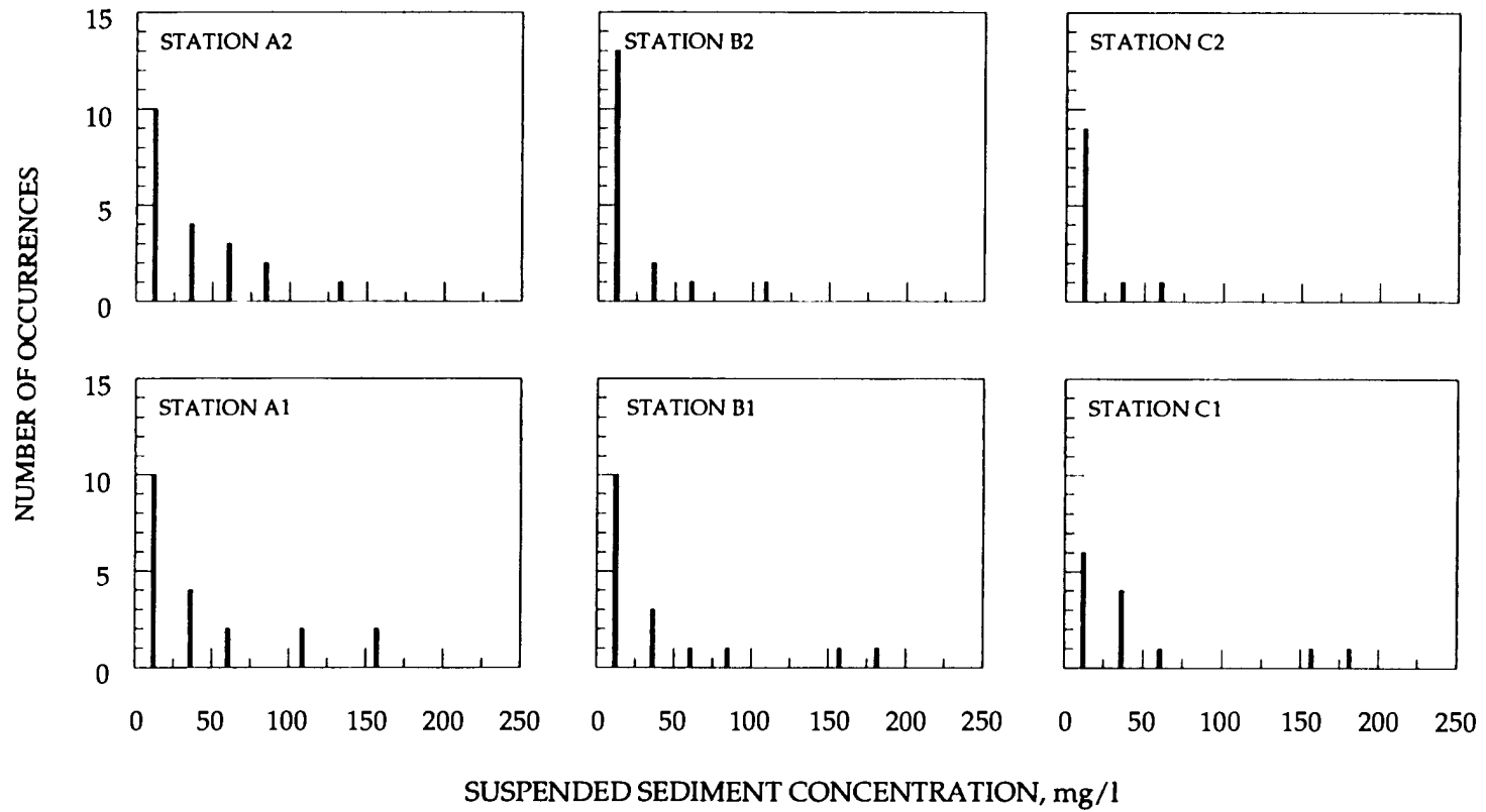
XXVI-4. Histograms of maximum increased suspended sediment concentration, Kampsville, trip 1
