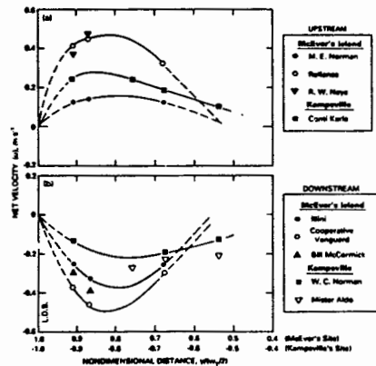
FIG. 5. Net Longitudinal Velocity Distributions due to Movement of Navigation Traffic
