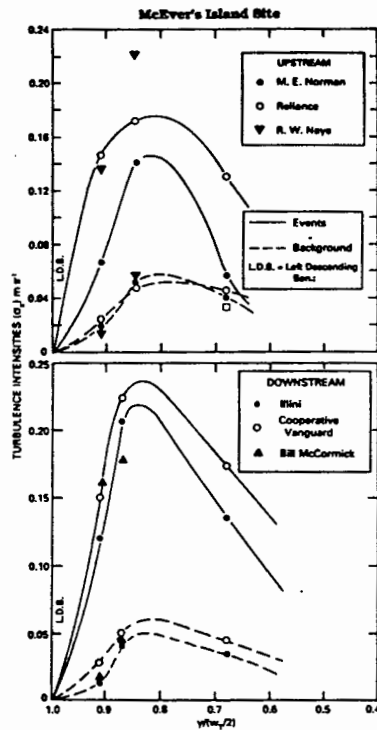
FIG. 9. Lateral Variations of Turbulence Intensities for Upstream and Downstream Barge Movement: Background and Events
