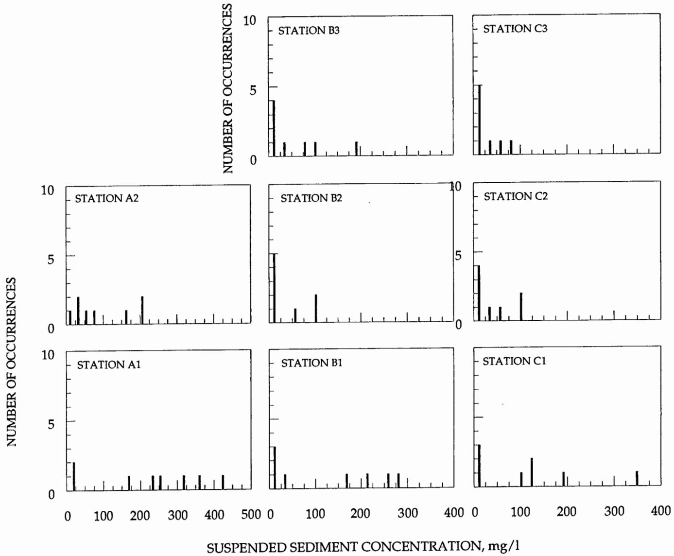
XXVI-1. Histograms of maximum increased suspended sediment concentration, McEver's Island
