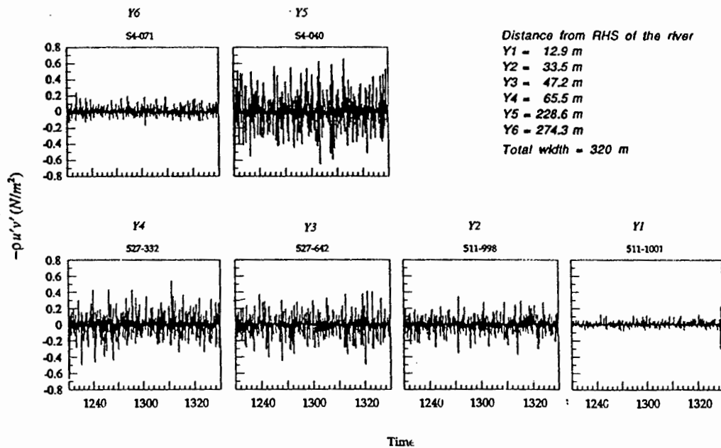
Fig. 11. Variation of instantaneous turbulent shear stresses with time for October 13, 1990 from 1230 to 1330 h.
