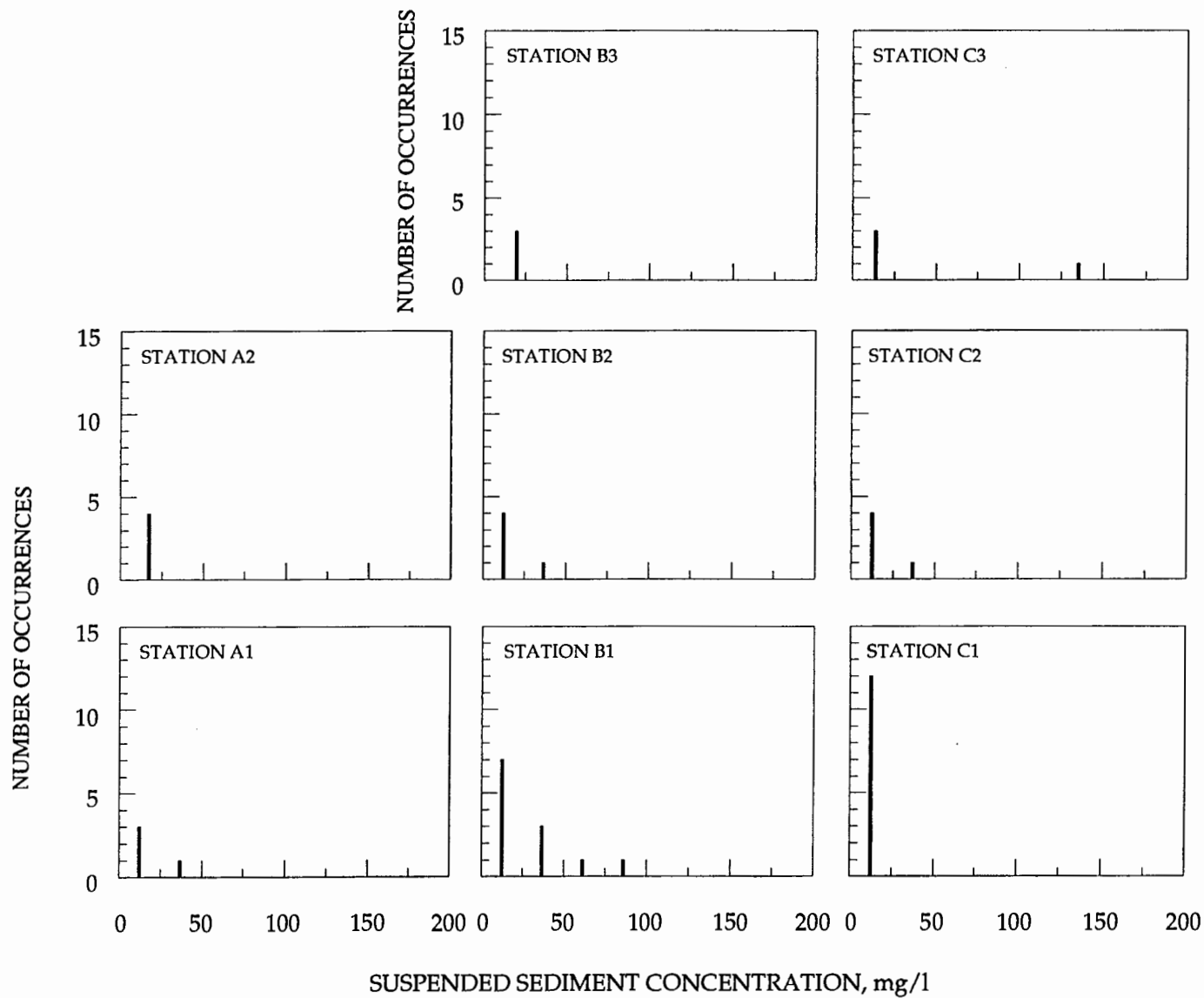
XXVI-5. Histograms of maximum increased suspended sediment concentration, Clarks Ferry, trip 1
