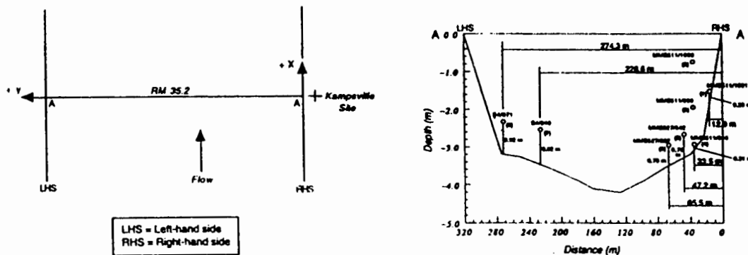
Fig. 1. Schematic diagram showing the data collection set-up on the Illinois River at Kampsville.
