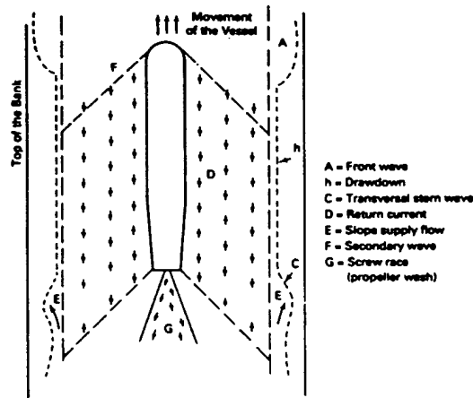
FIG. 1. Schematic Design Showing Water Motion Generated by Moving Ship In Stagnant Water (after Blaauw et al. 1984)
