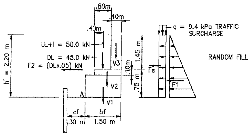
b) Abutment seat configuration
