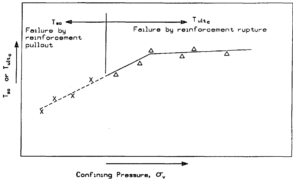
Figure A.3. Determination of T_{sc} and T_{ultc} at Various Facing Block Confining Pressures.
