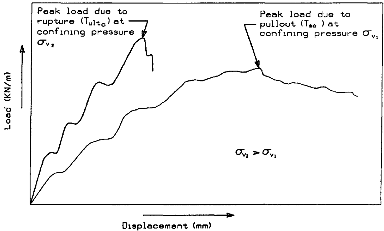
Figure A.2. Load Versus Displacement for Connection Strength Test.
