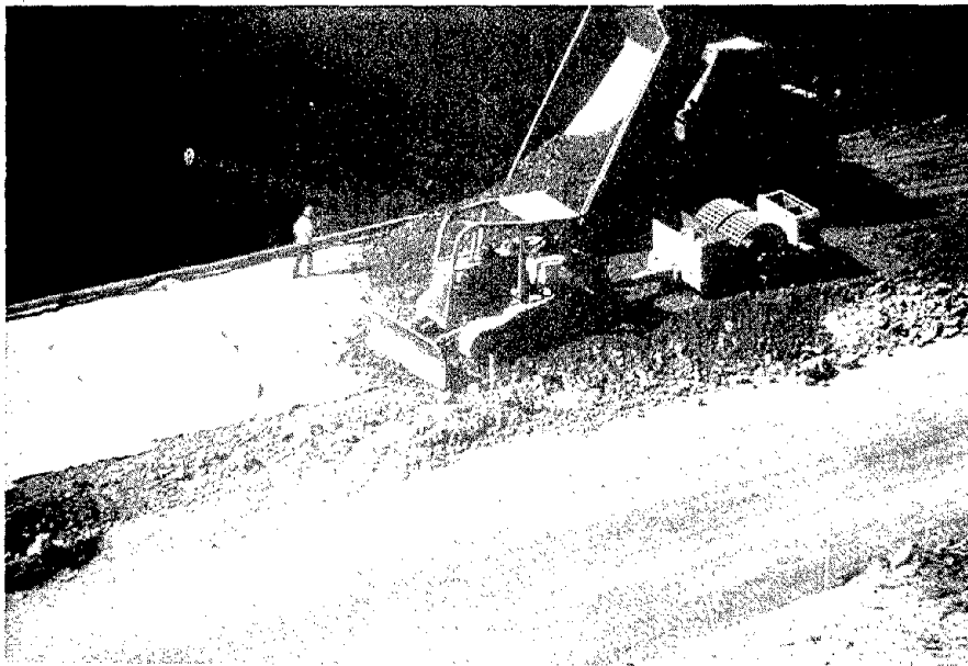
Figure 79. Placement of reinforced backfill.
