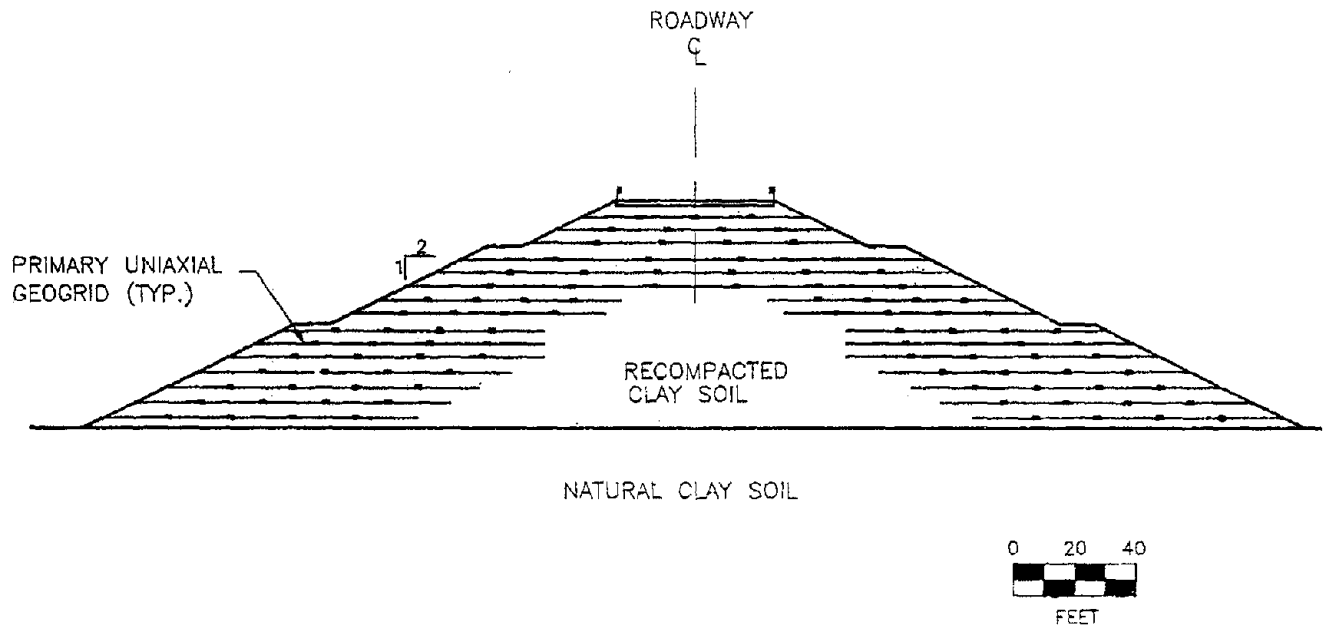
Figure 58. Cannon Creek project.
