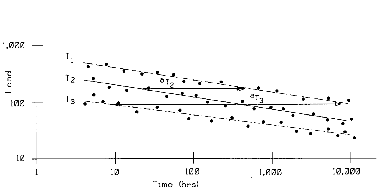
(a) Stress rupture envelope without "knee"
