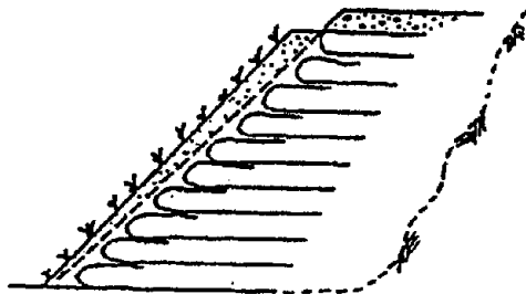
SLOPING SOIL AND VEGETATION FACING
