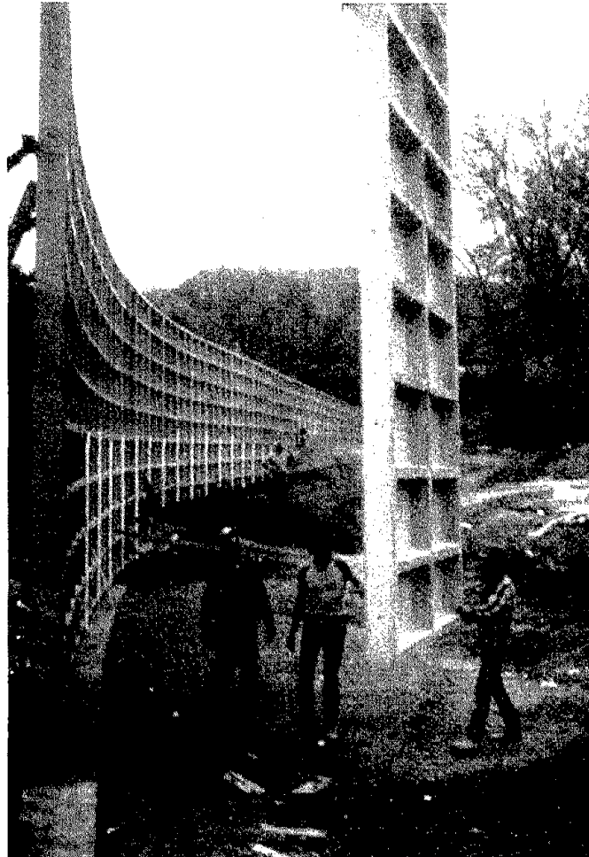
Figure 77. Full height facing panels require special alignment care.
