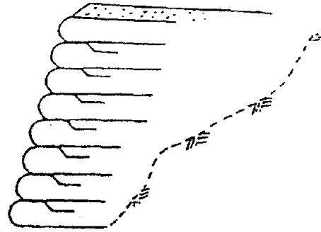
SLOPING GEOSYNTHETIC FACING
