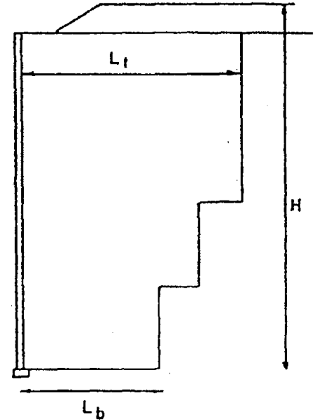
(c) TRAPEZOIDAL WALLS
