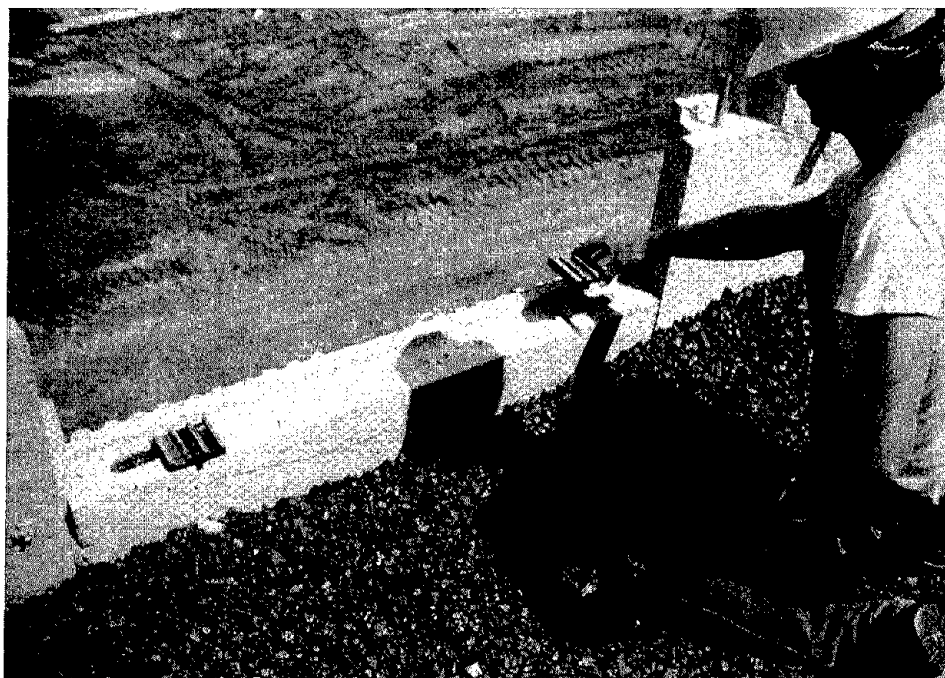
Figure 82. Geotextile joint cover and neoprene pads.
