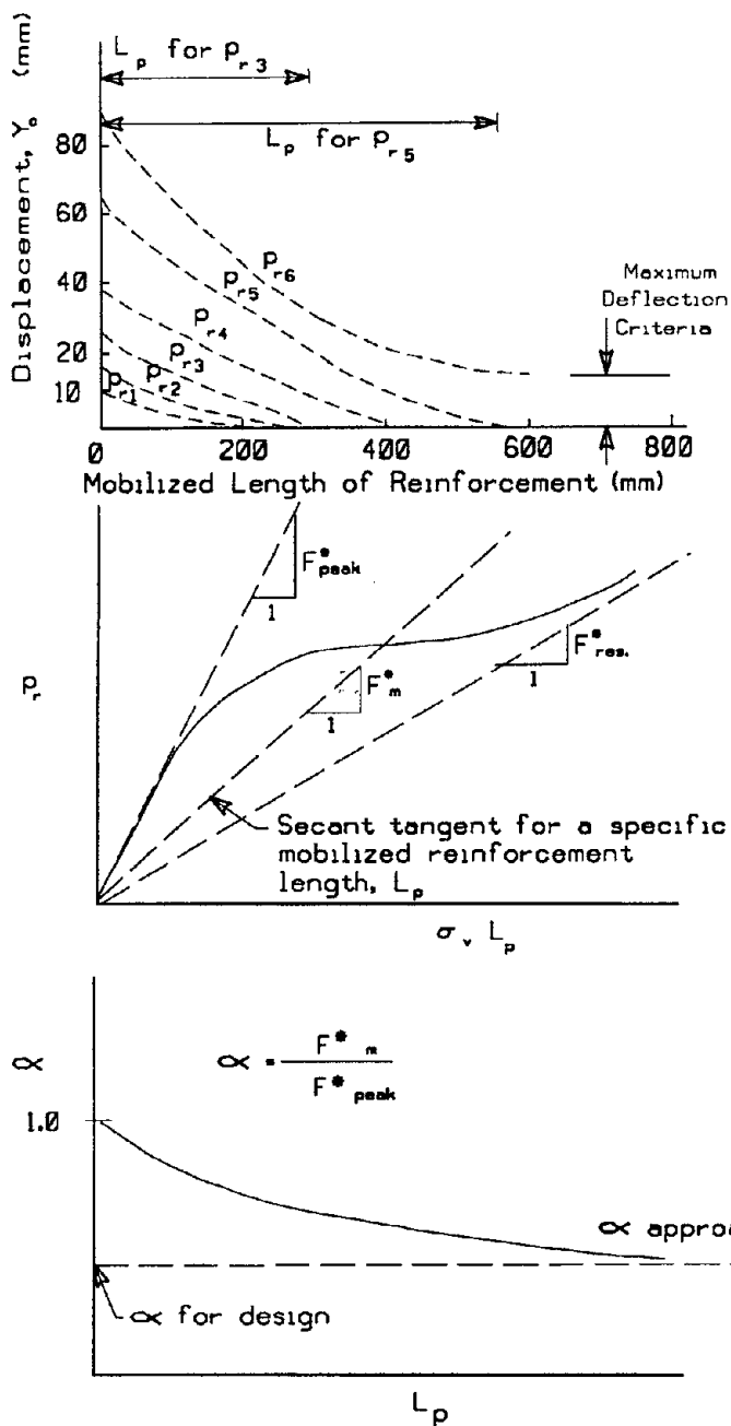
Figure A.1. Experimental procedure to determine F^* and \alpha for Soil Reinforcement using pullout test.
