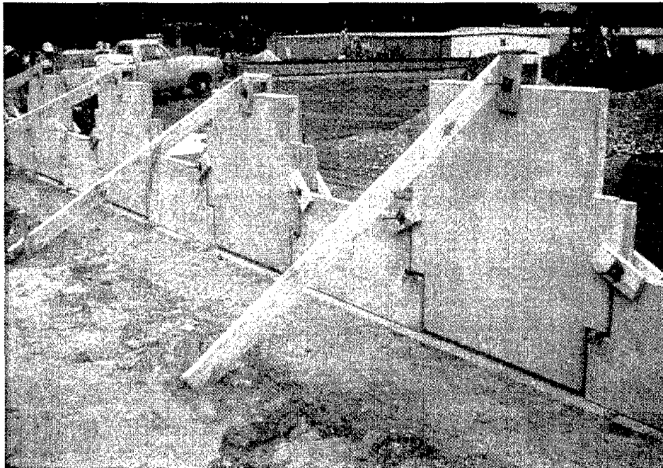
Figure 78. Setting first row of precast facing elements.
