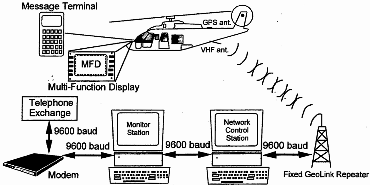
Figure 2-2 Datalink Configuration
