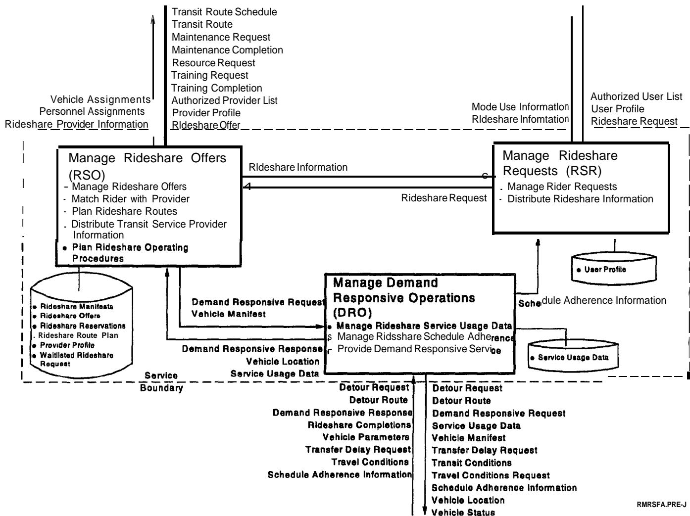
Figure 74. Ride Matching and Reservation - Functional Architecture
