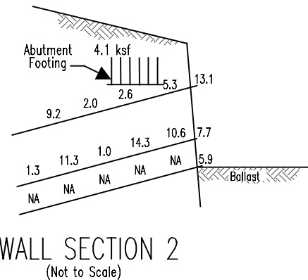
Figure 4.3: Wall 13A Section 2
