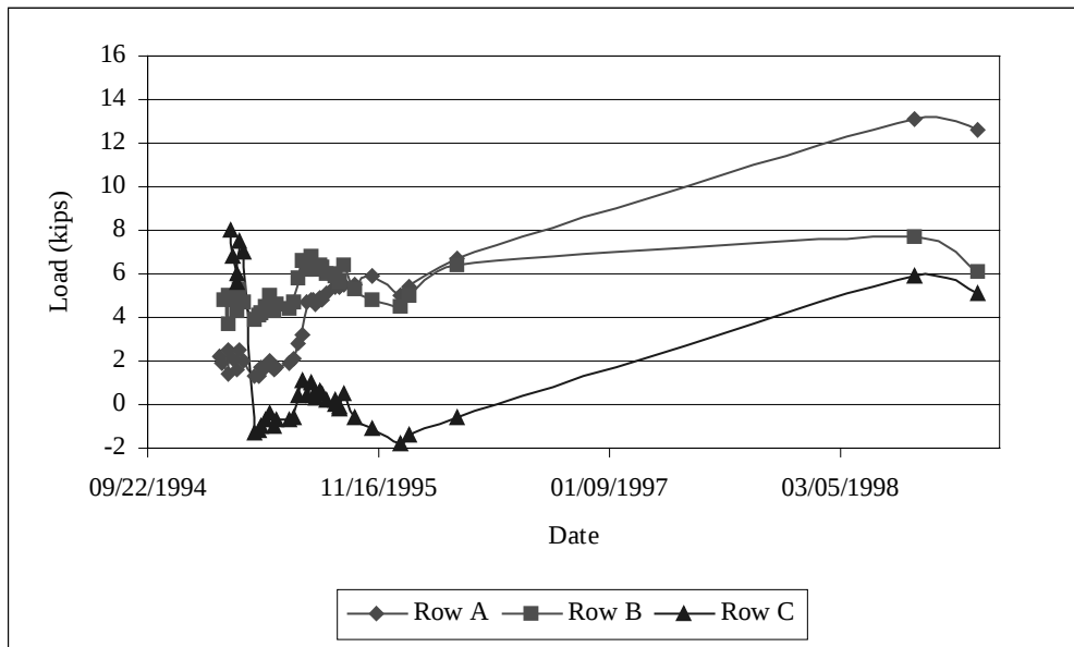
Figure 7.4: Wall Section 2 Load Cell Readings
