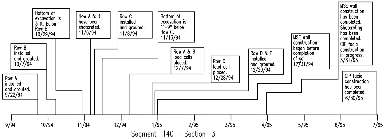
Figure 5.1: Construction timeline
