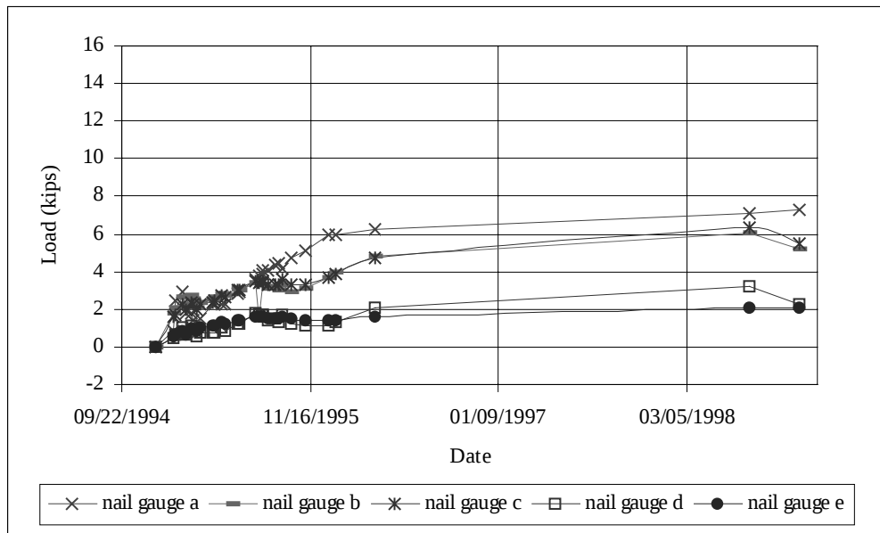
Figure 7.12: Wall Section 3 Row D Strain Gauge Readings
