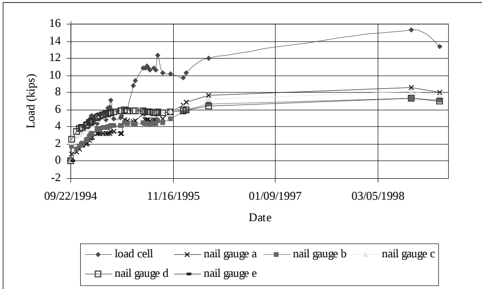
Figure 7.10: Wall Section 3 Row A Strain Gauge Readings
