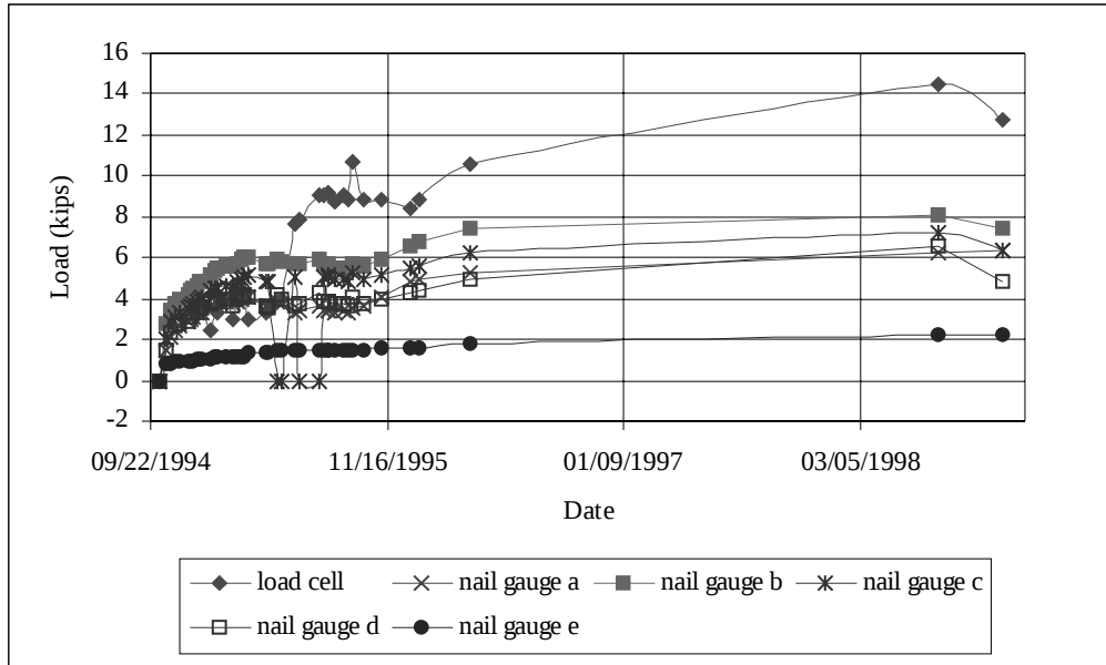
Figure 7.11: Wall Section 3 Row B Strain Gauge Readings
