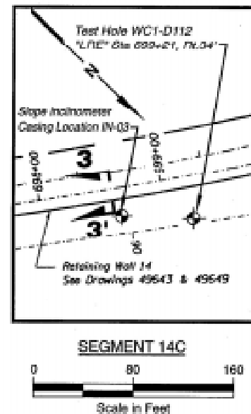
Figure 3.2: Site plan for Wall 14
