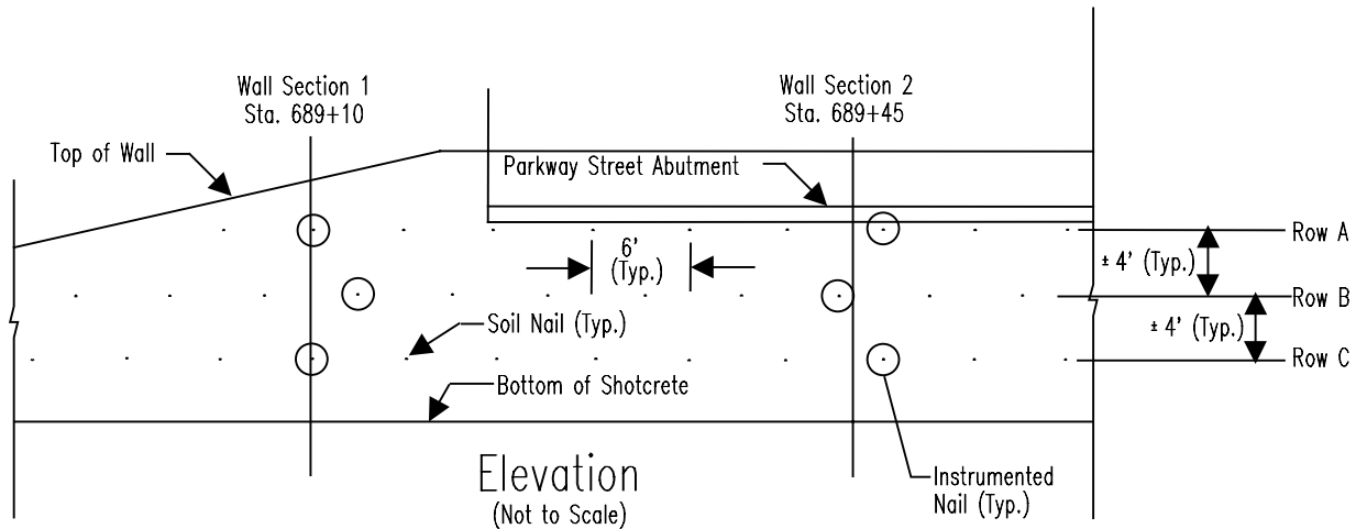
Figure 4.1: Wall 13A elevation
