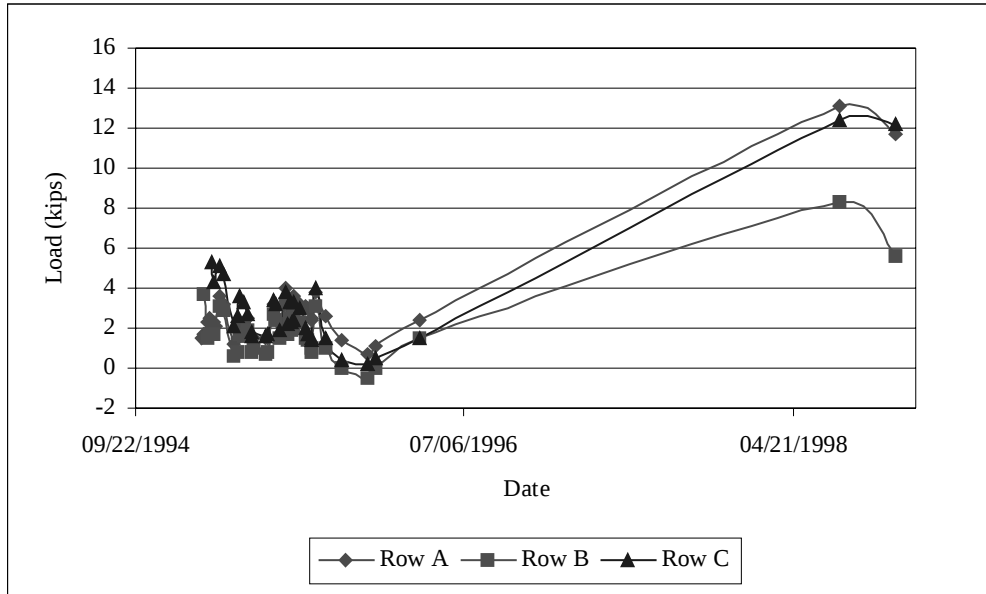
Figure 7.3: Wall Section 1 Load Cell Readings
