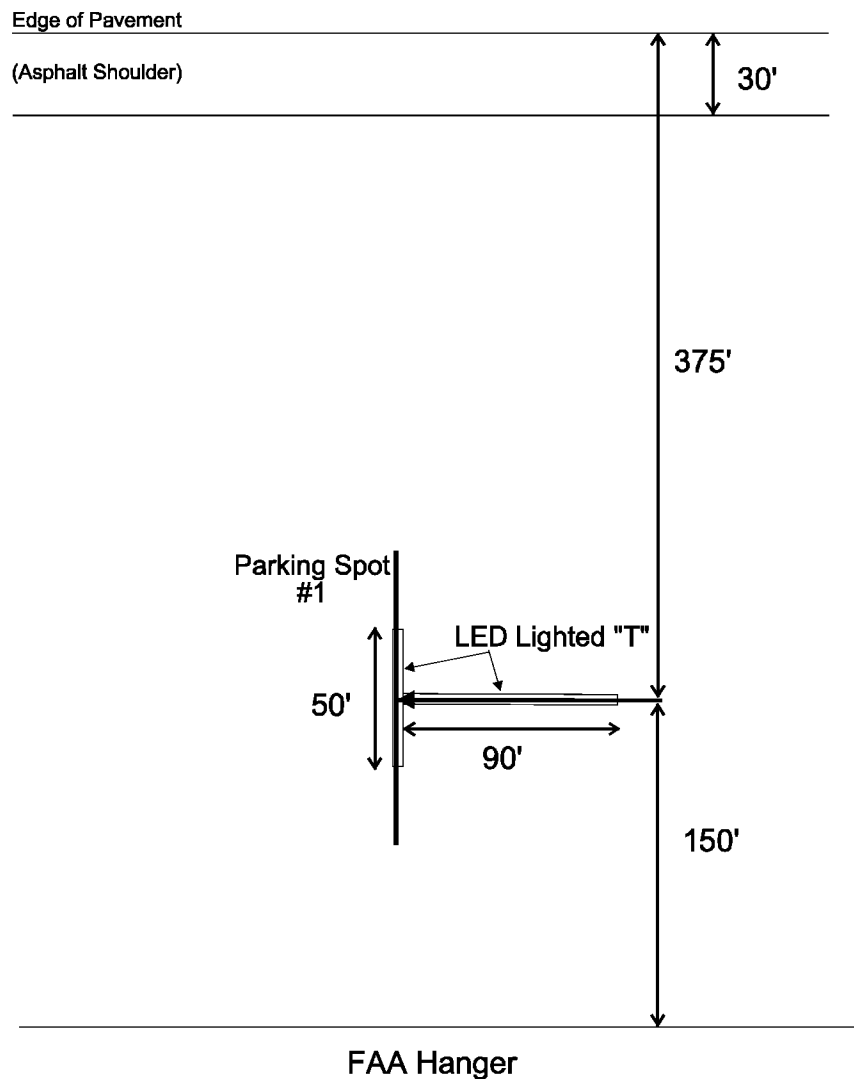
FIGURE 2. PARKING LOCATION INDICATOR LAYOUT
