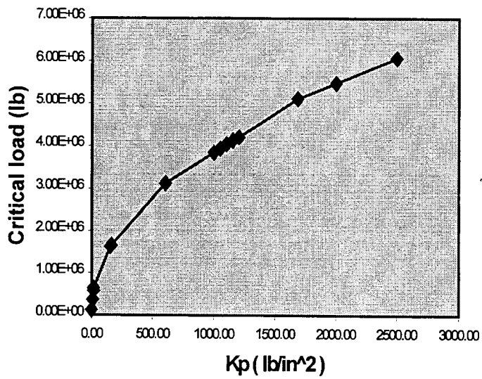
Fig. 5.4.1 Critical load ( L=45' , Simply Supported )
