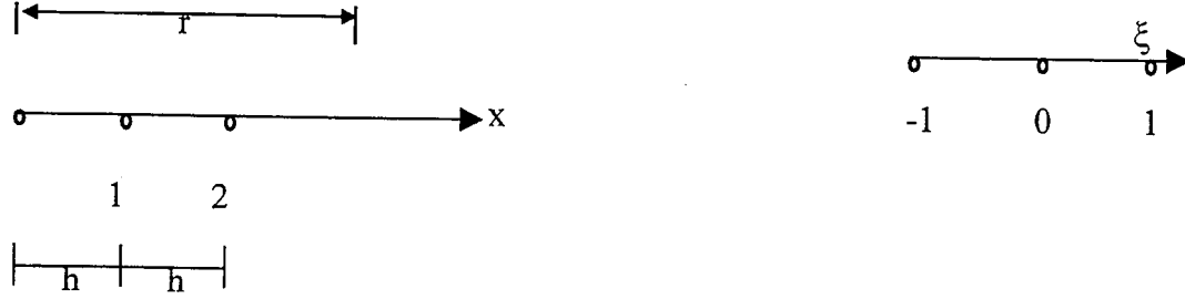
Fig.4.3.1 Mapping of an one-dimensional infinite element
