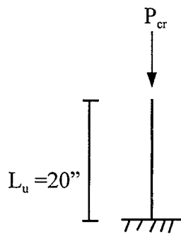
Fig. 4.5.1 Free-fixed column
