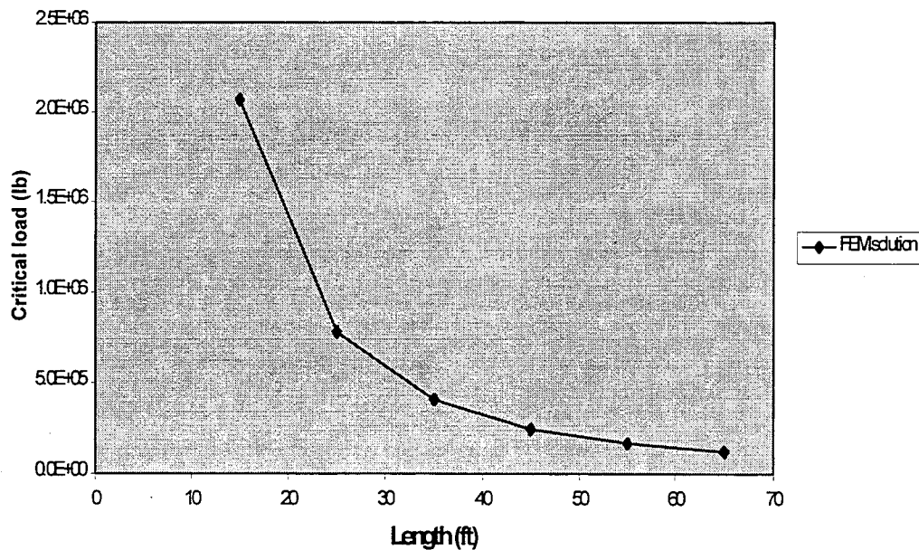
Fig. 5.46 Critical load ( K_p=0.0 , K_t=1000 \text{ lb/in}^2 , K_b=10000 \text{ lb/in} )
