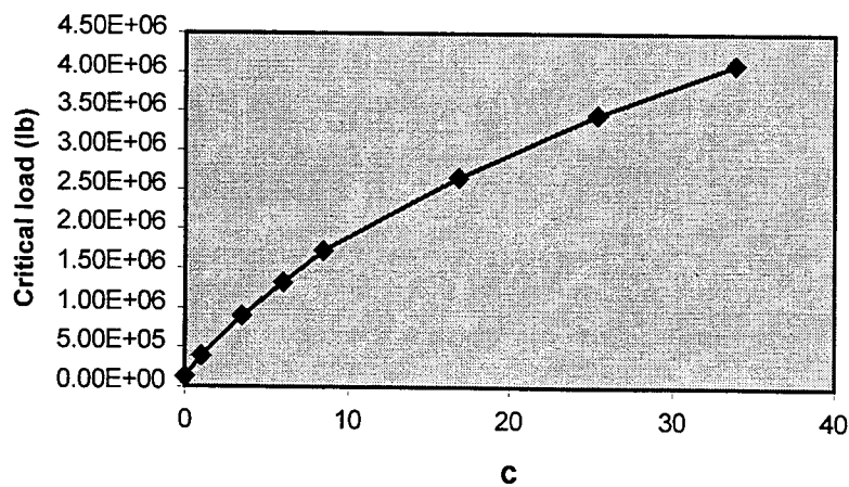
Fig. 5.4.3 Critical load ( L = 45' , Simply Supported, K_{p0} = c \cdot 18.0 , K_{t0} = c \cdot 180.0 )
