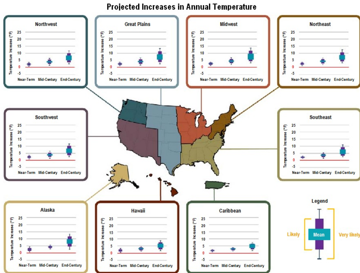
Figure 2.2. Projected changes in annual average air temperature for six regions of the U.S., Alaska, Hawaii, and the Caribbean through 2100, relative to 1961-1979 averages, compiled using the A2 (high) and B1 (low) scenarios. [Adapted from ICF International, 2010]
