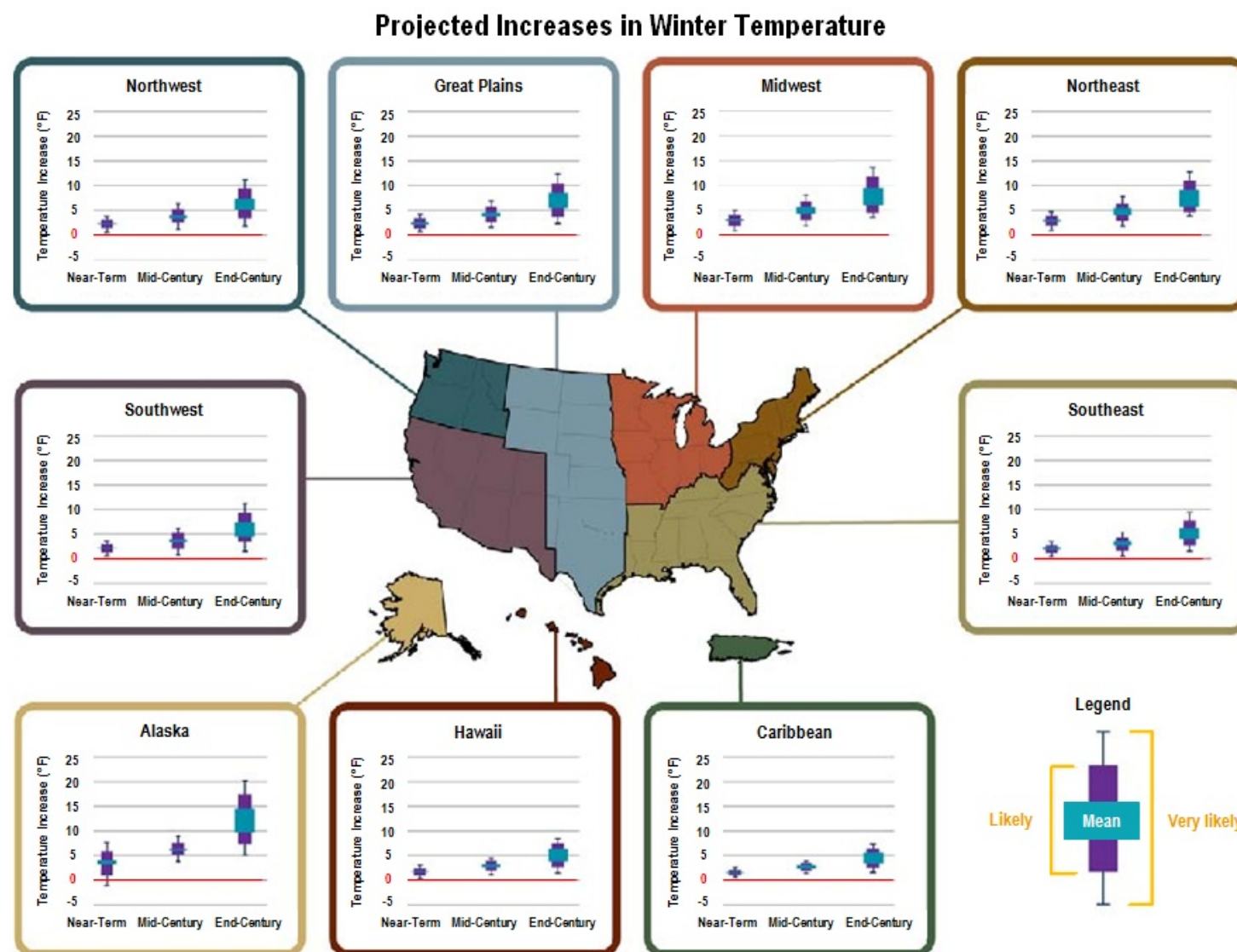
Figure 2.3. Projected changes in winter average air temperature for six regions of the U.S., Alaska, Hawaii, and the Caribbean through 2100, relative to 1961-1979 averages, compiled using the A2 (high) and B1 (low) scenarios. [Adapted from ICF International, 2010]
