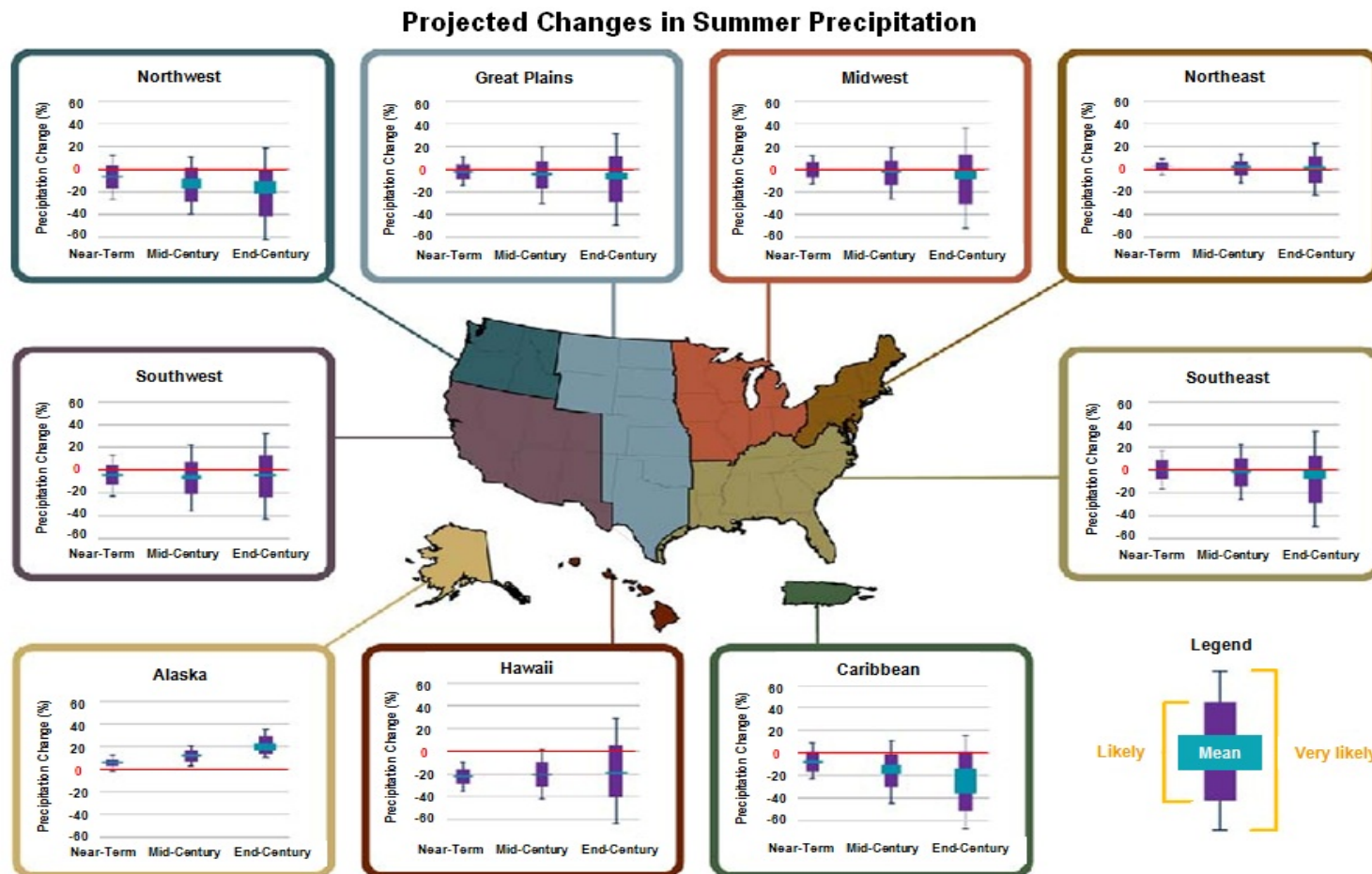
Figure 2.5. Projected changes in annual summer precipitation for six regions of the U.S., Alaska, Hawaii, and the Caribbean through 2100, relative to 1961-1979 averages, compiled using the A2 (high) and B1 (low) scenarios. [Adapted from ICF International, 2010]
