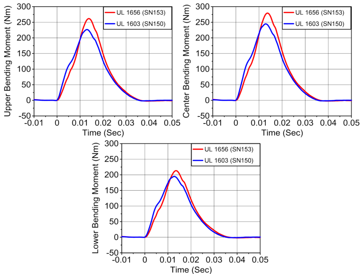
Figure 36. Reproducibility: 2016 Honda Fit femur bending moment time histories of impacts at ± 500 mm from centerline comparing impacts performed a couple months apart
