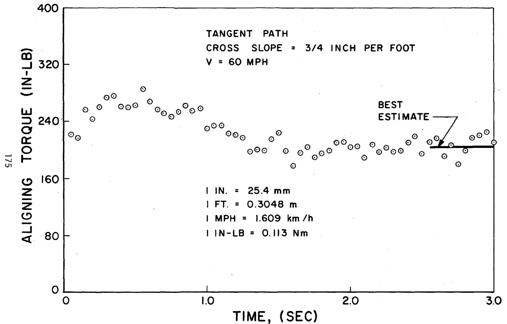
FIGURE A-5. RUN NO. 6 ALIGNING TORQUES
