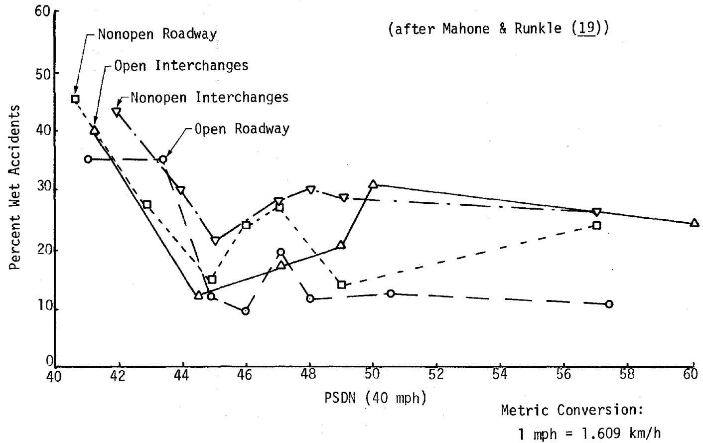
Figure 38. Variation of wet skidding accidents in traffic and passing lanes with stopping distance skid number (PSDN).
