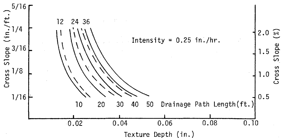
Figure 61. Curves of zero water depth for an intensity of 0.25 in./hr.
