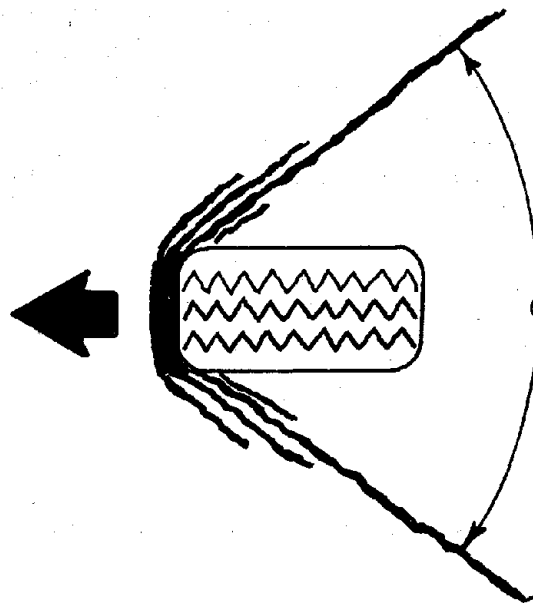
Figure 1. Viscous hydroplaning of smooth truck tire at 40 mph (64 km/h) in 0.080 in. (2 mm) of water (free rolling).
