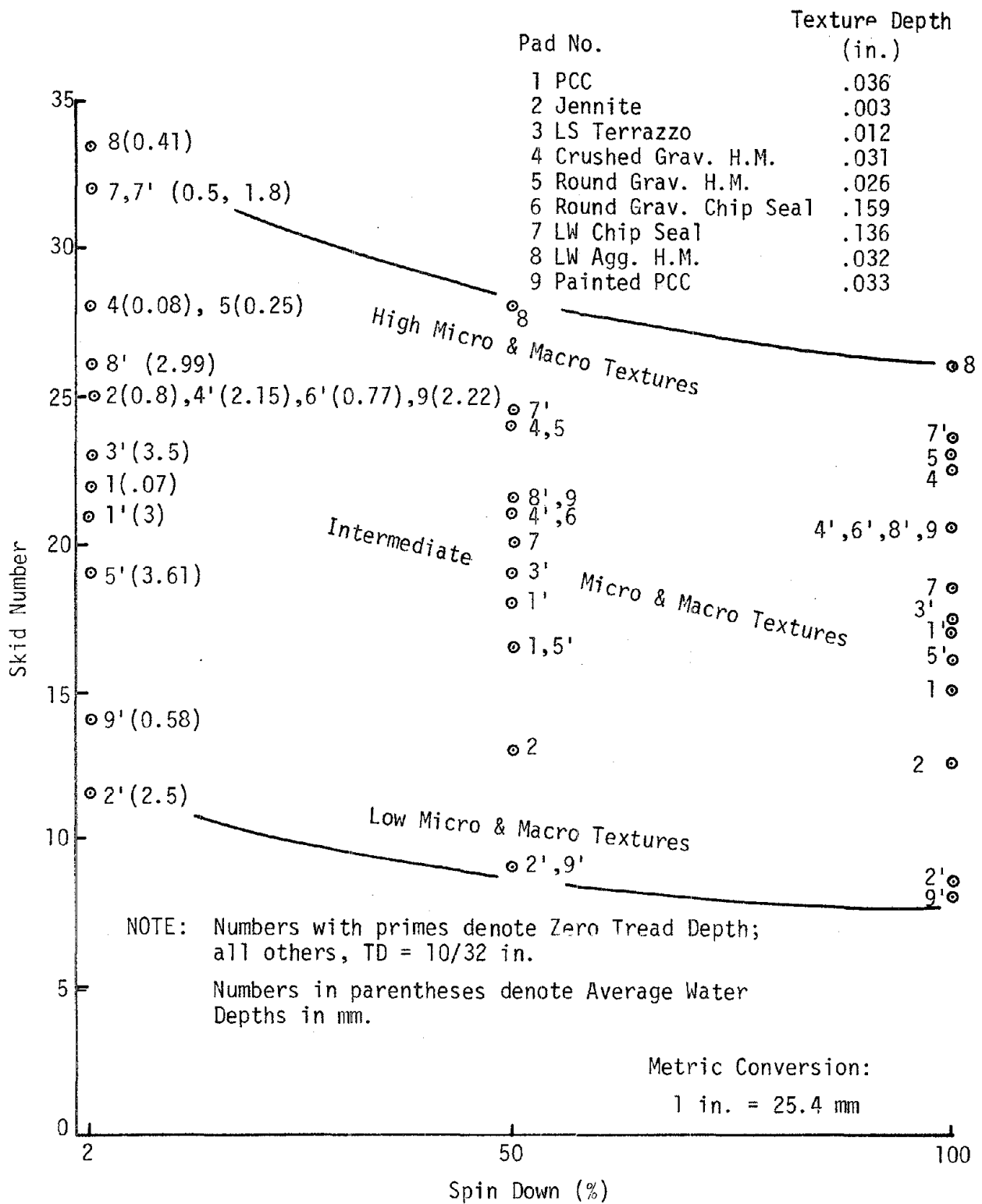
Figure 22. Skid numbers from 138 vs. spin down from 147.
