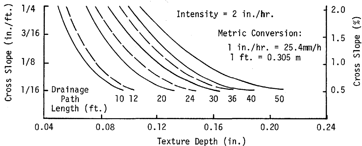
Figure 65. Curves of zero water depth for an intensity of 2 in./hr.
