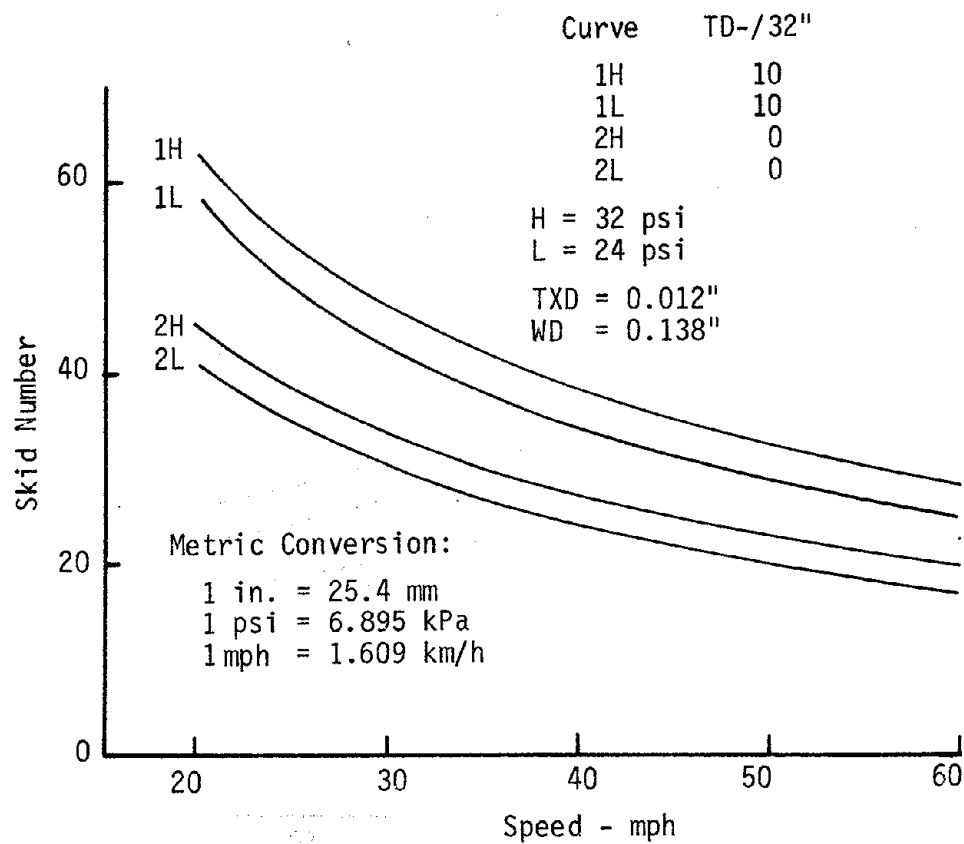
Figure 45. Effect of tire inflation pressure on skid numbers (SN) for the ASTM 14" (356 mm) tire at maximum water depth (WD), minimum and maximum tire tread depth (TD), on low texture depth pavement (TXD).
