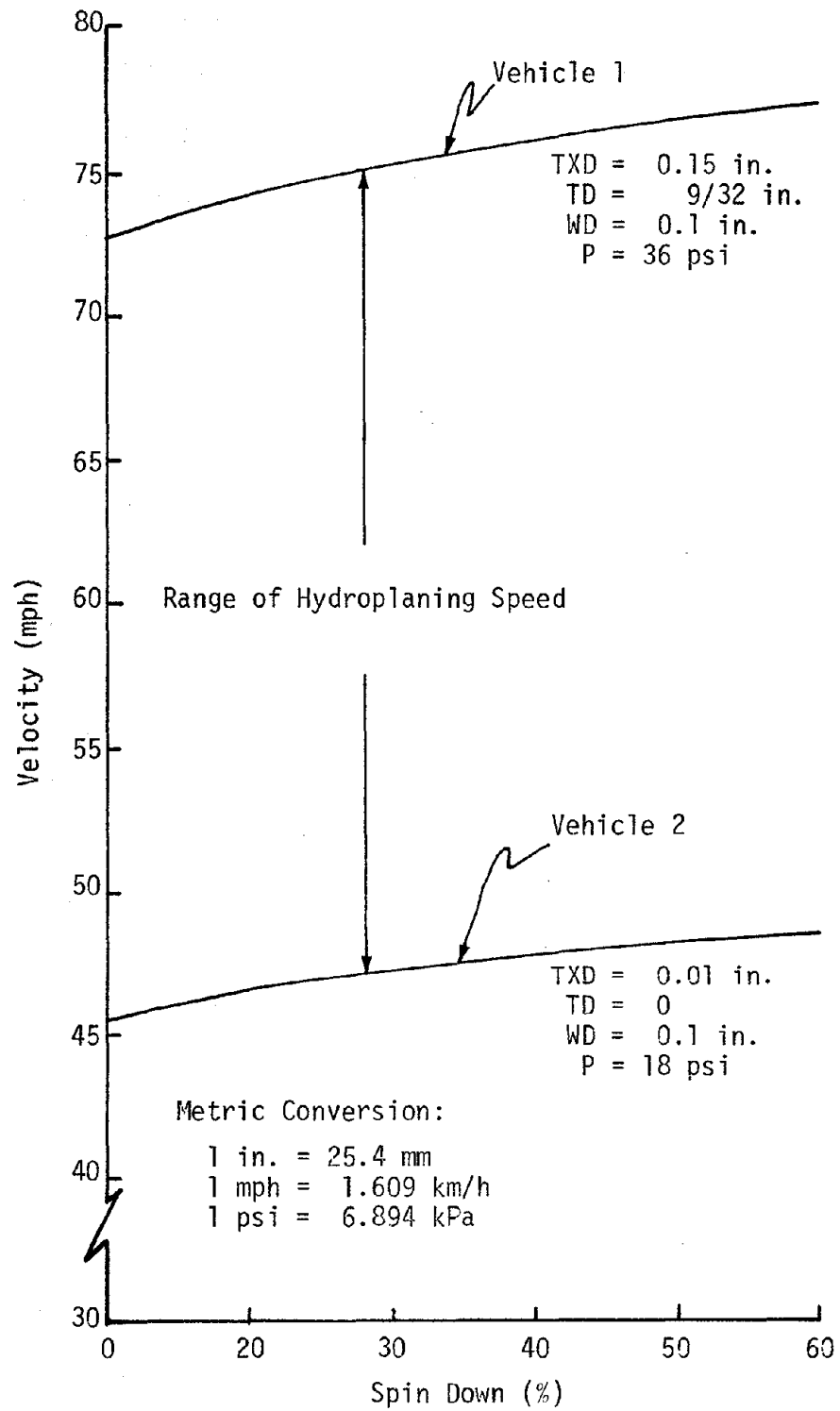
Figure 21. Possible range of hydroplaning speeds.
