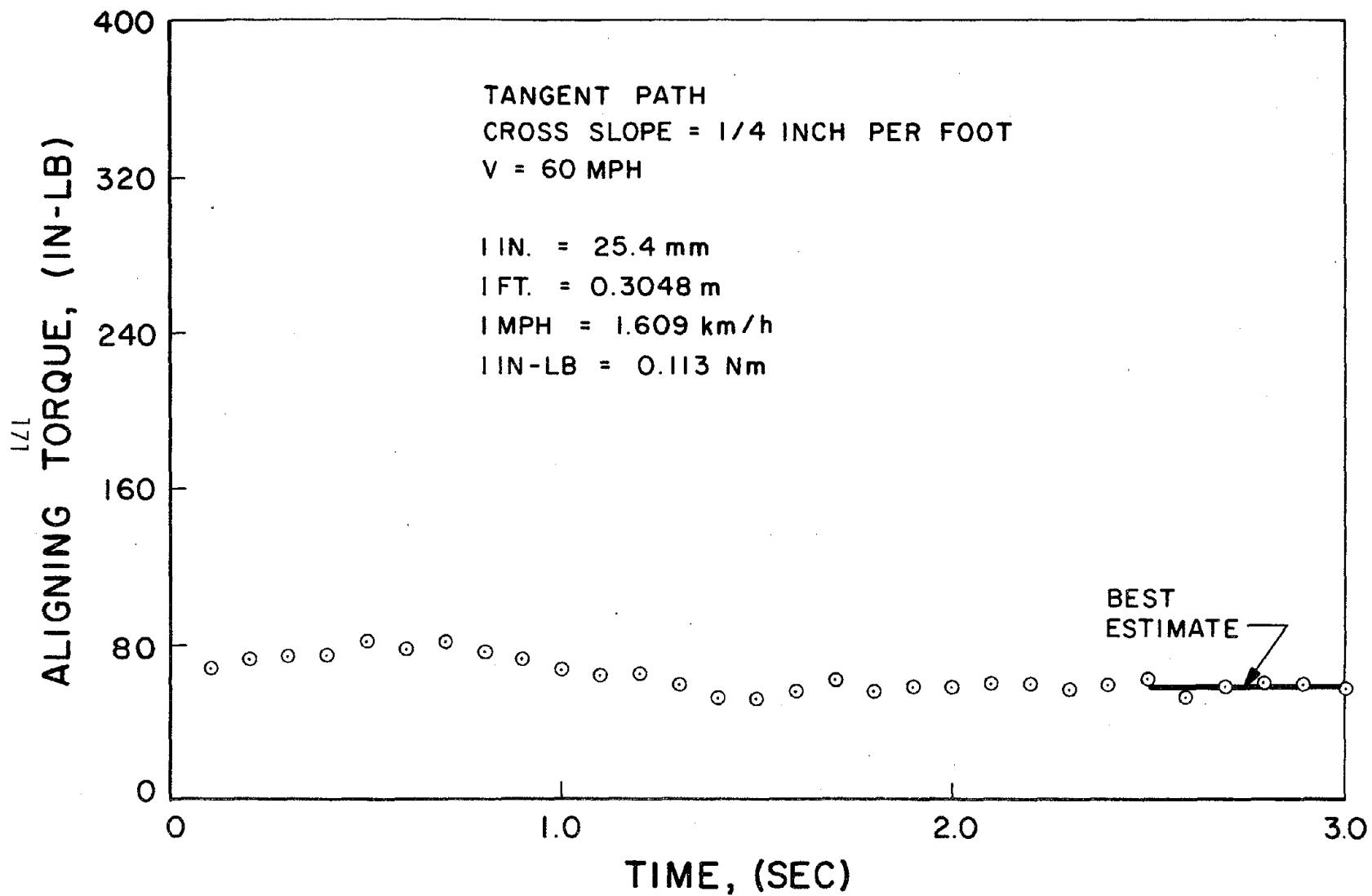
FIGURE A-1. RUN NO. 2 ALIGNING TORQUE
