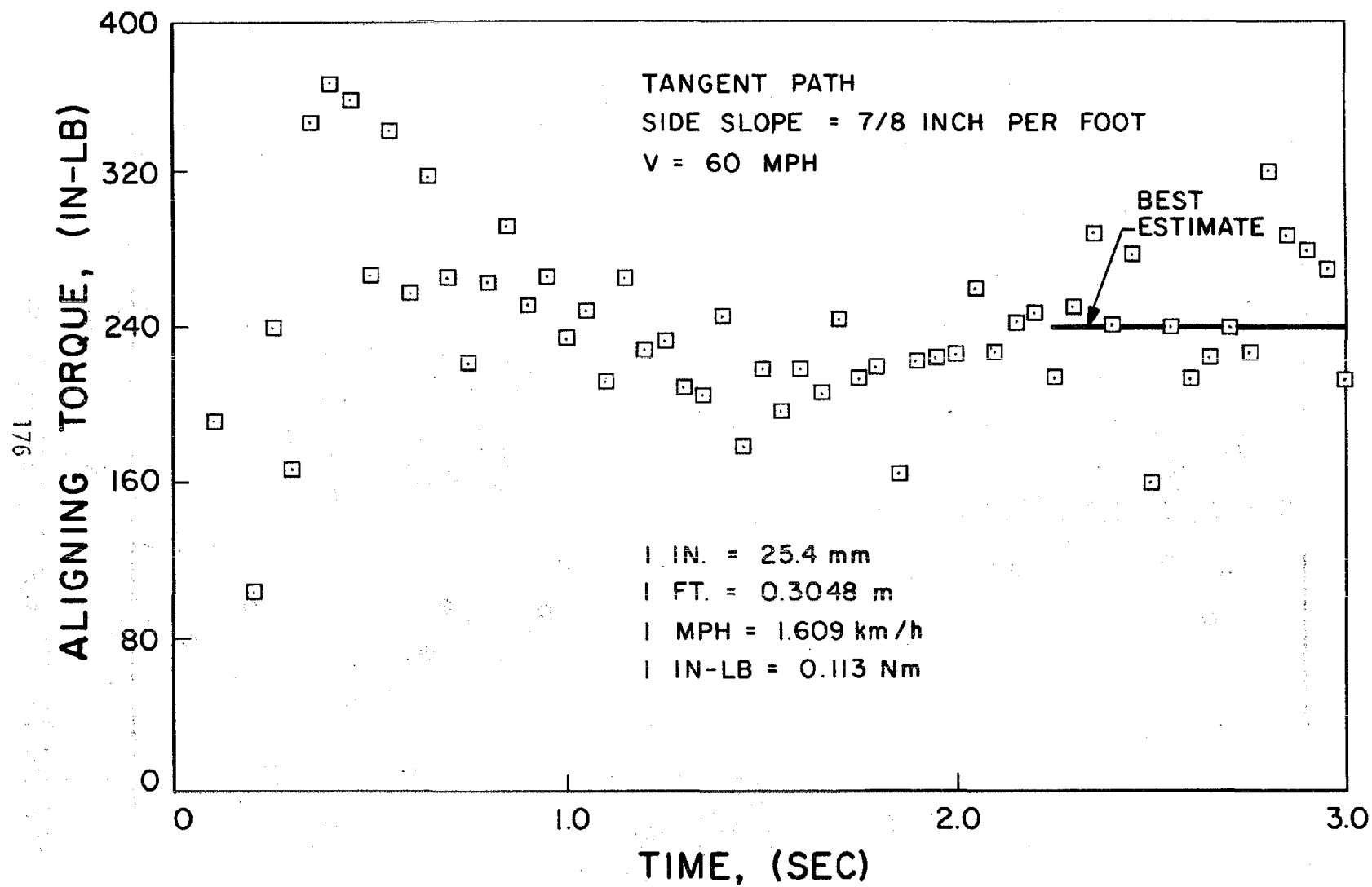
FIGURE A-6. RUN NO. 7 ALIGNING TORQUES
