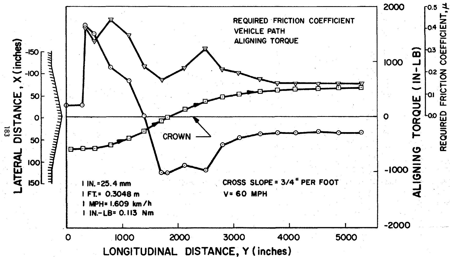
FIGURE B-5. RUN NO.14 RESULTS
