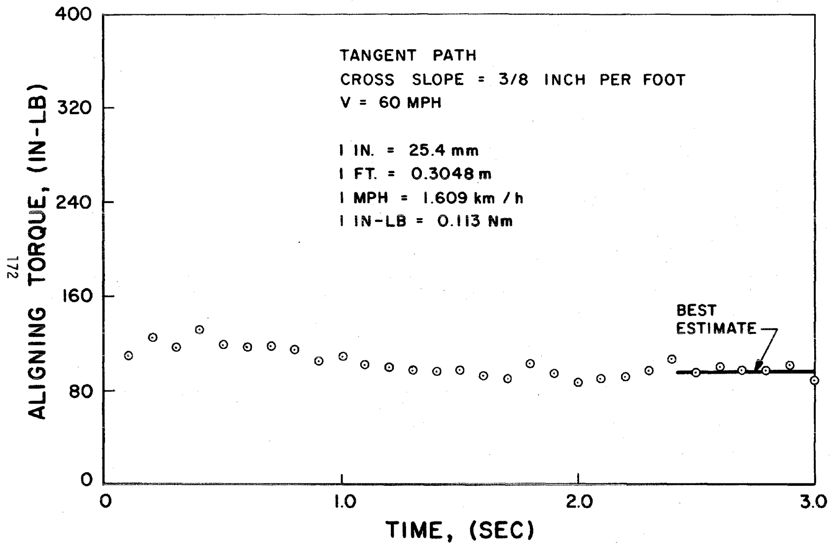
FIGURE A-2. RUN NO. 3 ALIGNING TORQUES
