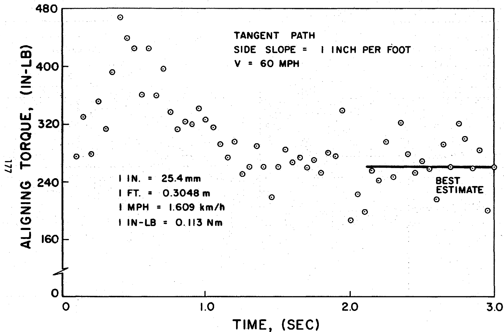
FIGURE A-7. RUN NO. 8 ALIGNING TORQUES
