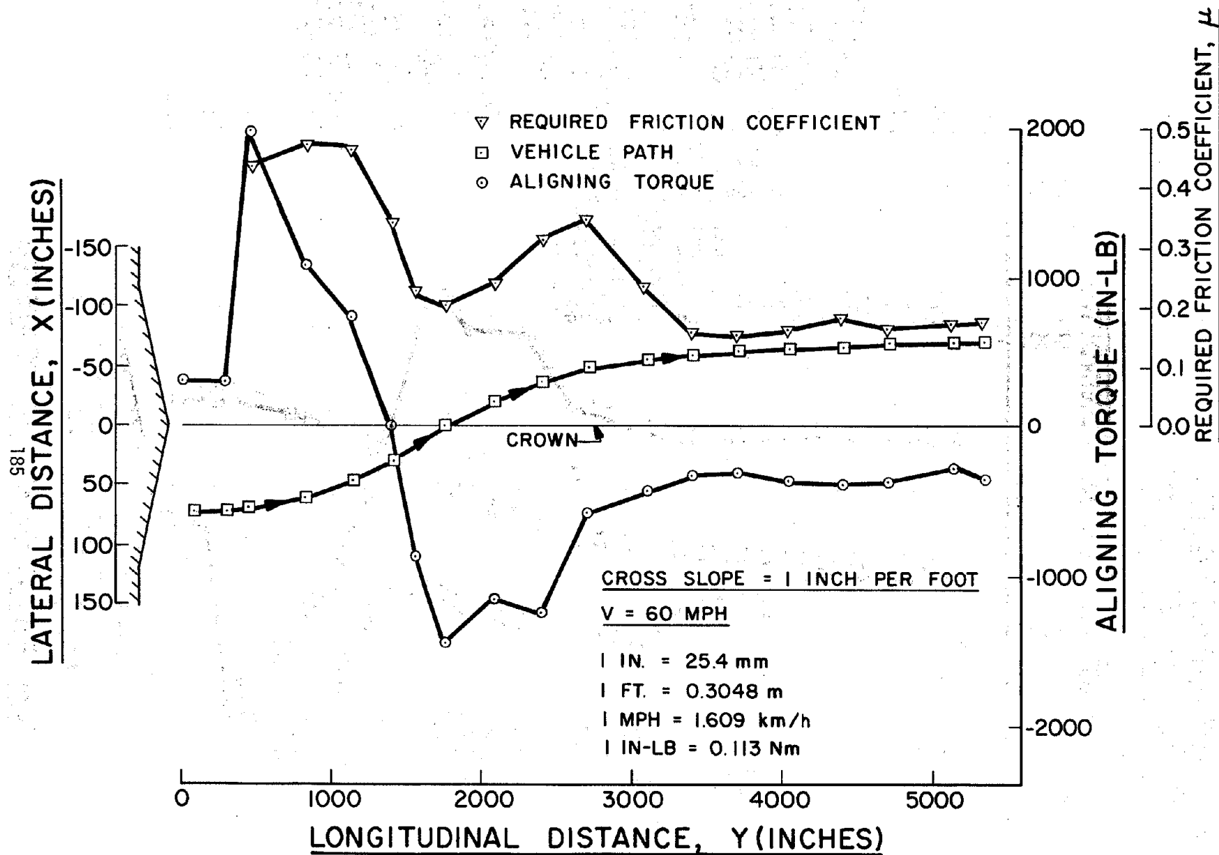
FIGURE B-7. RUN NO. 16 RESULTS
