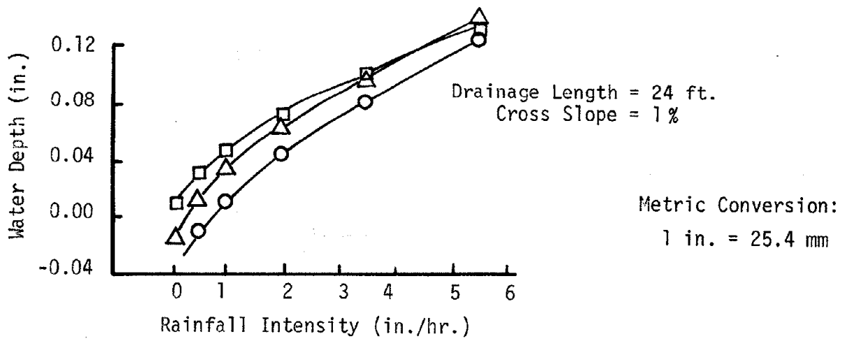
Figure 31. Plot of water depths vs. variables for combined surfaces (points calculated from Equation 18).
