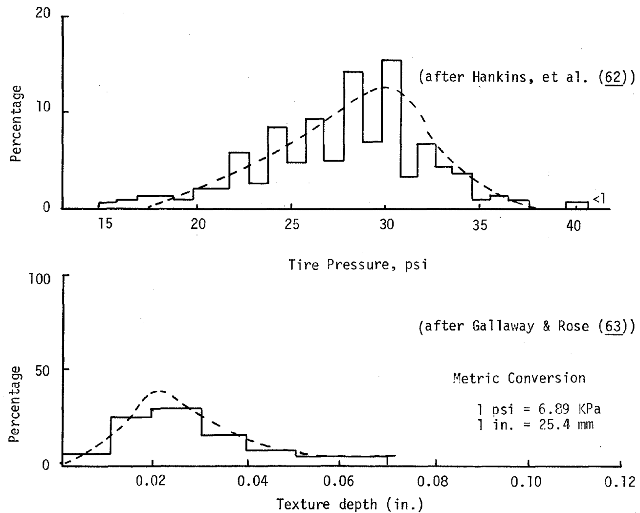
Figure 59. Approximate distributions of tire tread, tire pressure and surface texture for one state.
