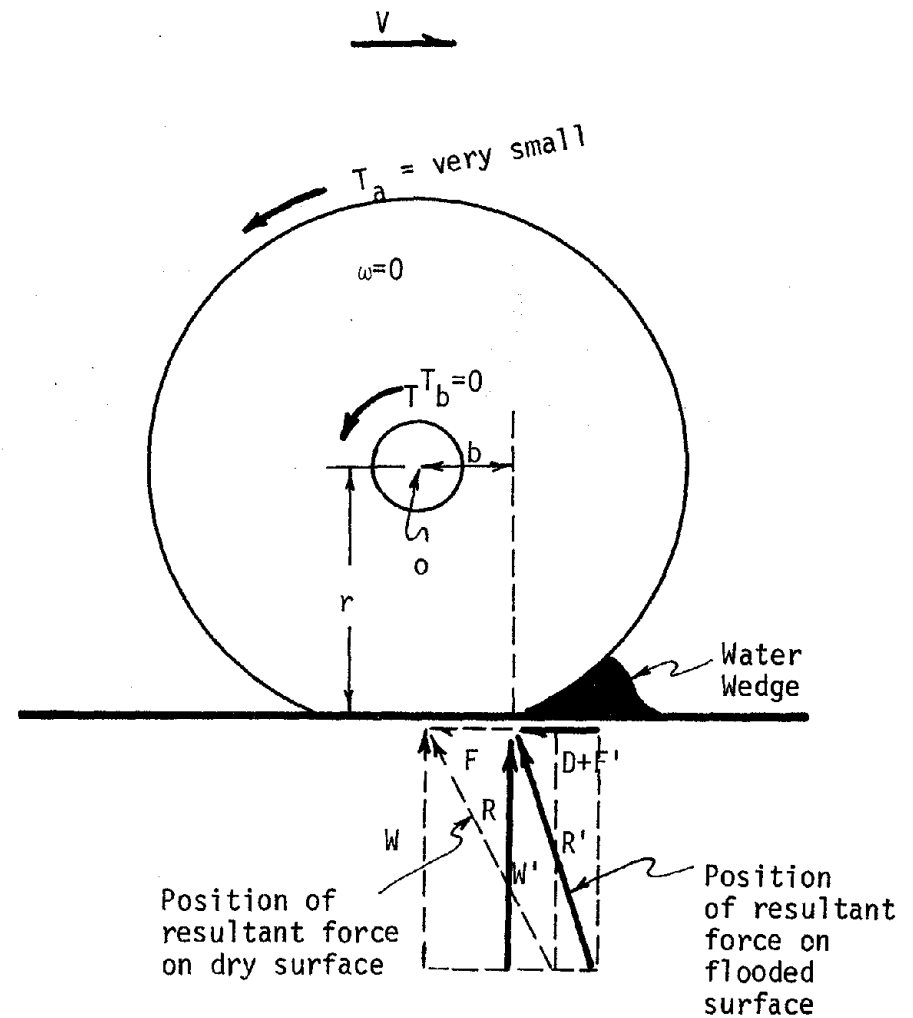
Figure 11(b). Wheel not turning, 100% spin down condition.
