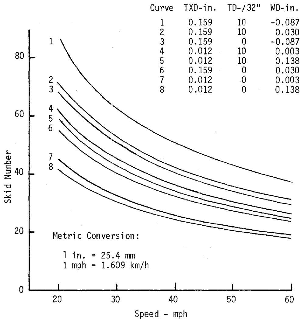
Figure 43. Effects of pavement texture depth (TXD), tire tread depth (TD), and water depth (WD) on the skid number (SN) at speeds of 20 mph to 60 mph (32 to 97 km/h), ASTM-14" (356 mm), 24 psi (165.5 kPa) tire inflation pressure.
