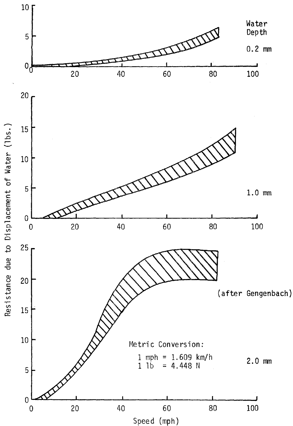
Figure 25. Resistance due to the displacement of water as a function of velocity for different water depths.
