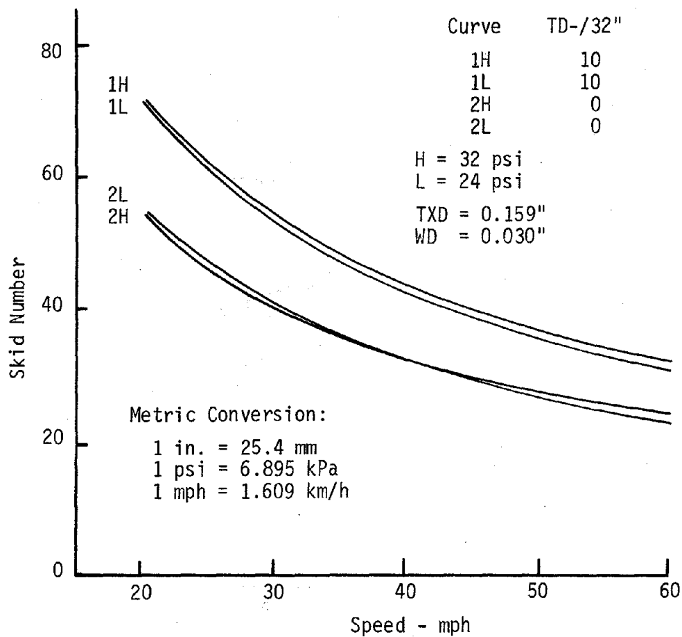
Figure 47. Effect of tire inflation pressure on skid numbers (SN) for the ASTM 14" (356 mm) tire at maximum water depth (WD), minimum and maximum tire tread depth (TD) on high texture depth pavement (TXD).
