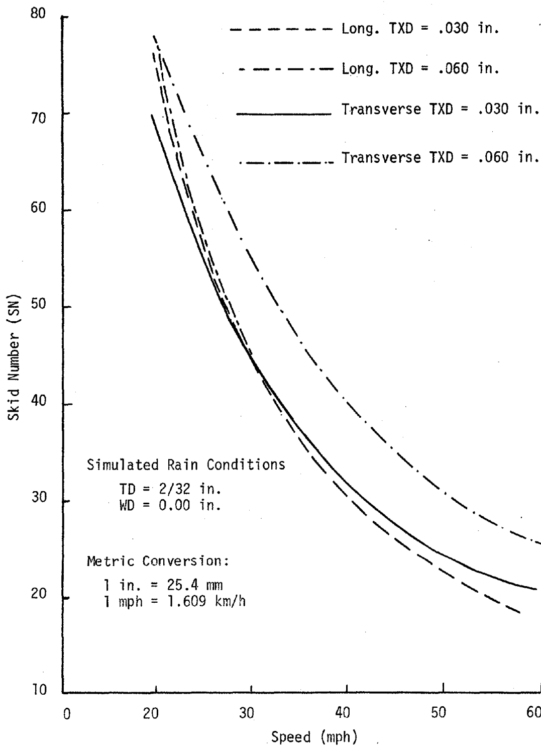
Figure 53. Effect of vehicle speed on skid number for tread depth of 2/32 in. and water depth of 0.00 in. (curves calculated from equations).
