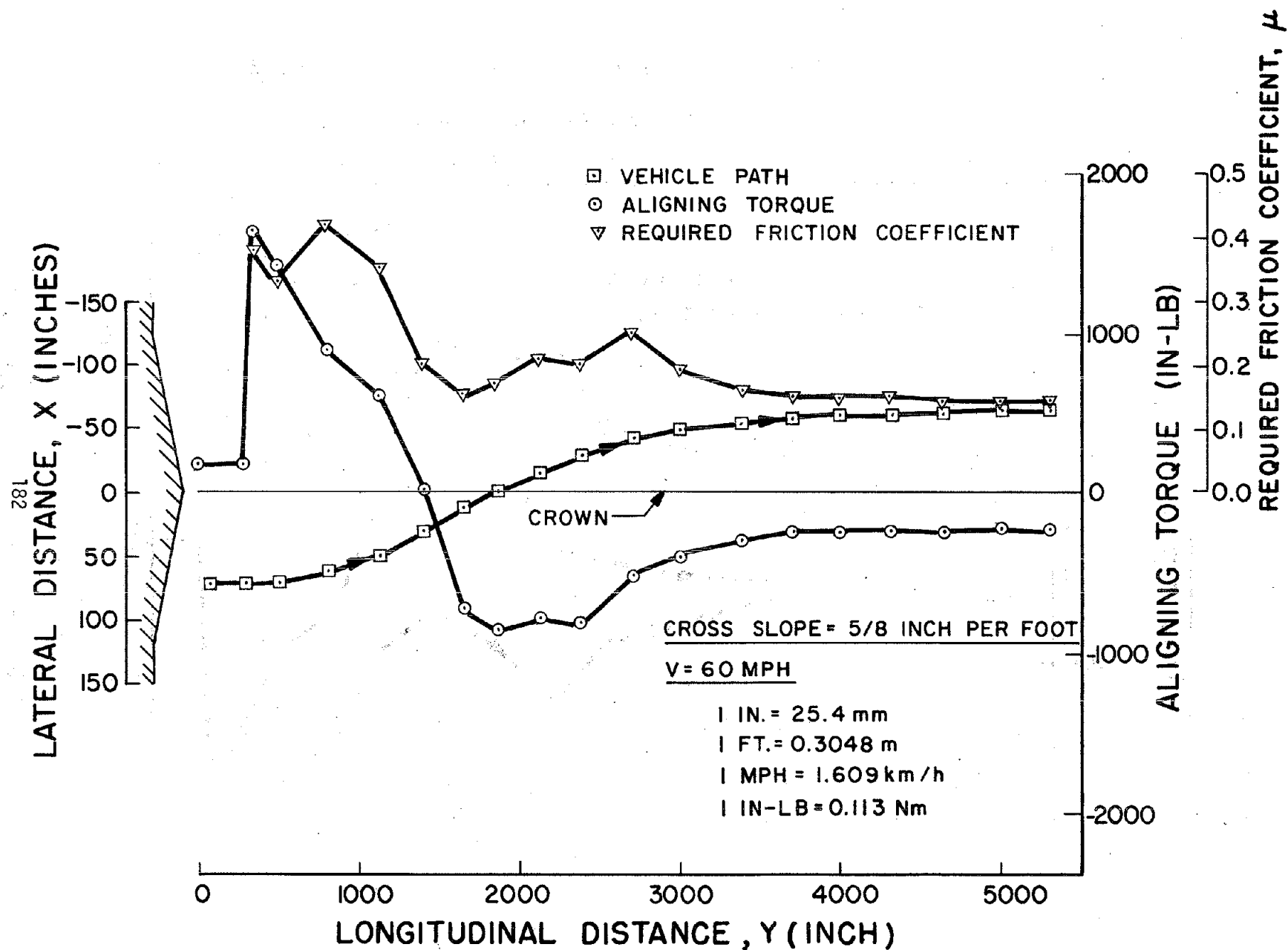
FIGURE B-4. RUN NO.13 RESULTS
