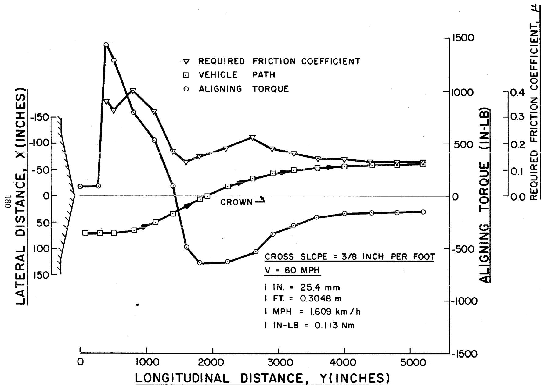
FIGURE B-2. RUN NO. II RESULTS
