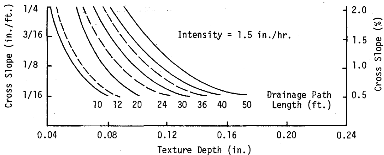
Figure 64. Curves of zero water depth for an intensity of 1.5 in./hr.
