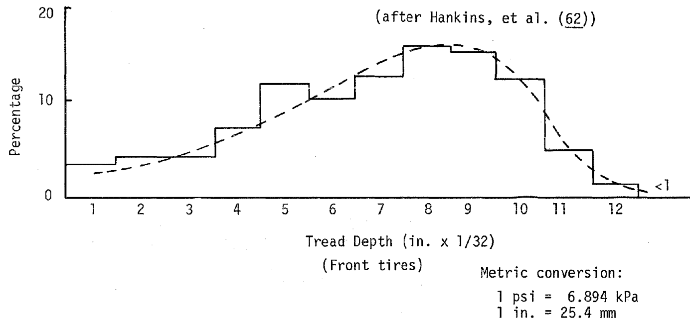
Figure 59. Approximate distributions of tire tread, tire pressure and surface texture for one state. (continued next page)
