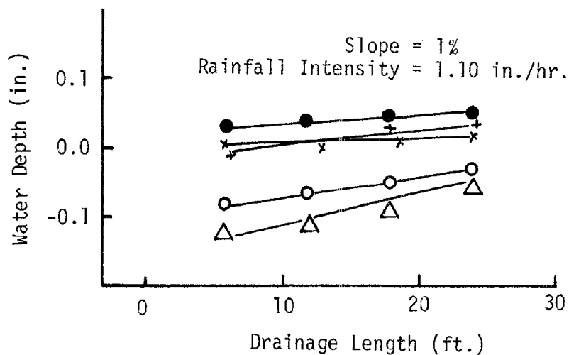
Figure 32. Plot of water depths vs. variables of selected individual surfaces (observed or average data points). (continued next page)
