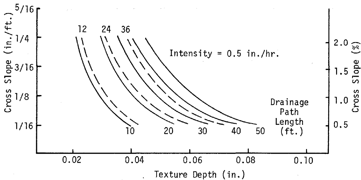
Figure 62. Curves of zero water depth for an intensity of 0.5 in./hr.
