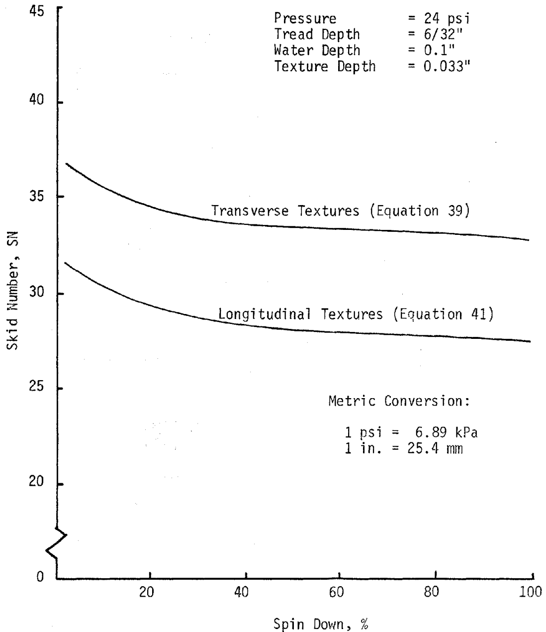
Figure 26. Effect of texture direction on skid numbers at calculated values of spin down.
