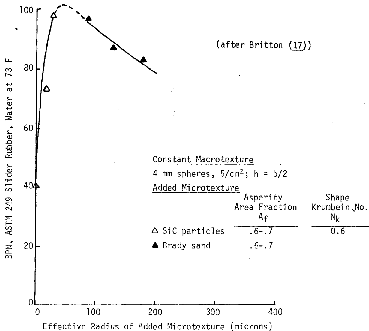
Figure 41. Variation of British Pendulum Number (BPN) with microtexture size and shape added to 4 mm glass spheres.
