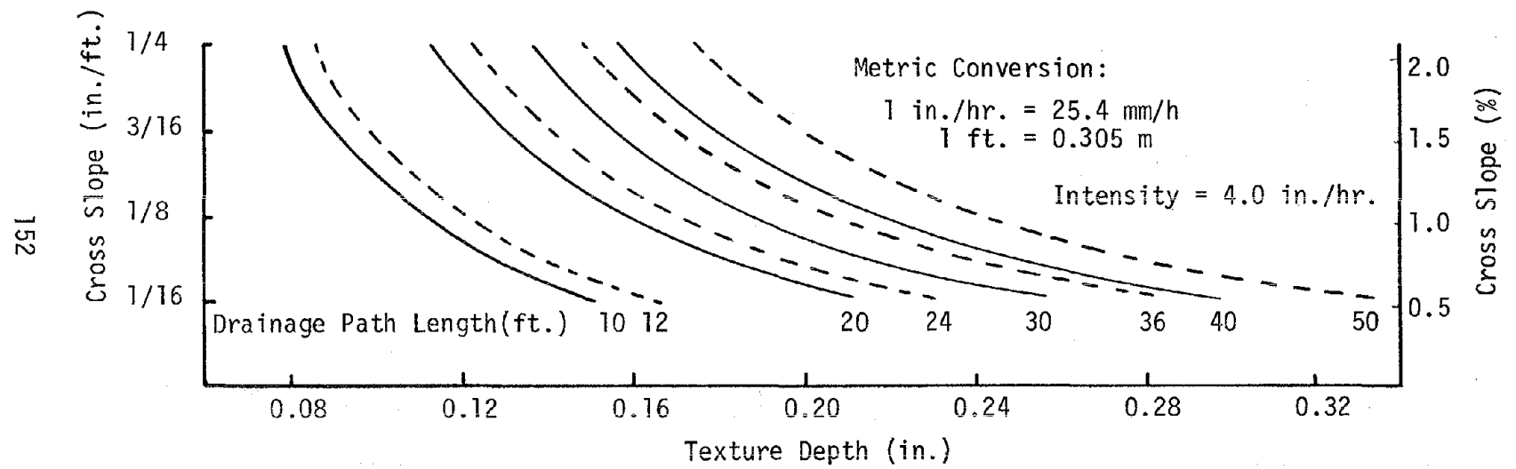
Figure 66. Curves of zero water depth for an intensity of 4.0 in./hr.
