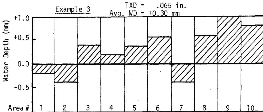
Figure 23. Variation of water depth during rainmaker SN tests.
