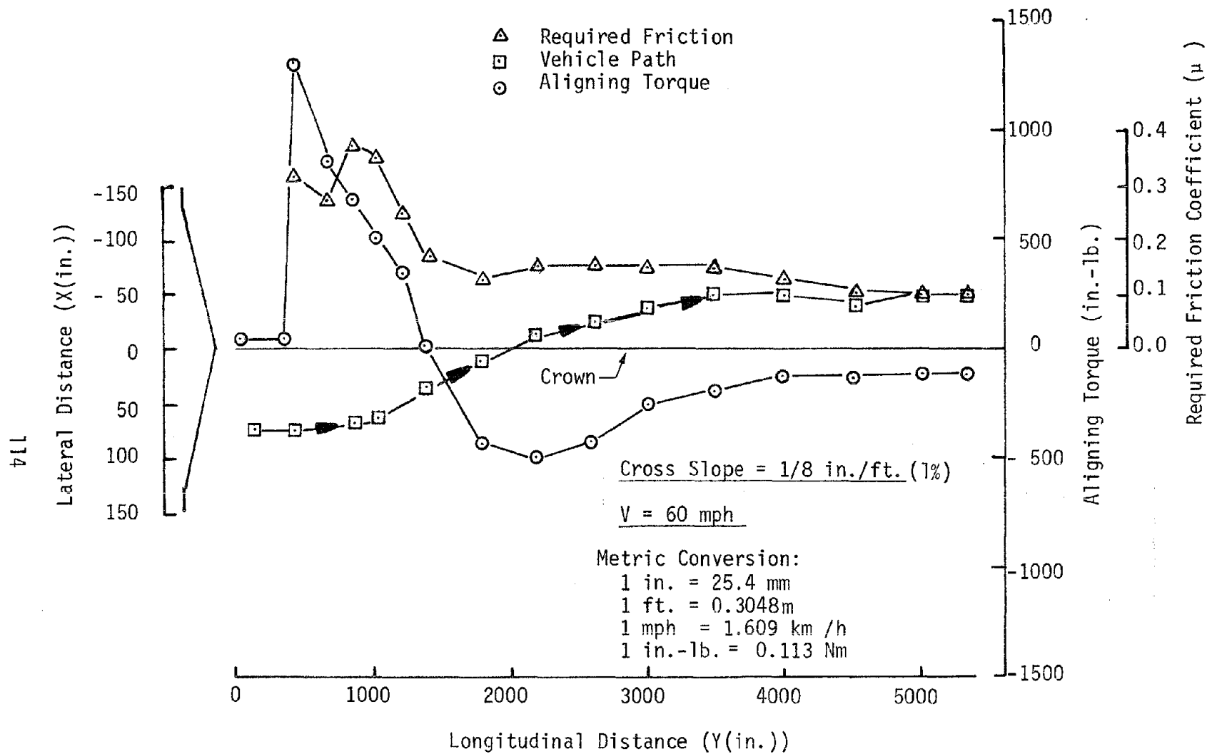
Figure 57. Run No. 9 results.
