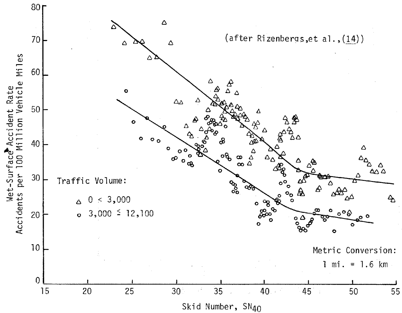
Figure 33. Skid number versus accident rate.
