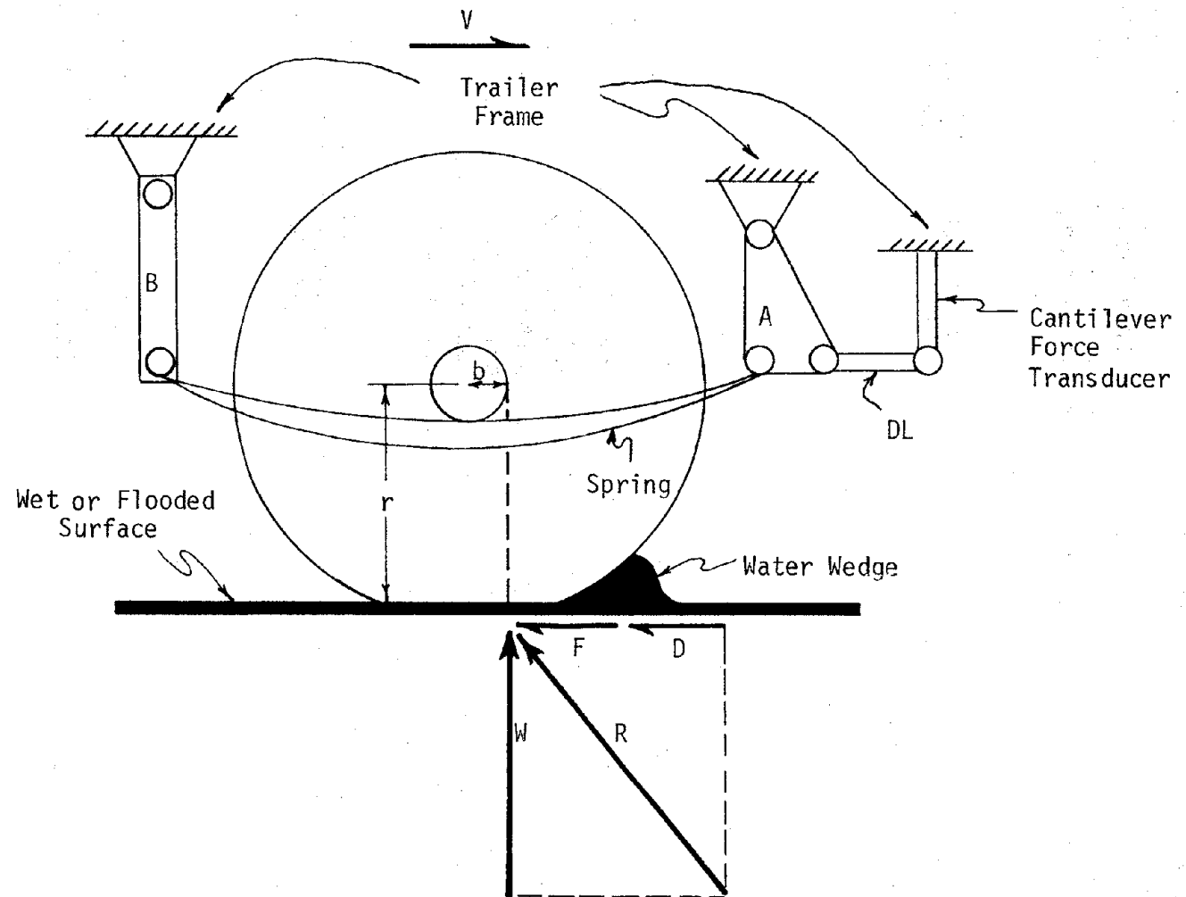
Figure 12. Skid number trailer - drag link force measurement system and interface force diagram.
