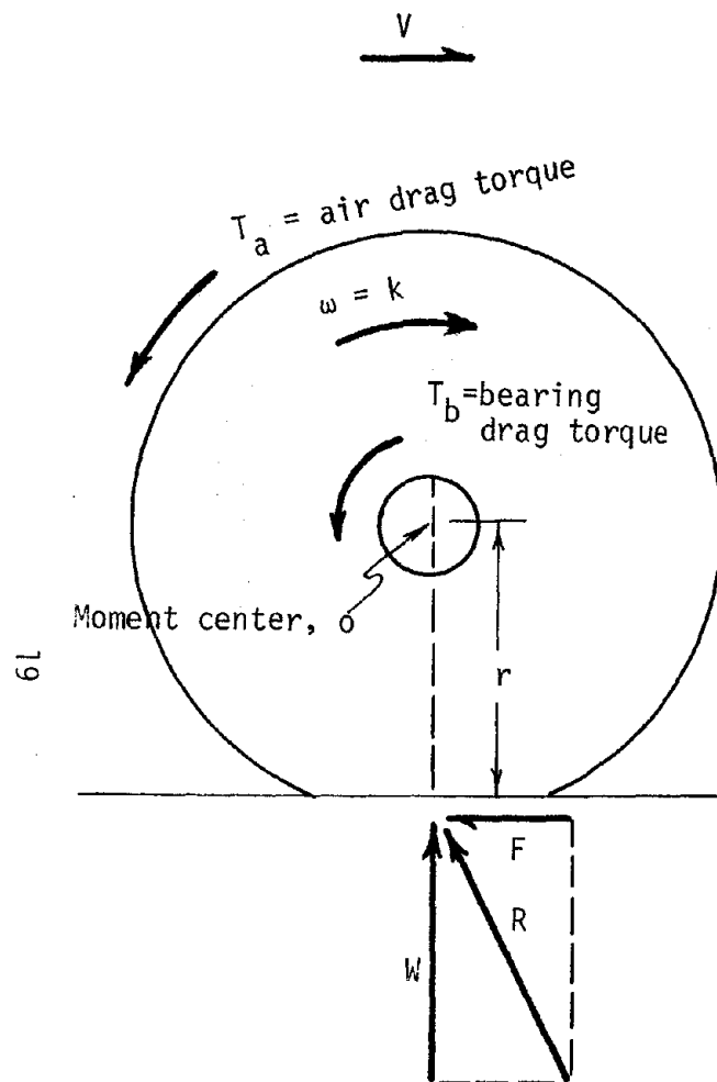
Figure 11(a). Wheel freely rolling on dry surface.
