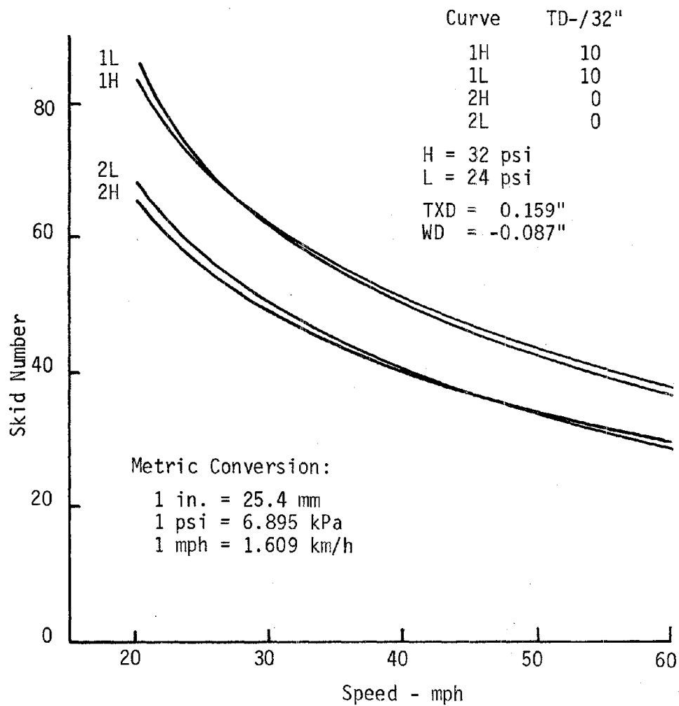
Figure 46. Effect of tire inflation pressure on skid numbers (SN) for the ASTM 14" tire at minimum depth (WD), minimum and maximum tire tread depth (TD) on high texture depth pavement (TXD).
