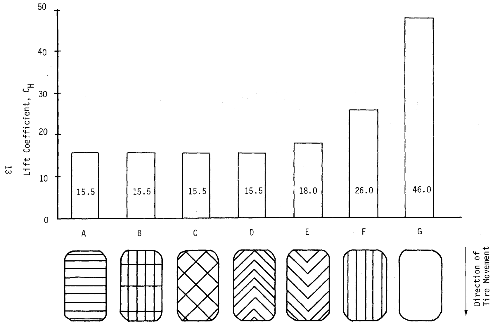
Figure 9. Influence of tread pattern on lift coefficient.
