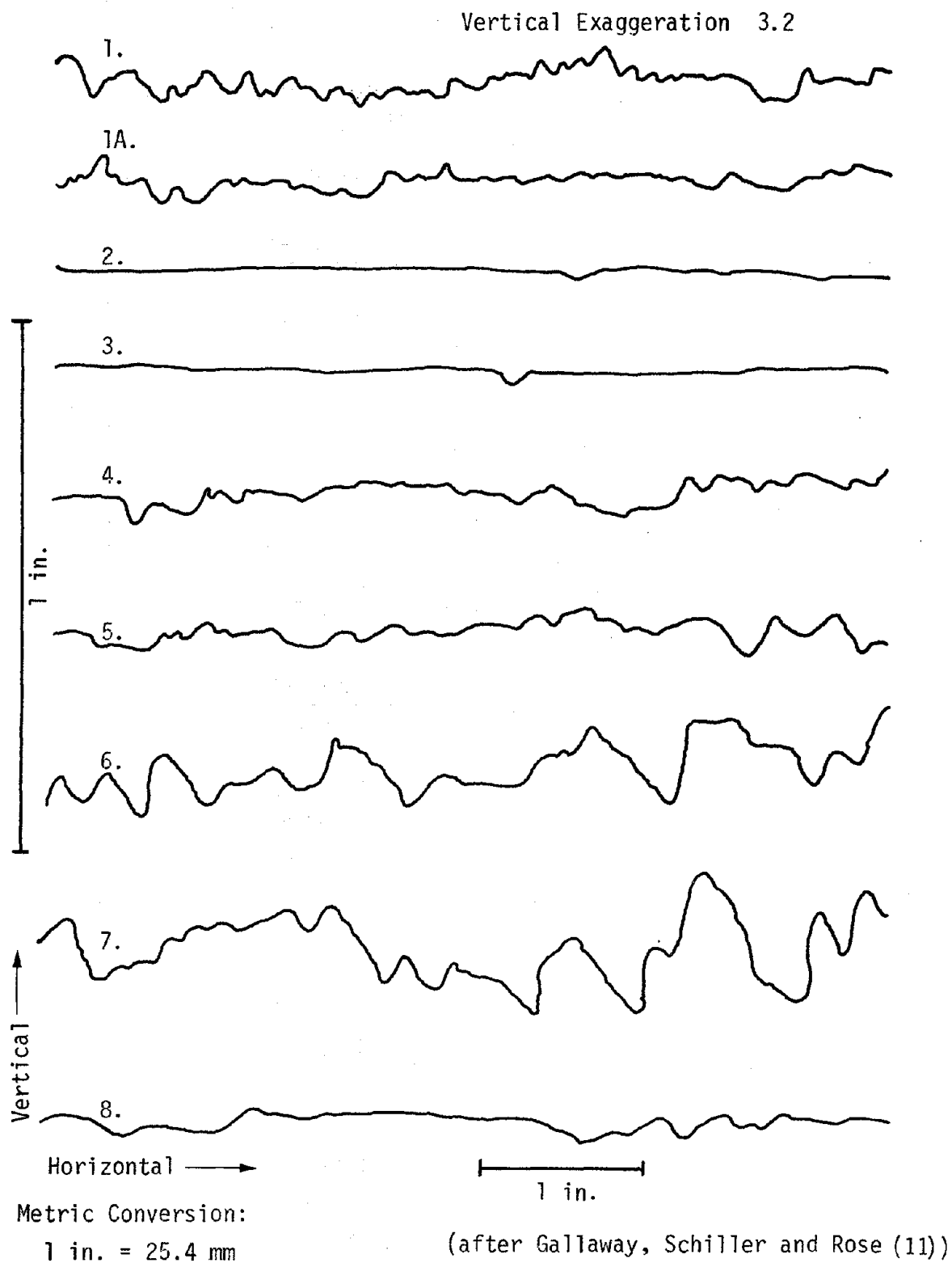
Figure 29. Textural profiles of the surfaces.
