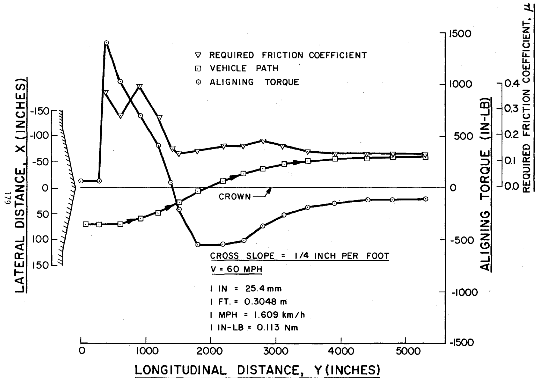
FIGURE B-I. RUN NO. 10 RESULTS
