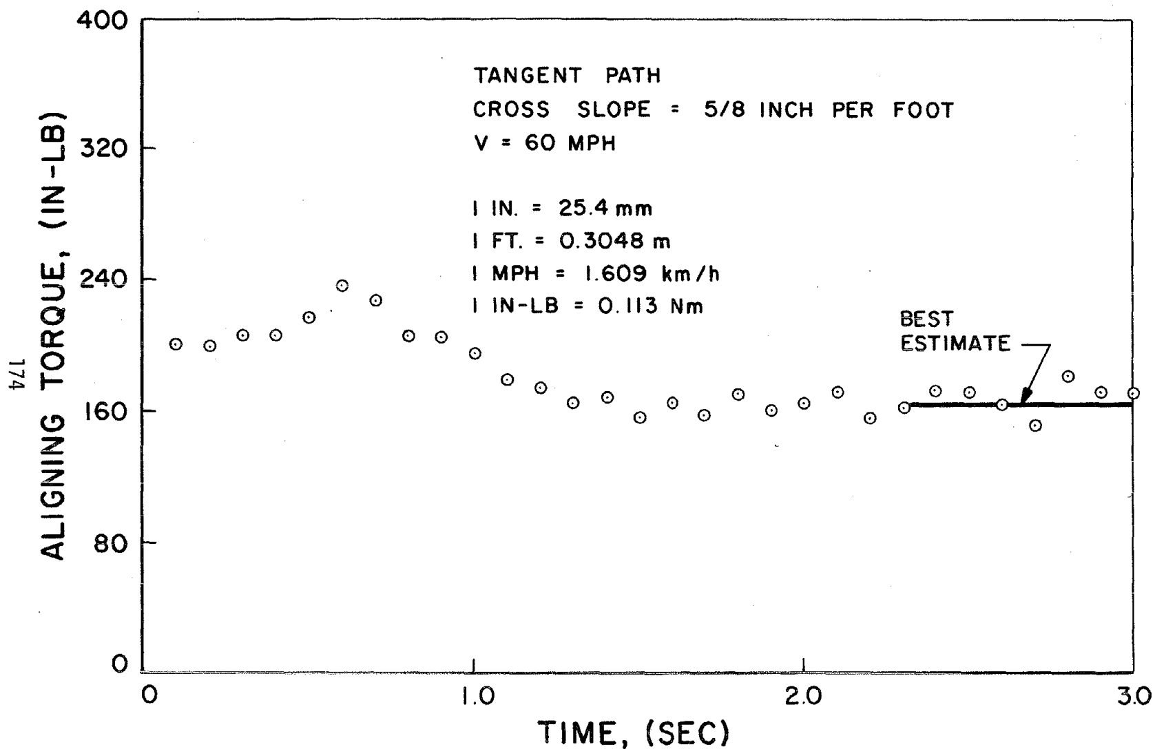
FIGURE A-4. RUN NO. 5 ALIGNING TORQUES
