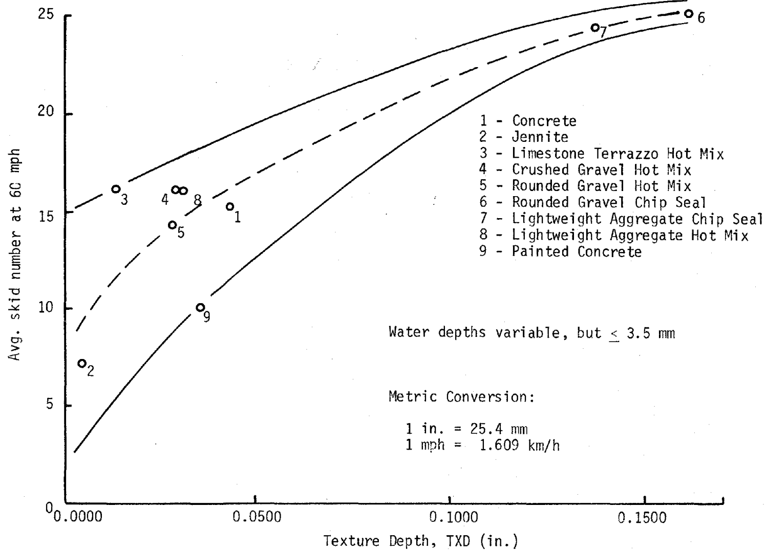
Figure 24. 60 mph skid numbers vs. texture depths.
