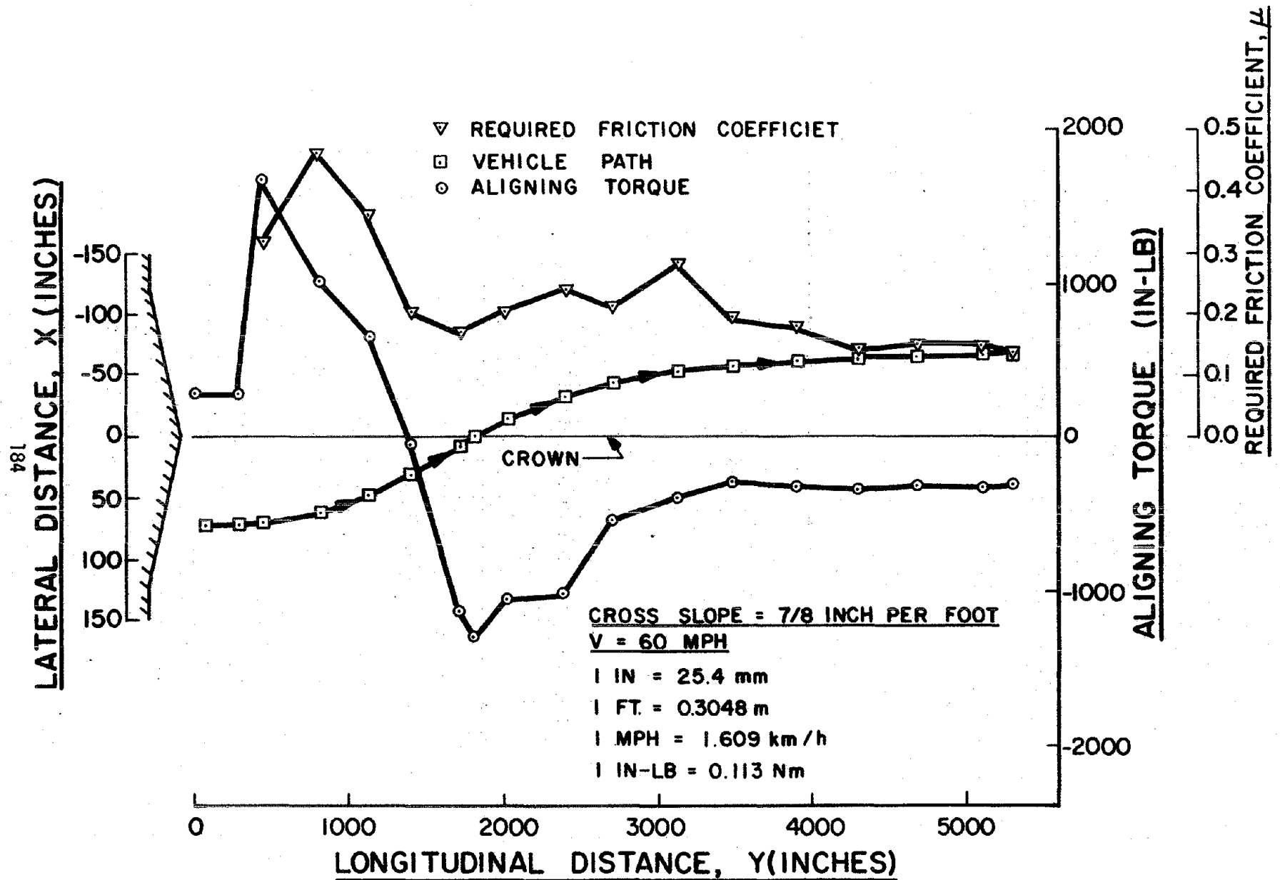
FIGURE B-6. RUN NO. 15 RESULTS
