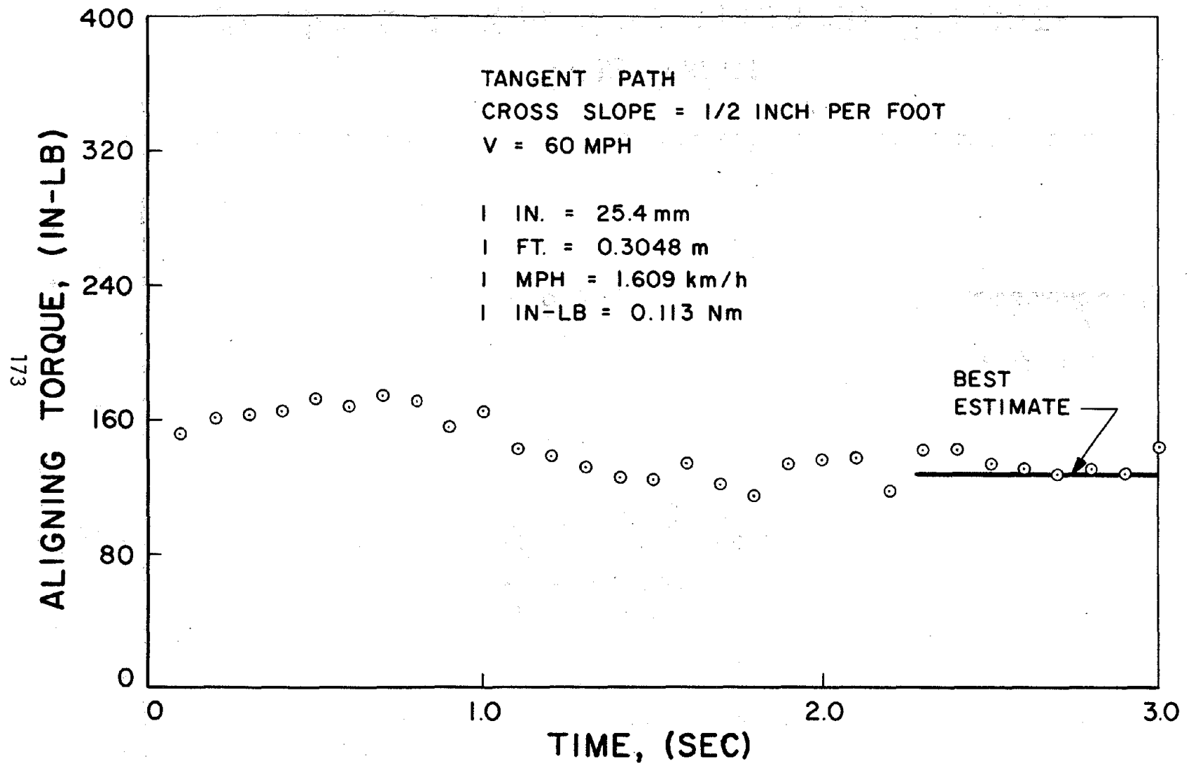
FIGURE A-3. RUN NO. 4 ALIGNING TORQUES
