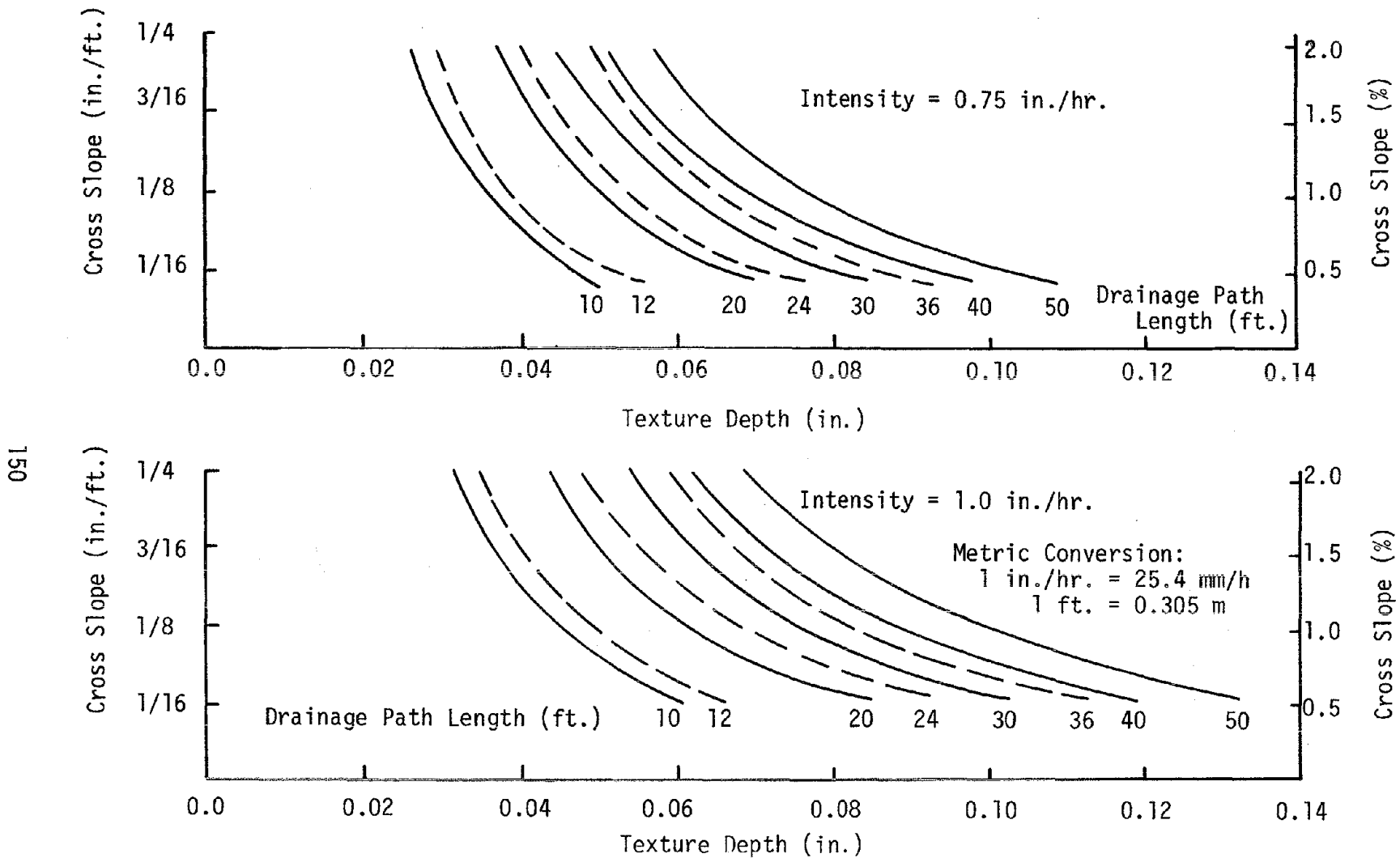
Figure 63. Curves of zero water depth for intensities of 0.75 and 1.0 in./hr.
