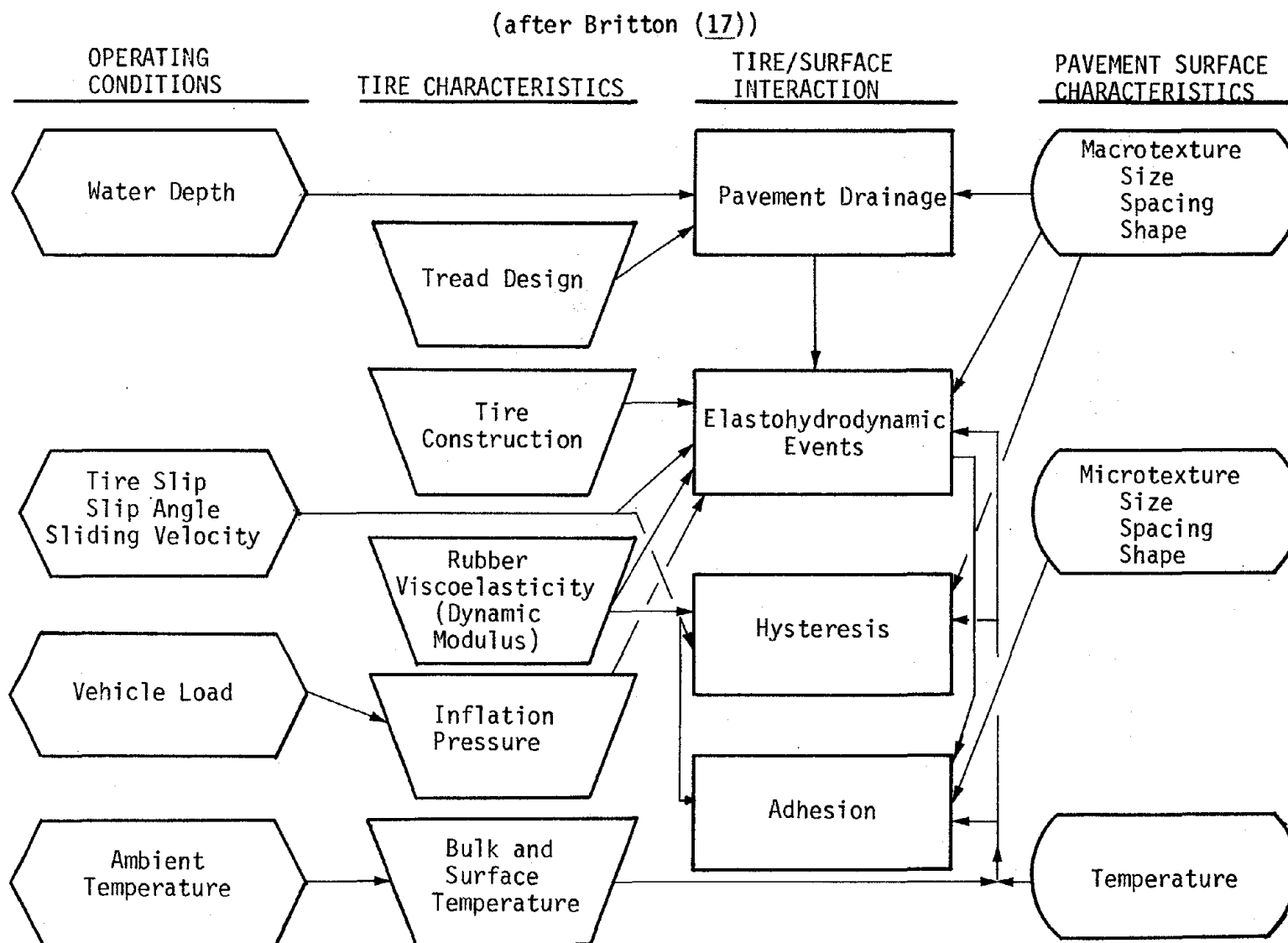
Figure 39. Interrelation among variables influencing automobile skidding on wet pavements.
